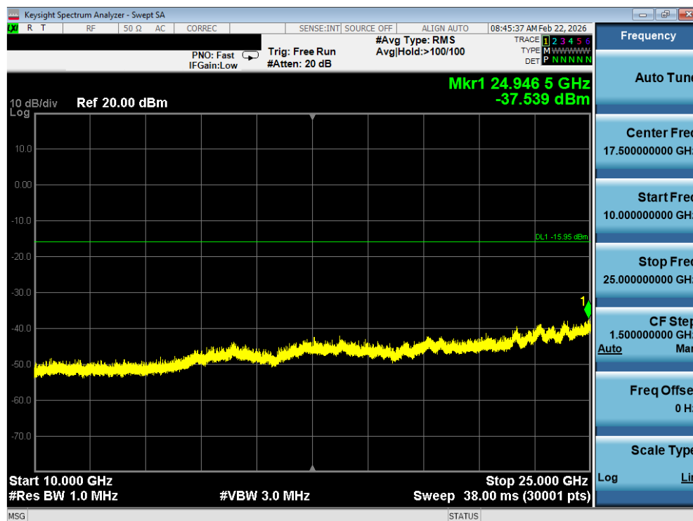
Plot 7-36. Conducted Spurious Plot (Bluetooth (LE), 2Mbps – Ch. 17)
