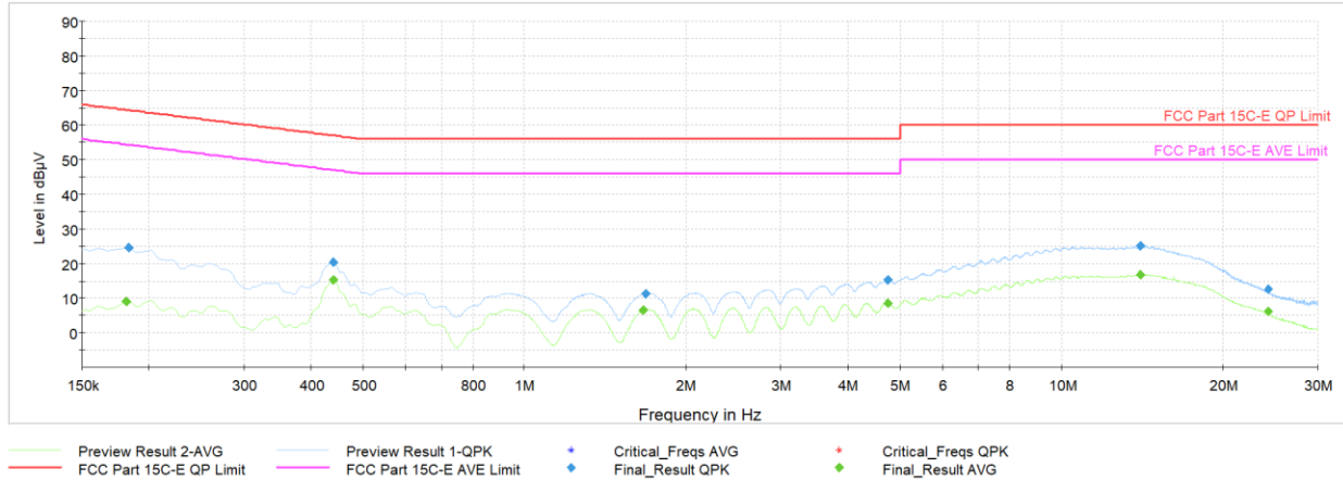
Plot 7-50. AC Line Conducted Plot with Bluetooth LE (L1, 1Mbps – Ch.17 with AC/DC Adapter)
