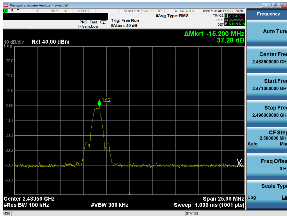
Plot 7-23. Band Edge Plot (Bluetooth (LE), 1Mbps – Ch.39)
