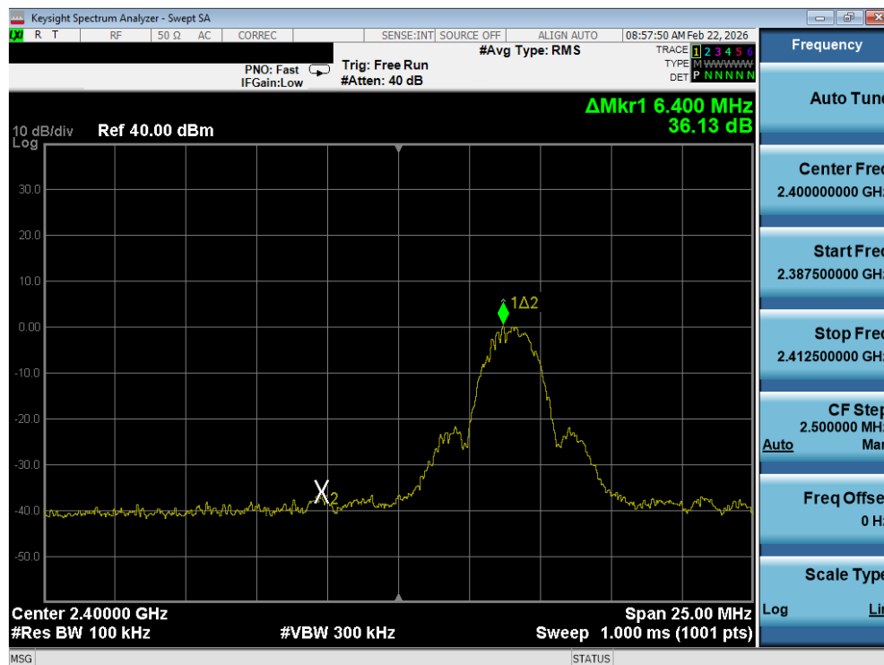
Plot 7-24. Band Edge Plot (Bluetooth (LE), 2Mbps – Ch. 0)
