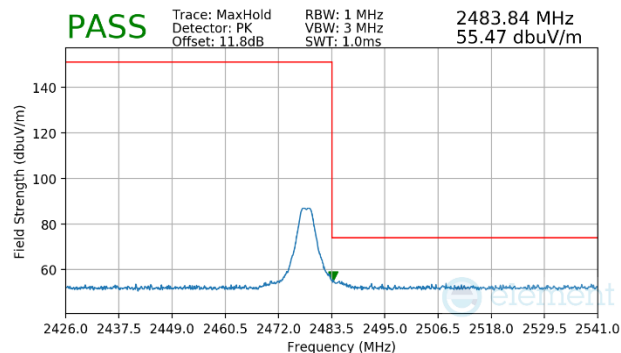
Plot 7-48. Radiated Restricted Upper Band Edge Measurement (Peak)
