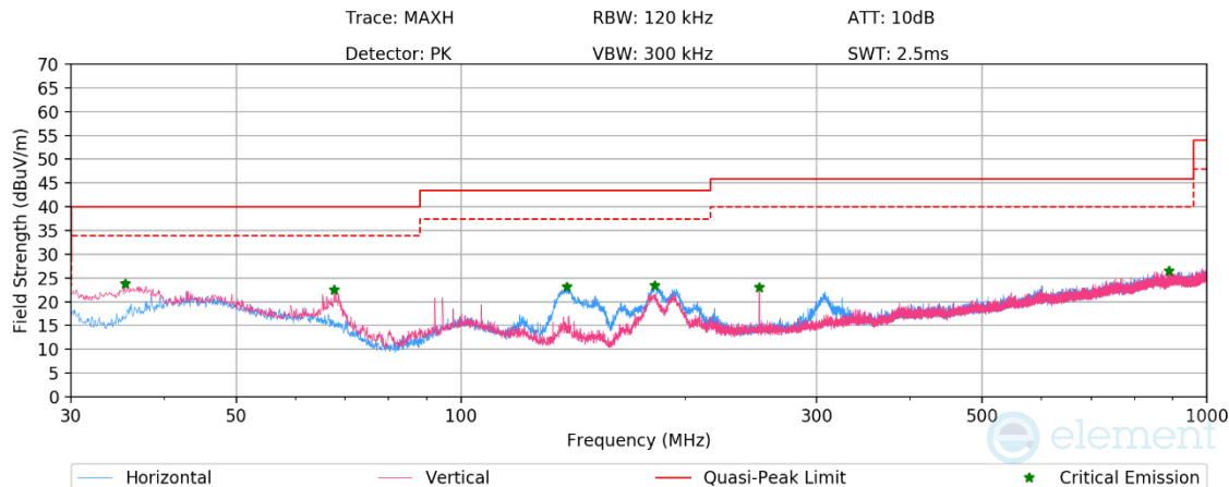
Plot 7-49. Radiated Spurious Emissions Below 1 GHz (1Mbps – Ch.17, Pol. H & V, with AC/DC Adapter)
