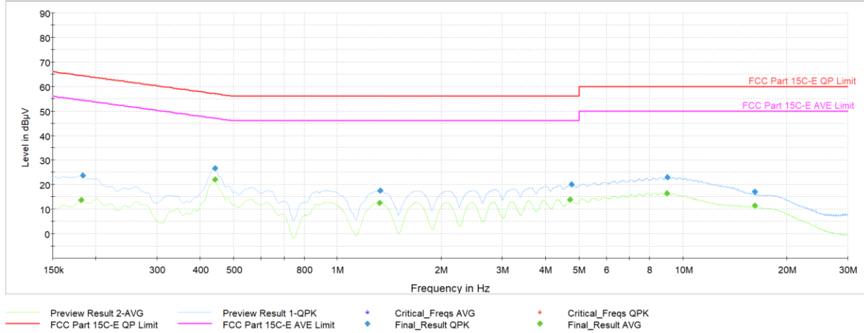
Plot 7-51. AC Line Conducted Plot with Bluetooth LE (N, 1Mbps – Ch.17, with AC/DC Adapter)
