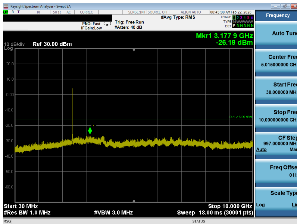
Plot 7-35. Conducted Spurious Plot (Bluetooth (LE), 2Mbps – Ch. 17)
