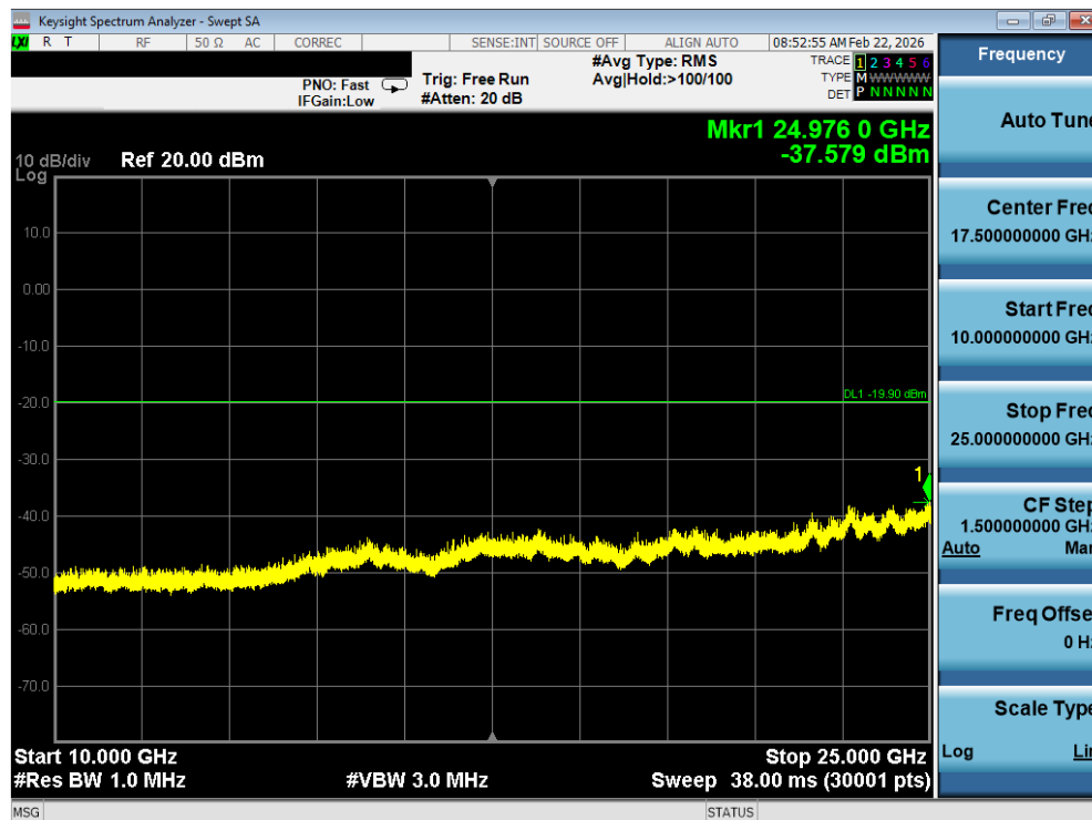
Plot 7-38. Conducted Spurious Plot (Bluetooth (LE), 2Mbps – Ch. 36)
