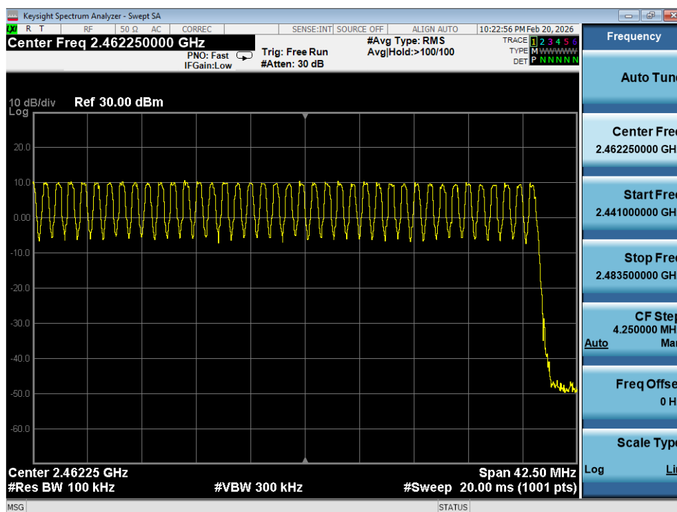
Plot 7-23. High End Spectrum Channel Hopping Plot (Bluetooth, GFSK)
