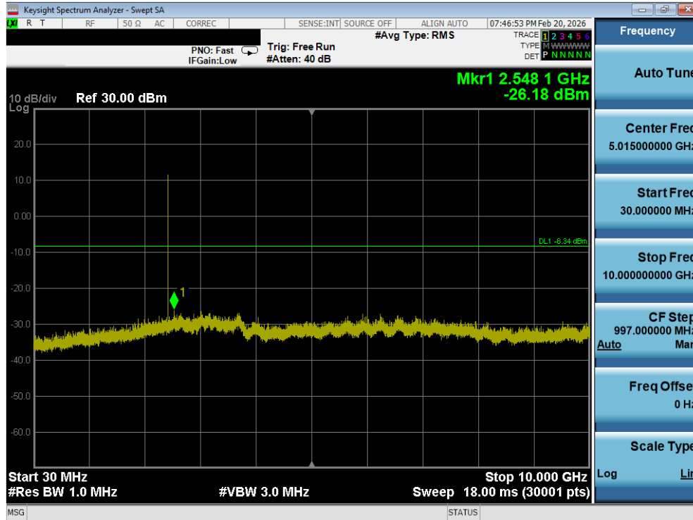
Plot 7-30. Conducted Spurious Plot (Bluetooth, GFSK – Ch. 39)
