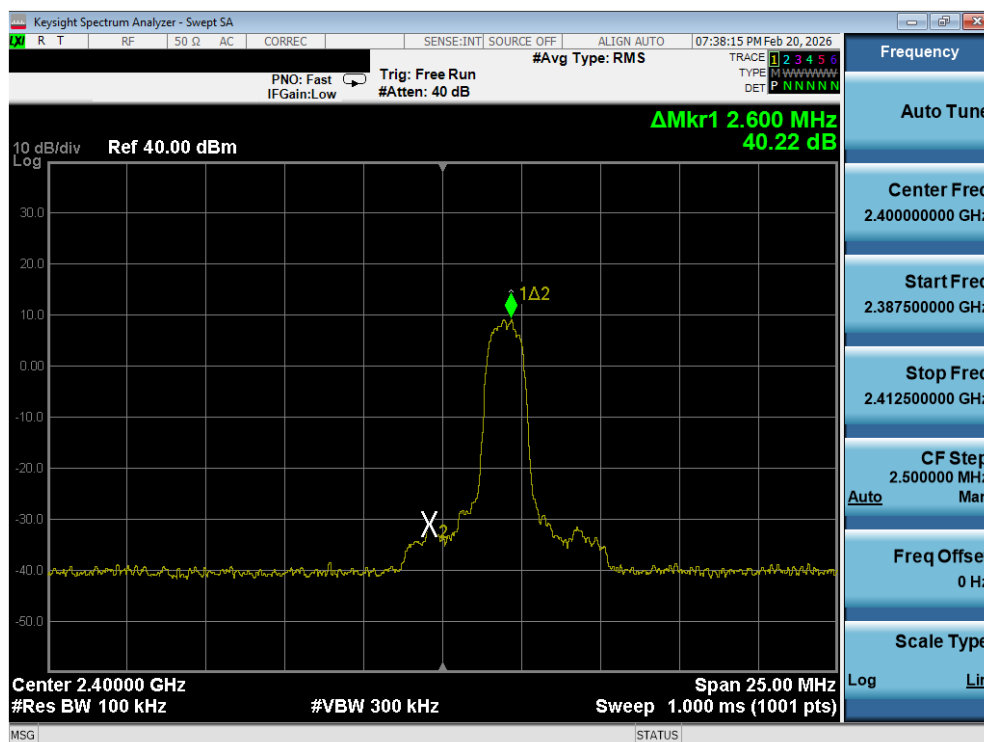
Plot 7-8. Band Edge Plot (Bluetooth with Hopping Disabled, DQPSK – Ch. 0)
