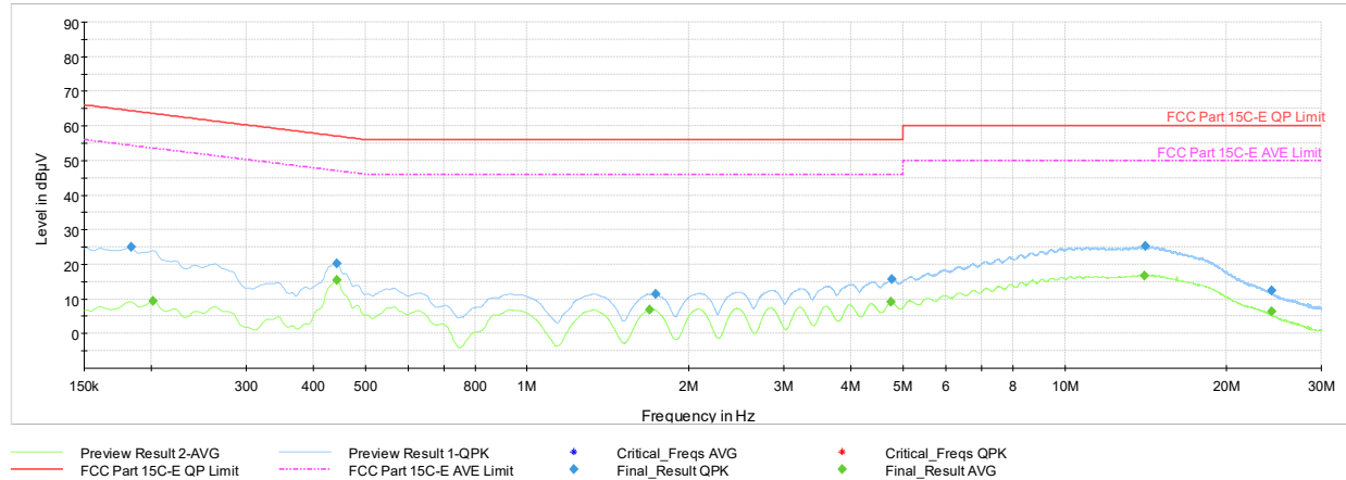
Plot 7-47. AC Line-Conducted Test Plot (L1, GFSK – Ch.39, with AC/DC Adapter)
