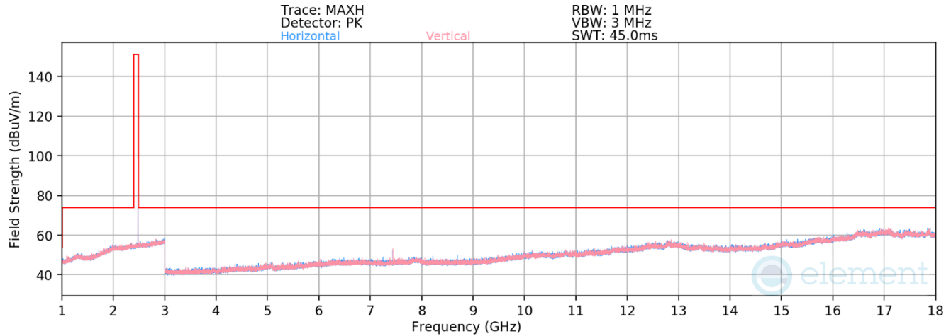
Plot 7-37. Radiated Spurious Emissions above 1GHz (BT GFSK – Ch. 78)
