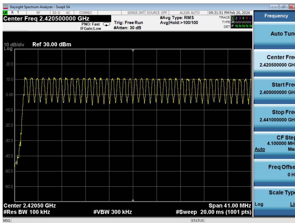
Plot 7-22. Low End Spectrum Channel Hopping Plot (Bluetooth, GFSK)
