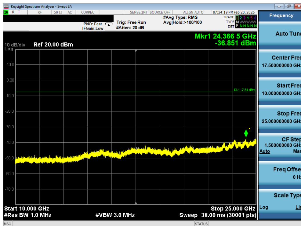
Plot 7-29. Conducted Spurious Plot (Bluetooth, GFSK – Ch. 0)
