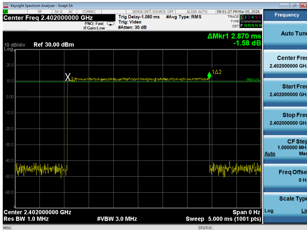
Plot 7-20. Time of Occupancy Plot (Bluetooth, \pi/4 -DQPSK)
