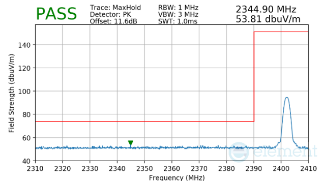
Plot 7-41. Radiated Restricted Lower Band Edge Measurement (Peak)
