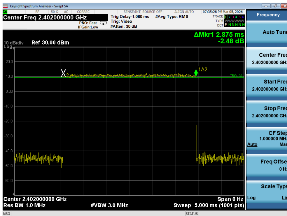
Plot 7-21. Time of Occupancy Plot (Bluetooth, 8DPSK)
