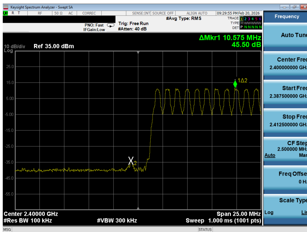
Plot 7-6. Band Edge Plot (Bluetooth with Hopping Enabled, GFSK)
