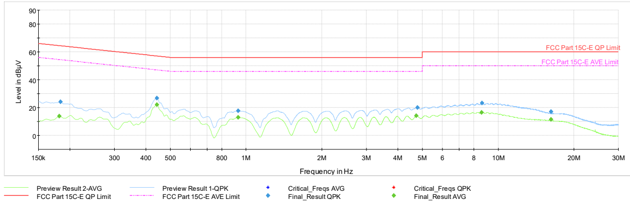
Plot 7-48. AC Line-Conducted Test Plot (N, GFSK – Ch.39, with AC/DC Adapter)
