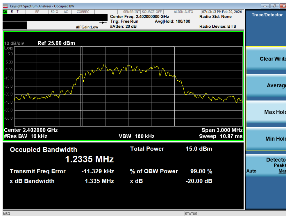
Plot 7-3. 20dB BW and 99% OBW Plot (Bluetooth, 8DPSK – Ch. 0)
