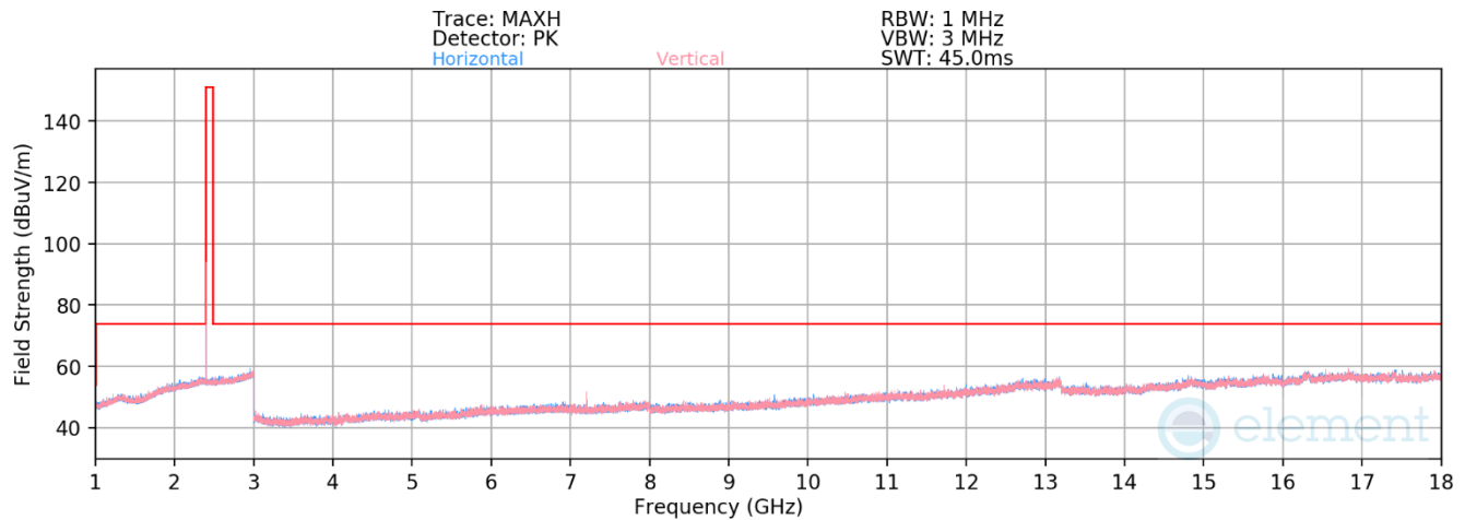
Plot 7-34. Radiated Spurious Emissions above 1GHz (BT GFSK – Ch. 0)
