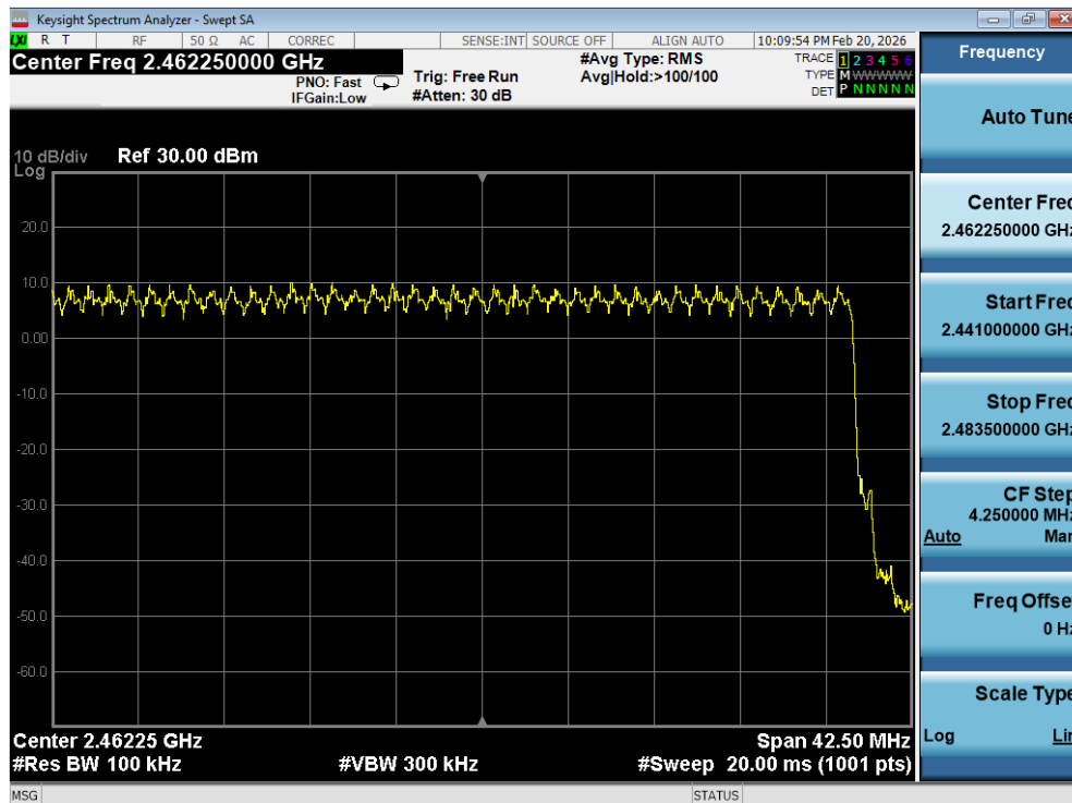
Plot 7-27. High End Spectrum Channel Hopping Plot (Bluetooth, 8DPSK)
