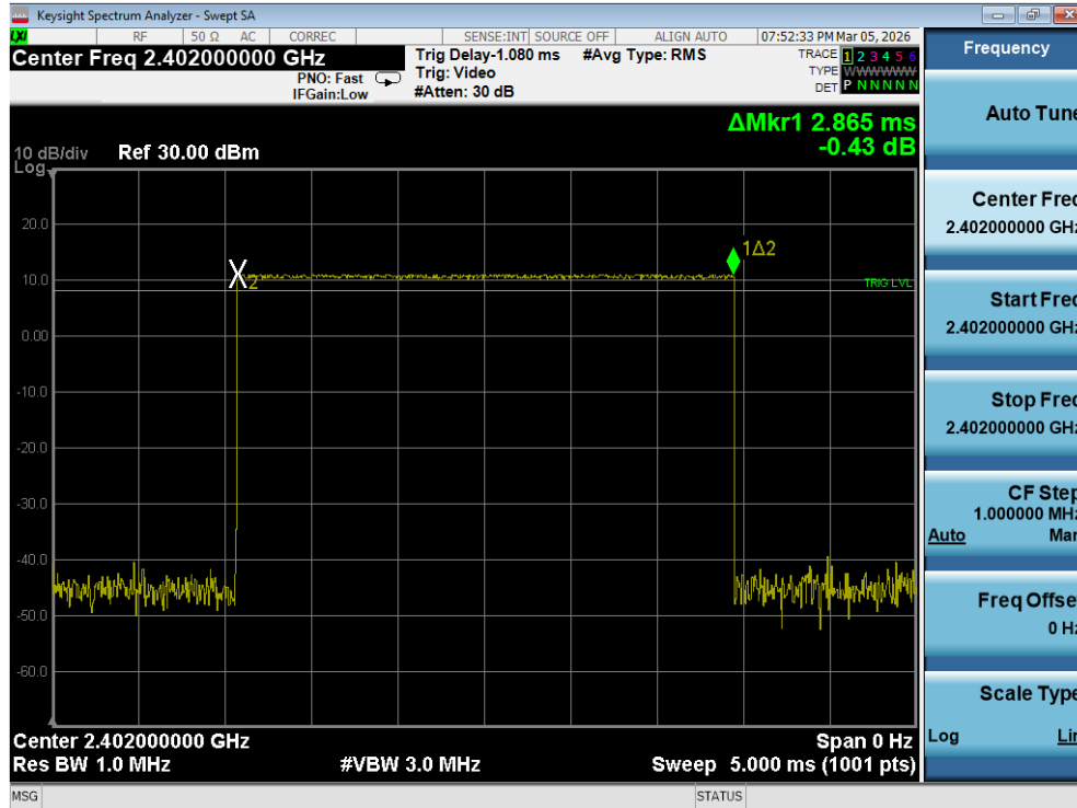
Plot 7-19. Time of Occupancy Plot (Bluetooth, GFSK)
