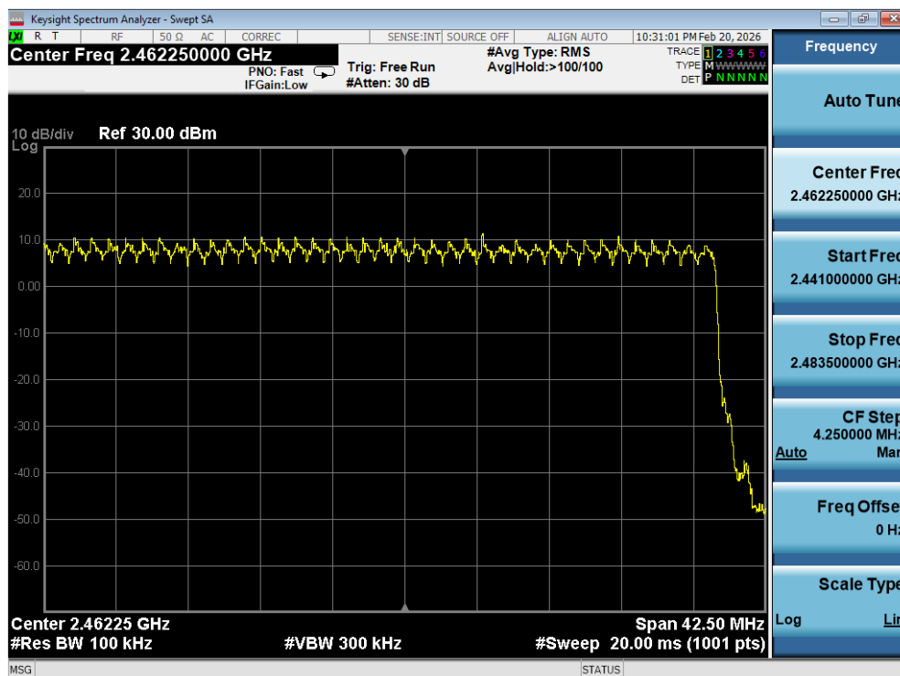
Plot 7-25. High End Spectrum Channel Hopping Plot (Bluetooth, \pi/4 -DQPSK)
