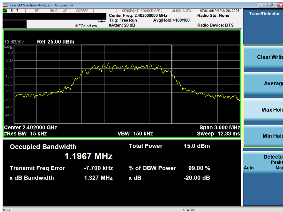
Plot 7-2. 20dB BW and 99% OBW Plot (Bluetooth, \pi/4 -DQPSK – Ch. 0)
