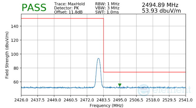
Plot 7-45. Radiated Restricted Upper Band Edge Measurement (Peak)
