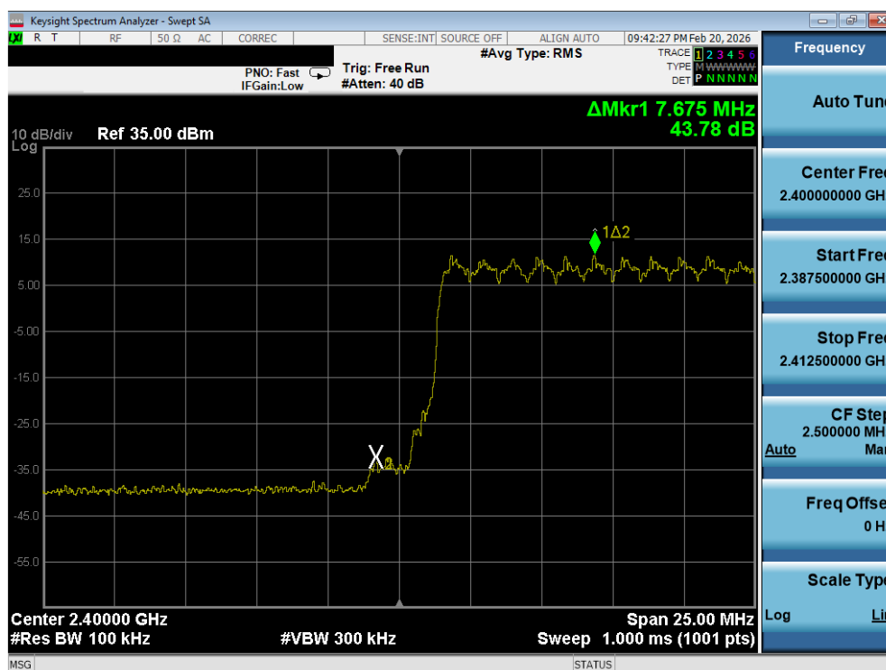
Plot 7-10. Band Edge Plot (Bluetooth with Hopping Enabled, DQPSK)
