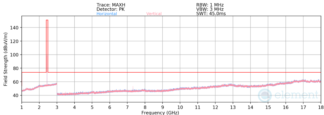
Plot 7-35. Radiated Spurious Emissions above 1GHz (BT GFSK – Ch. 39)
