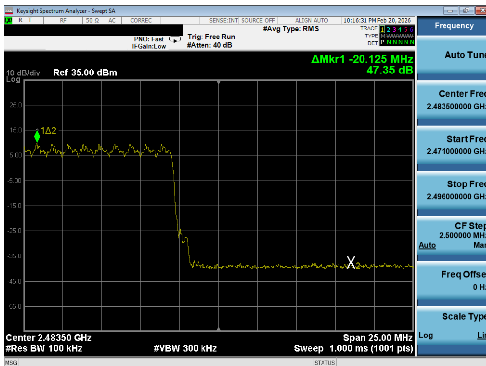
Plot 7-15. Band Edge Plot (Bluetooth with Hopping Enabled, 8DPSK)
