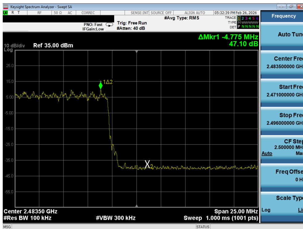
Plot 7-11. Band Edge Plot (Bluetooth with Hopping Enabled, DQPSK)
