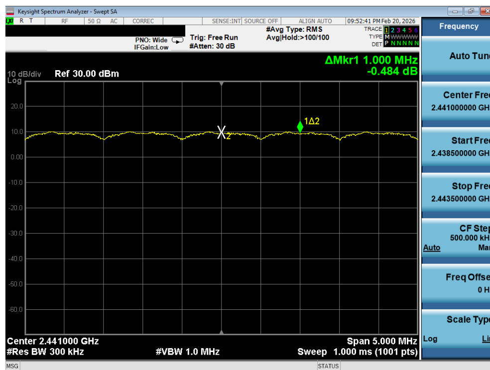
Plot 7-18. Channel Spacing Plot (Bluetooth, 8DPSK)
