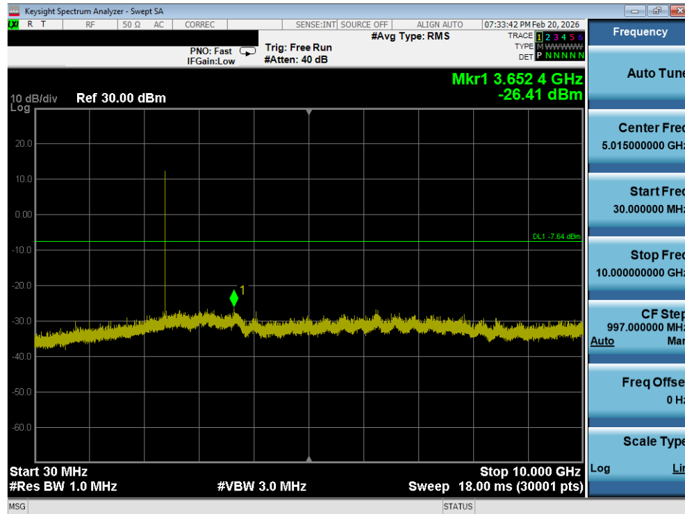
Plot 7-28. Conducted Spurious Plot (Bluetooth, GFSK- Ch. 0)
