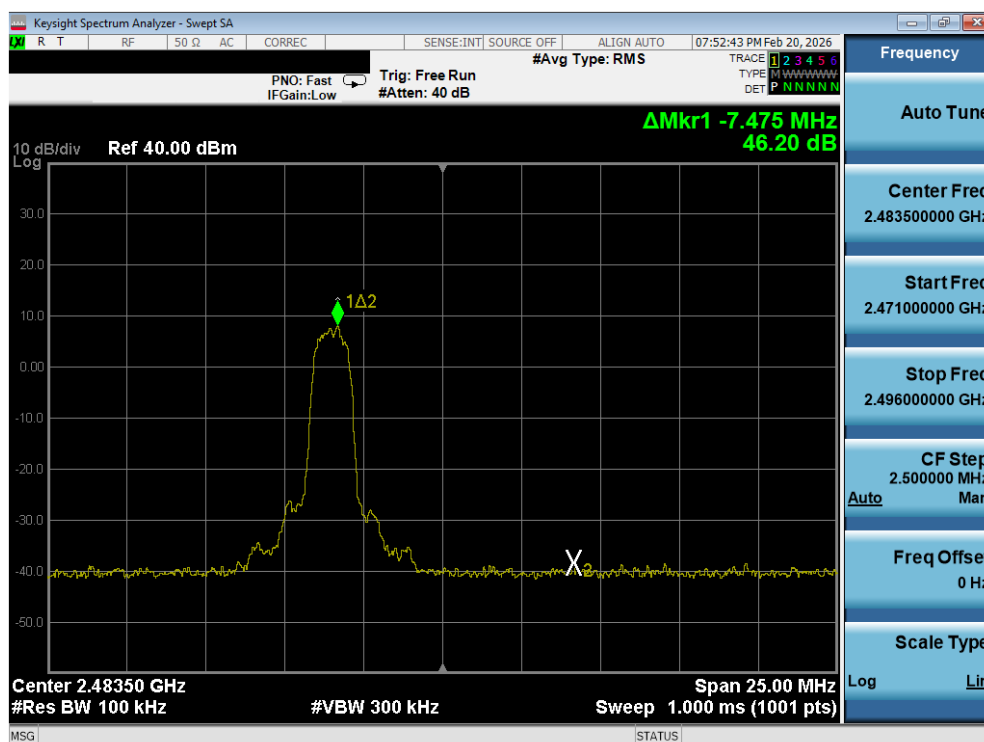
Plot 7-9. Band Edge Plot (Bluetooth with Hopping Disabled, DQPSK – Ch. 78)
