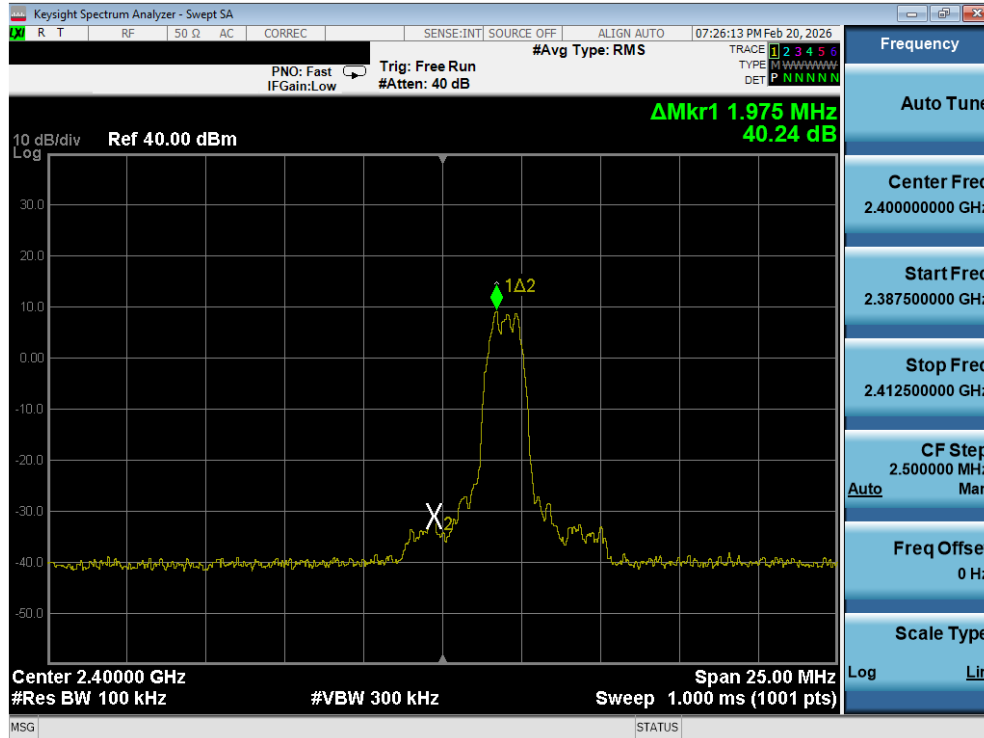
Plot 7-12. Band Edge Plot (Bluetooth with Hopping Disabled, 8DPSK – Ch. 0)
