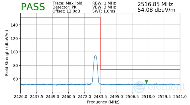
Plot 7-43. Radiated Restricted Upper Band Edge Measurement (Peak)
