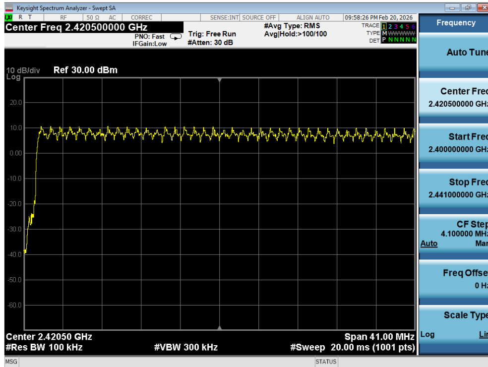
Plot 7-26. Low End Spectrum Channel Hopping Plot (Bluetooth, 8DPSK)
