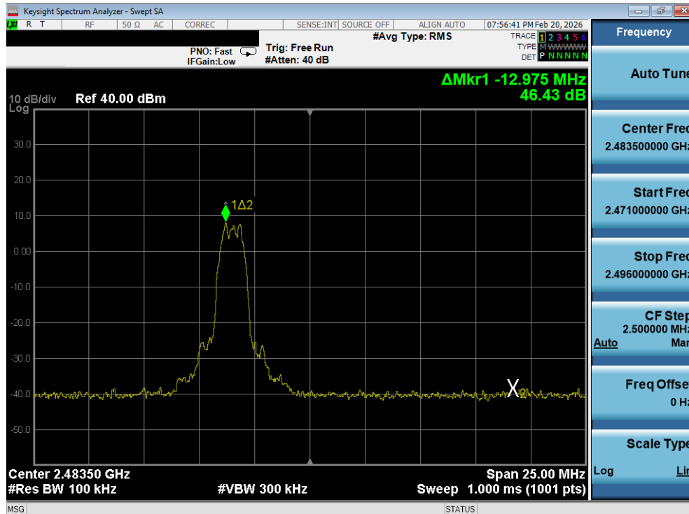
Plot 7-13. Band Edge Plot (Bluetooth with Hopping Disabled, 8DPSK – Ch. 78)
