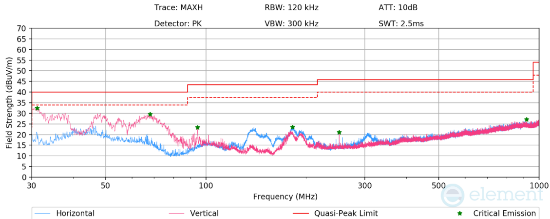
Plot 7-46. Radiated Spurious Emissions Below 1GHz (GFSK – Ch.39, with AC/DC Adapter)
