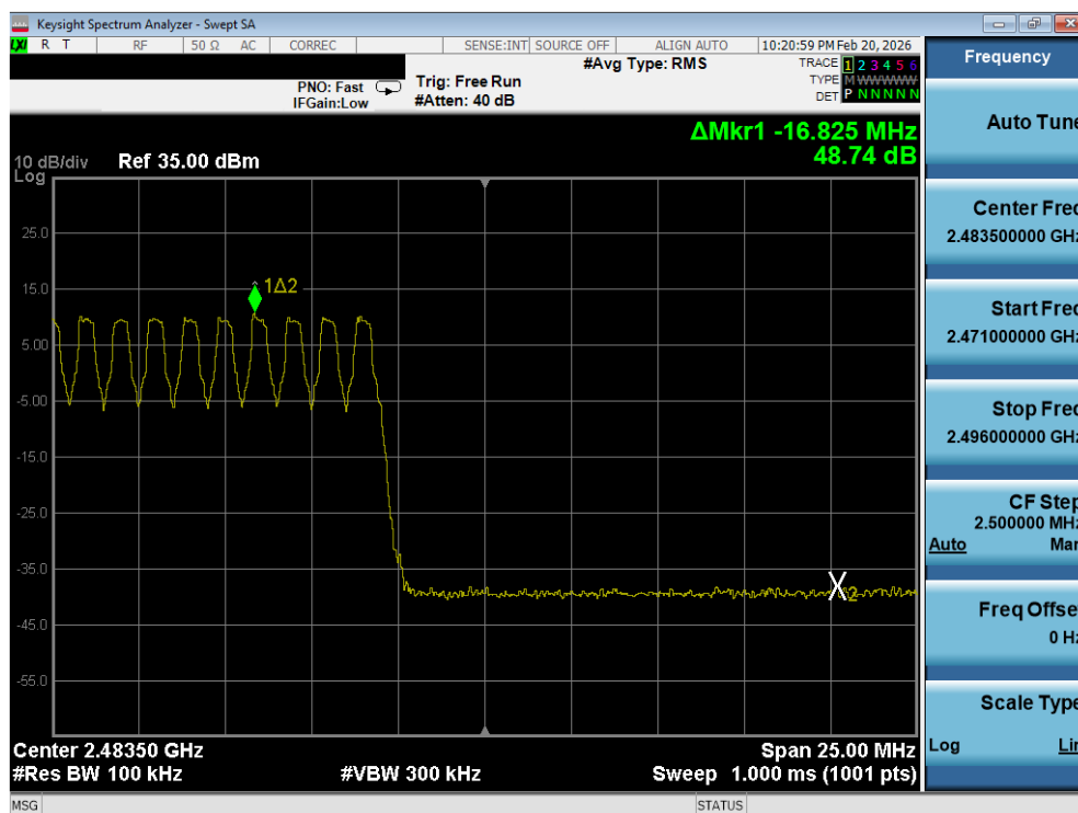
Plot 7-7. Band Edge Plot (Bluetooth with Hopping Enabled, GFSK)
