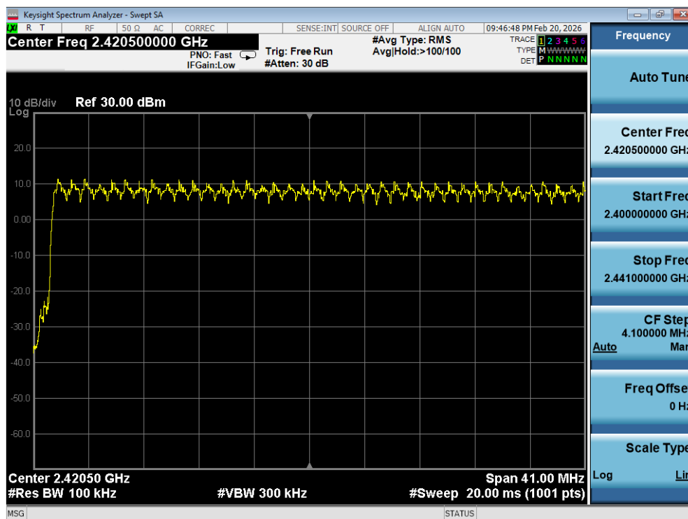
Plot 7-24. Low End Spectrum Channel Hopping Plot (Bluetooth, \pi/4 -DQPSK)
