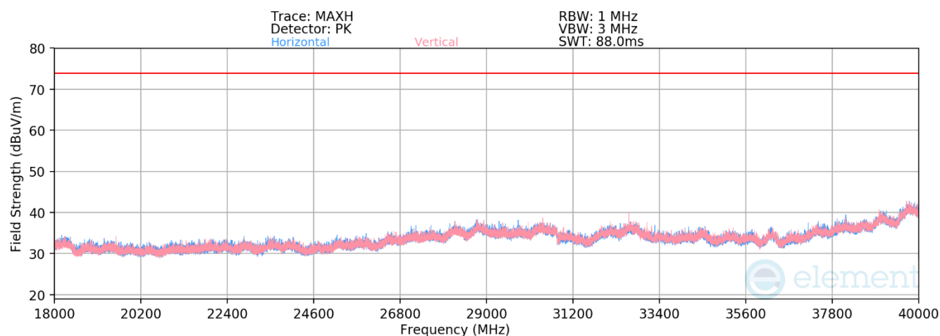
Plot 7-36. Radiated Spurious Emissions above 18GHz (BT GFSK – Ch. 39)
