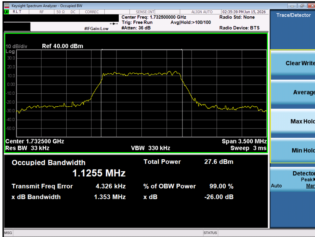
Plot 7-19. Occupied Bandwidth Plot (LTE Band 4 - 1.4MHz QPSK - Full RB - ANT1)
