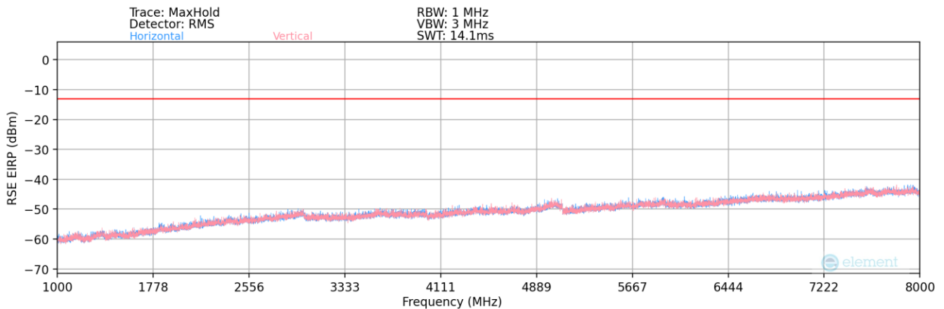
Plot 7-22. Radiated Spurious Plot (LTE CAT-M1 Band 12)
