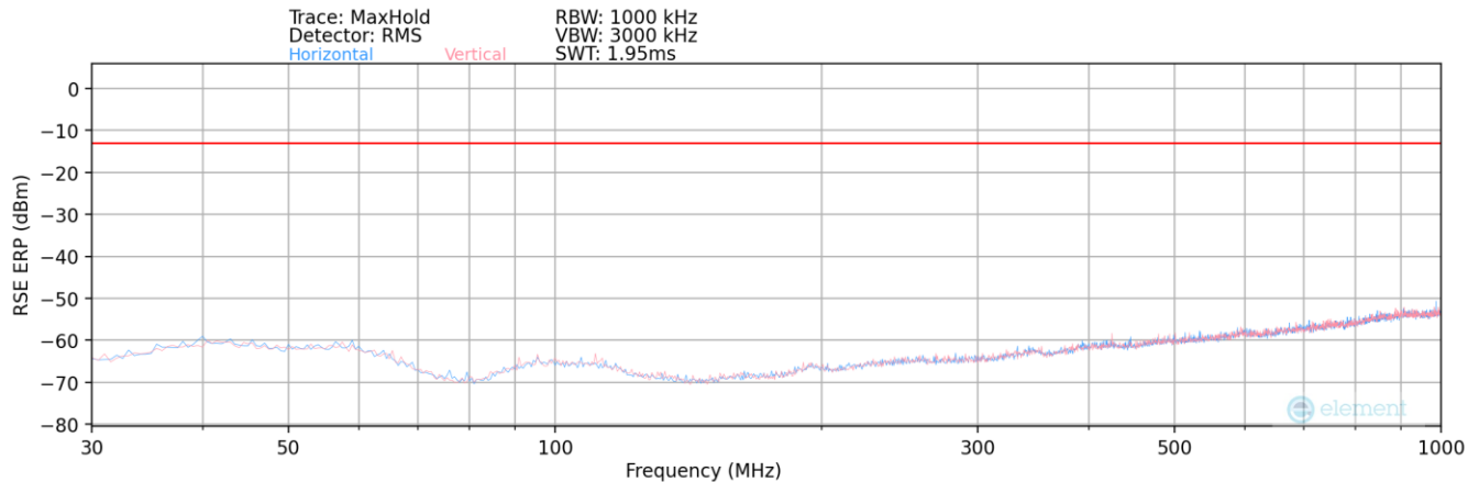
Plot 7-23. Radiated Spurious Plot (LTE CAT-M1 Band 4)
