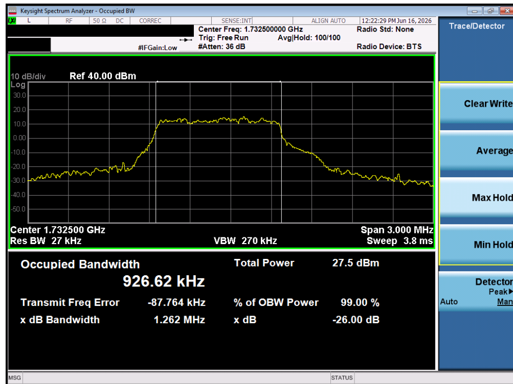
Plot 7-20. Occupied Bandwidth Plot (LTE Band 4 - 1.4MHz 16-QAM - Full RB - ANT1)
