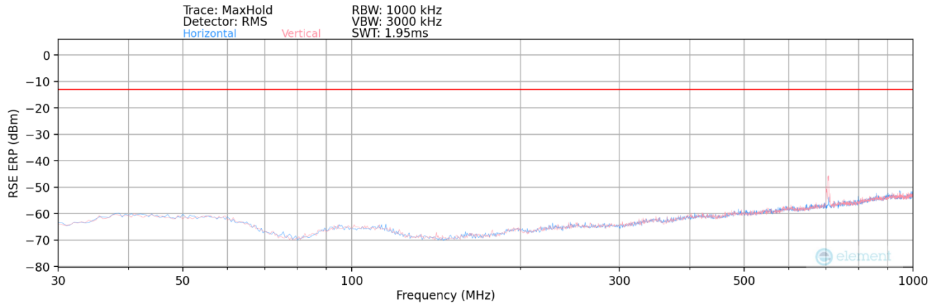
Plot 7-25. Radiated Spurious Plot below 1GHz LTE CAT-M1 Band 4 + Bluetooth
