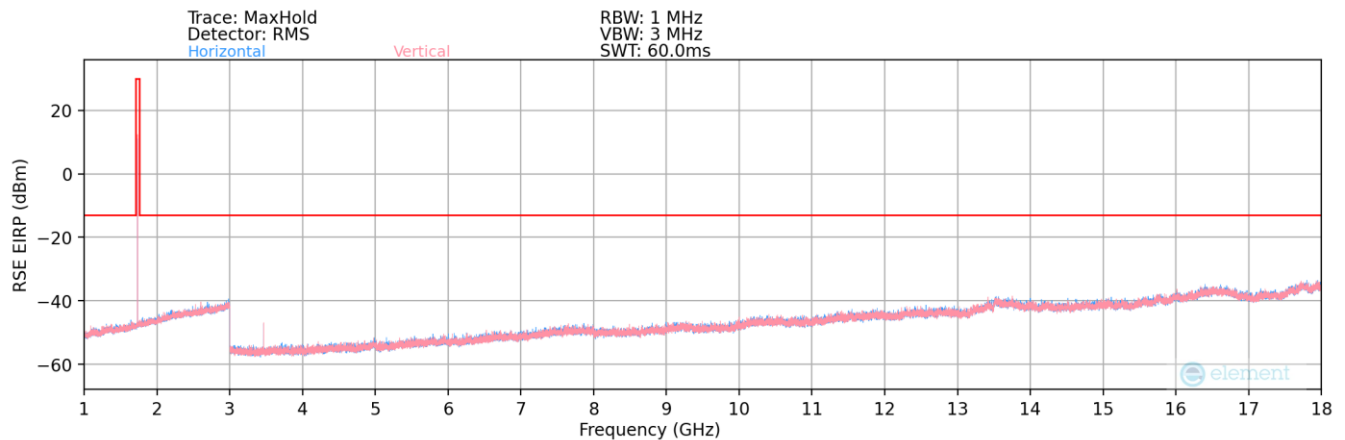
Plot 7-24. Radiated Spurious Plot (LTE CAT-M1 Band 4)
