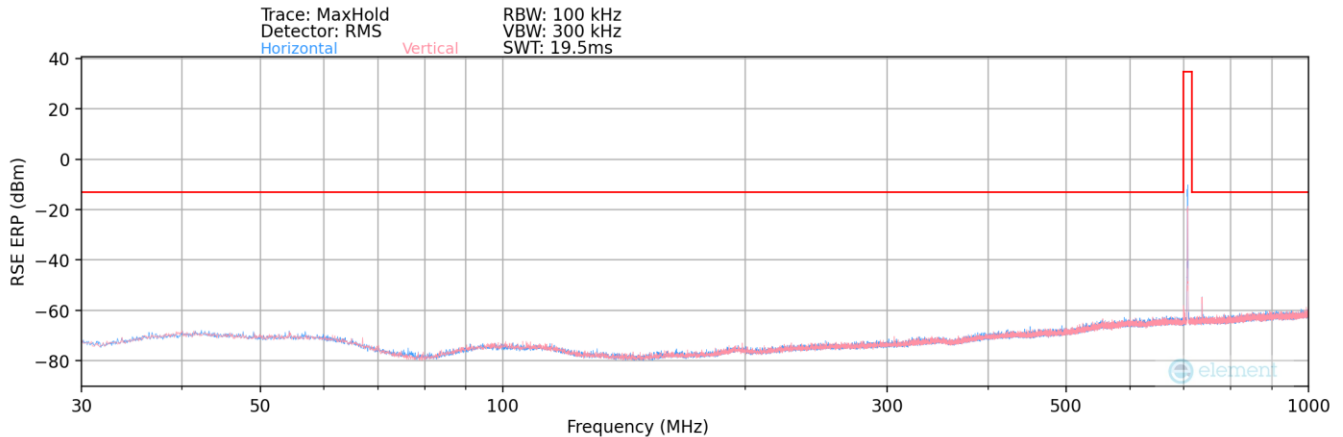
Plot 7-21. Radiated Spurious Plot (LTE CAT-M1 Band 12)
