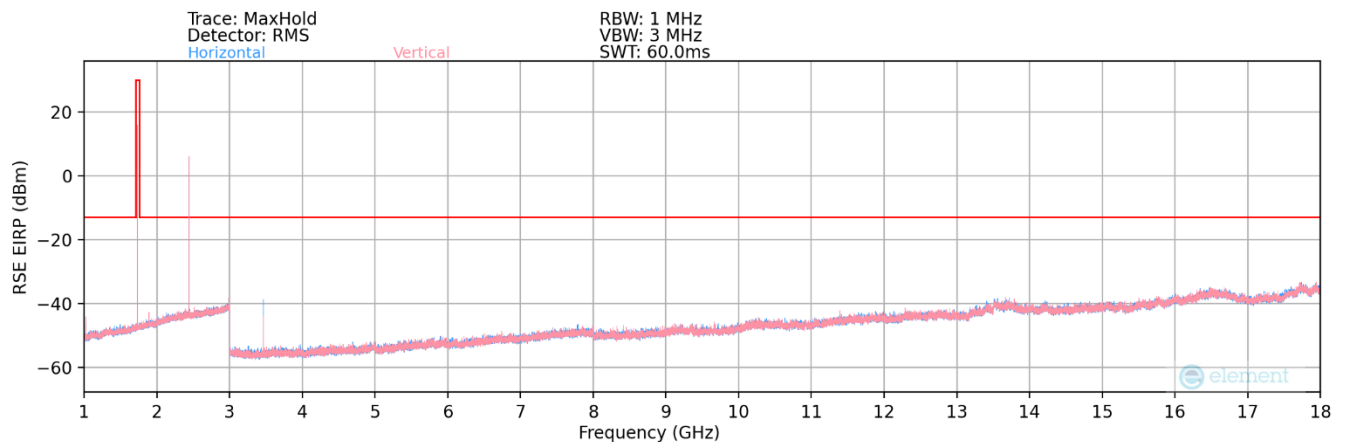
Plot 7-26. Radiated Spurious Plot below 1-18GHz LTE CAT-M1 Band 4 + Bluetooth
