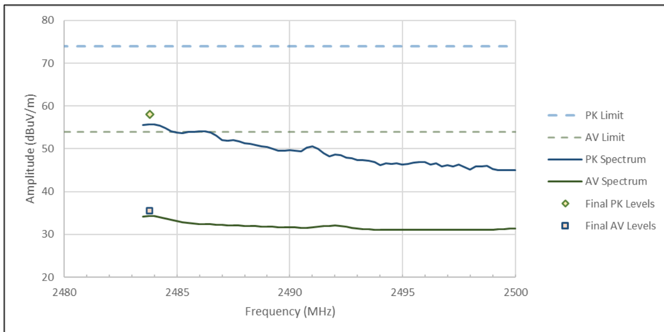
Figure RE03.4: BLE 2 Mbps FCC restricted band spectral data from 2483.5 to 2500 MHz
