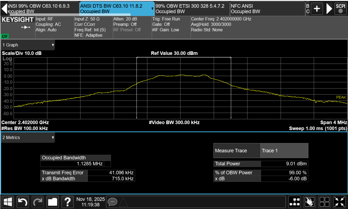
Figure TR11.3: Bandwidth data for BLE 1 Mbps at low channel (2402 MHz)
