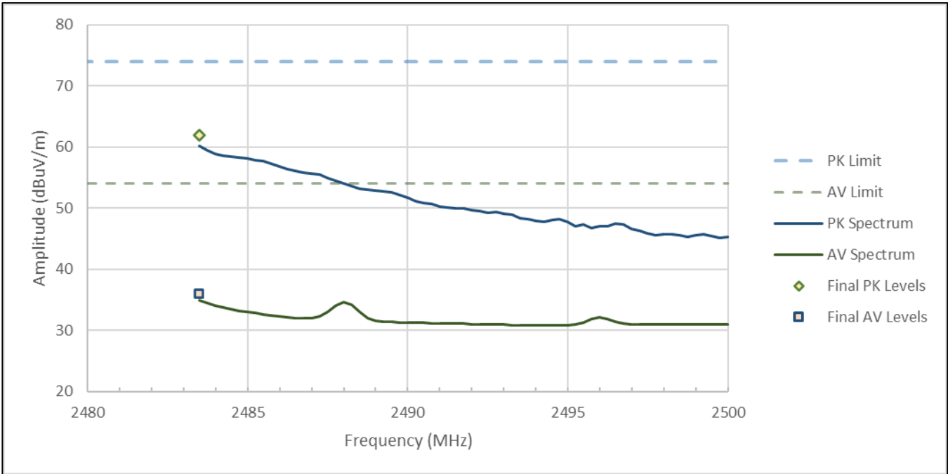
Figure RE03.2: BLE 1 Mbps FCC restricted band spectral data from 2483.5 to 2500 MHz
