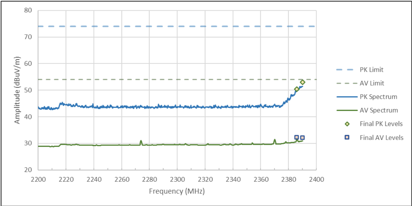
Figure RE03.1: BLE 1 Mbps FCC restricted band spectral data from 2200 to 2390 MHz
