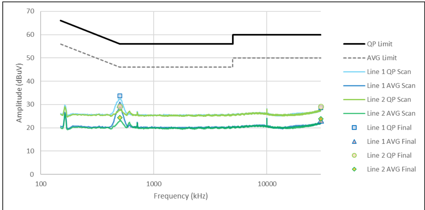
Figure CE01.1: Spectral data (BLE, 1 Mbps, 2440 MHz)
