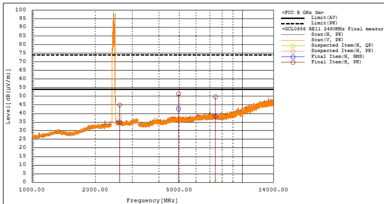
Figure RE11.3: Spectral data (BLE1, 2480 MHz)
