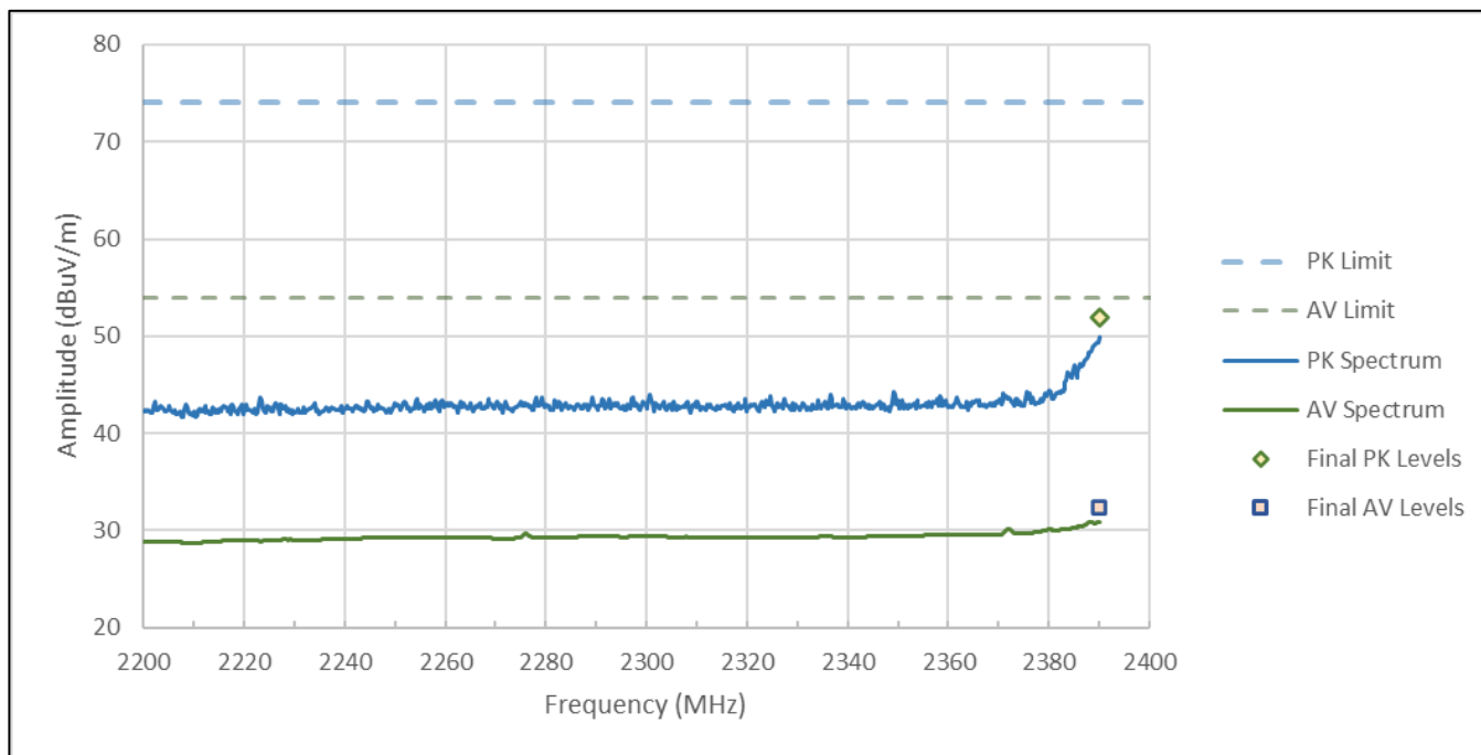
Figure RE03.3: BLE 2 Mbps FCC restricted band spectral data from 2200 to 2390 MHz
