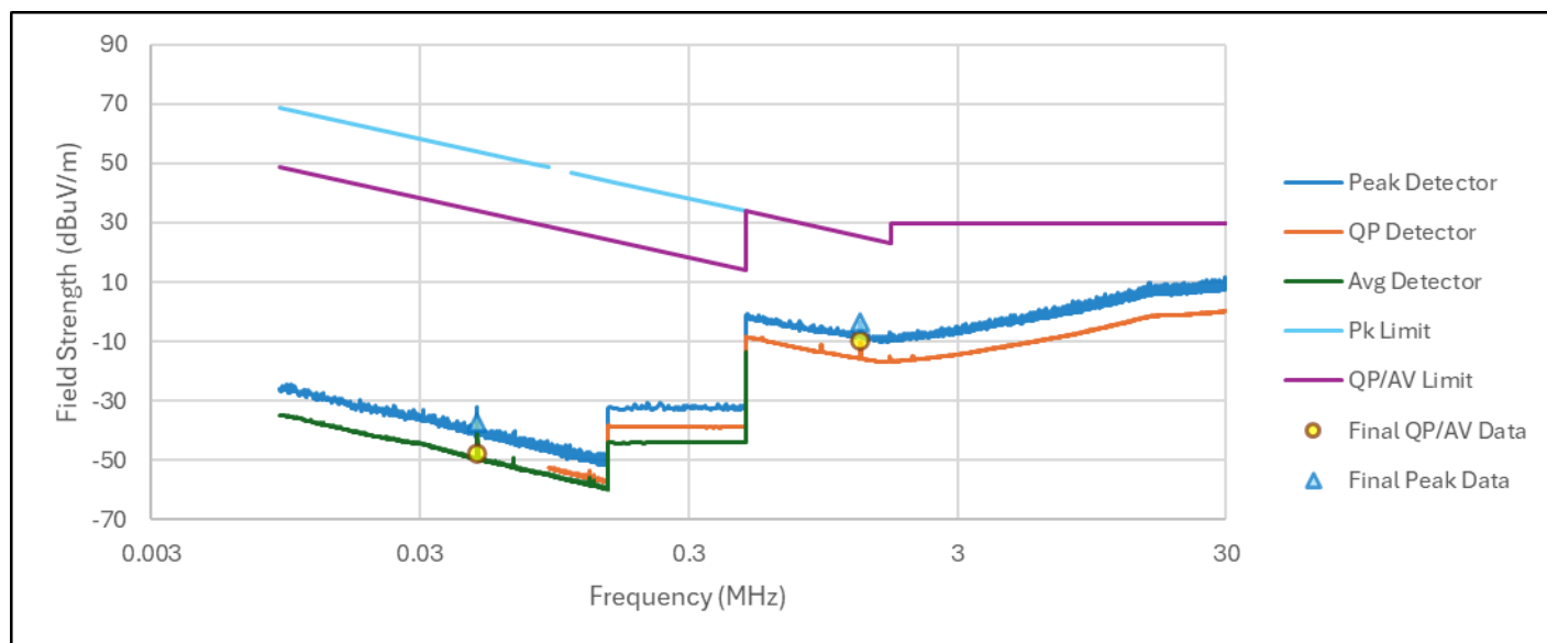
Figure RE22.1: Spectral data (BLE 1 Mbps, 2480 MHz)
