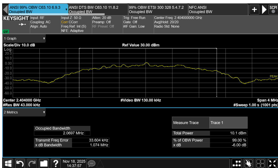
Figure TR15.2: Occupied bandwidth data for BLE 2 Mbps at low channel (2404 MHz)
