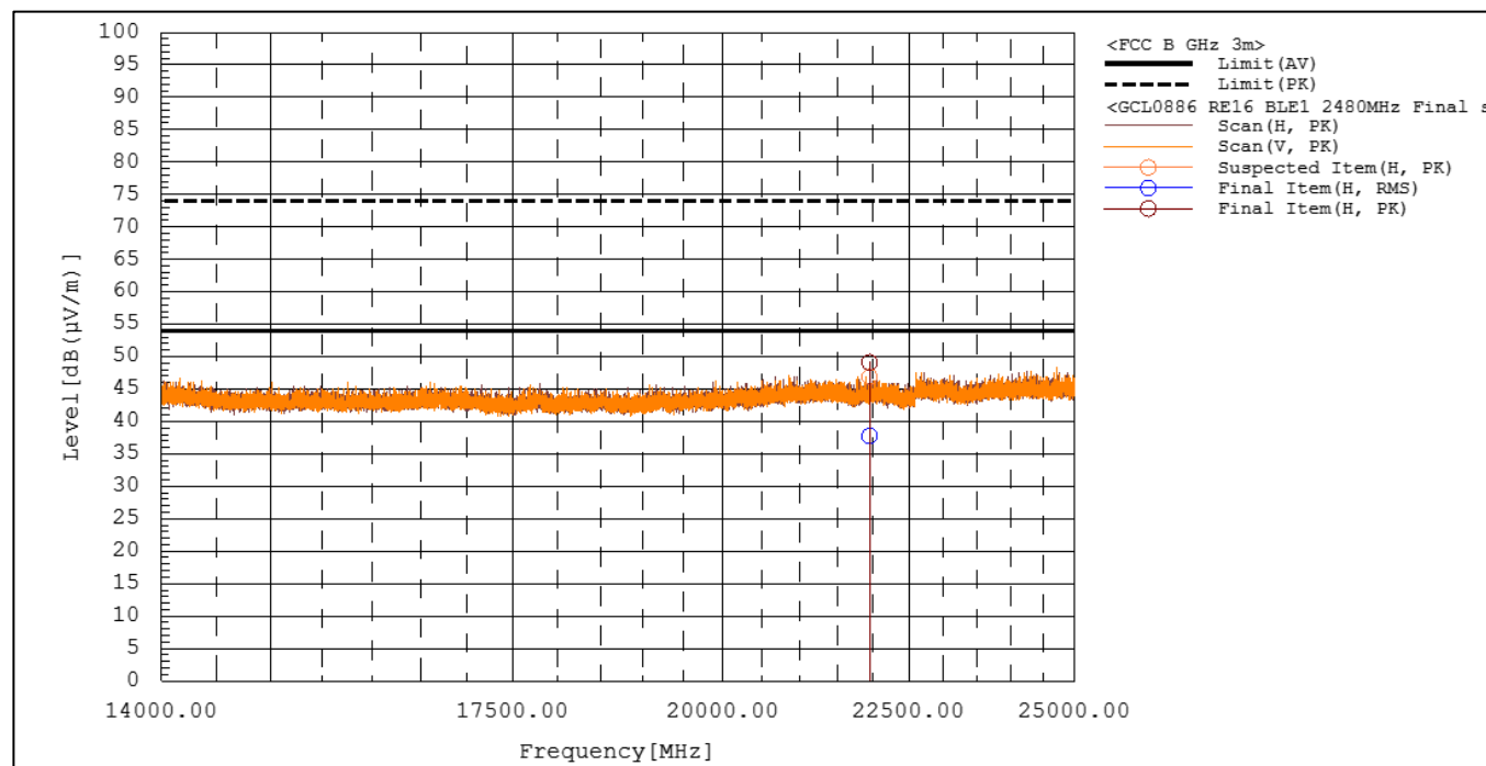
Figure RE16.1: Spectral data (BLE 1 Mbps, 2480 MHz)
