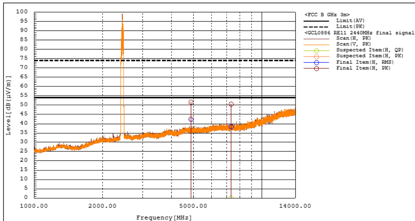
Figure RE11.2: Spectral data (BLE1, 2440 MHz)
