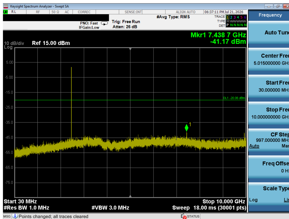
Plot 7-31. Conducted Spurious Plot (ANT/ANT+ – Ch. 79)
