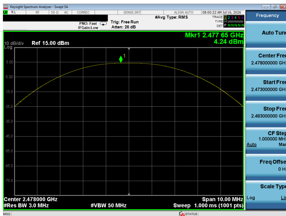
Plot 7-11. Peak Power Plot (ANT/ANT+ – Ch. 77)
