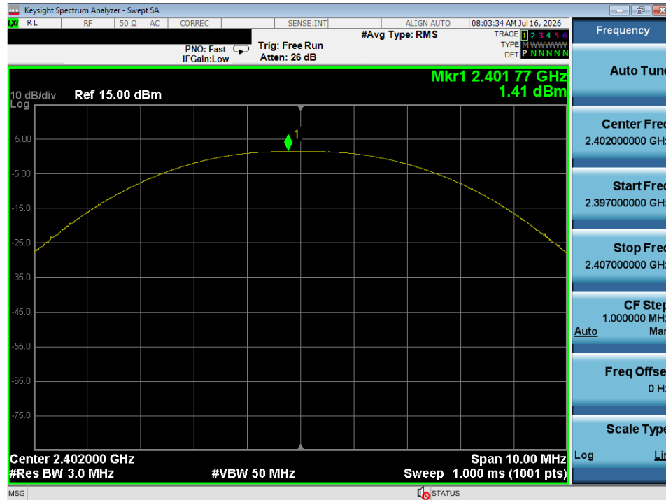
Plot 7-7. Peak Power Plot (ANT/ANT+ – Ch. 1)
