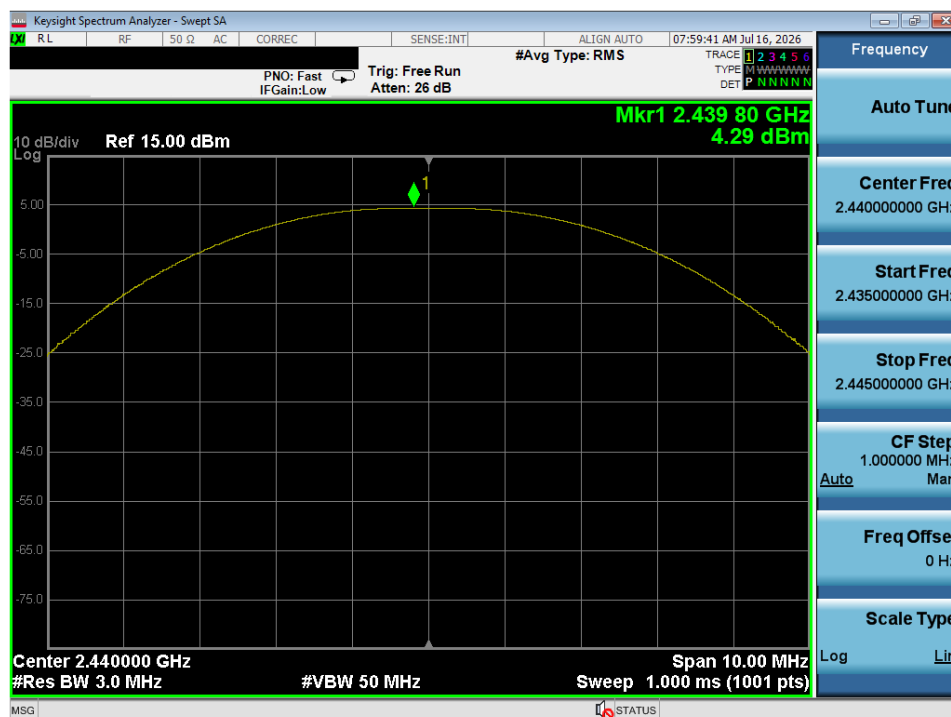
Plot 7-10. Peak Power Plot (ANT/ANT+ – Ch. 39)
