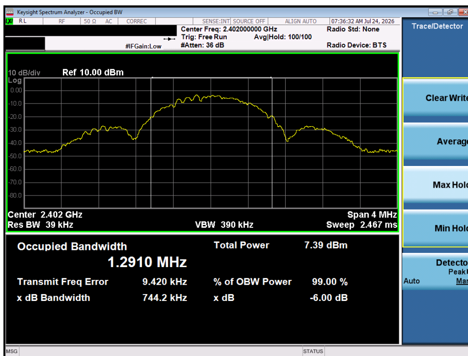
Plot 7-4. Occupied Bandwidth Plot (ANT/ANT+ – Ch. 1)
