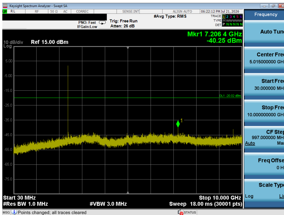
Plot 7-27. Conducted Spurious Plot (ANT/ANT+ – Ch. 1)
