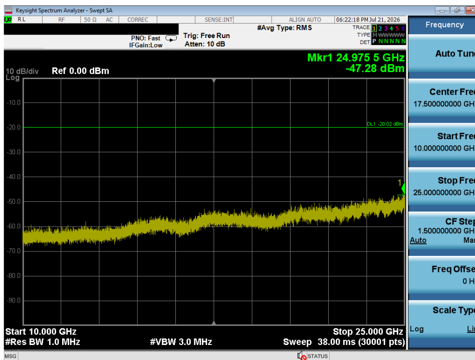
Plot 7-28. Conducted Spurious Plot (ANT/ANT+ – Ch. 1)
