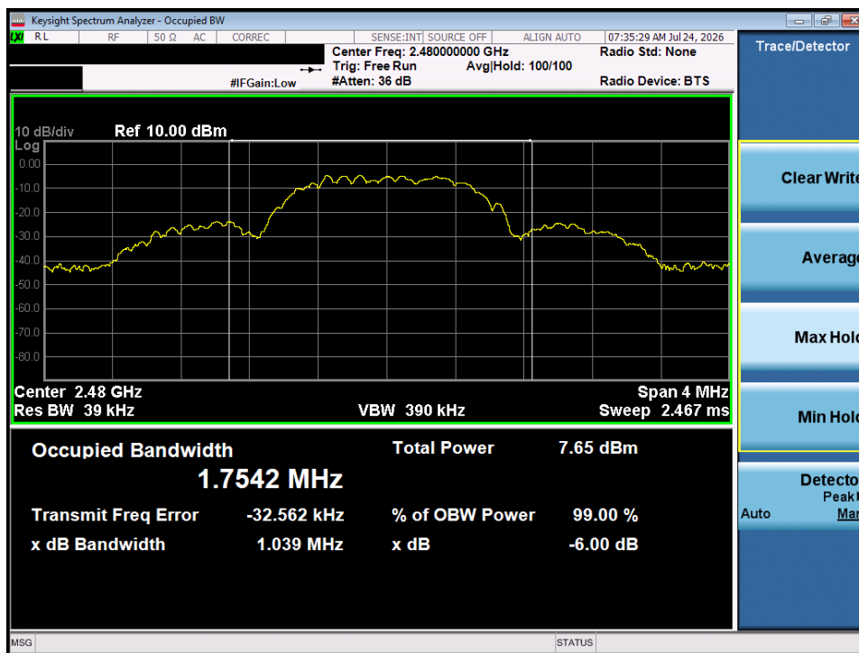
Plot 7-6. Occupied Bandwidth Plot (ANT/ANT+ – Ch. 79)
