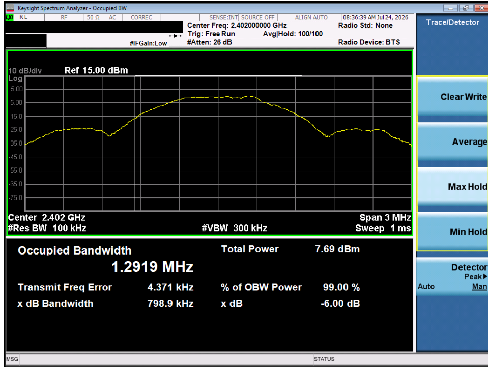
Plot 7-1. 6dB Bandwidth Plot (ANT/ANT+ – Ch. 1)
