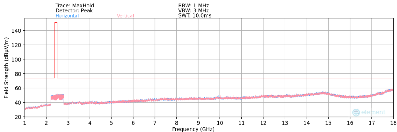
Plot 7-35. Radiated Spurious Plot above 1GHz (ANT/ANT+ – Ch. 79)
