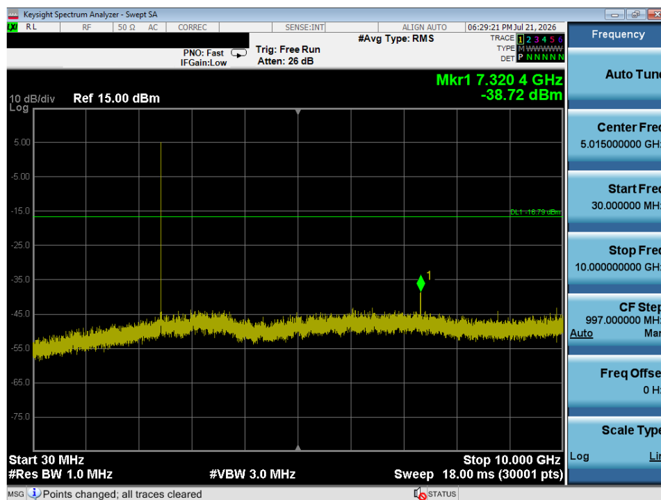
Plot 7-29. Conducted Spurious Plot (ANT/ANT+ – Ch. 39)
