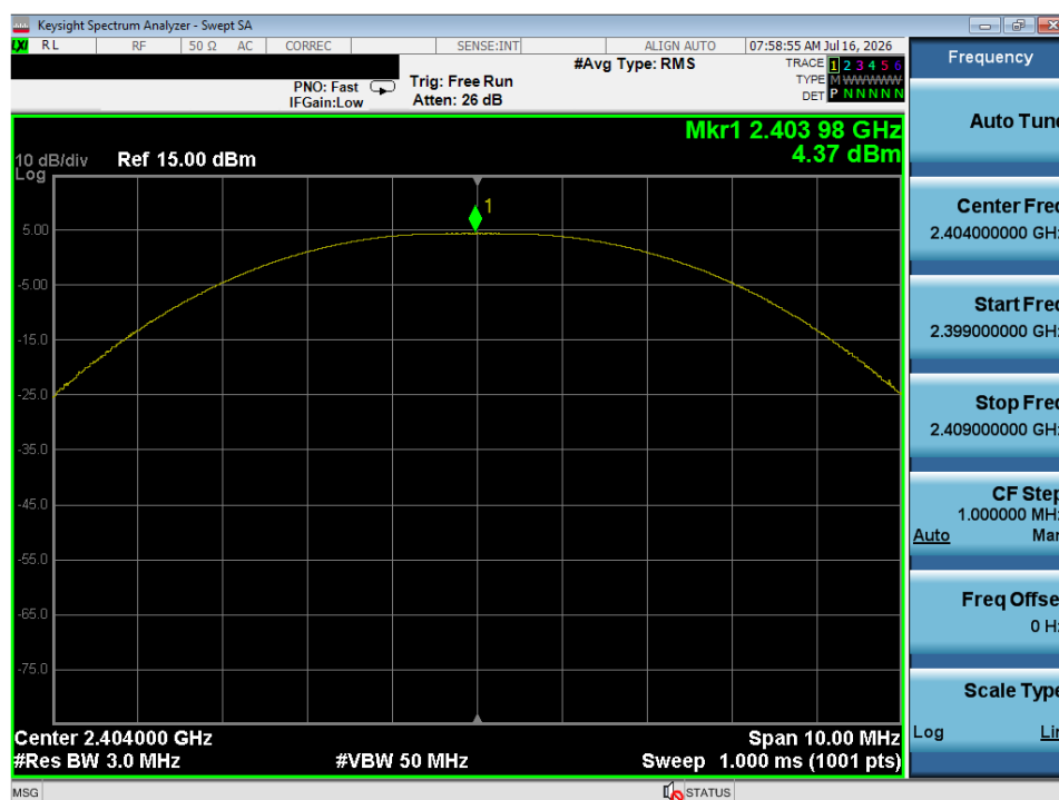
Plot 7-9. Peak Power Plot (ANT/ANT+ – Ch. 3)
