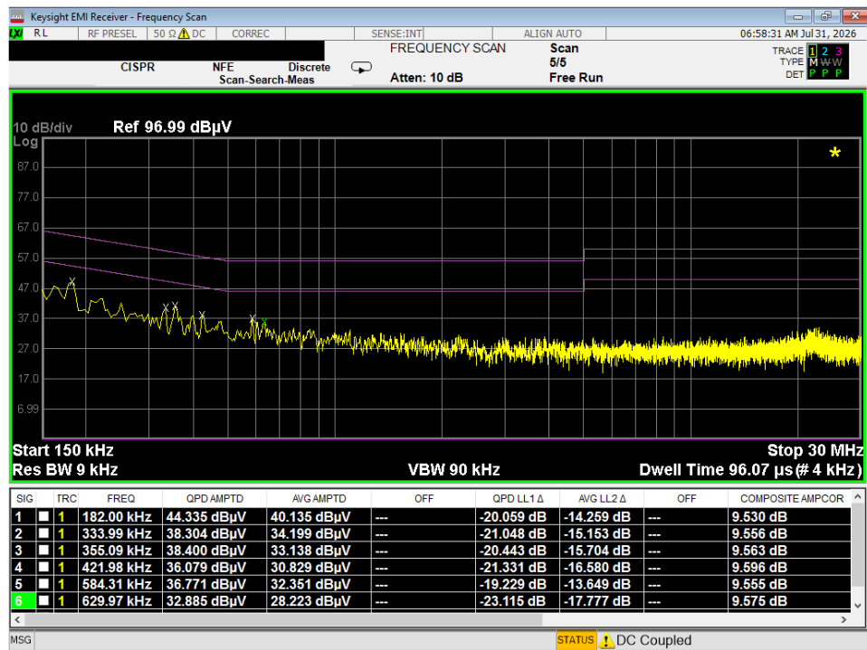
Plot 7-42. Line Conducted Plot with ANT/ANT+ (L1)
