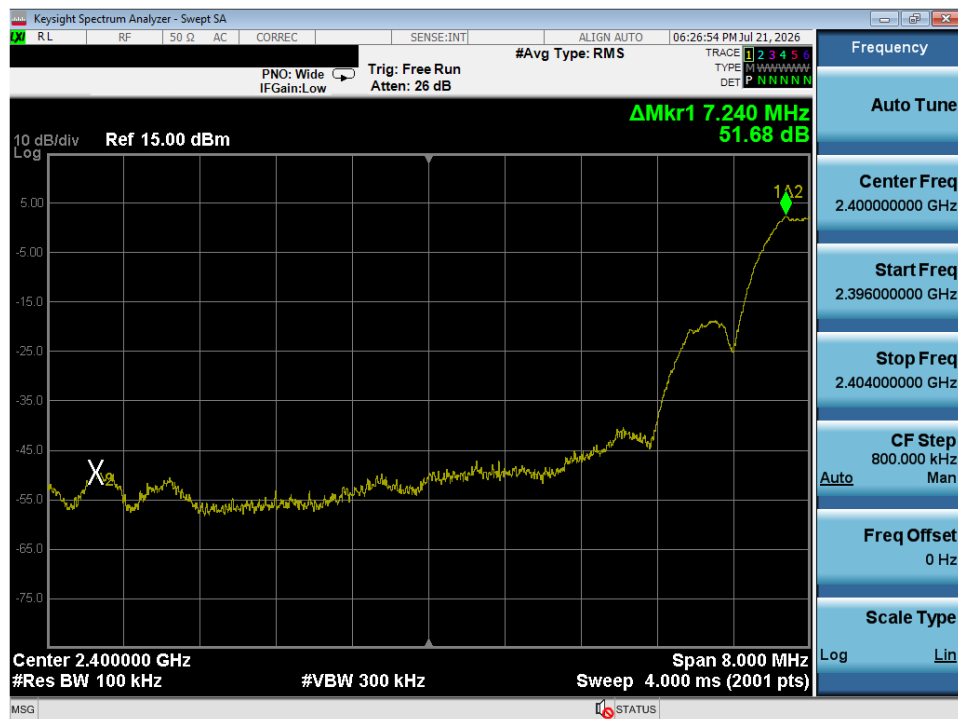
Plot 7-23. Band Edge Plot (ANT/ANT+ – Ch. 3)
