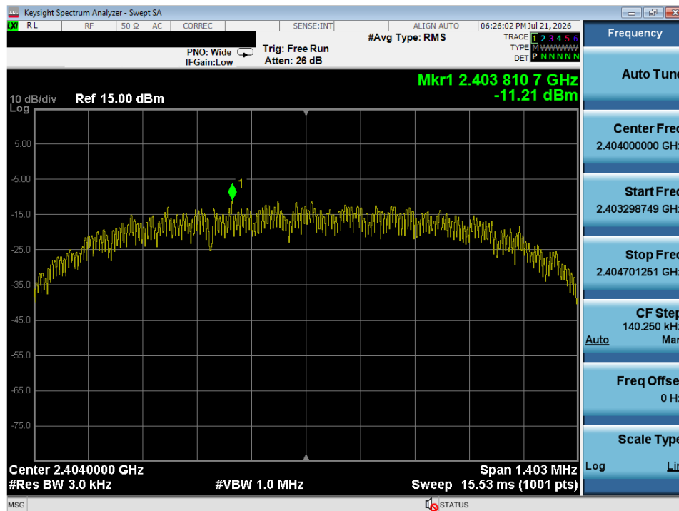
Plot 7-16. Power Spectral Density Plot (ANT/ANT+ – Ch. 3)
