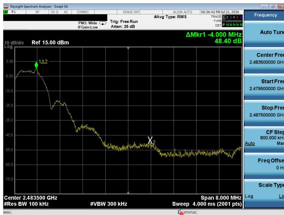
Plot 7-26. Band Edge Plot (ANT/ANT+ – Ch. 79)
