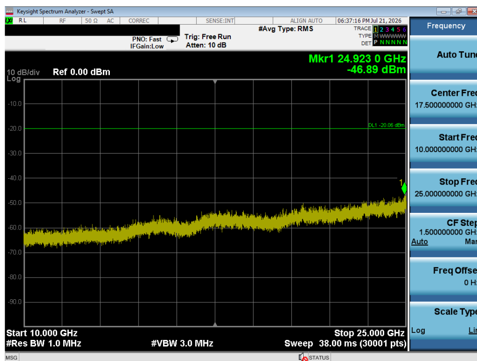
Plot 7-32. Conducted Spurious Plot (ANT/ANT+ – Ch. 79)
