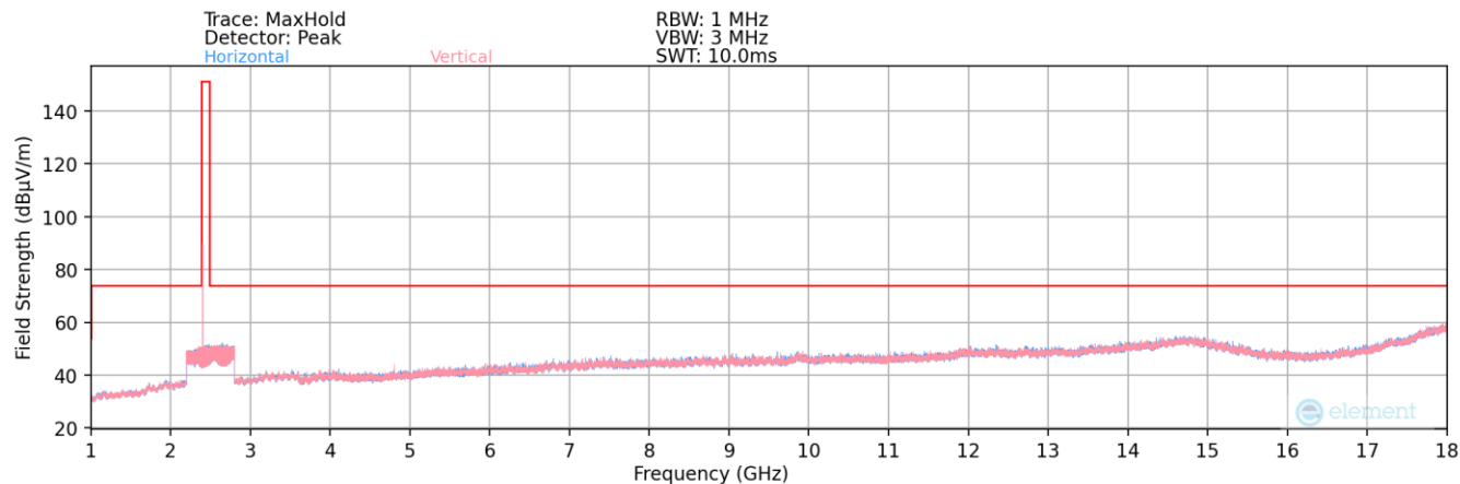
Plot 7-33. Radiated Spurious Plot above 1GHz (ANT/ANT+ – Ch. 1)
