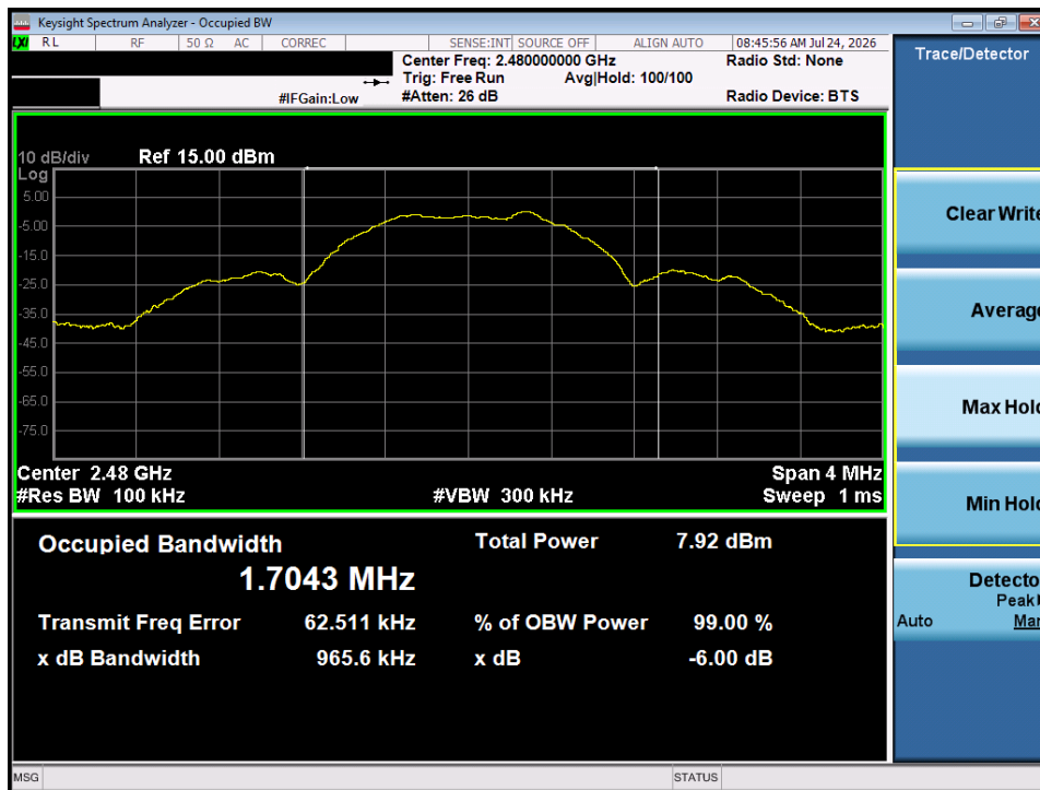
Plot 7-3. 6dB Bandwidth Plot (ANT/ANT+ – Ch. 79)
