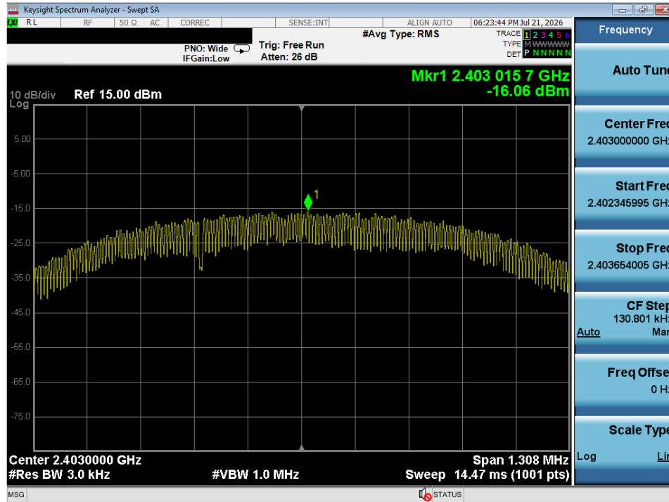
Plot 7-15. Power Spectral Density Plot (ANT/ANT+ – Ch. 2)
