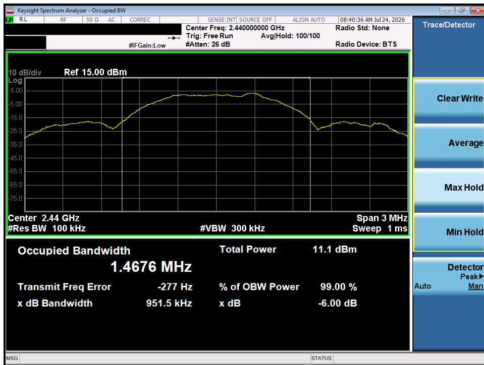
Plot 7-2. 6dB Bandwidth Plot (ANT/ANT+ – Ch. 39)
