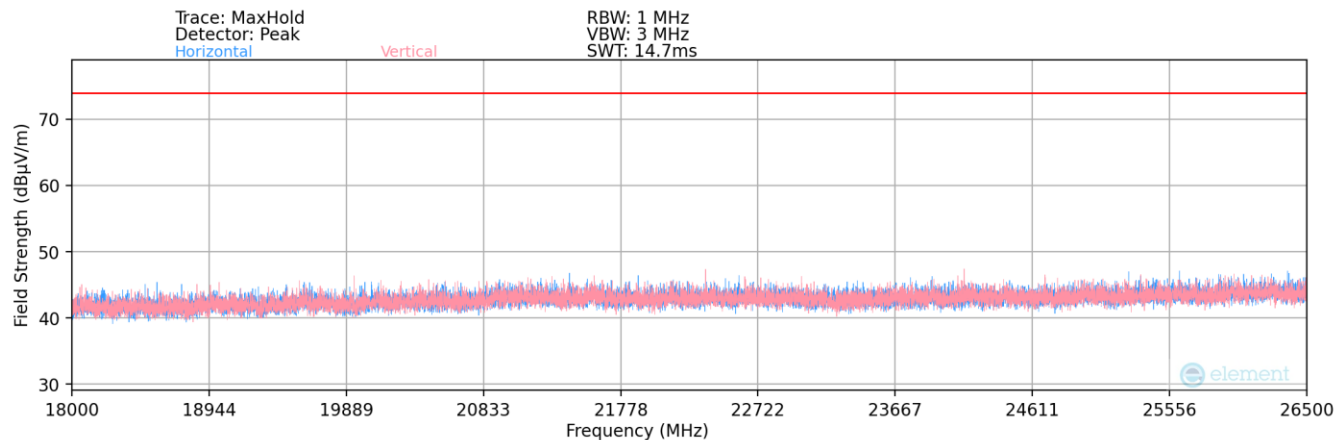
Plot 7-36. Radiated Spurious Plot above 18GHz (ANT/ANT+ – Ch. 39)
