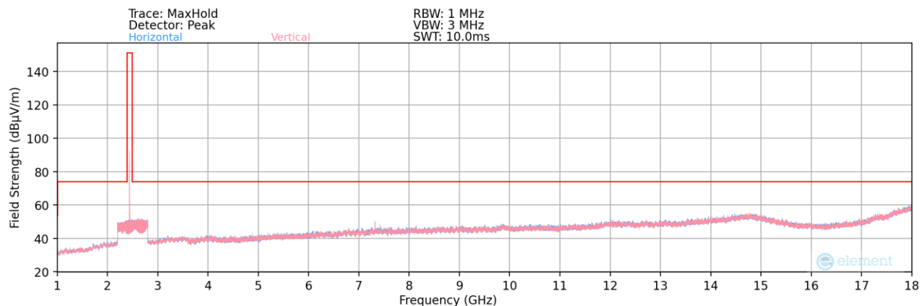
Plot 7-34. Radiated Spurious Plot above 1GHz (ANT/ANT+ – Ch. 39)
