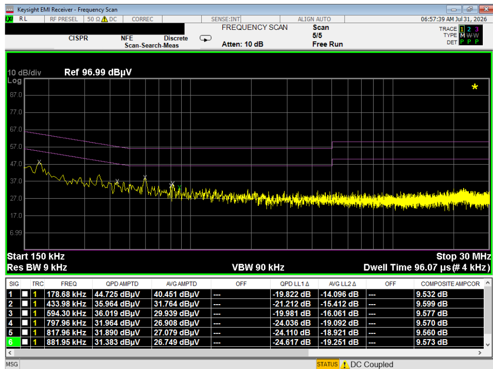
Plot 7-43. Line Conducted Plot with ANT/ANT+ (N)
