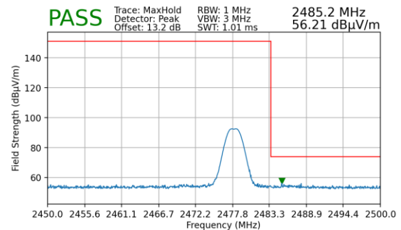
Plot 7-38. Radiated Restricted Upper Band Edge Measurement (Peak)
