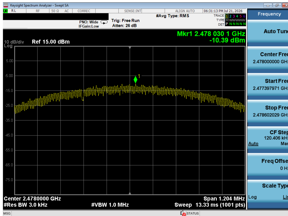
Plot 7-18. Power Spectral Density Plot (ANT/ANT+ – Ch. 77)
