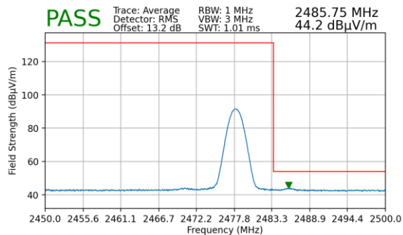
Plot 7-37. Radiated Restricted Upper Band Edge Measurement (Average)
