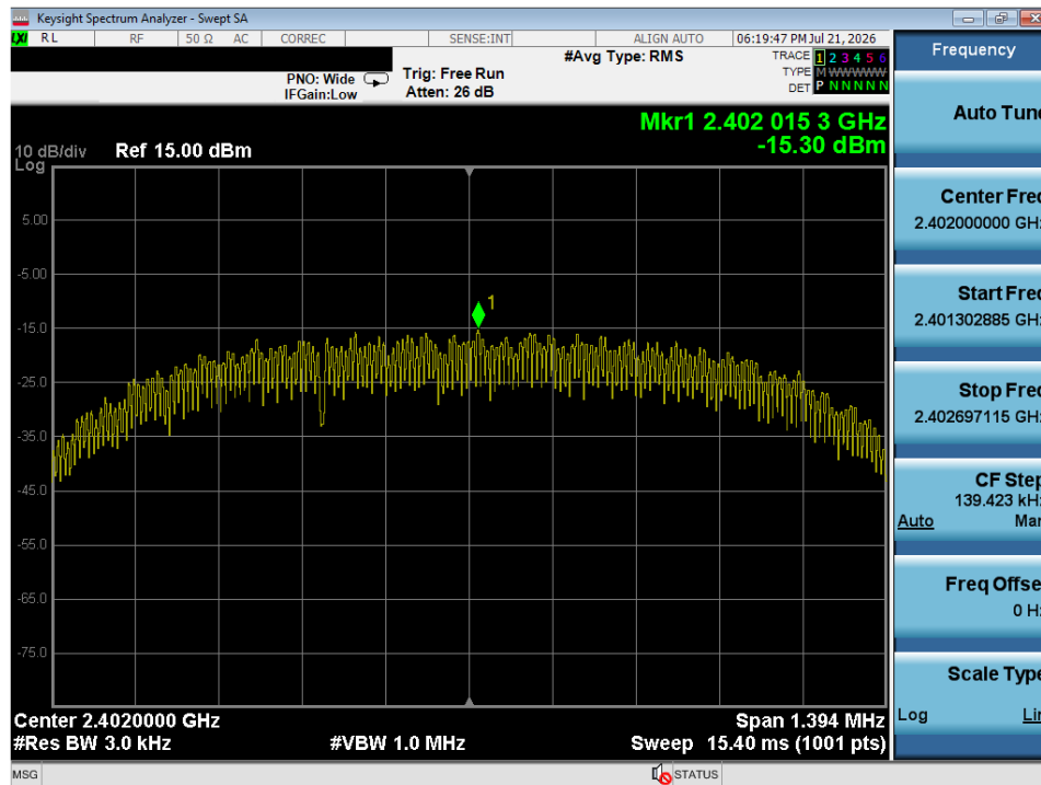
Plot 7-14. Power Spectral Density Plot (ANT/ANT+ – Ch. 1)
