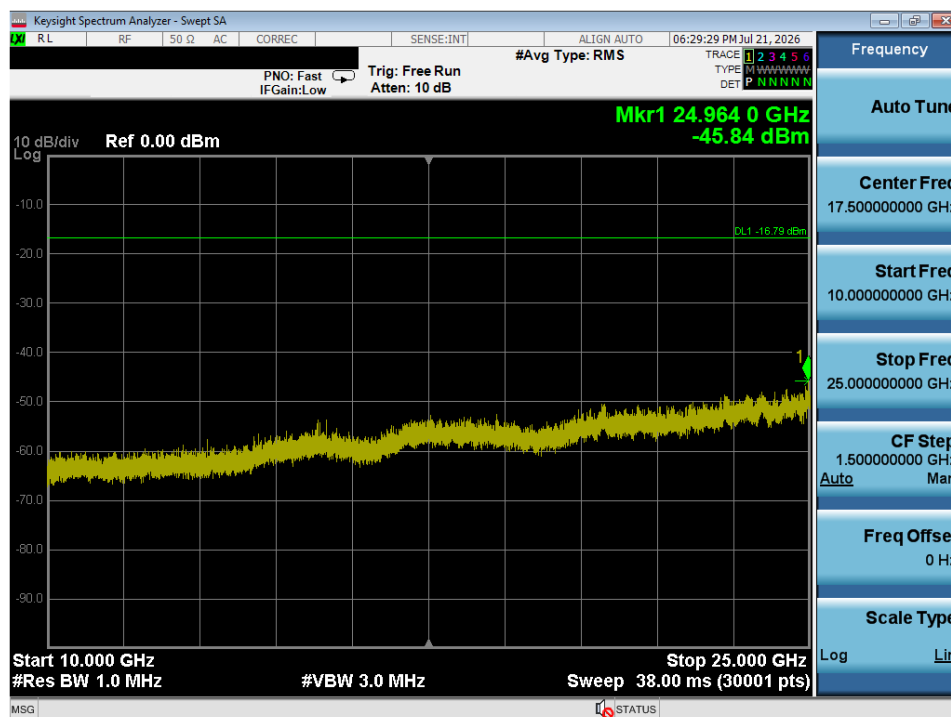
Plot 7-30. Conducted Spurious Plot (ANT/ANT+ – Ch. 39)
