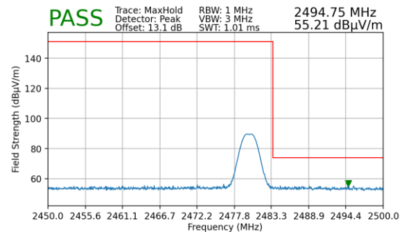
Plot 7-40. Radiated Restricted Upper Band Edge Measurement (Peak)
