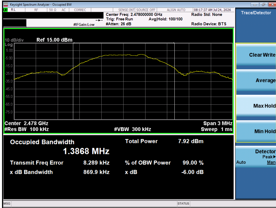
Plot 7-5. 6dB Bandwidth Plot (Bluetooth (LE), 1Mbps – Ch. 36)
