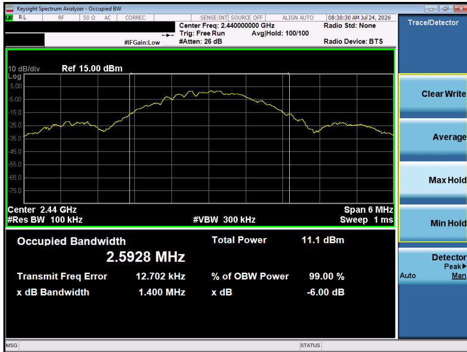
Plot 7-8. 6dB Bandwidth Plot (Bluetooth (LE), 2Mbps – Ch. 17)
