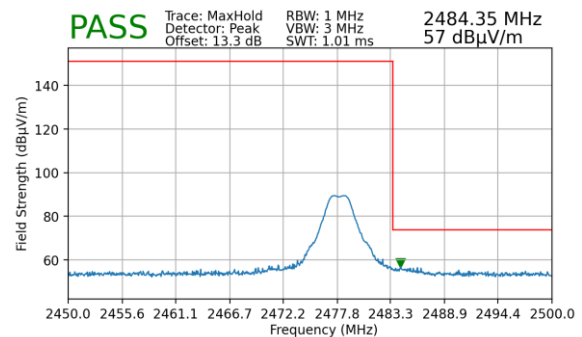
Plot 7-58. Radiated Restricted Upper Band Edge Measurement (Peak)
