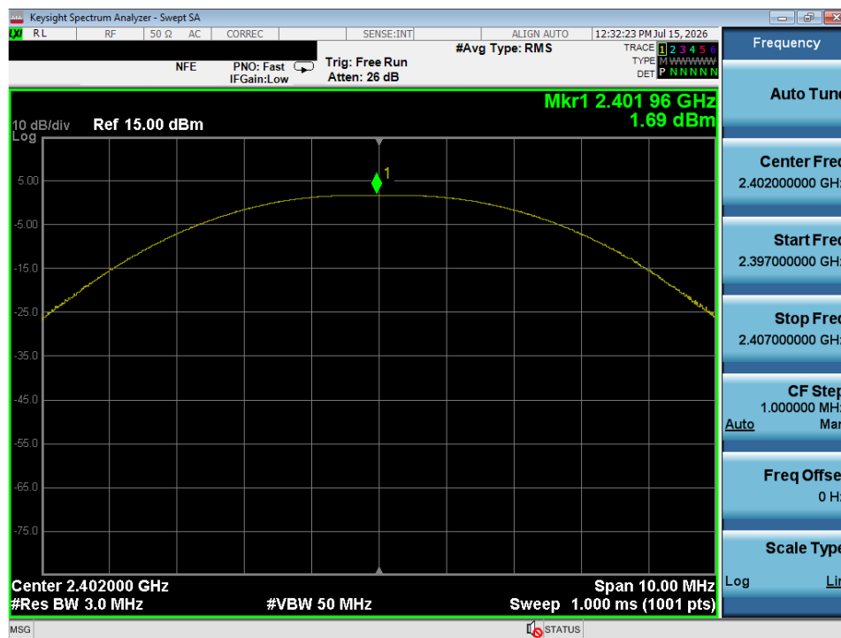
Plot 7-17. Peak Power Plot (Bluetooth (LE), 1Mbps – Ch. 37)
