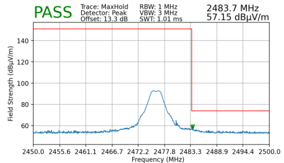
Plot 7-56. Radiated Restricted Upper Band Edge Measurement (Peak)
