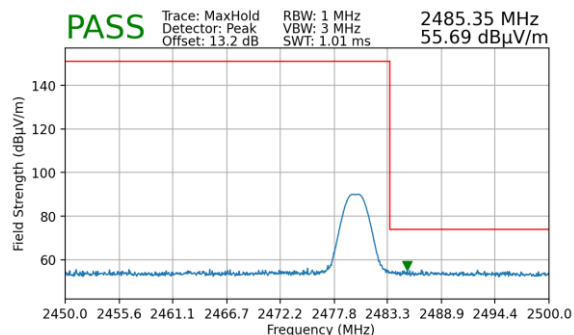
Plot 7-60. Radiated Restricted Upper Band Edge Measurement (Peak)
