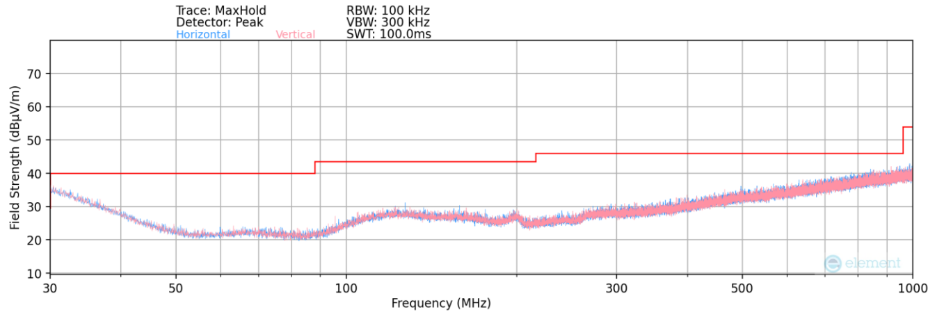
Plot 7-61. Radiated Spurious Plot below 1GHz
