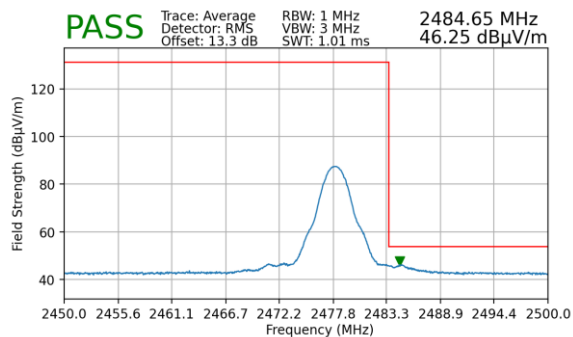
Plot 7-57. Radiated Restricted Upper Band Edge Measurement (Average)
