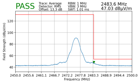
Plot 7-55. Radiated Restricted Upper Band Edge Measurement (Average)
