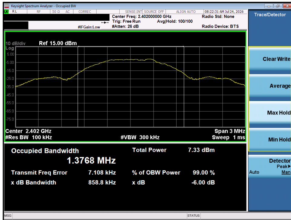
Plot 7-1. 6dB Bandwidth Plot (Bluetooth (LE), 1Mbps – Ch. 37)
