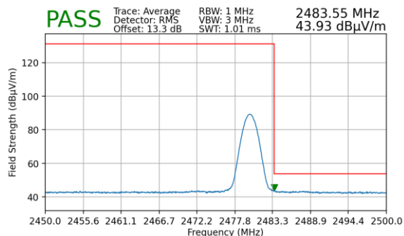
Plot 7-59. Radiated Restricted Upper Band Edge Measurement (Average)
