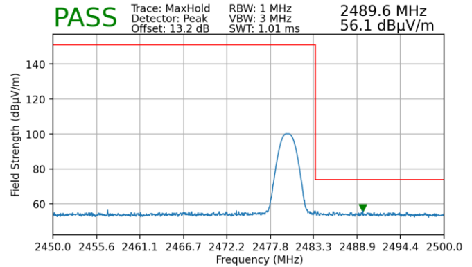
Plot 7-47. Radiated Restricted Upper Band Edge Measurement (Peak)
