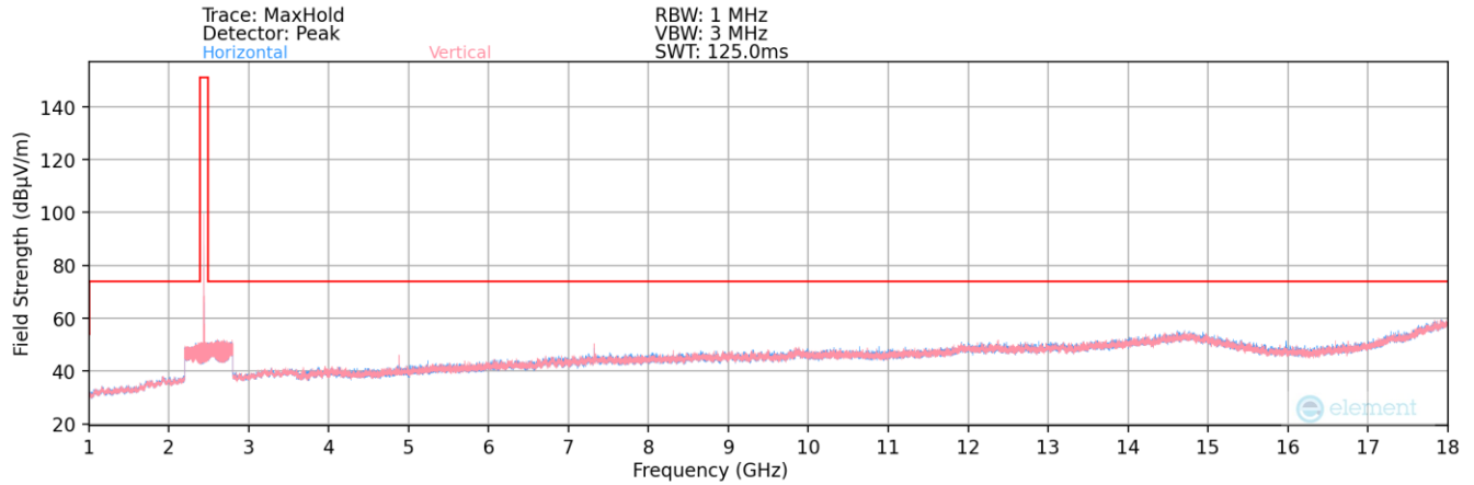
Plot 7-43. Radiated Spurious Plot above 1GHz (BT – Ch. 39) – Ant 1
