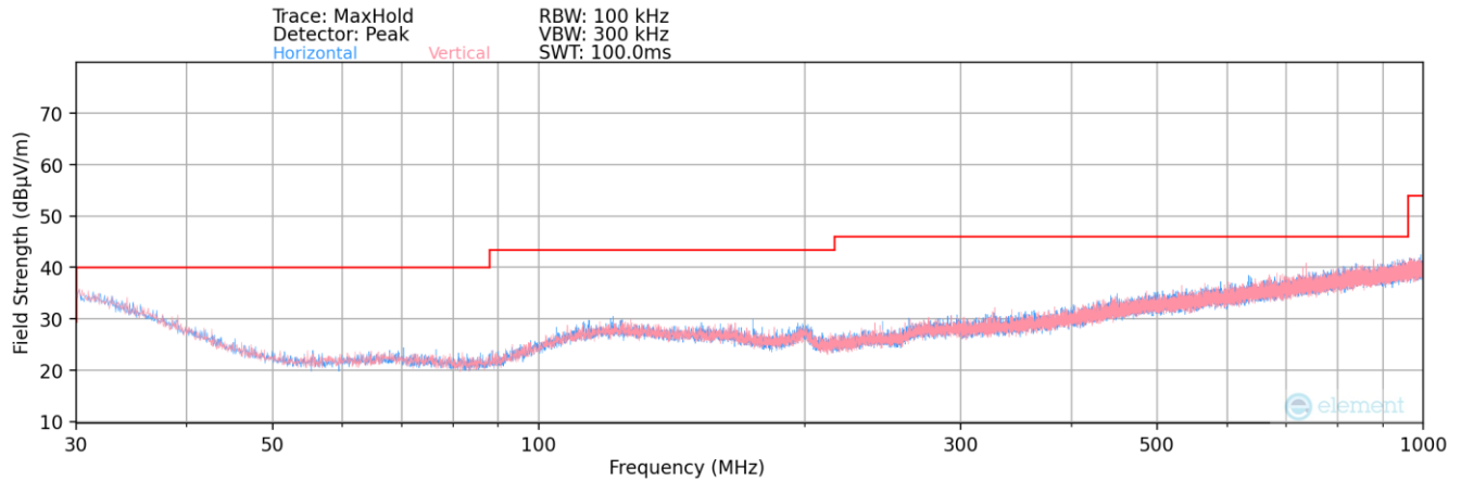
Plot 7-48. Radiated Spurious Plot below 1GHz – Ant 1
