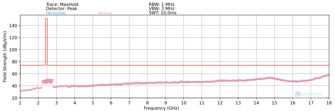
Plot 7-44. Radiated Spurious Plot above 1GHz (BT – Ch. 78) – Ant 1
