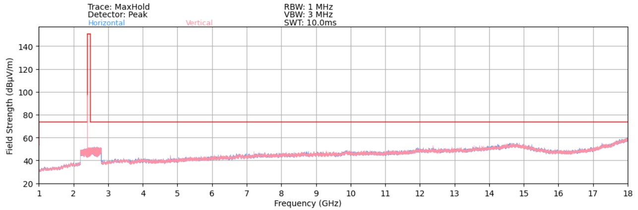
Plot 7-42. Radiated Spurious Plot above 1GHz (BT – Ch. 0) – Ant 1
