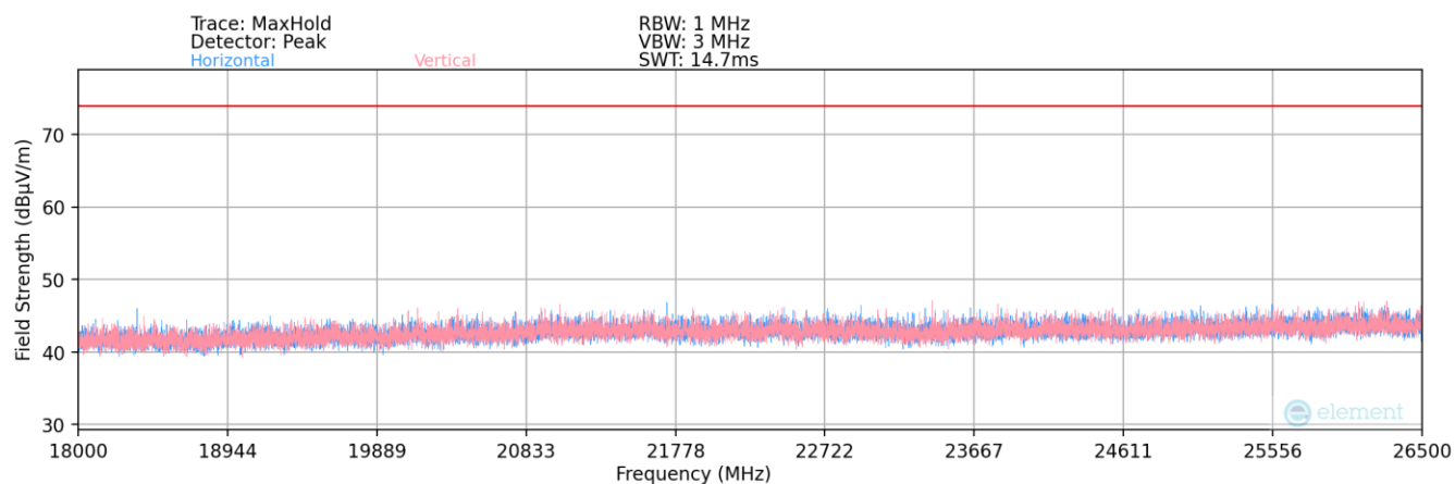
Plot 7-45. Radiated Spurious Plot above 18GHz – Ant 1
