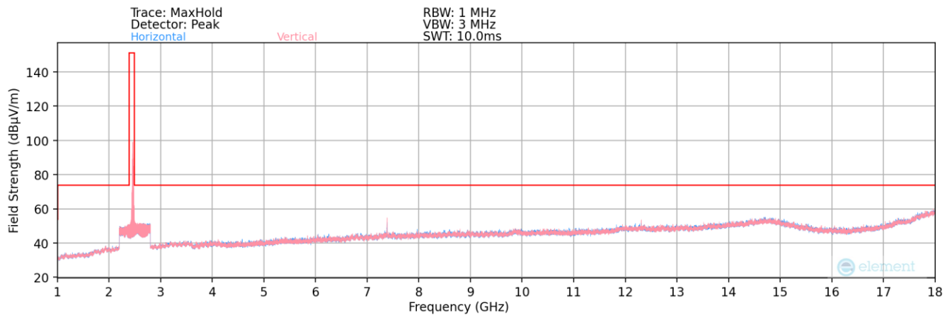
Plot 7-59. Radiated Spurious Plot above 1GHz (802.11b – Ch. OFDM 11)
