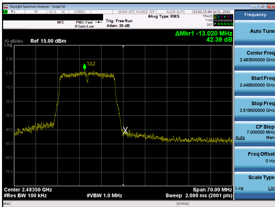
Plot 7-49. Band Edge Plot (802.11n – Ch. 13)
