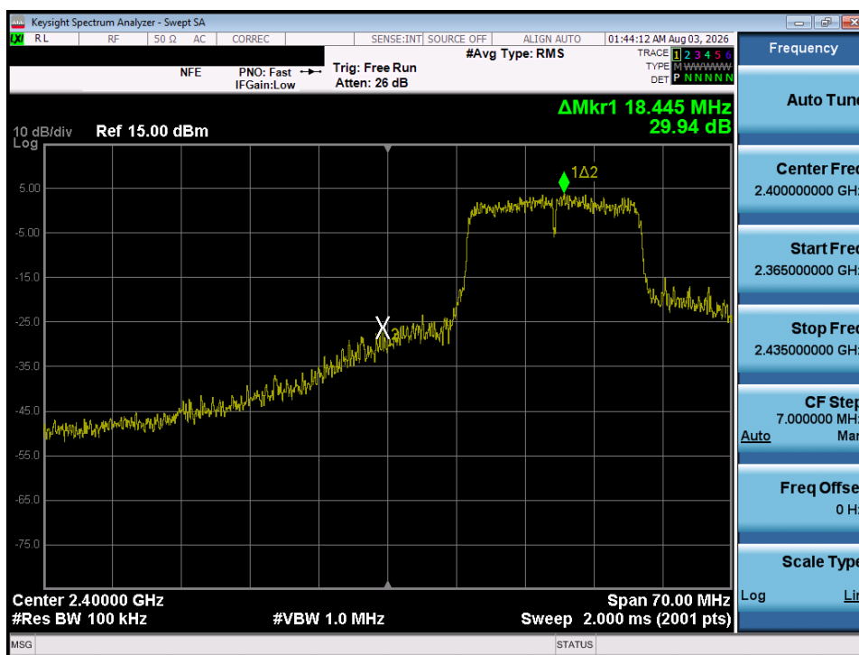
Plot 7-45. Band Edge Plot (802.11n – Ch. 2)
