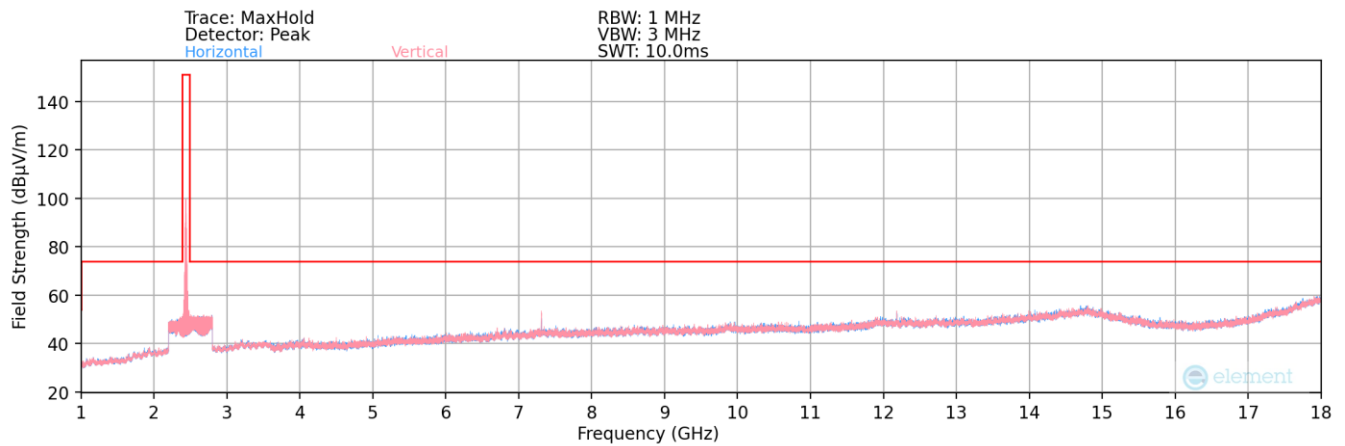
Plot 7-58. Radiated Spurious Plot above 1GHz (802.11b – Ch. OFDM 6)
