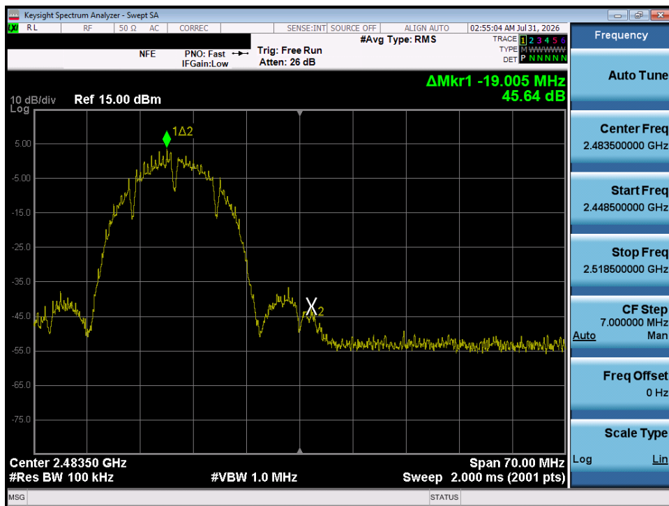
Plot 7-35. Band Edge Plot (802.11b – Ch. 12)
