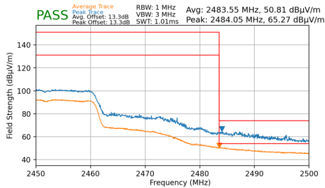
Plot 7-65. Radiated Restricted Upper Band Edge Measurement (Average & Peak)
