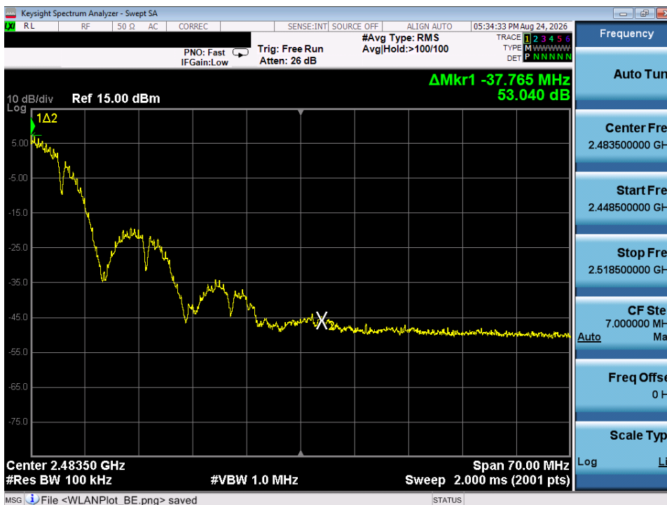
Plot 7-31. Band Edge Plot (802.11b – Ch. 8)
