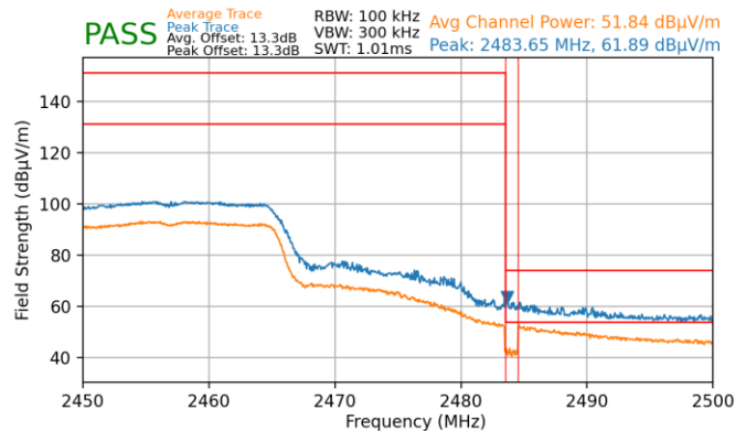
Plot 7-66. Radiated Restricted Upper Band Edge Measurement (Average & Peak)
