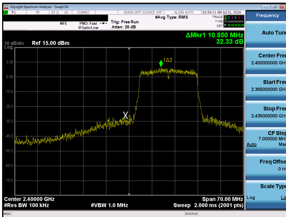
Plot 7-44. Band Edge Plot (802.11n – Ch. 1)
