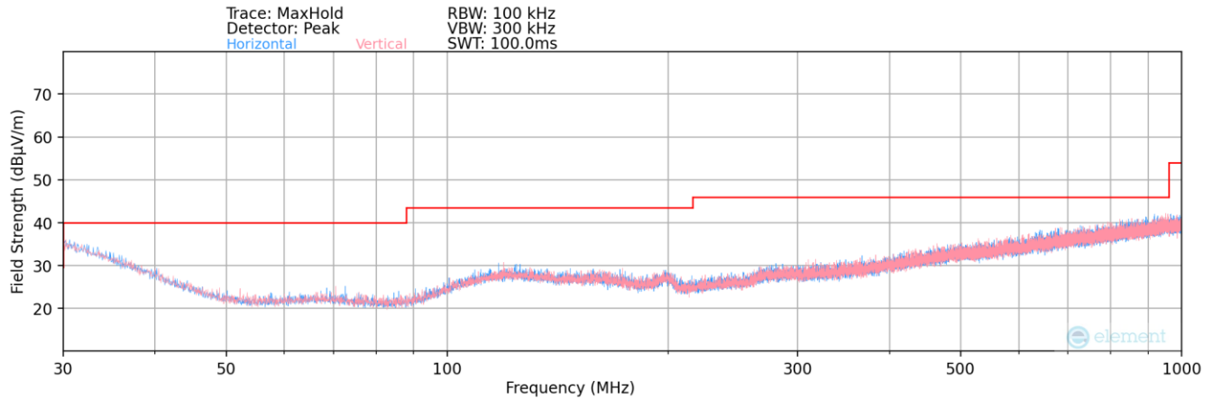
Plot 7-56. Radiated Spurious Plot below 1GHz
