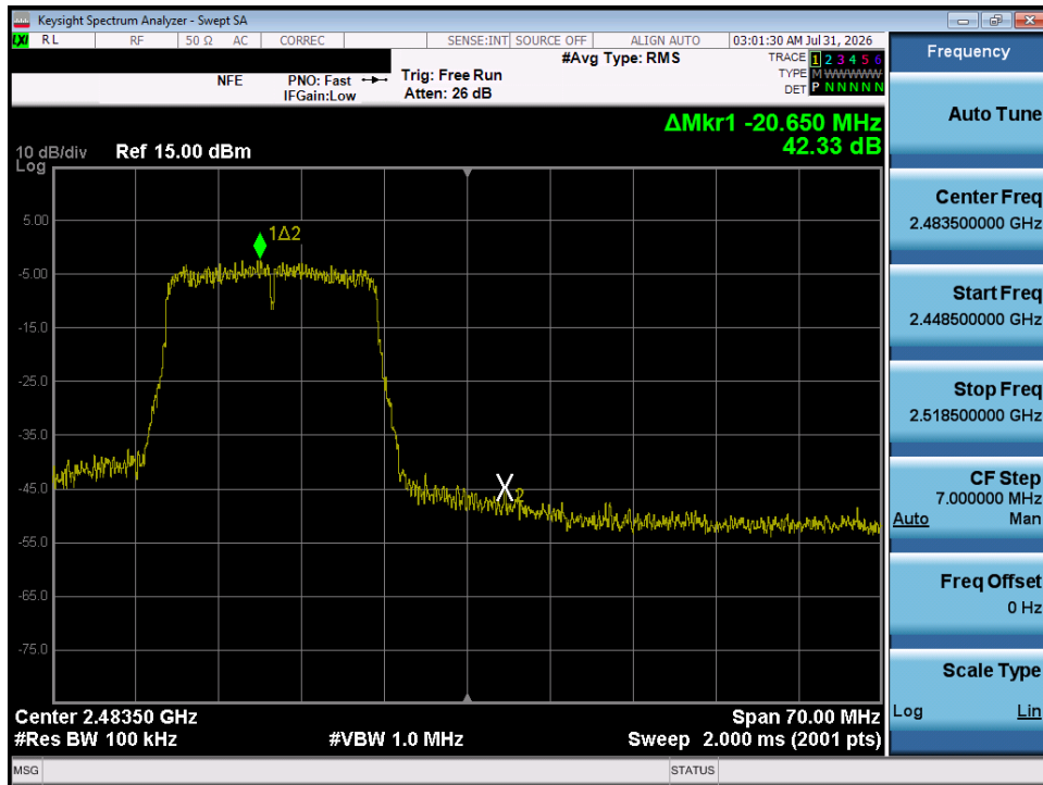
Plot 7-48. Band Edge Plot (802.11n – Ch. 12)
