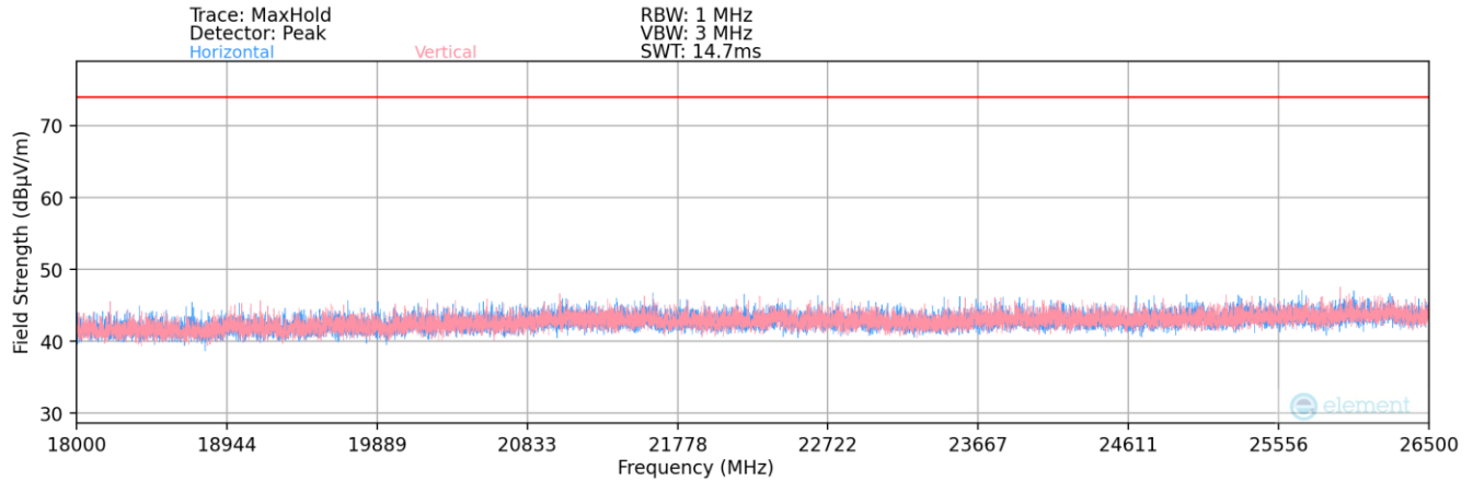
Plot 7-60. Radiated Spurious Plot above 18GHz
