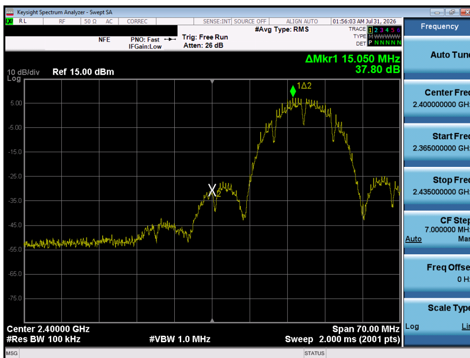
Plot 7-29. Band Edge Plot (802.11b – Ch. 2)
