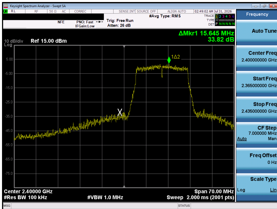
Plot 7-37. Band Edge Plot (802.11g– Ch. 1)
