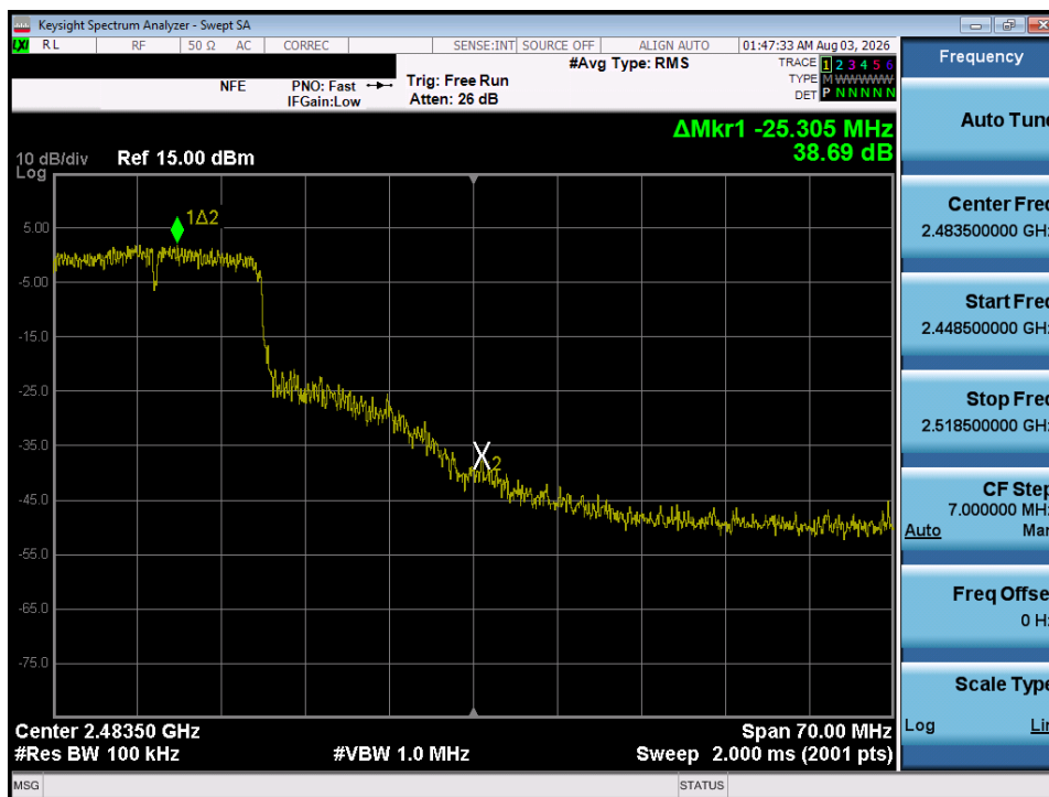
Plot 7-46. Band Edge Plot (802.11n – Ch. 10)
