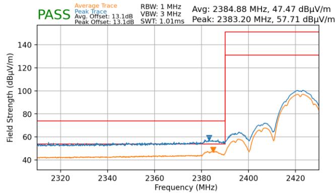
Plot 7-63. Radiated Restricted Lower Band Edge Measurement (Average & Peak)
