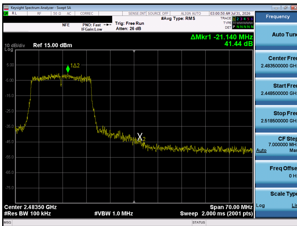
Plot 7-47. Band Edge Plot (802.11n – Ch. 11)
