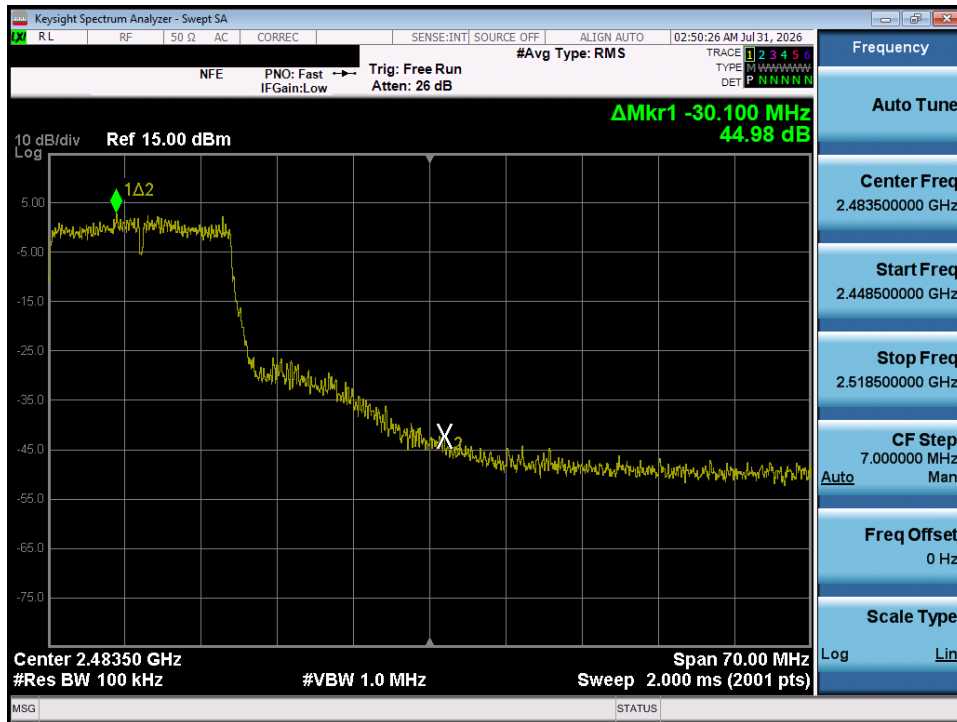
Plot 7-40. Band Edge Plot (802.11g – Ch. 10)
