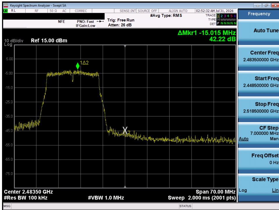
Plot 7-42. Band Edge Plot (802.11g – Ch. 12)
