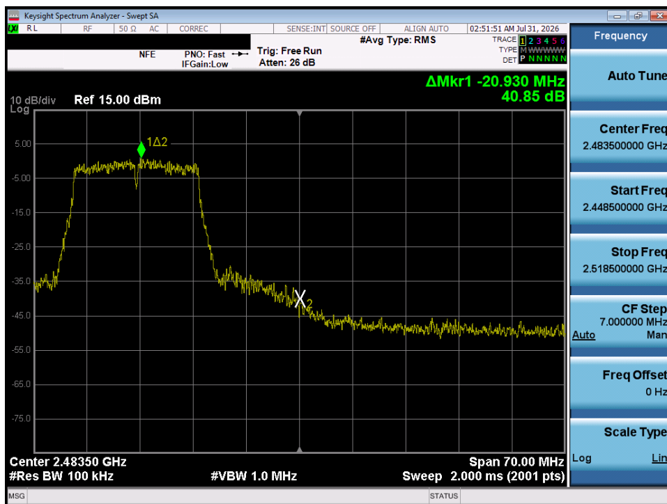
Plot 7-41. Band Edge Plot (802.11g – Ch. 11)
