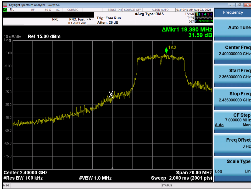
Plot 7-38. Band Edge Plot (802.11g– Ch. 2)
