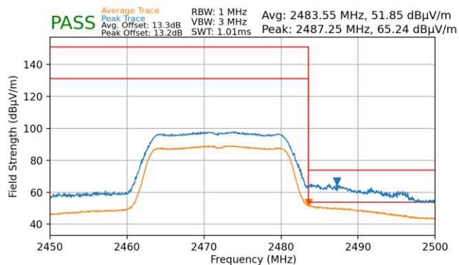
Plot 7-69. Radiated Restricted Upper Band Edge Measurement (Average & Peak)
