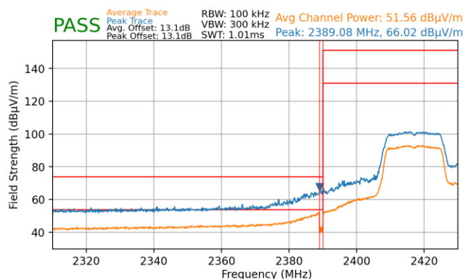
Plot 7-62. Radiated Restricted Lower Band Edge Measurement (Average & Peak)
