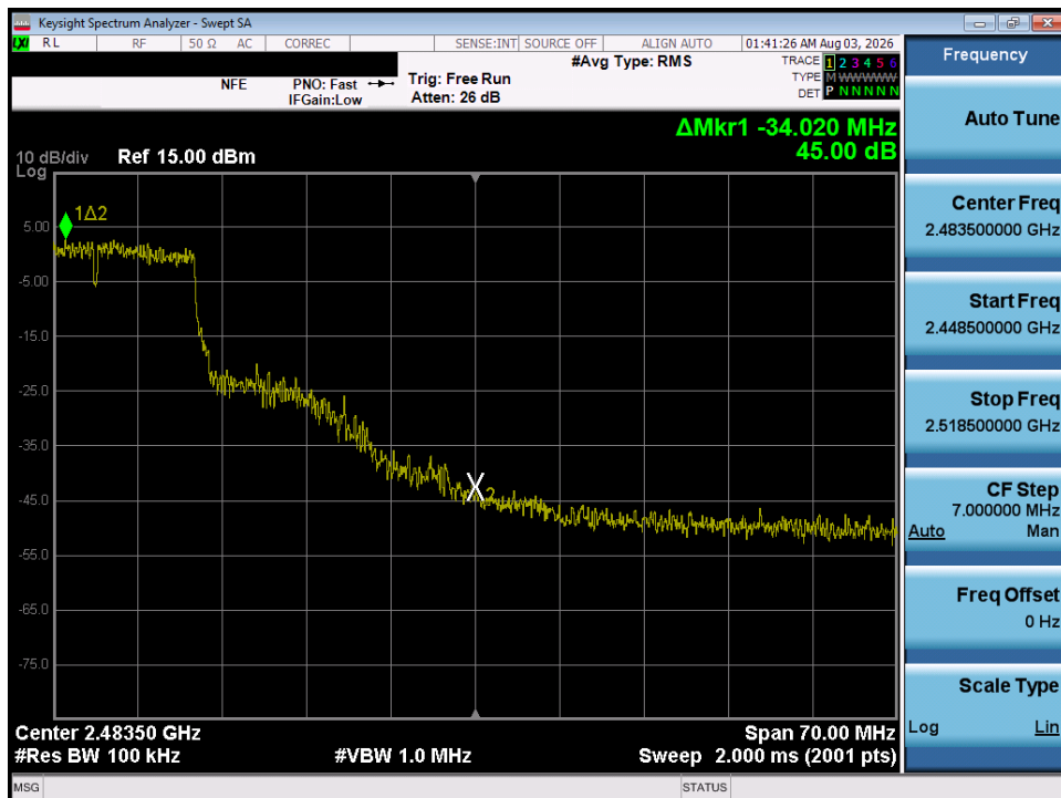
Plot 7-39. Band Edge Plot (802.11g – Ch. 9)
