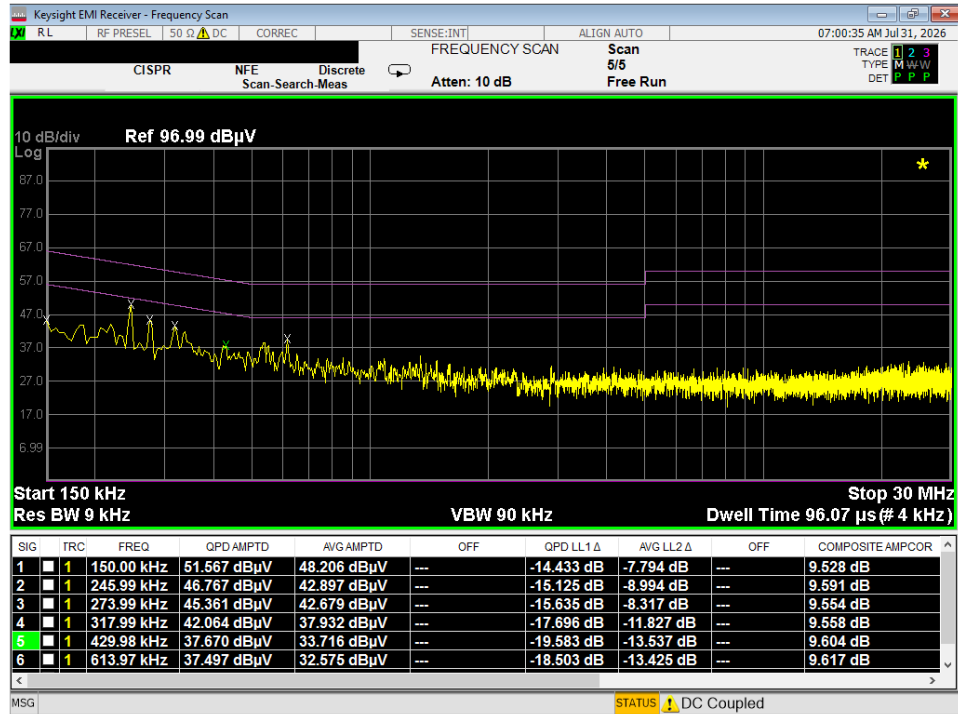
Plot 7-70. Line Conducted Plot with 802.11b (L1)
