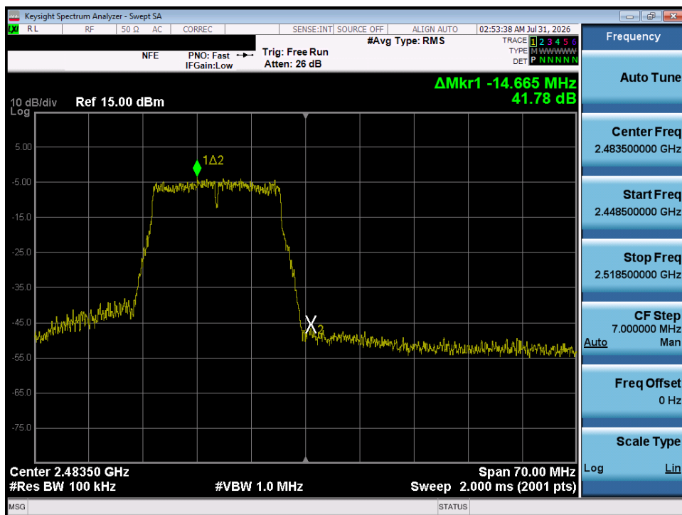
Plot 7-43. Band Edge Plot (802.11g – Ch. 13)
