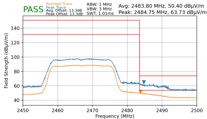
Plot 7-68. Radiated Restricted Upper Band Edge Measurement (Average & Peak)
