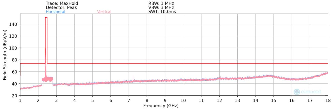
Plot 7-57. Radiated Spurious Plot above 1GHz (802.11b – Ch. OFDM 1)
