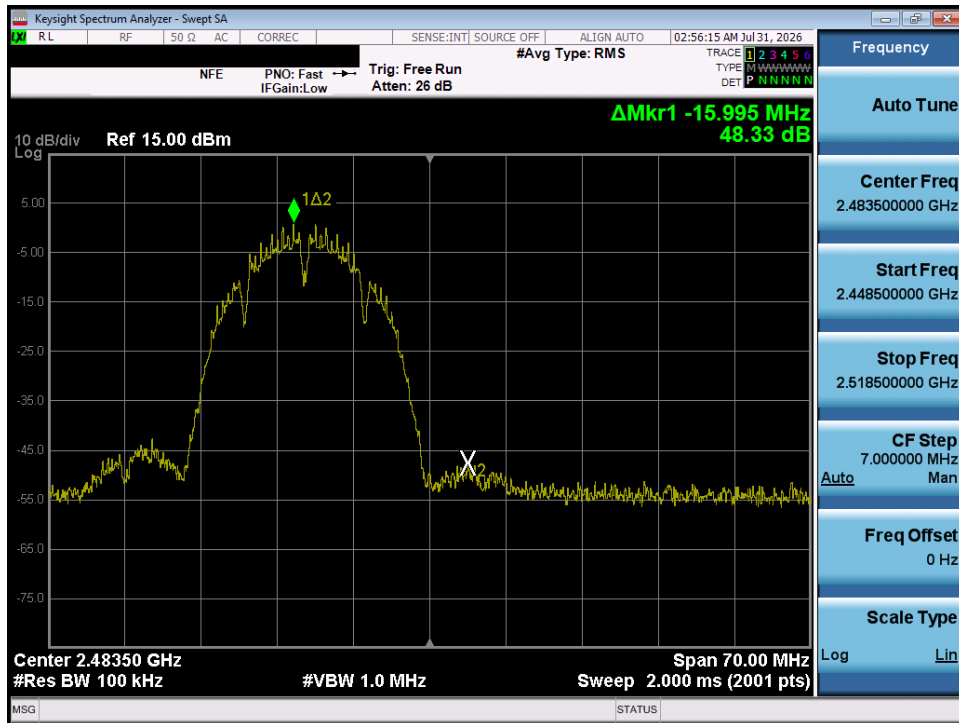
Plot 7-36. Band Edge Plot (802.11b – Ch. 13)
