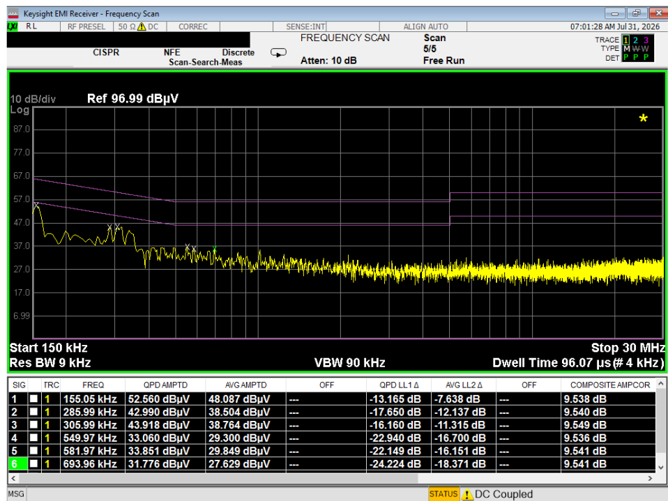
Plot 7-71. Line Conducted Plot with 802.11b (N)
