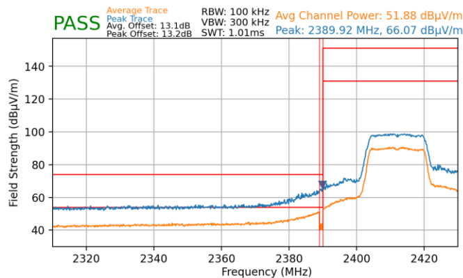
Plot 7-61. Radiated Restricted Lower Band Edge Measurement (Average & Peak)
