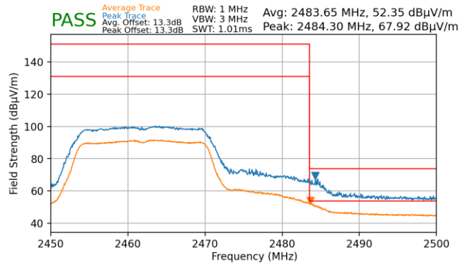
Plot 7-67. Radiated Restricted Upper Band Edge Measurement (Average & Peak)
