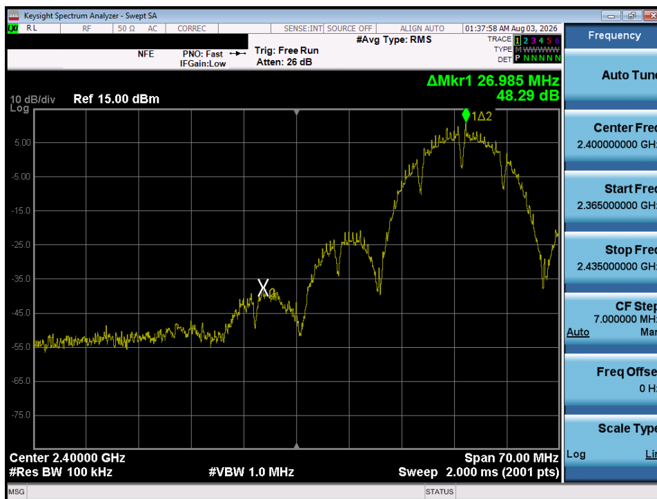
Plot 7-30. Band Edge Plot (802.11b – Ch. 3)
