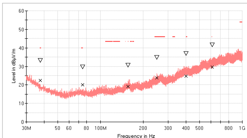
RF_FCC_15.407_E Field_30MHz_1GHz
