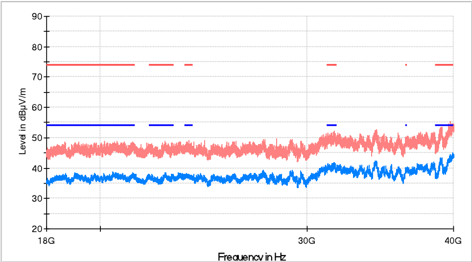
RF_FCC_15.407_E Field_18GHz_40GHz(SAC2)
