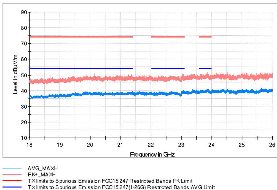
RF_FCC_15.247_E Field_18GHz_26GHz(SAC2)
