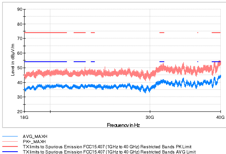
RF_FCC15.407_E Field_18GHz_40GHz(SAC2)
