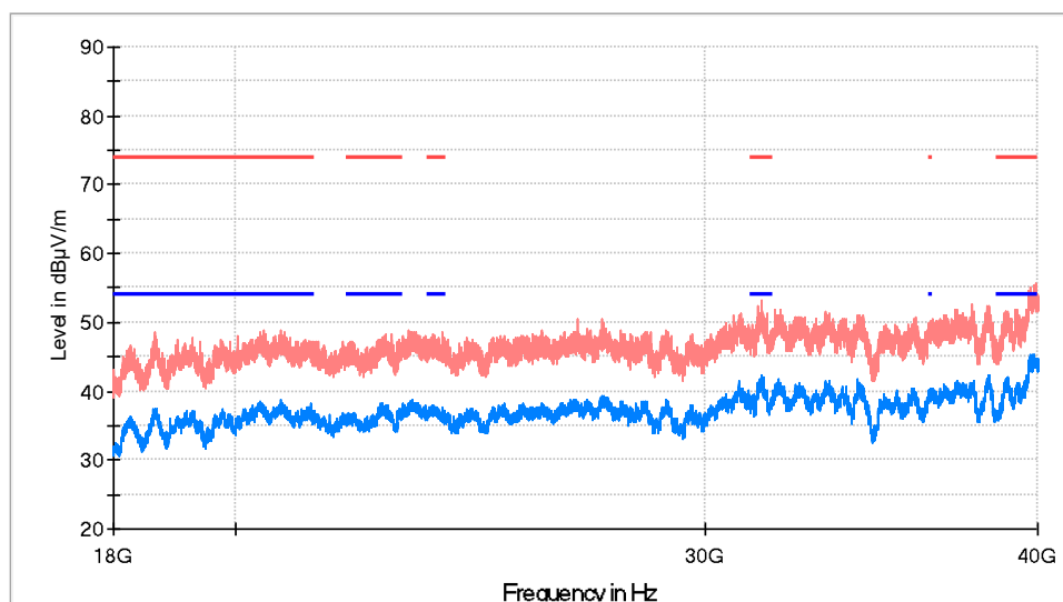
RF_FCC_15.407_E Field_18GHz_40GHz(SAC2)
