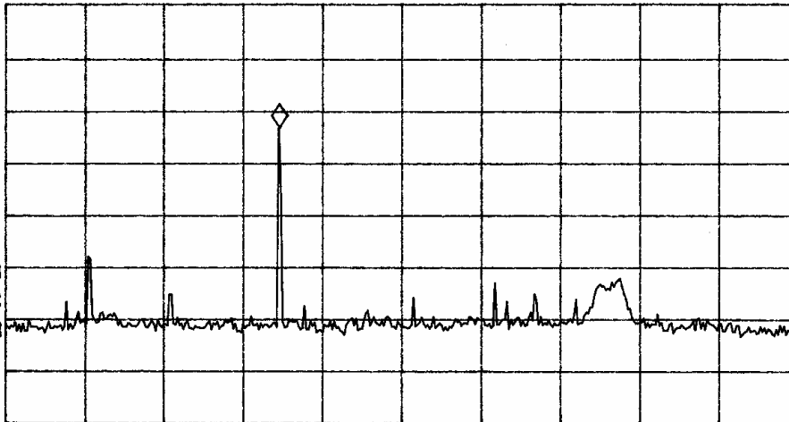
Figure five Radiated Emissions @ 1 Meter in Screen Room
