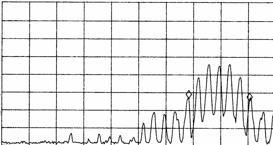
Figure two Band Edges of operation (at 107.9 MHz)
