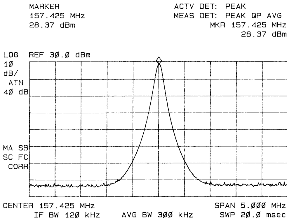
Figure 3: Low Power Output Channel 88A
