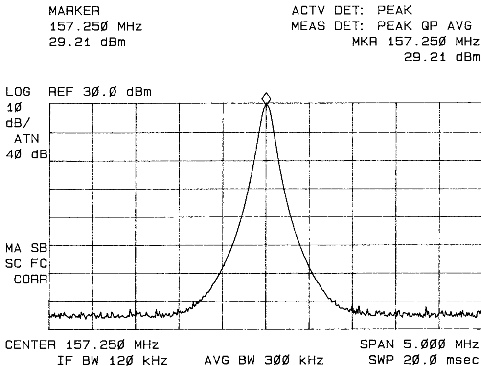
Figure 2: Low Power Output Channel 25
