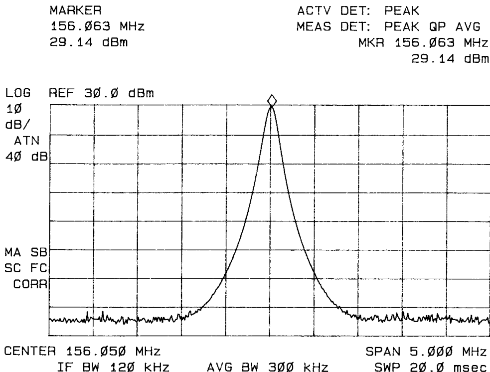
Figure 1: Low Power Output Channel 1A
