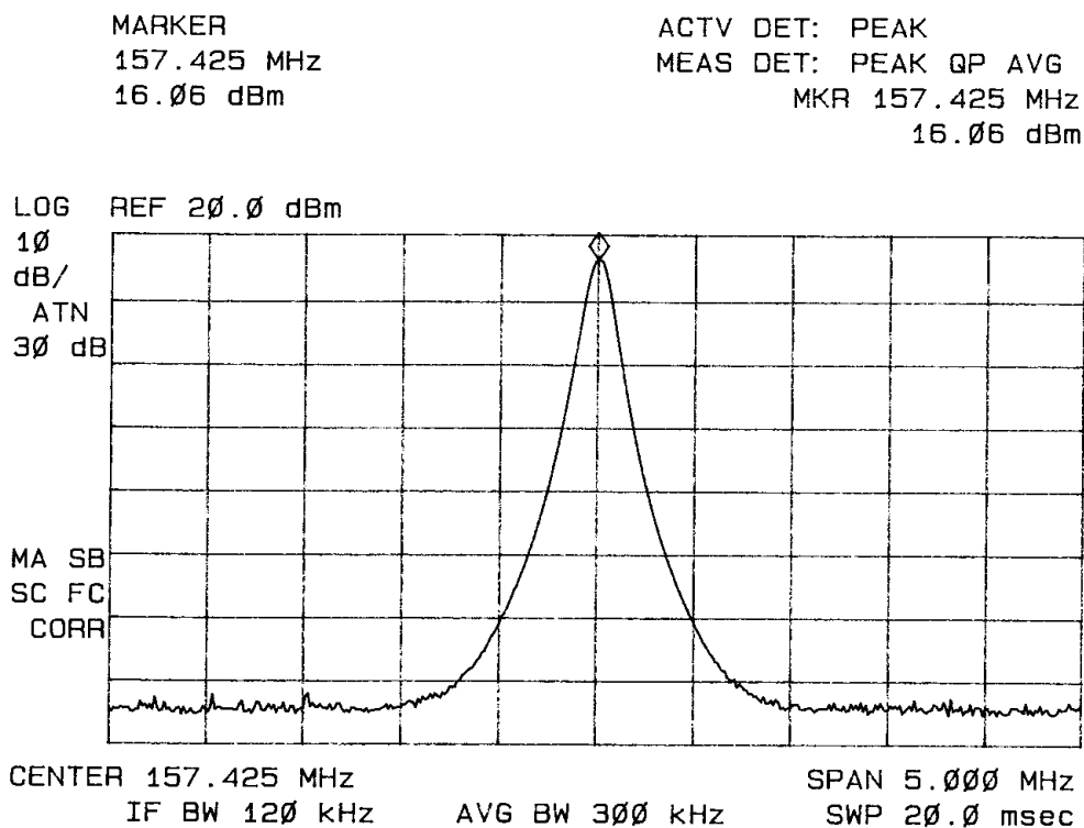
Figure 6: High Power Output Channel 88A
