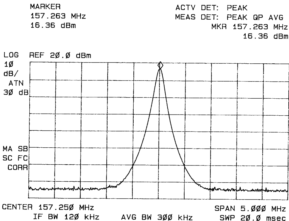
Figure 5: High Power Output Channel 25
