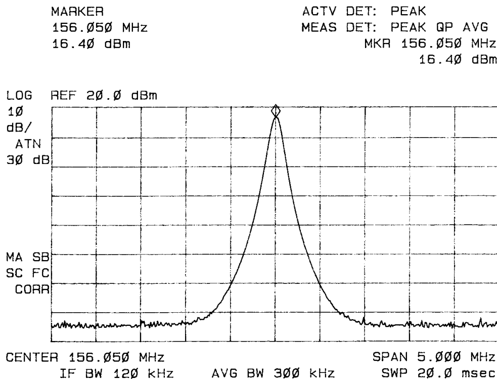
Figure 4: High Power Output Channel 1A
