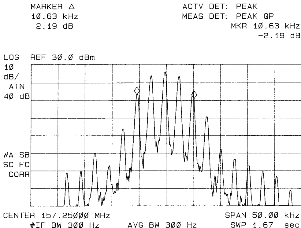
Figure 10: Occupied Band Width Channel 25 High Power.
