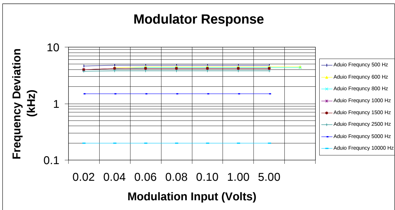
Figure 8: Modulation Characteristics.
