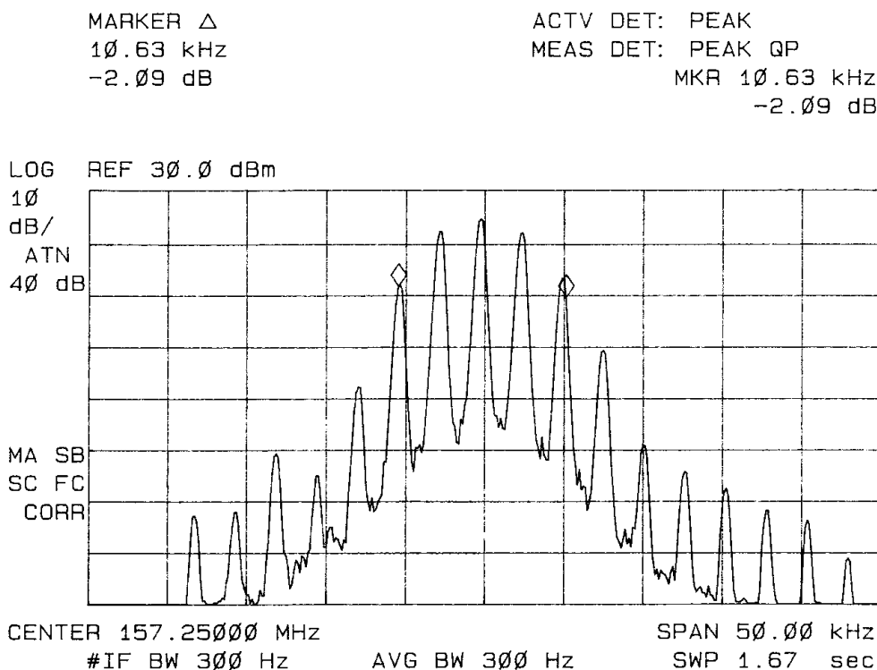
Figure 9: Occupied Band Width Channel 25 Low Power.
