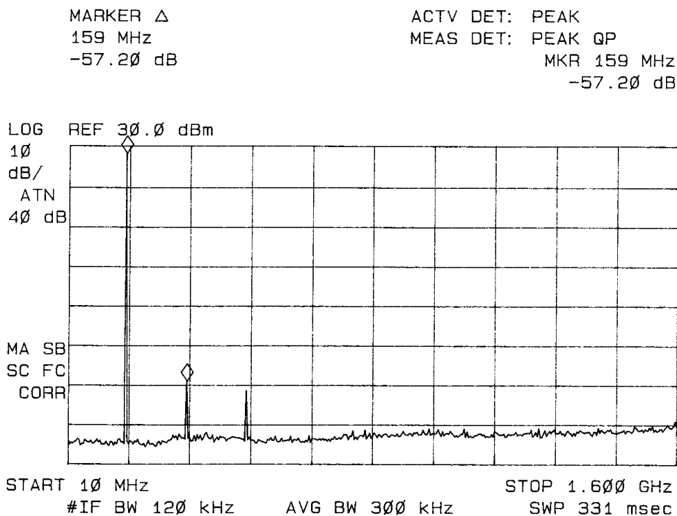
Figure 12: Emissions at Antenna Terminal.
