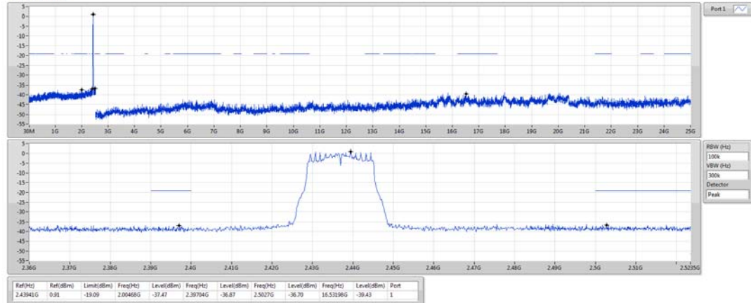
802.11g_Nss1,(6Mbps)_1TX 2437MHz
