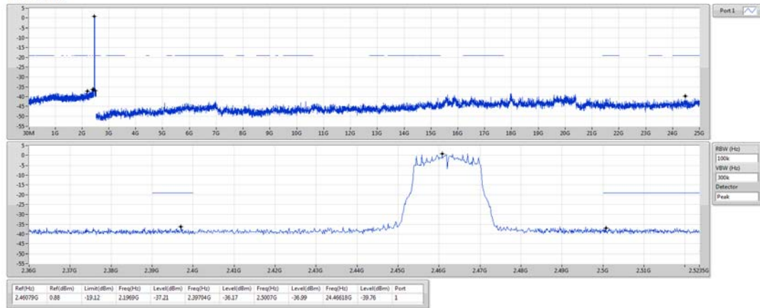
802.11g_Nss1,(6Mbps)_1TX 2462MHz
