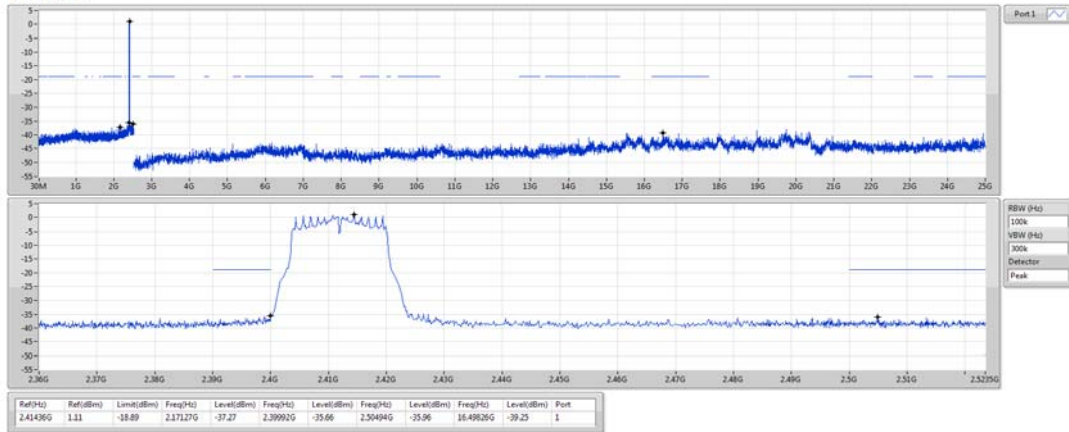
802.11g_Nss1,(6Mbps)_1TX 2412MHz
