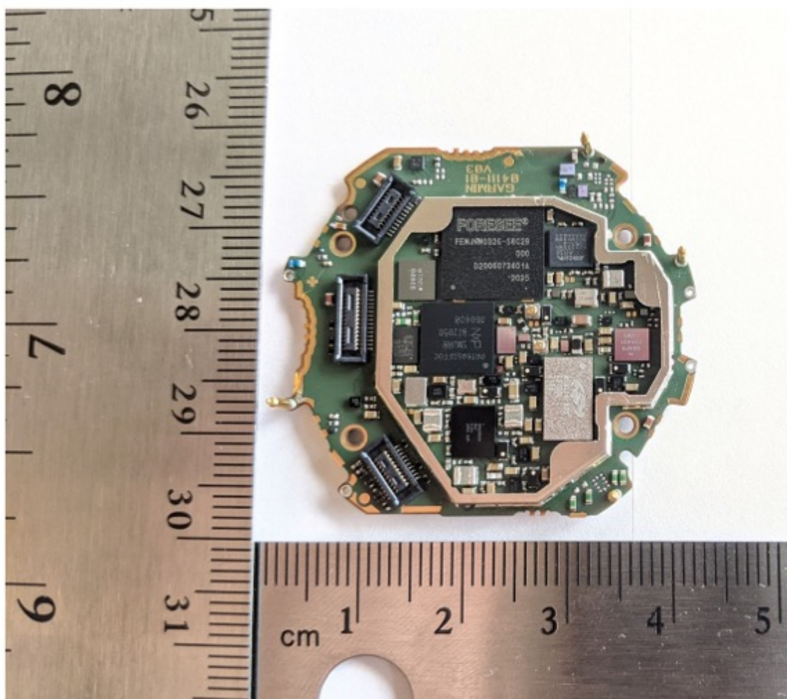
Front face of main PCB, shield removed
