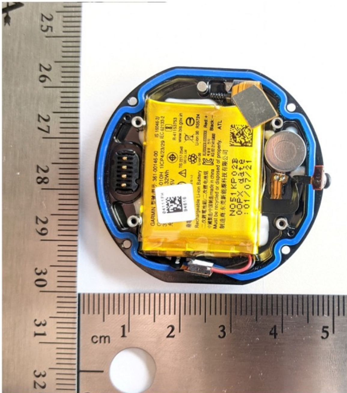
Inside of rear case
