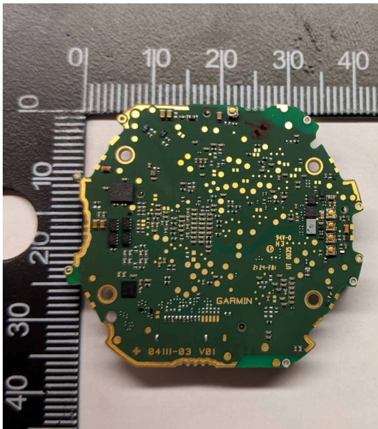
Rear face of main PCB
