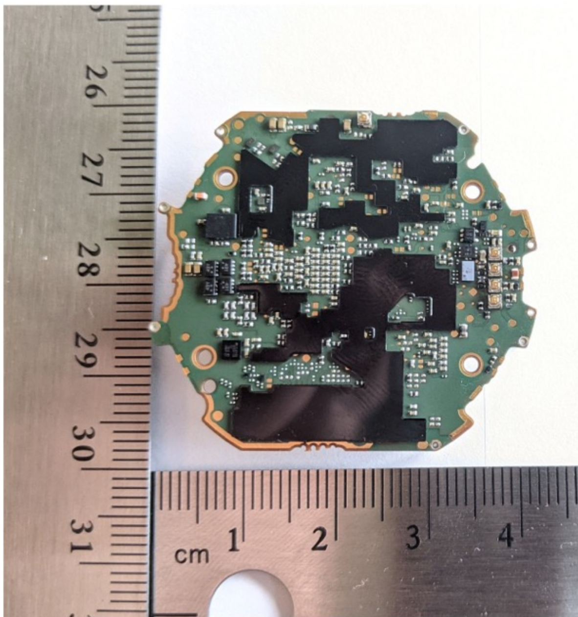
Rear face of main PCB
