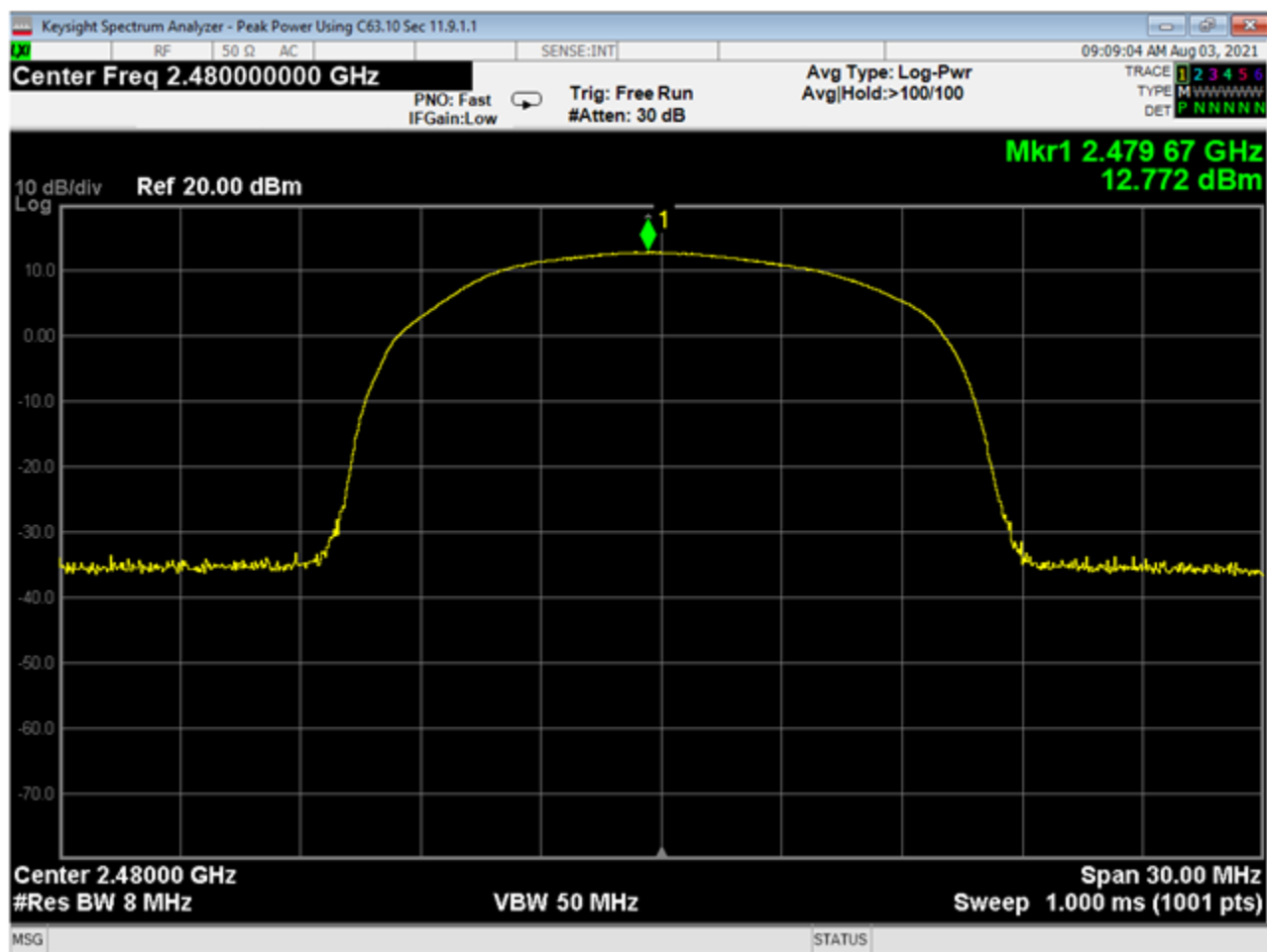
16 Peak Output Power, High Channel, 3EDR
