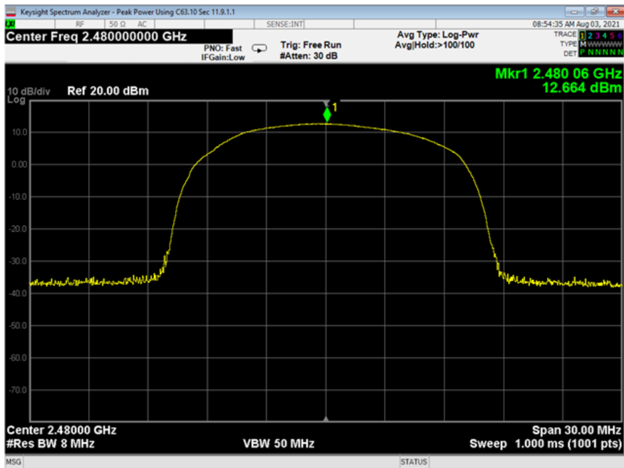
03 Peak Output Power, High Channel, 2EDR
