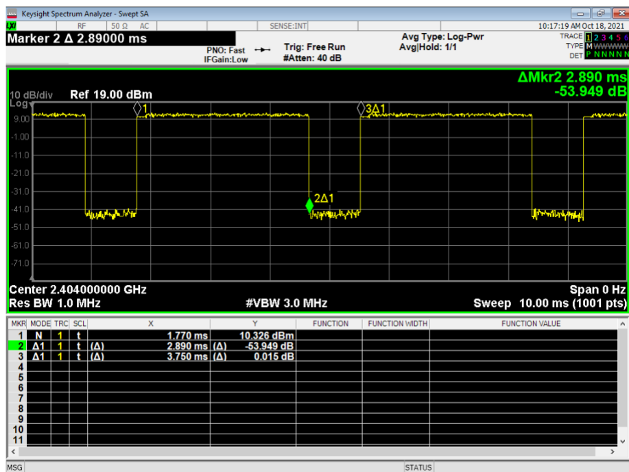
Figure 4 – 3EDR Duty Cycle
