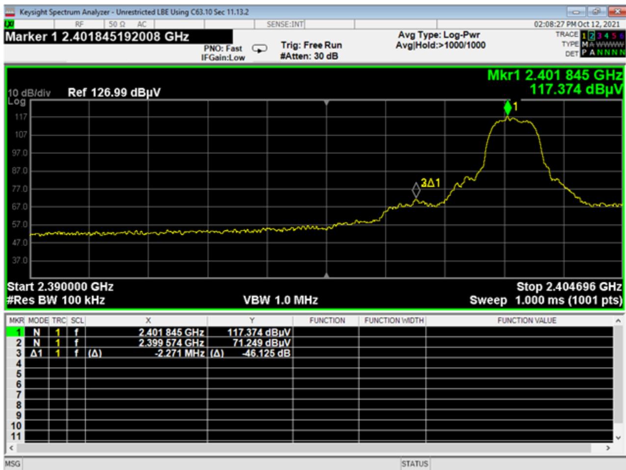
26 Lower Bandedge Unrestricted, 3EDR
