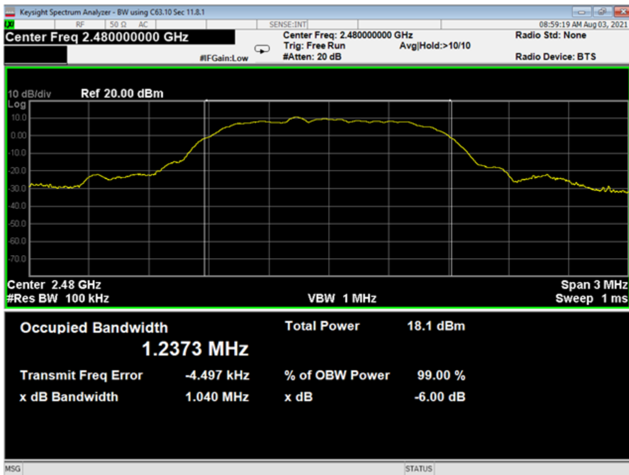
06 Bandwidth, High Channel, 2EDR
