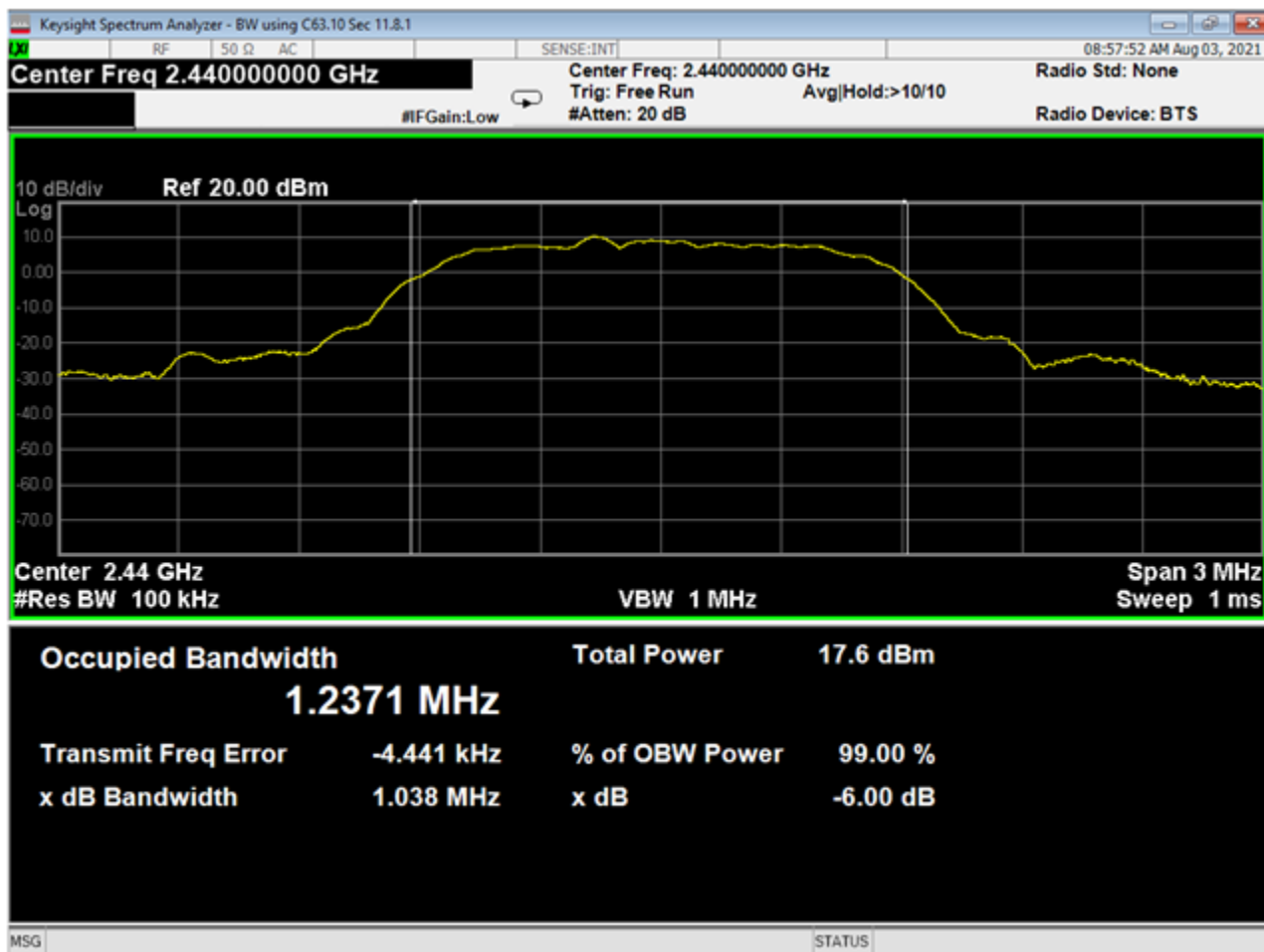
05 Bandwidth, Mid Channel, 2EDR
