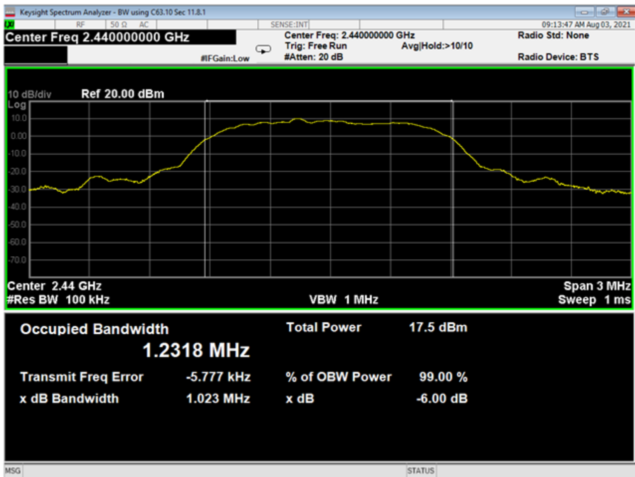
18 Bandwidth, Mid Channel, 3EDR
