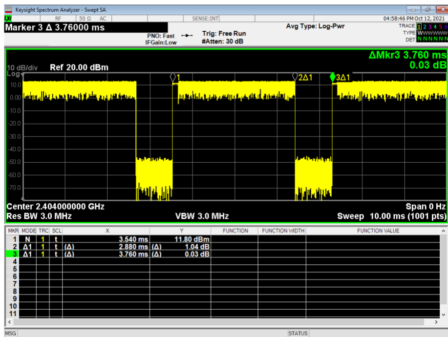
Figure 3 – 2EDR Duty Cycle
