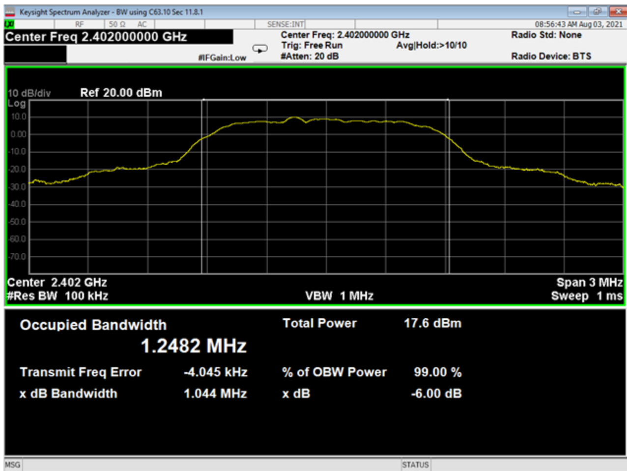
04 Bandwidth, Low Channel, 2EDR
