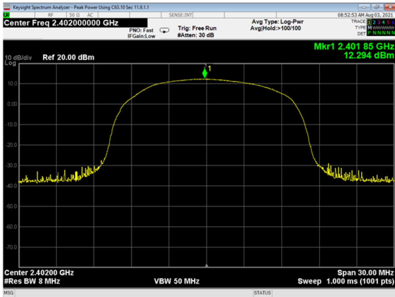
01 Peak Output Power, Low Channel, 2EDR
