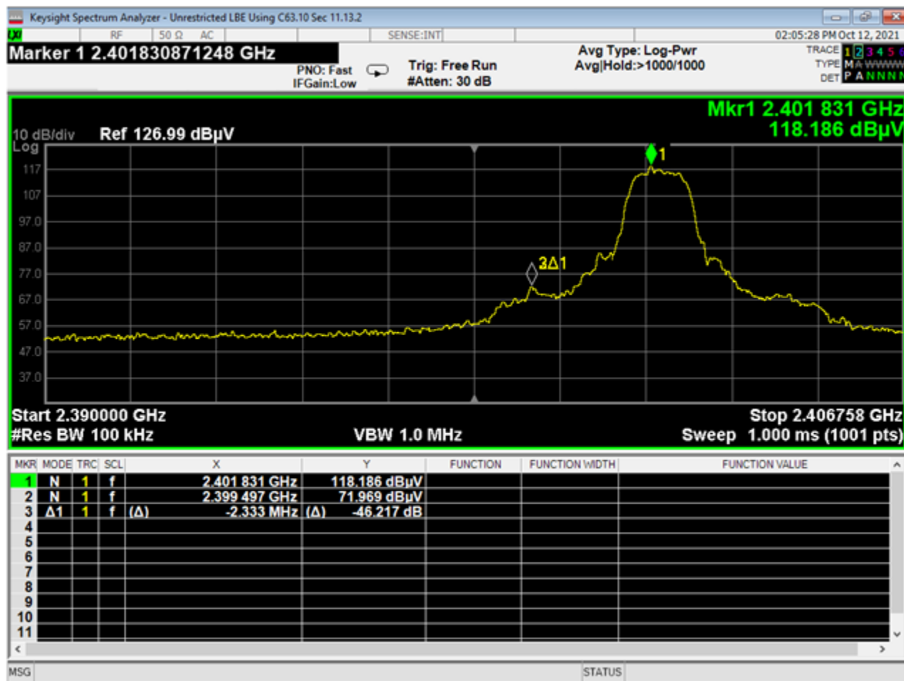
12 Lower Bandedge Unrestricted, 2EDR
