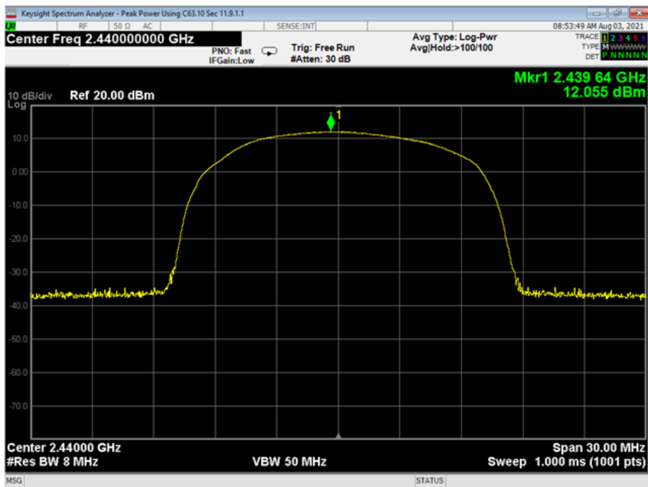
02 Peak Output Power, Mid Channel, 2EDR
