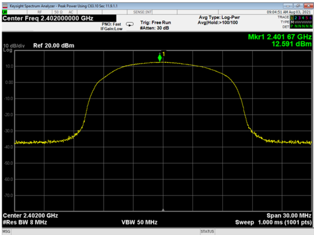
14 Peak Output Power, Low Channel, 3EDR
