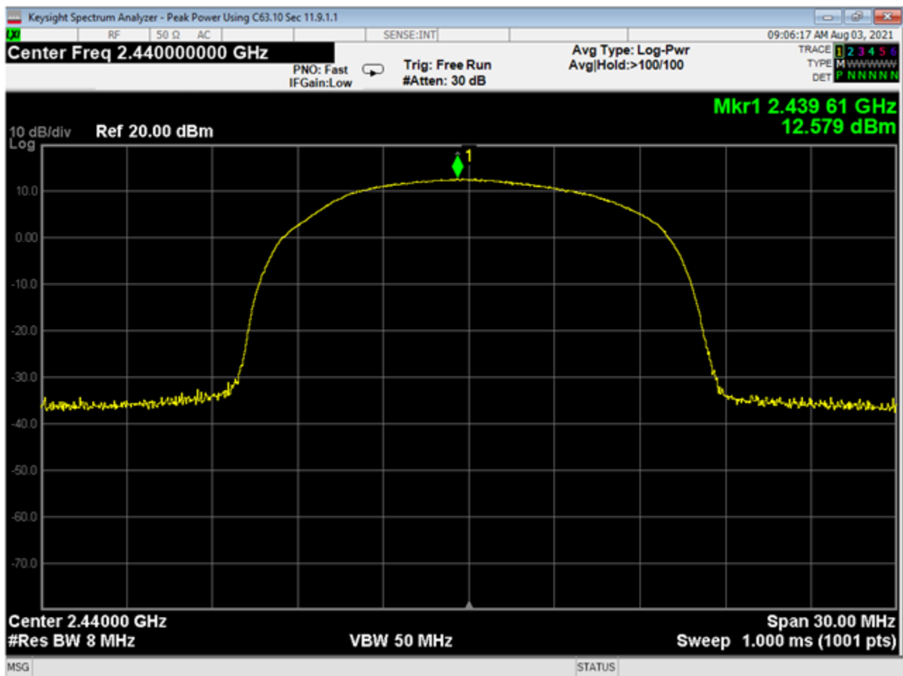
15 Peak Output Power, Mid Channel, 3EDR
