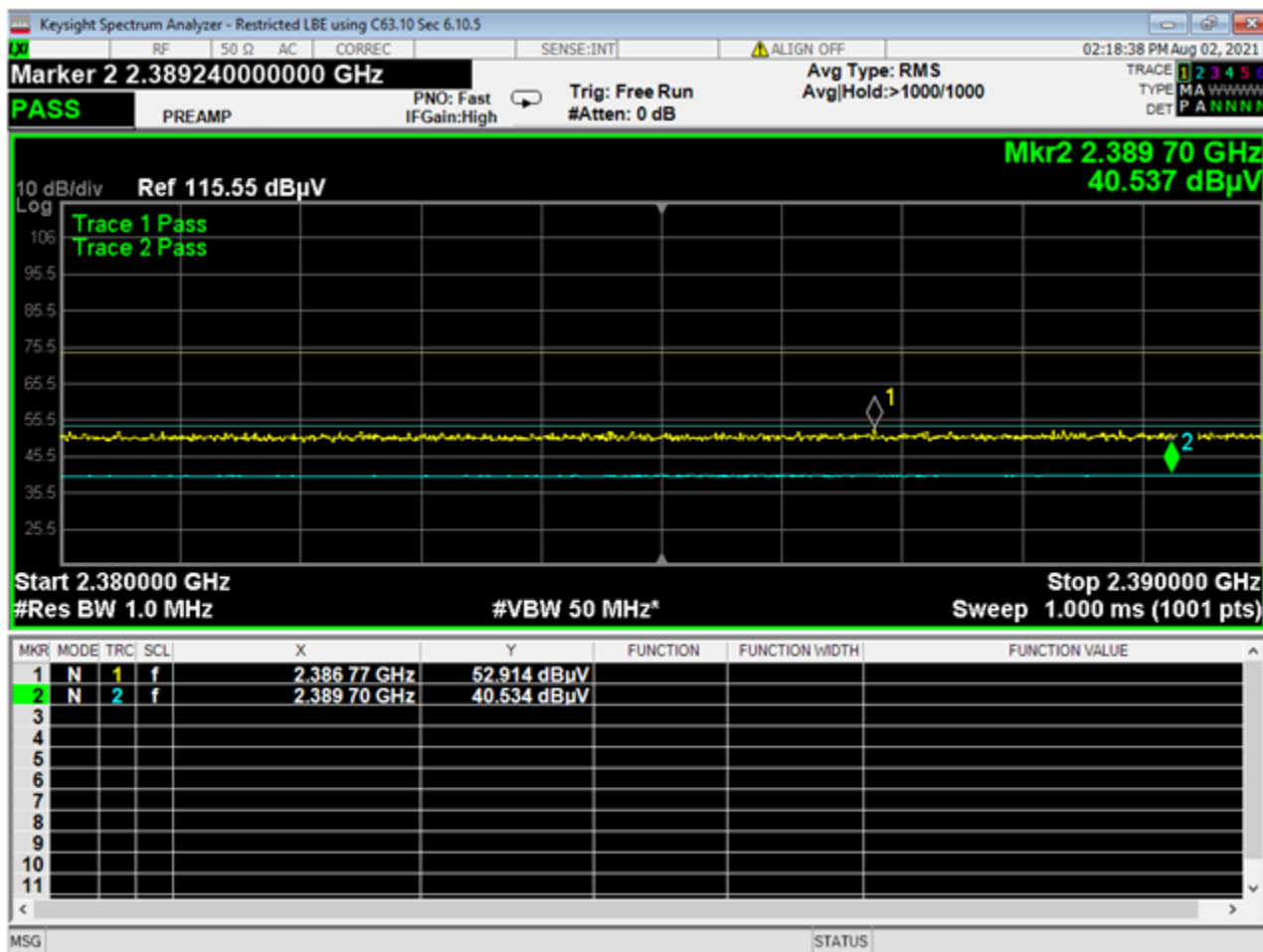
23 Lower Bandedge Restricted, 3EDR
