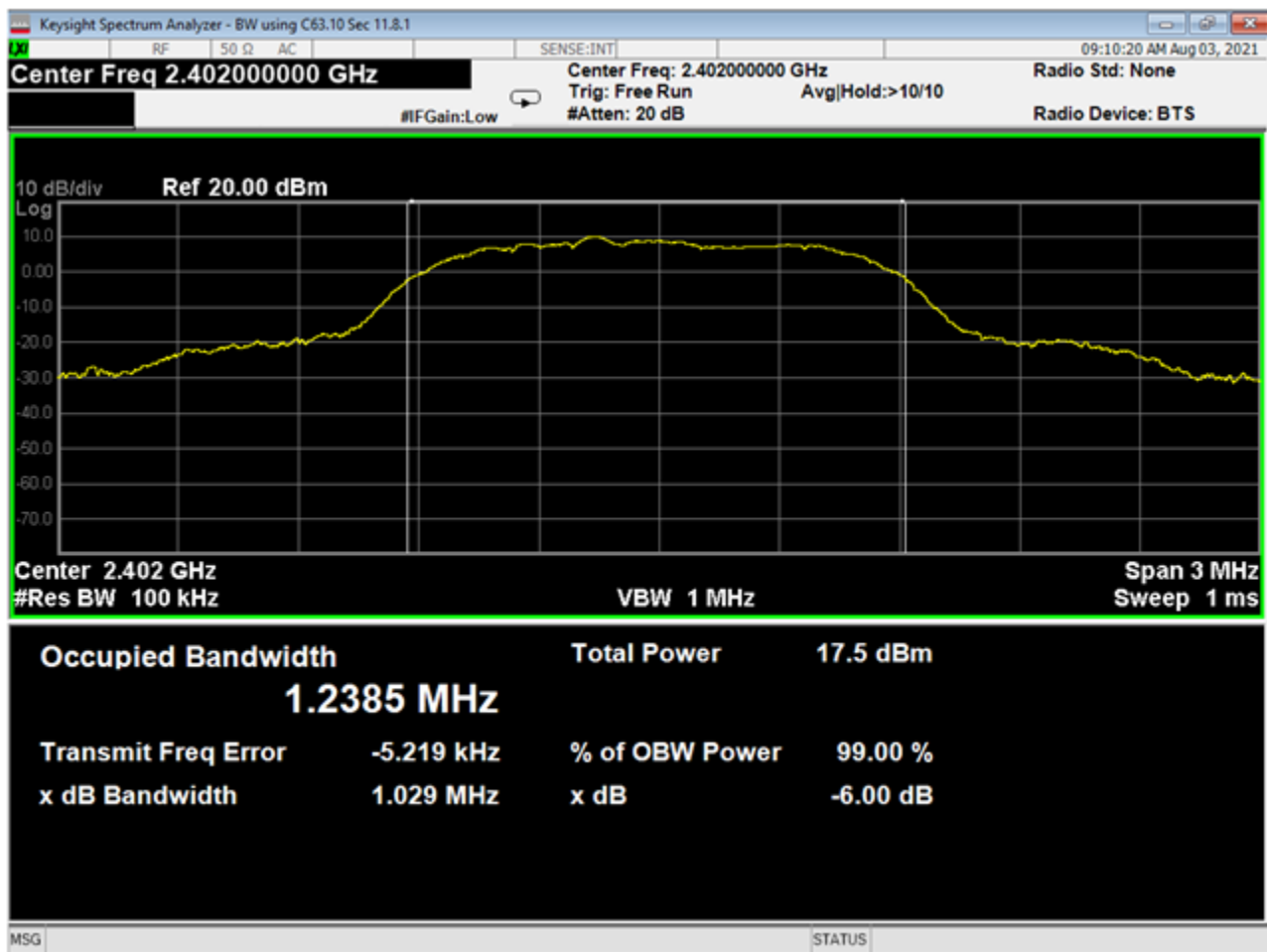
17 Bandwidth, Low Channel, 3EDR
