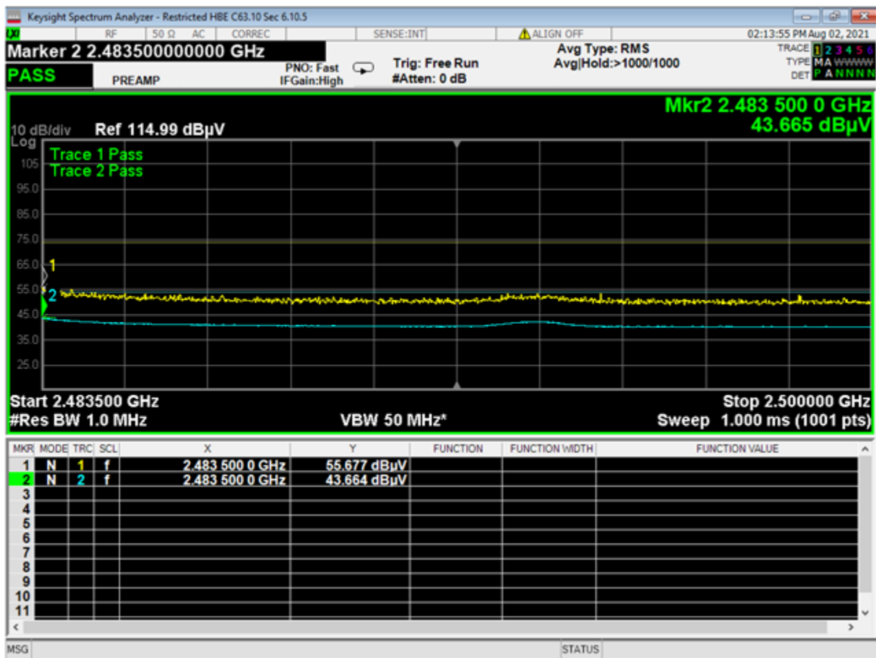
11 Higher Bandedge Restricted, 2EDR
