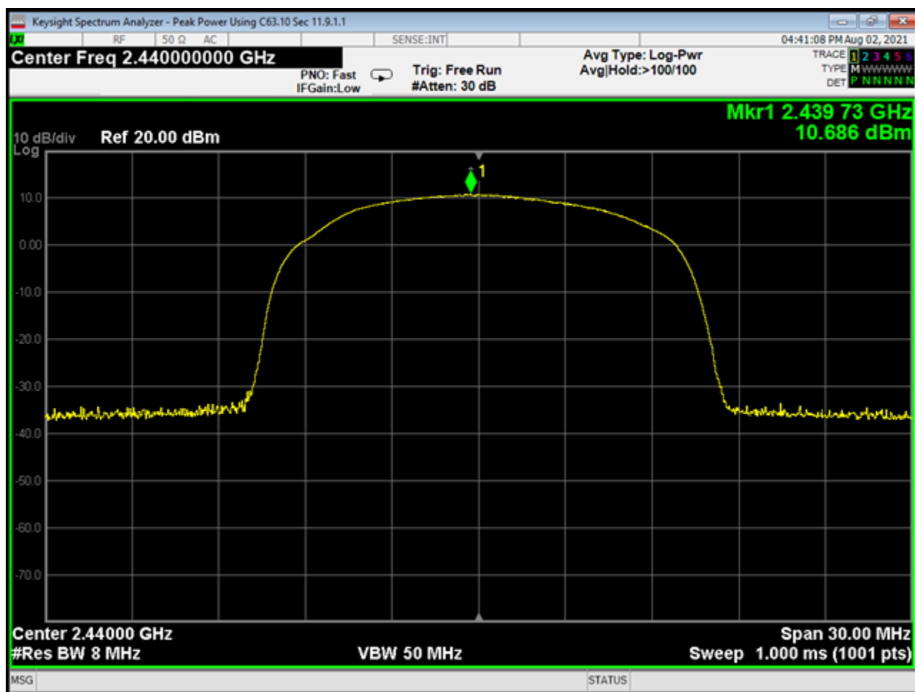
02 Peak Output Power, Mid Channel, BTBR
