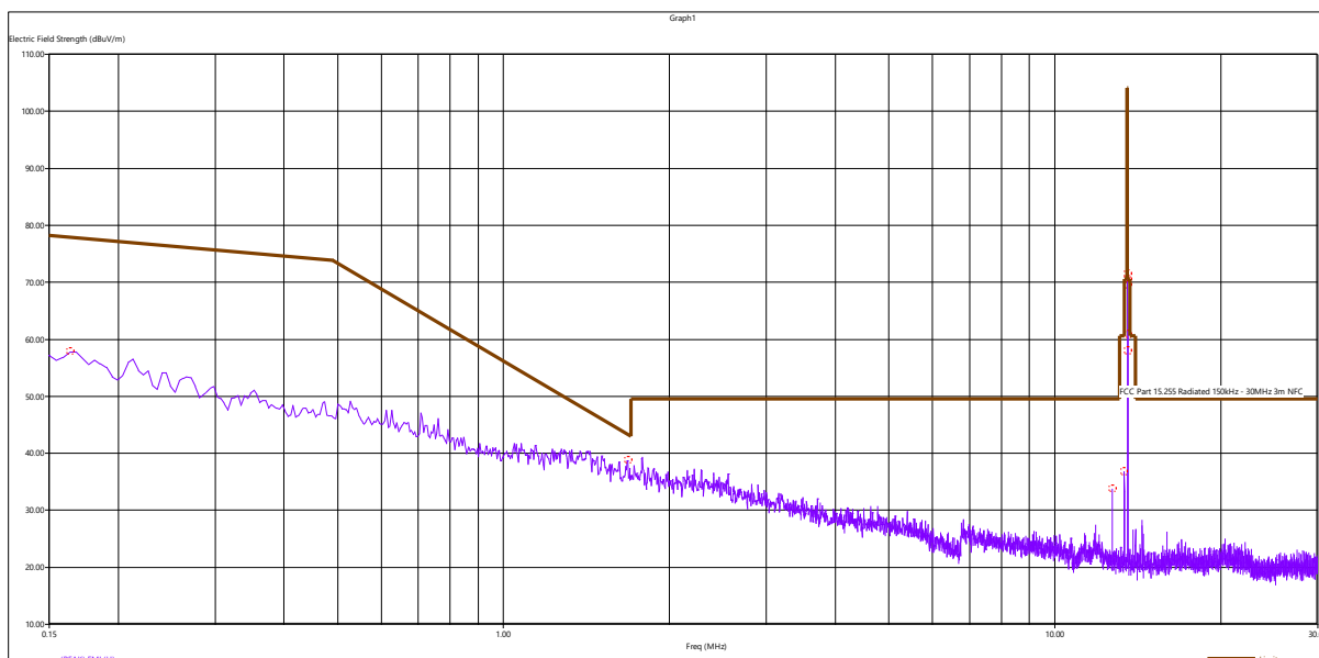
Figure 1 – NFC Radiated Emissions Plot, 150kHz – 30MHz
