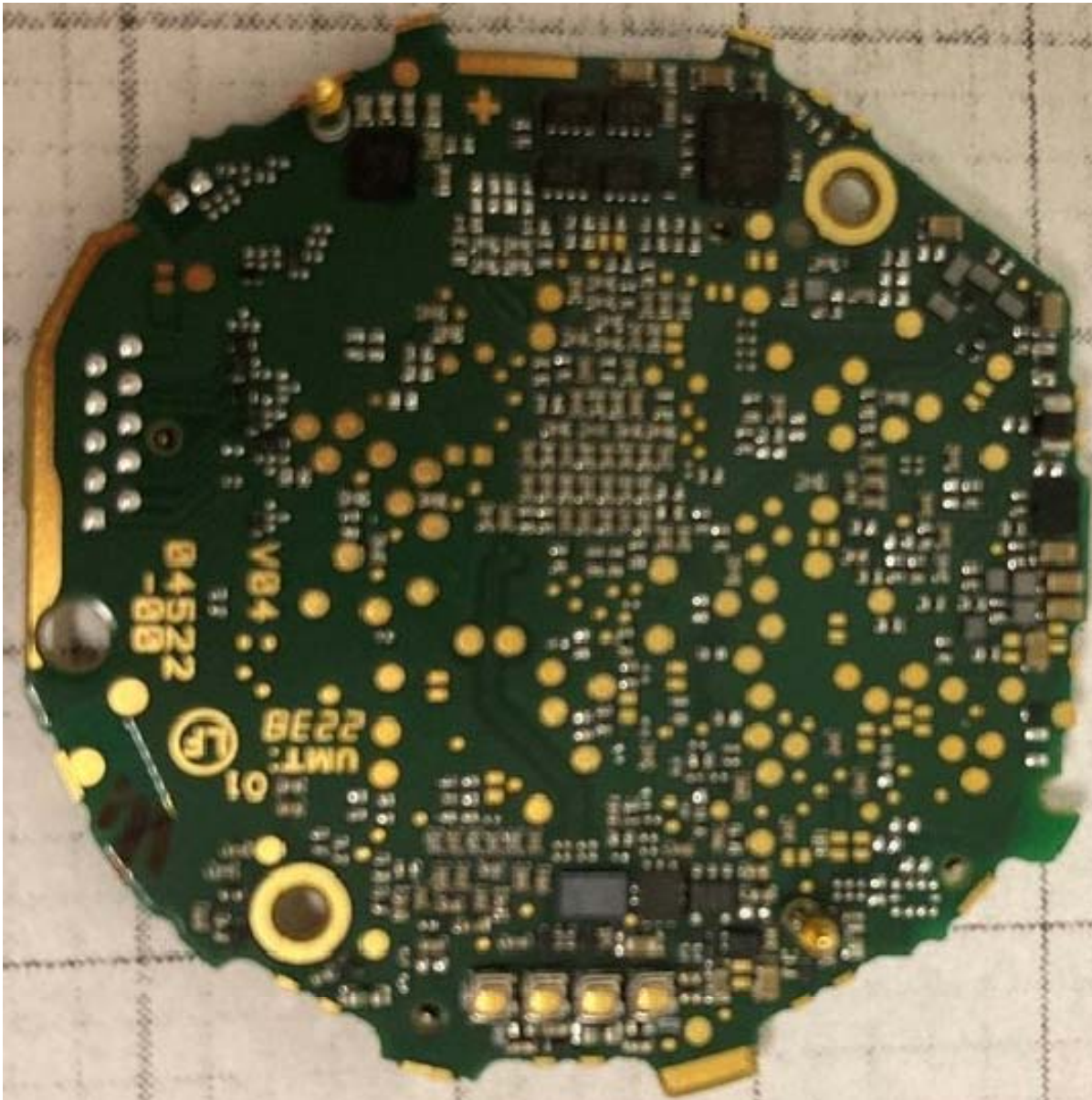
Figure E15.5 – Internal, PCB Bottom Side, Shield Removed
