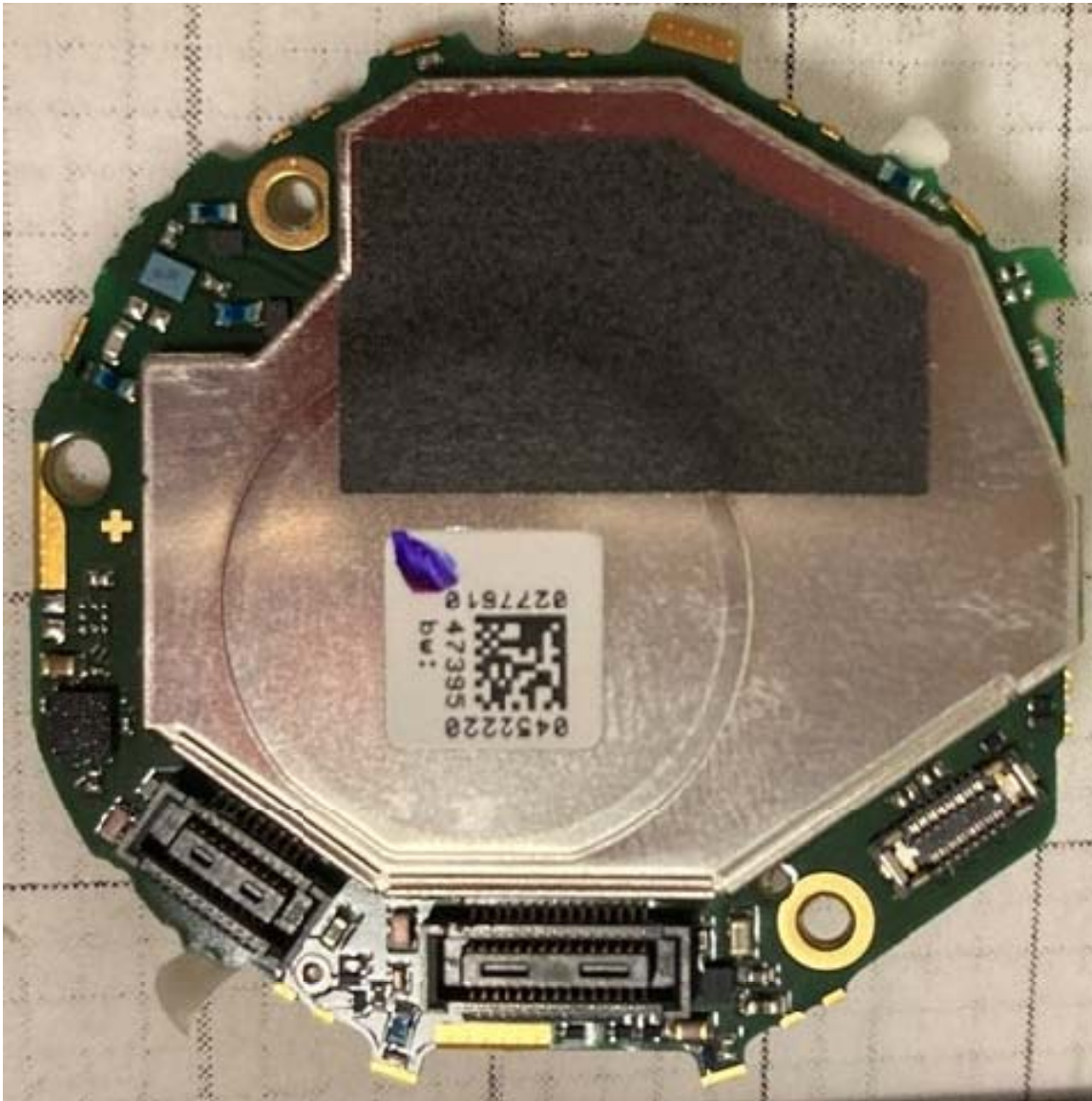
Figure E15.4 – Internal, PCB Top Side
