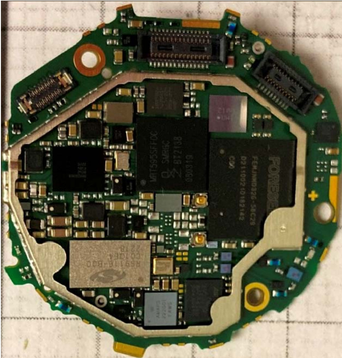
Figure E15.6 – Internal, PCB Top Side, Shield Removed
