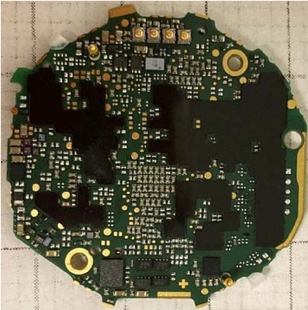
Figure E15.3 – Internal, PCB Bottom Side
