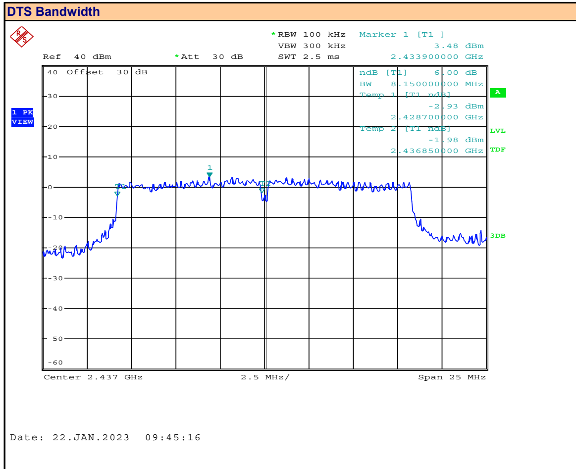
Plot 8.2 – 6dB DTS Bandwidth 802.11g
