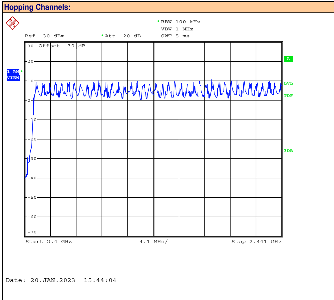
Plot 12.3 – Number of Hopping Channels, BT 2EDR
