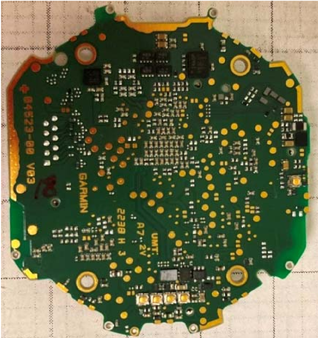
Figure E15.5 – Internal, PCB Bottom Side, Shield Removed
