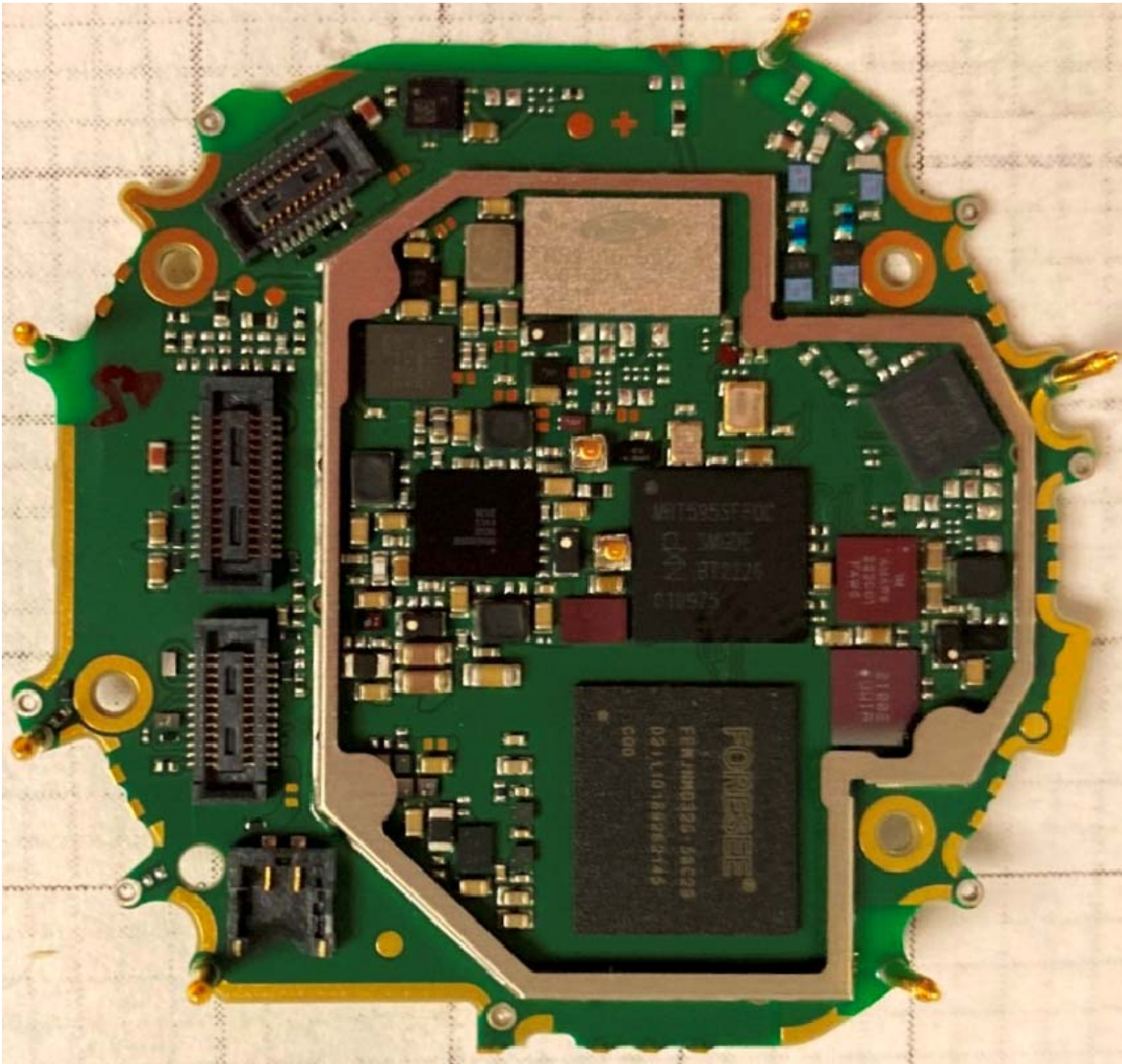
Figure E15.6 – Internal, PCB Top Side, Shield Removed
