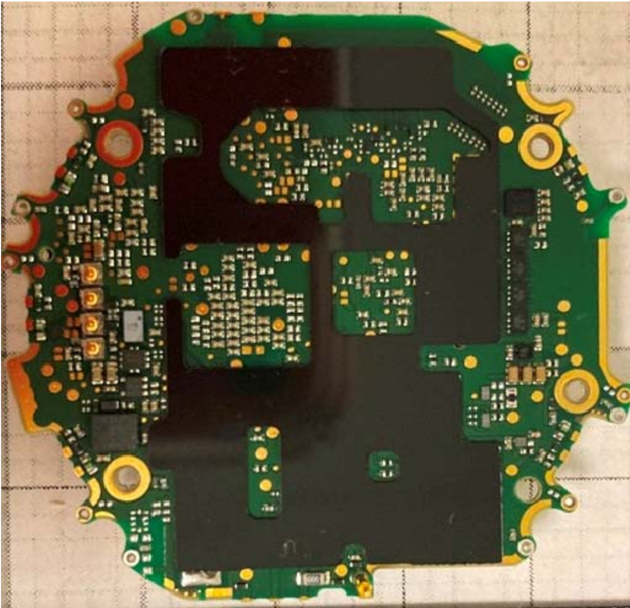
Figure E15.3 – Internal, PCB Bottom Side
