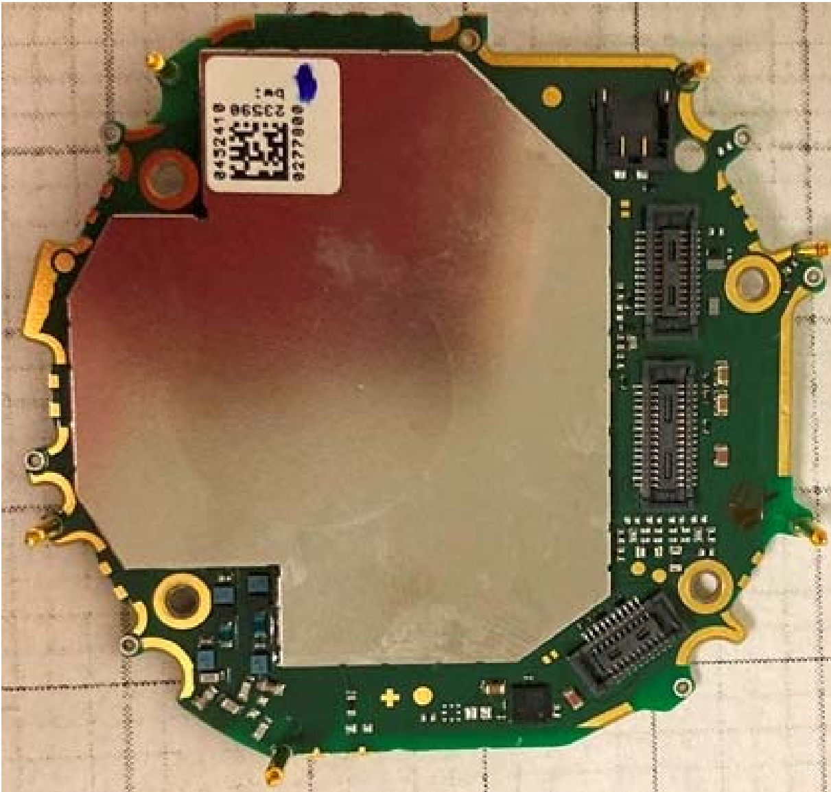
Figure E15.4 – Internal, PCB Top Side
