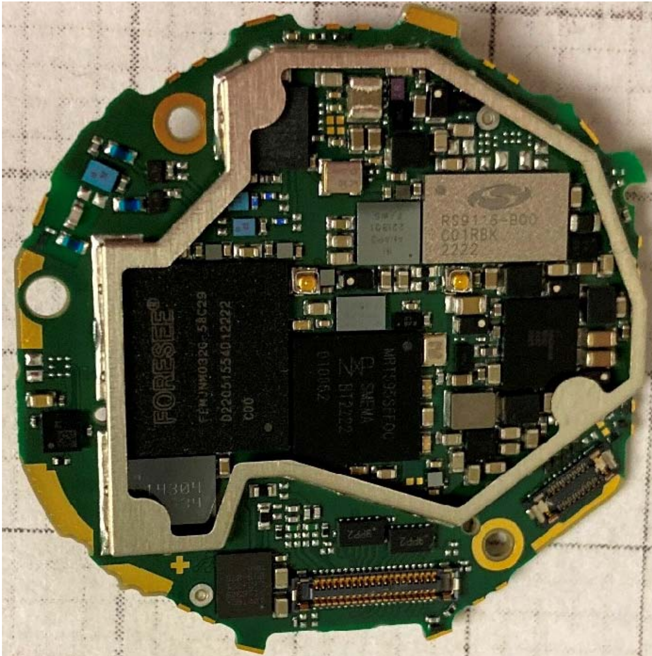
Figure E15.5 – Internal, PCB Top Side, Shield Removed
