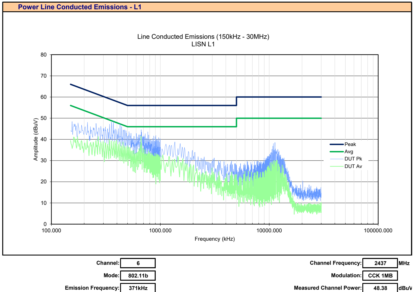
Plot 14.1 – Power Line Conducted Emissions, Line 1
