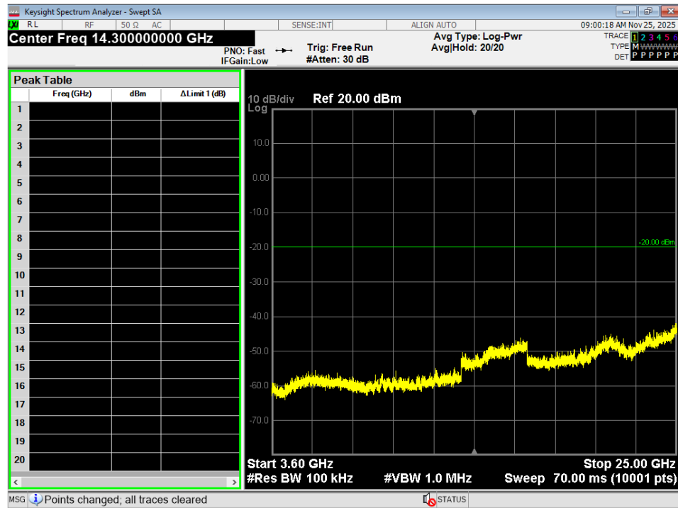
Figure 9 - Conducted Spurious Plot, 3.6GHz – 25GHz, RX
