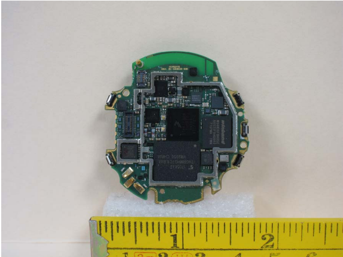
PCB Front – Shield Off
