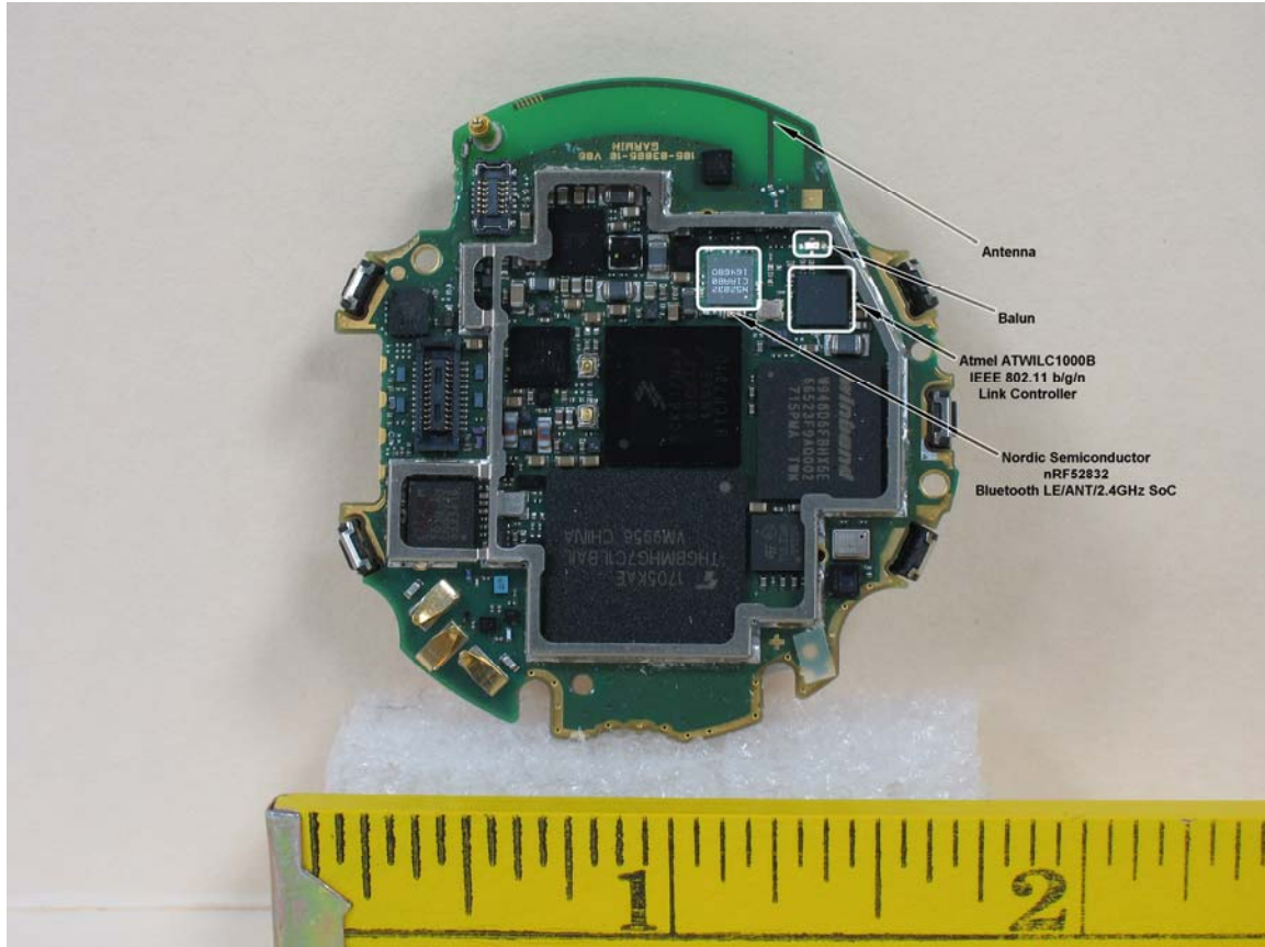
PCB Front – Labeled
