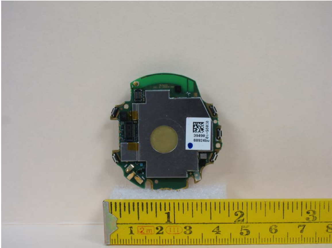
PCB Front – Shield On
