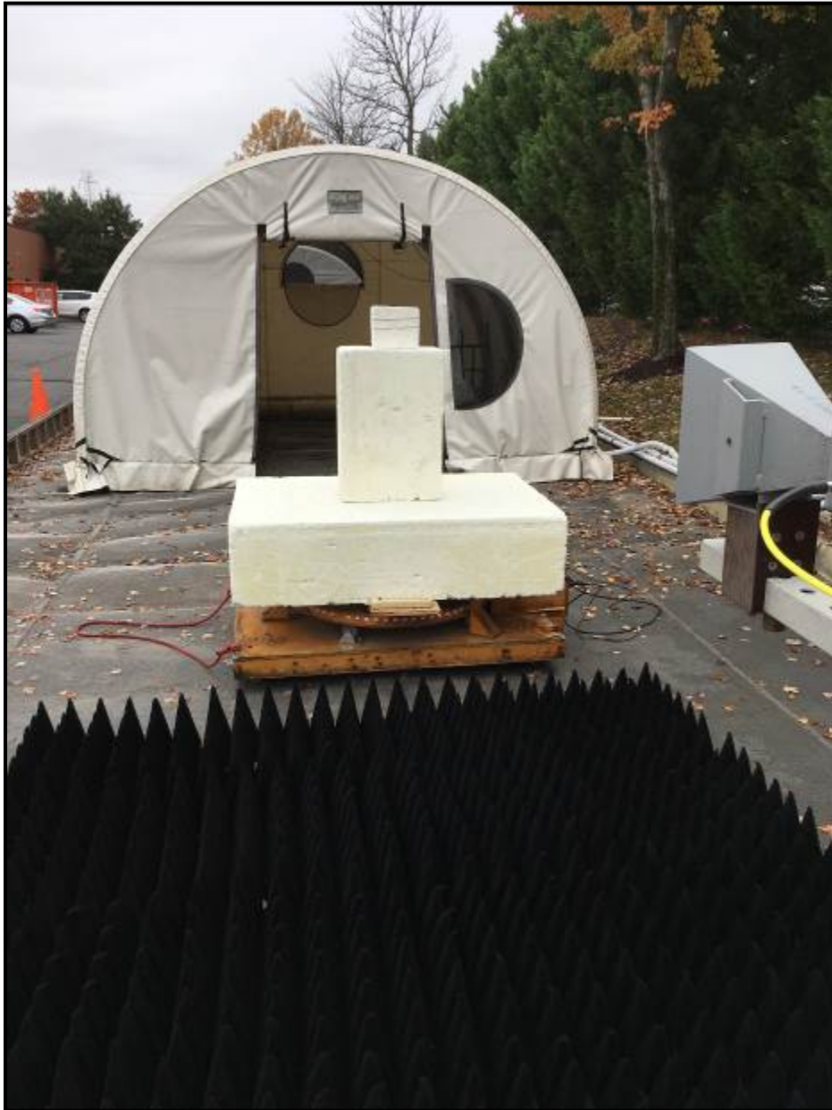
Photograph 2: Radiated Emissions Testing – Back View (Spurious Emissions, >1 GHz)
