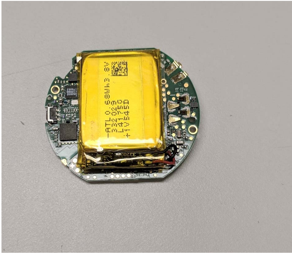
Bottom side of PCB [battery attached]
