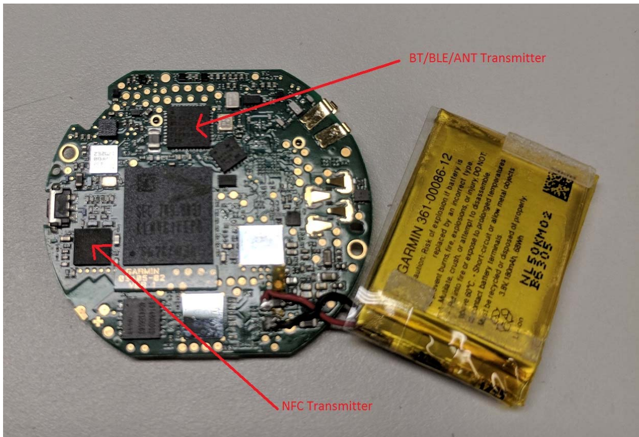
Bottom side of PCB [battery removed]
