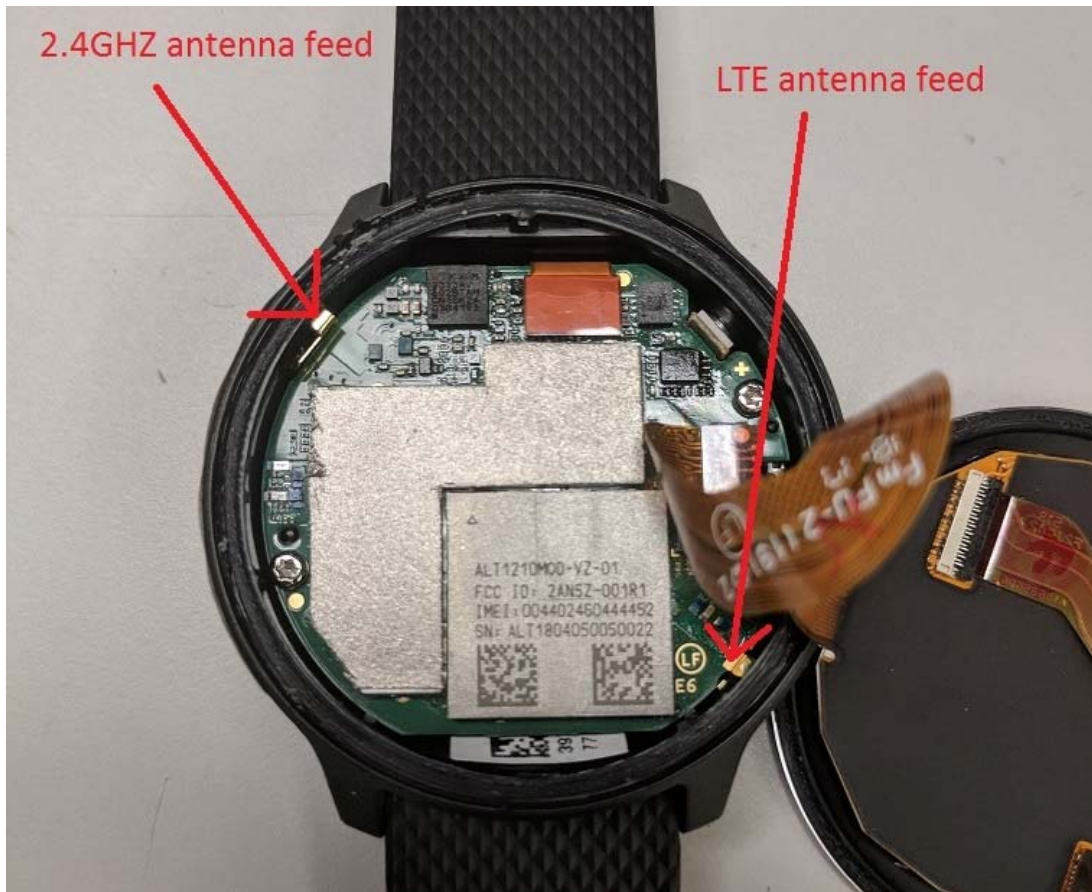
Top side of PCB in watch case
