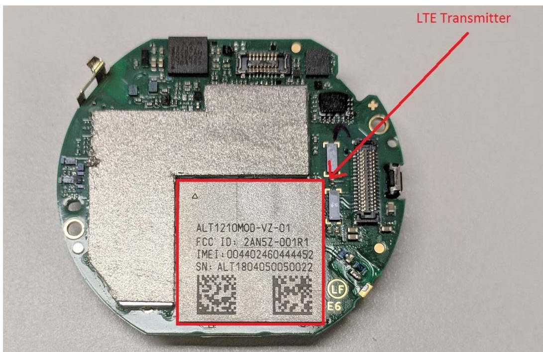
Top side of PCB extracted from watch
