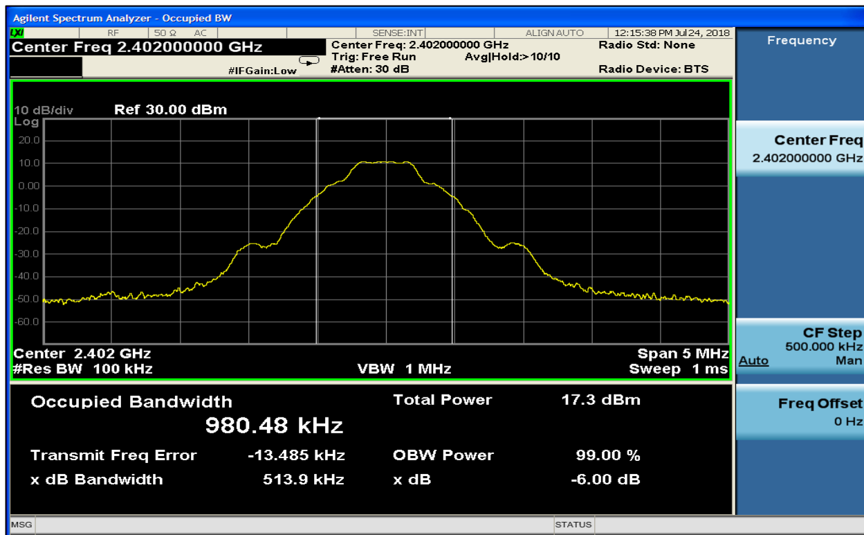
Plot 5-1: 6 dB BW – ANT+ – 2402 MHz
