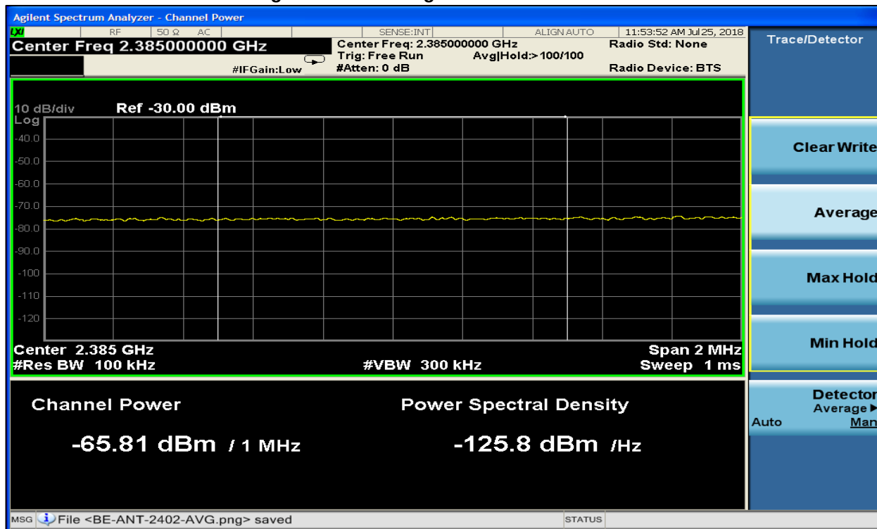
Plot 8-3: Lower Band Edge – BLE – Average
