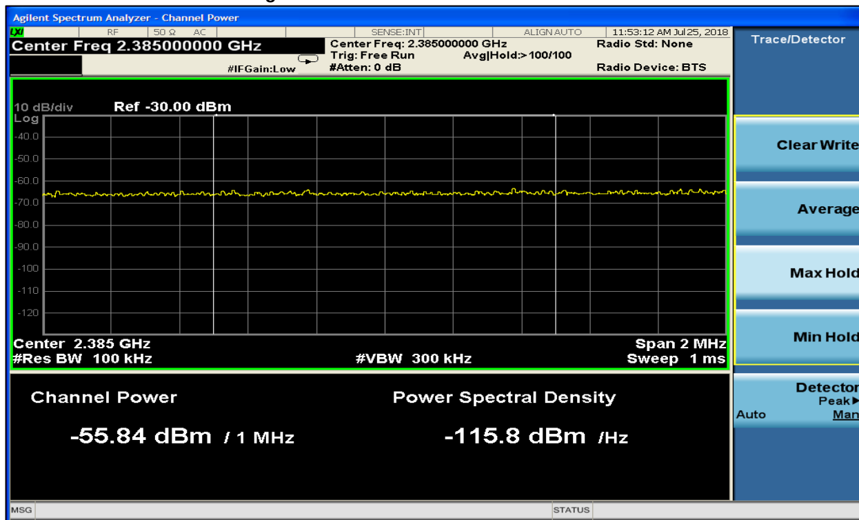
Plot 8-2: Lower Band Edge – ANT+ – Peak
