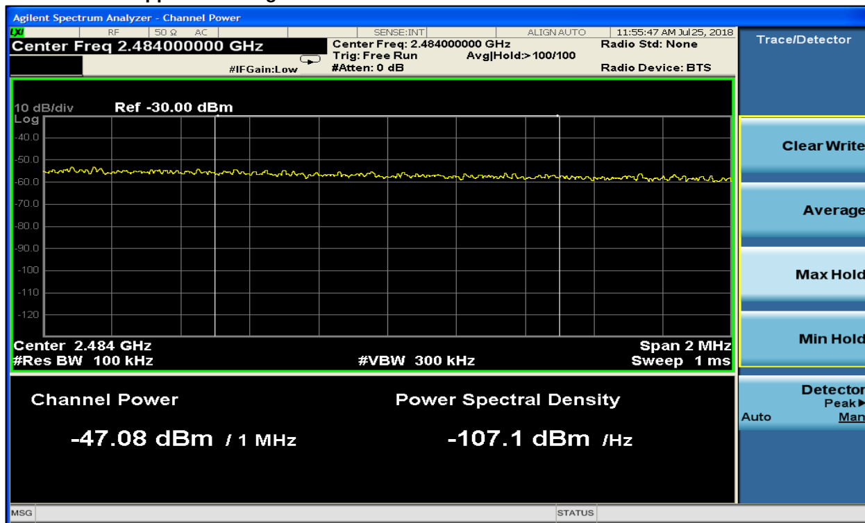
Plot 8-6: Upper Band Edge – ANT+ – Peak
