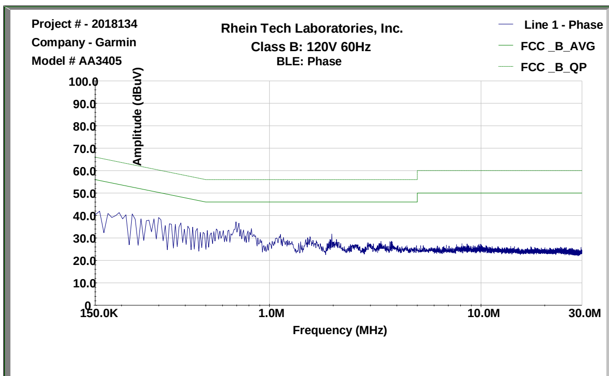
Plot 3-4: Conducted Emissions – BLE – Phase
