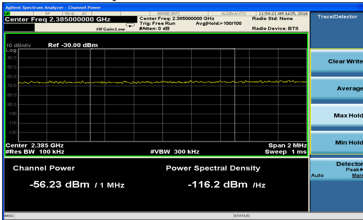
Plot 8-4: Lower Band Edge – BLE – Peak
