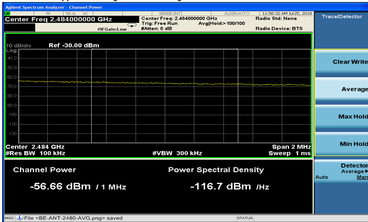
Plot 8-7: Upper Band Edge – BLE – Average
