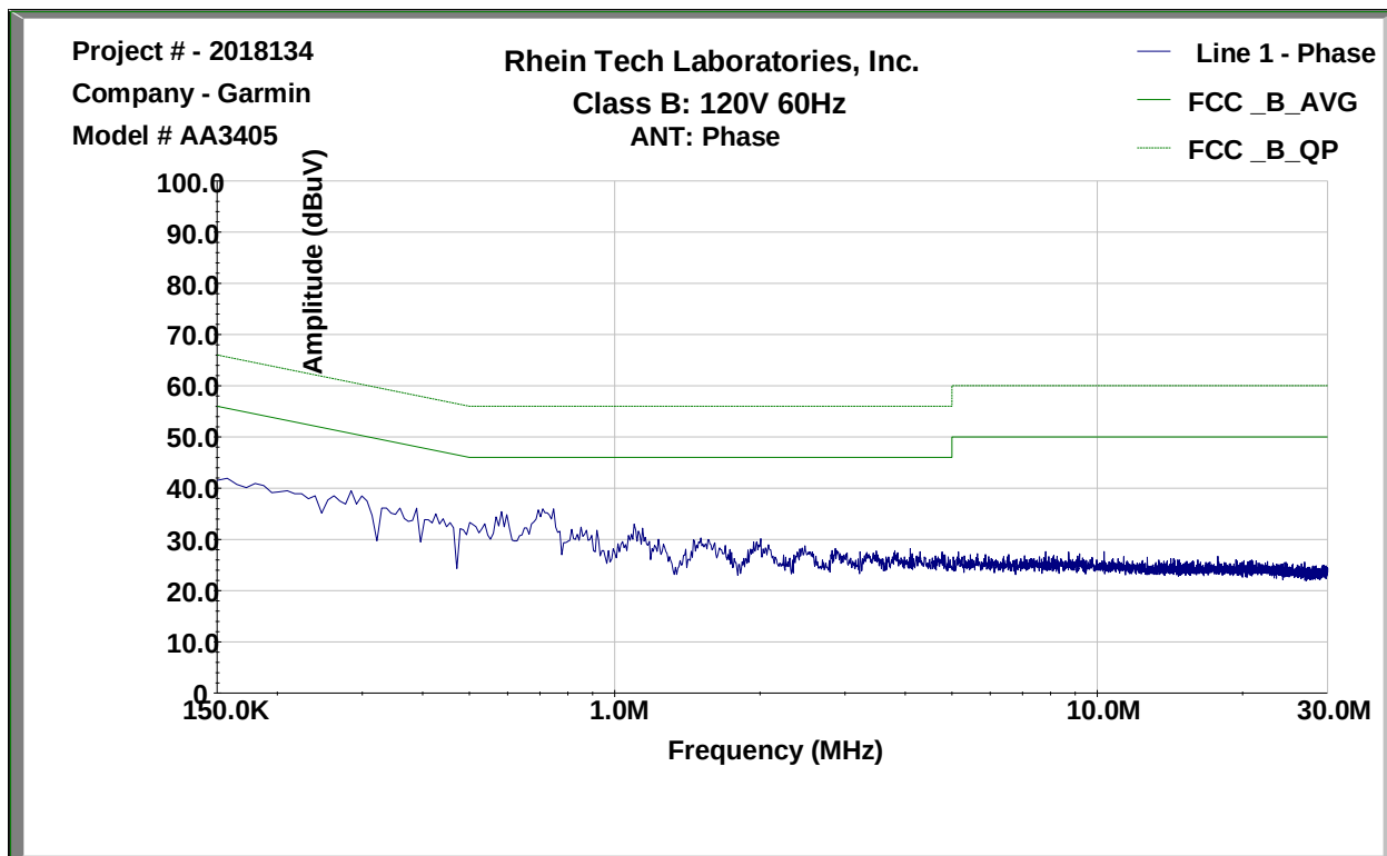
Plot 3-2: Conducted Emissions – ANT+ – Phase
