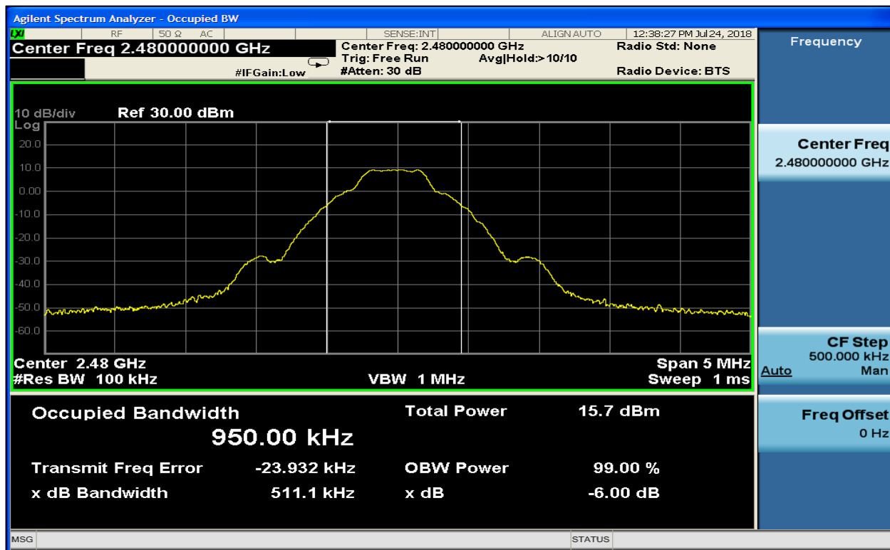
Plot 5-3: 6 dB BW – ANT+ – 2480 MHz
