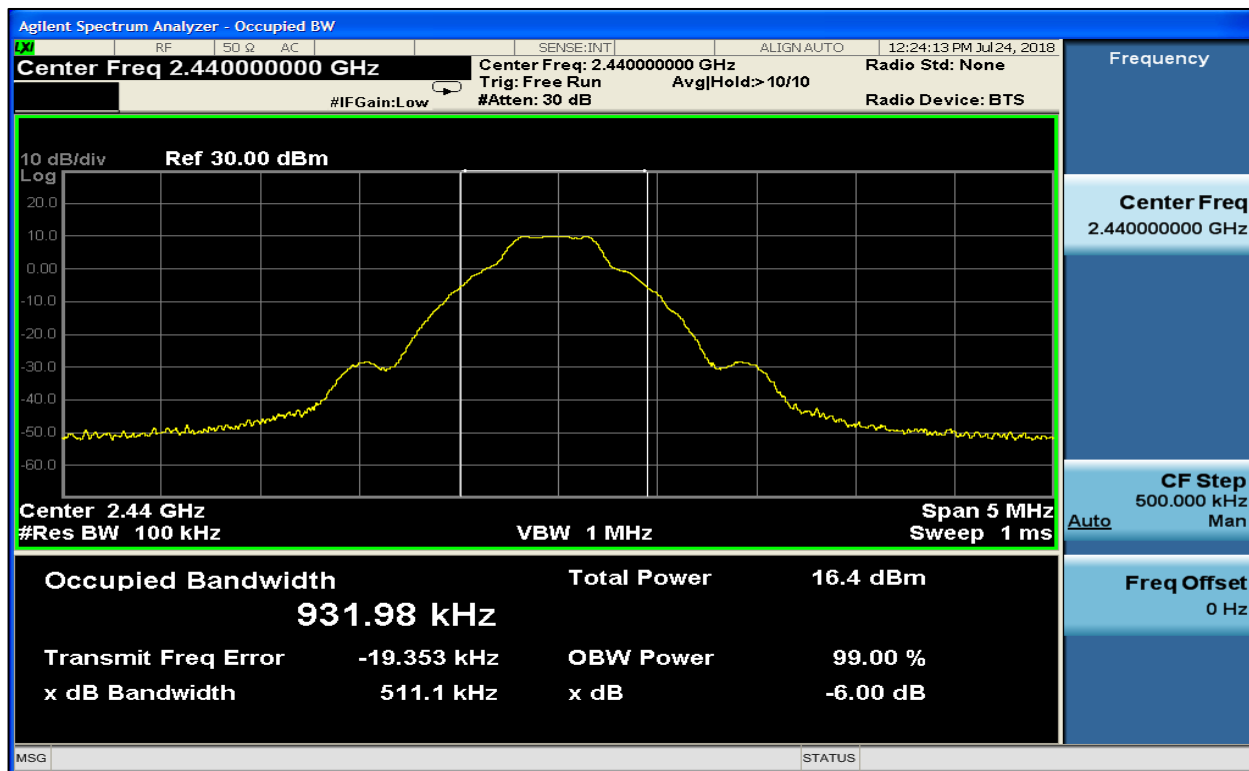
Plot 5-2: 6 dB BW – ANT+ – 2440 MHz
