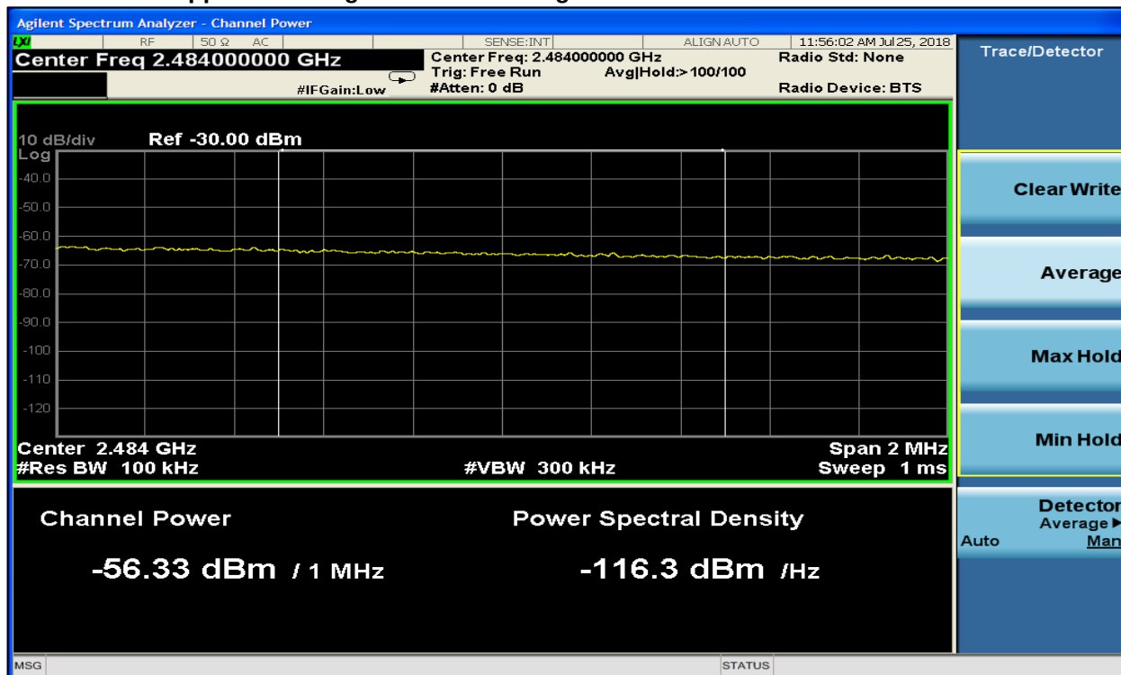
Plot 8-5: Upper Band Edge – ANT+ – Average
