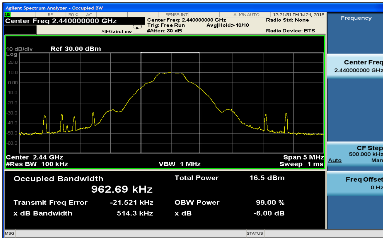
Plot 5-5: 6 dB BW – BLE – 2440 MHz
