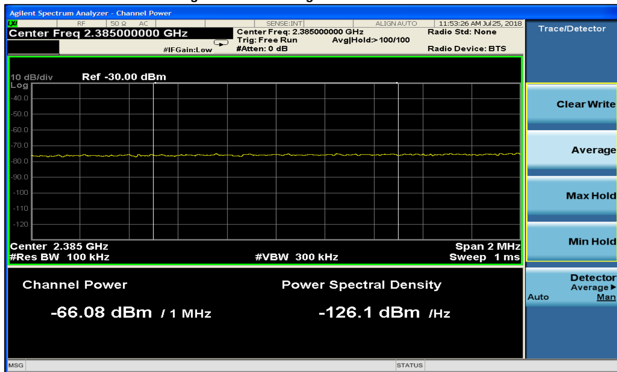
Plot 8-1: Lower Band Edge – ANT+ – Average
