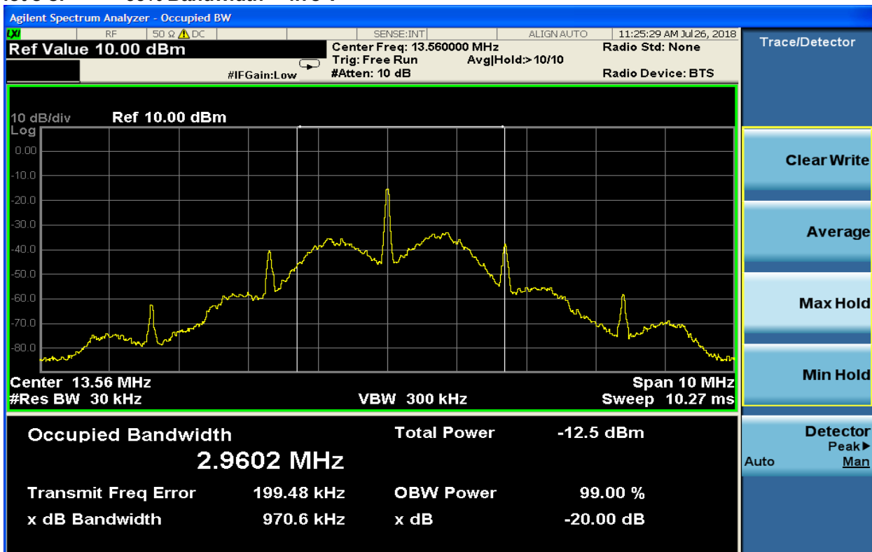
Plot 5-3: 99% Bandwidth – 4.75 V
