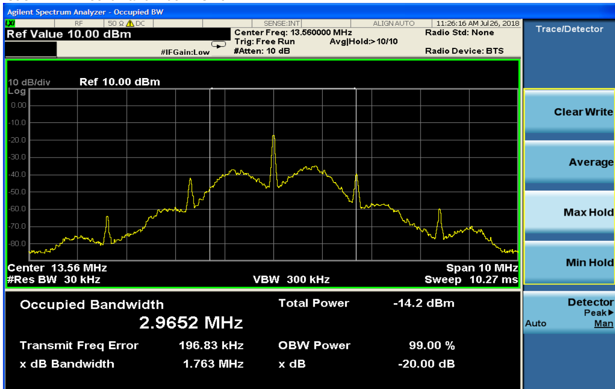
Plot 5-1: 99% Bandwidth – 3.20 V
