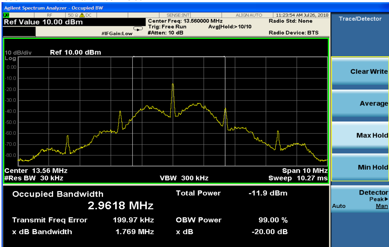
Plot 5-2: 99% Bandwidth – 3.90 V
