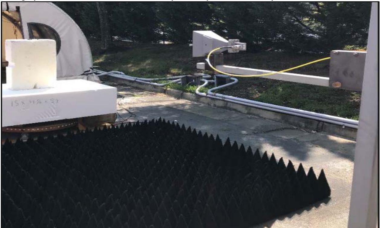
Photograph 4: Radiated Emissions Test Setup – Rear (Above 1000 MHz)
