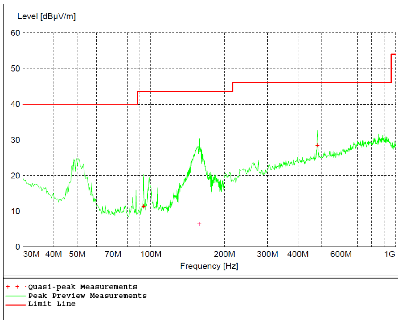
Figure 21 - Radiated Emissions Plot, Mid Channel, GMSK
