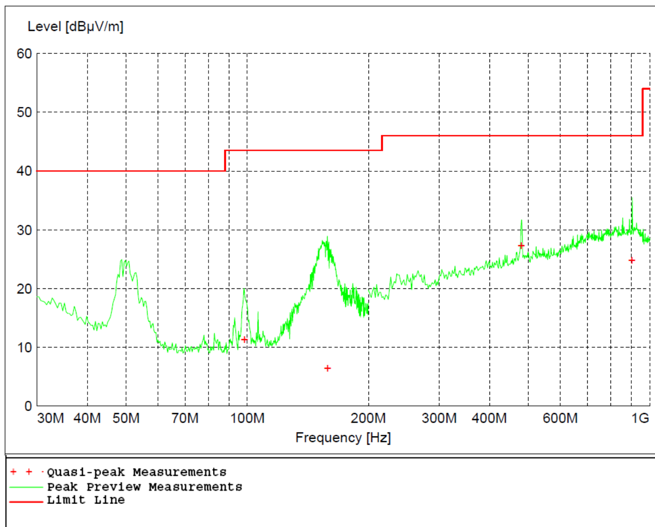
Figure 19 - Radiated Emissions Plot, High Channel, GFSK
