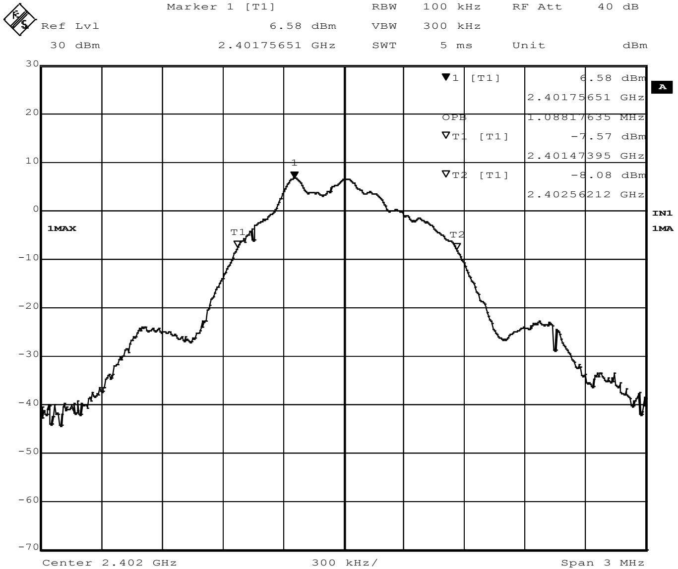
Figure 8 – Occupied Bandwidth, Low Channel, GMSK
