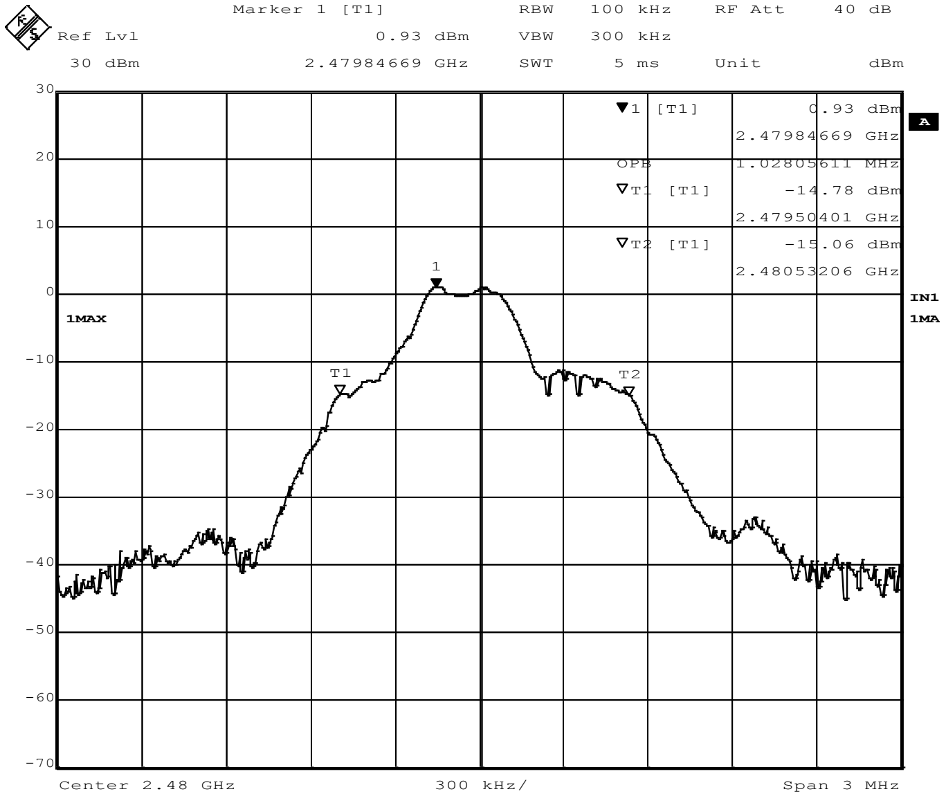
Figure 13 - Occupied Bandwidth, High Channel, GFSK
