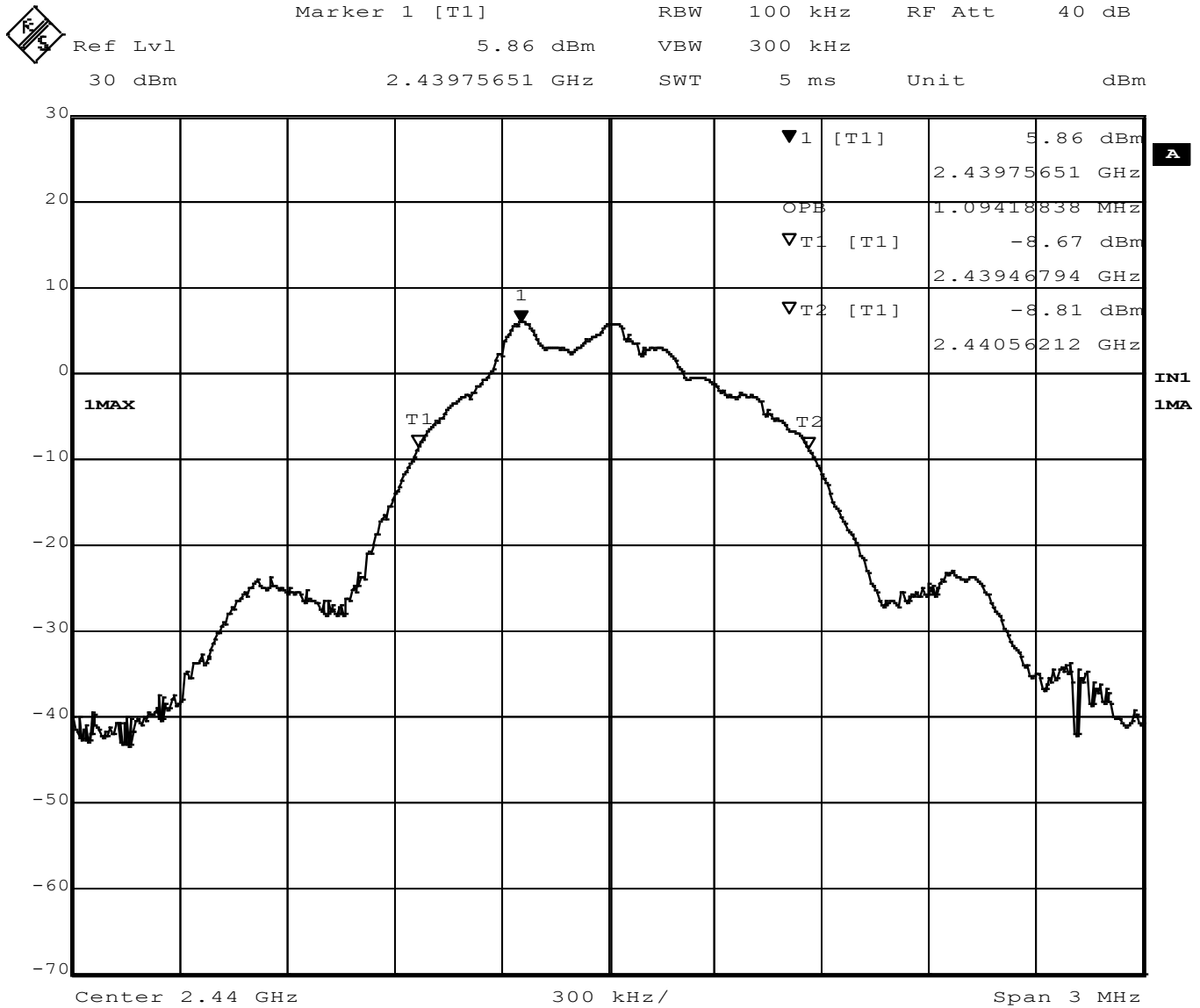
Figure 9 - Occupied Bandwidth, Mid Channel, GMSK
