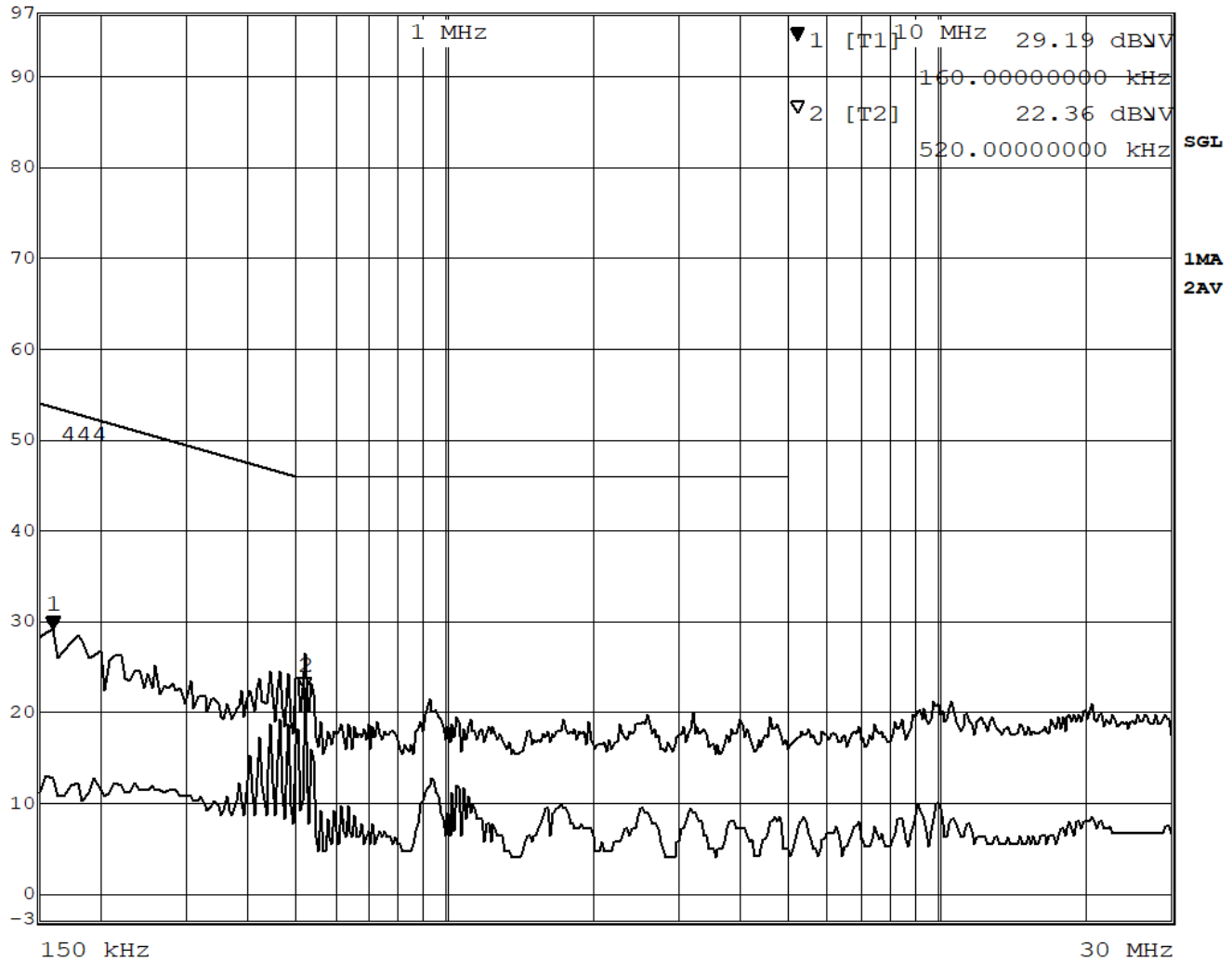
Figure 28 - Conducted Emissions Plot, N-F
