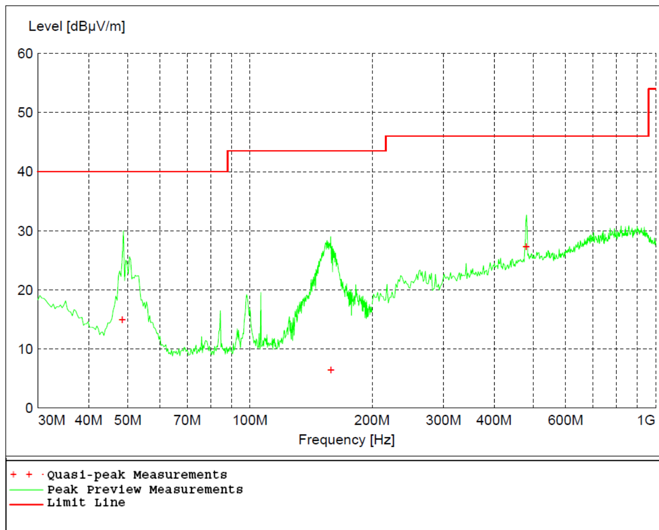
Figure 17 - Radiated Emissions Plot, Low Channel, GFSK
