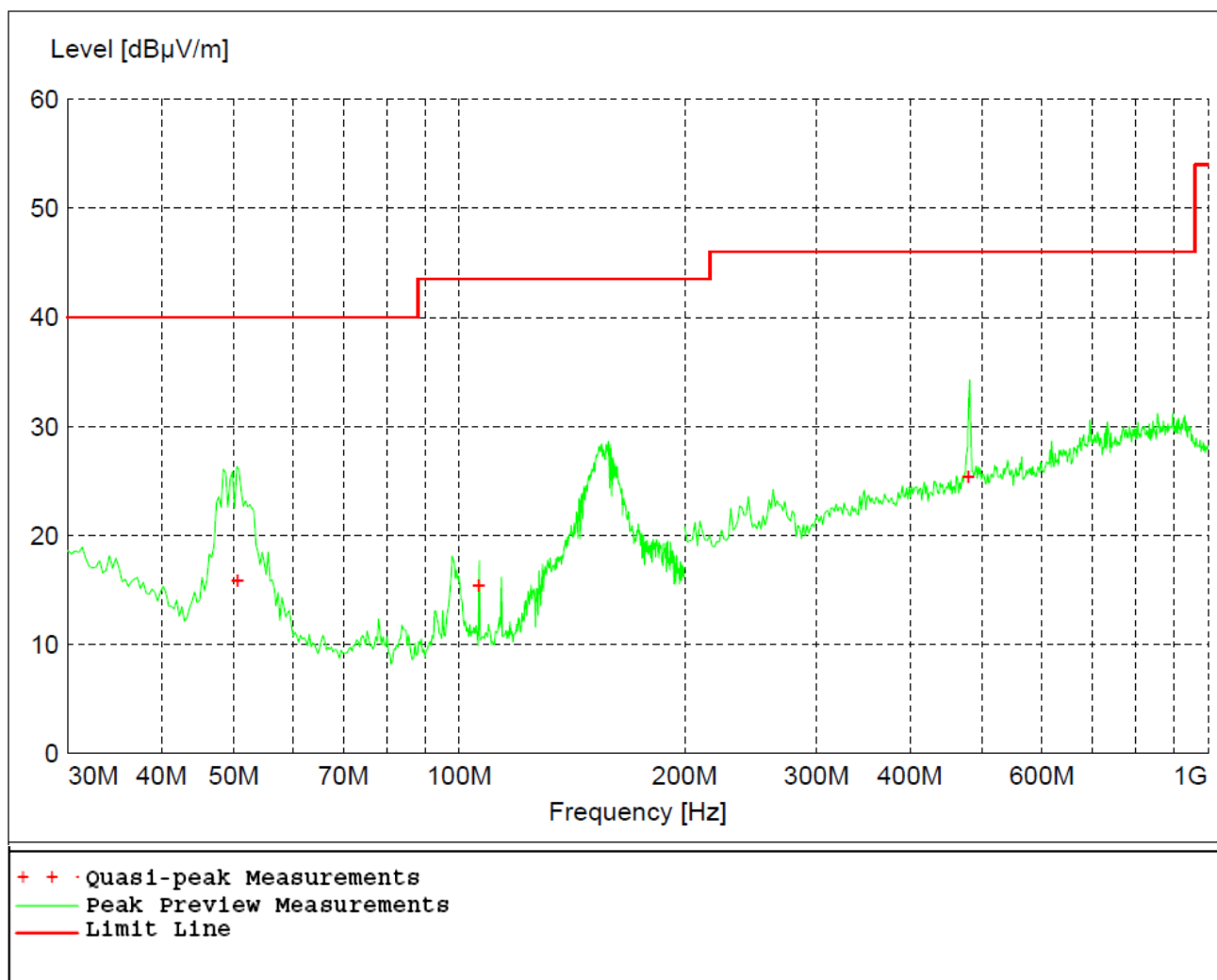
Figure 16 - Radiated Emissions Plot, Receive, GMSK
