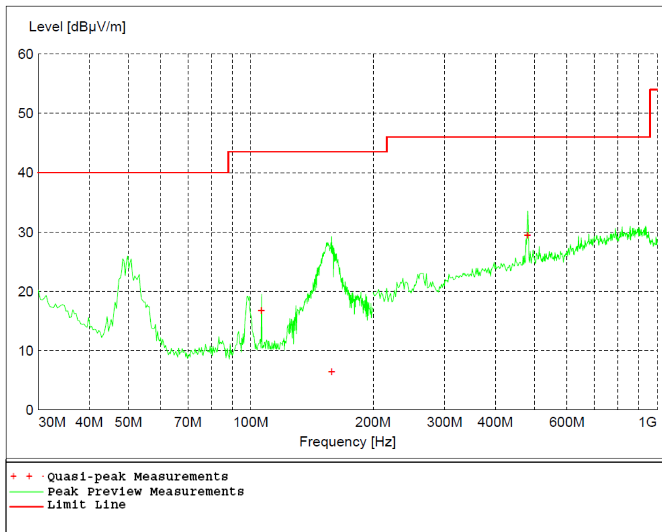
Figure 18 - Radiated Emissions Plot, Mid Channel, GFSK
