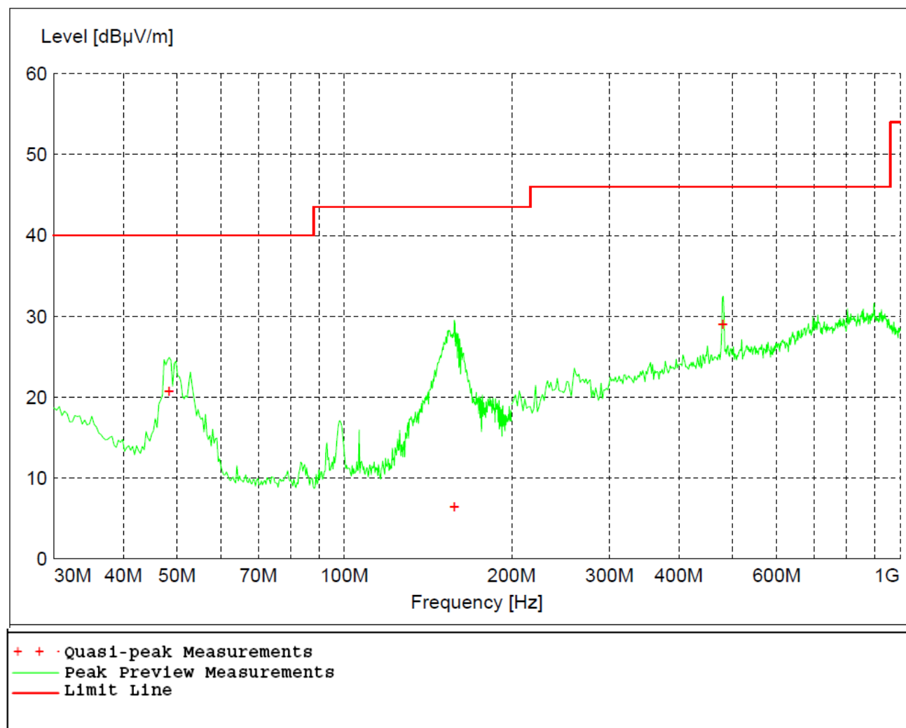
Figure 20 - Radiated Emissions Plot, Low Channel, GMSK
