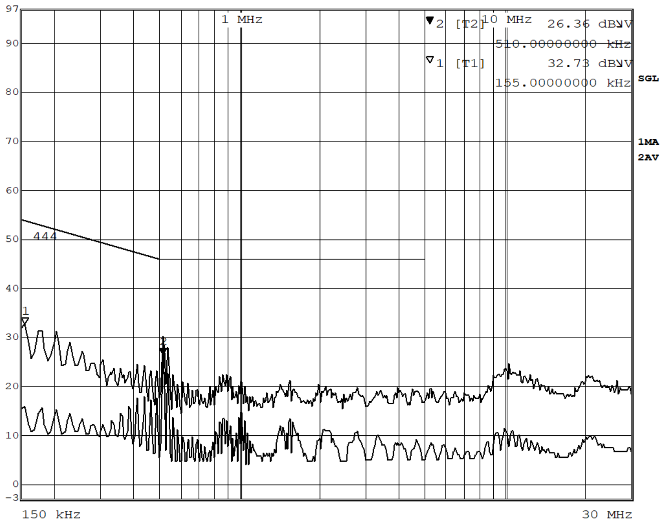
Figure 27 - Conducted Emissions Plot, L-F
