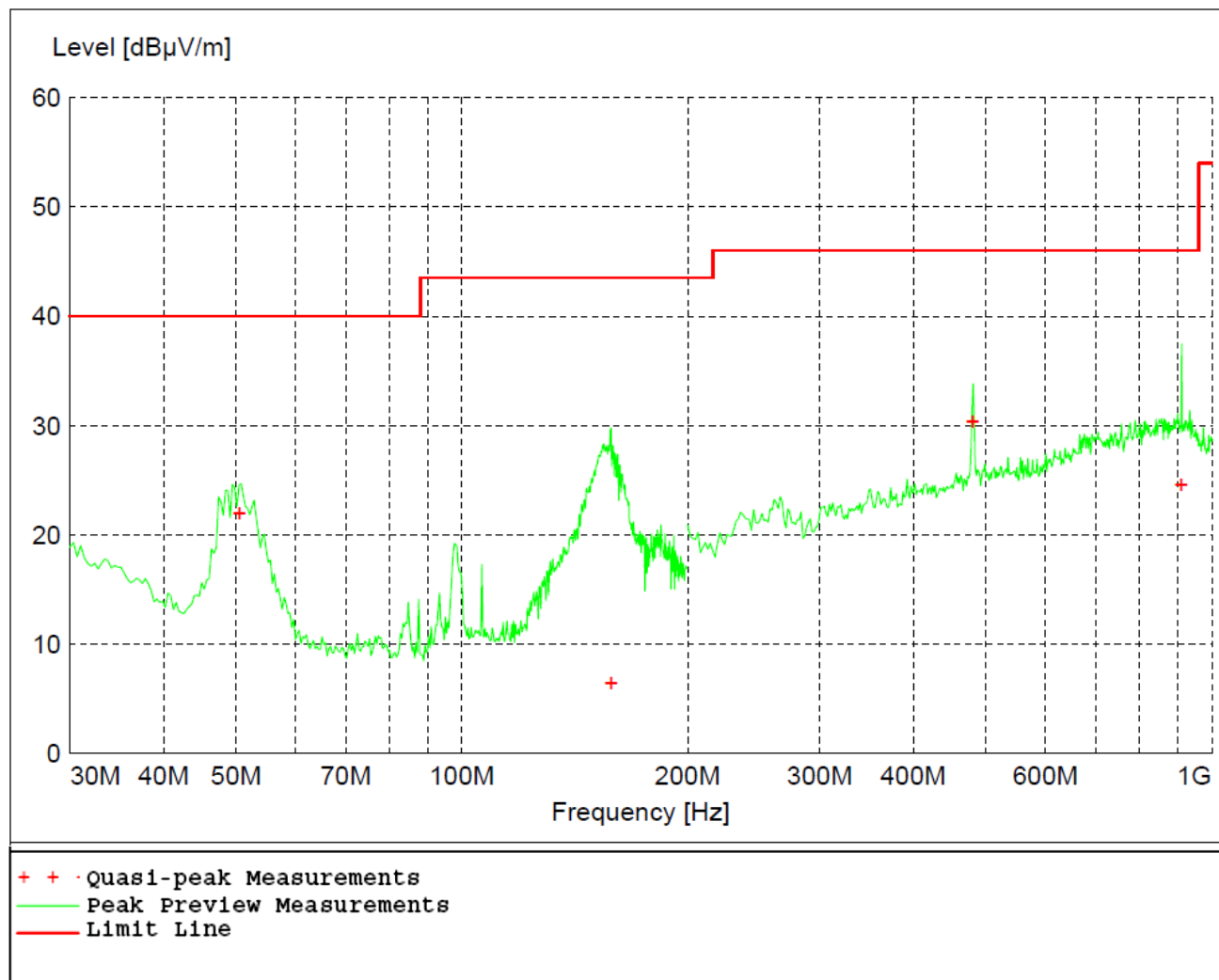
Figure 22 - Radiated Emissions Plot, High Channel, GMSK
