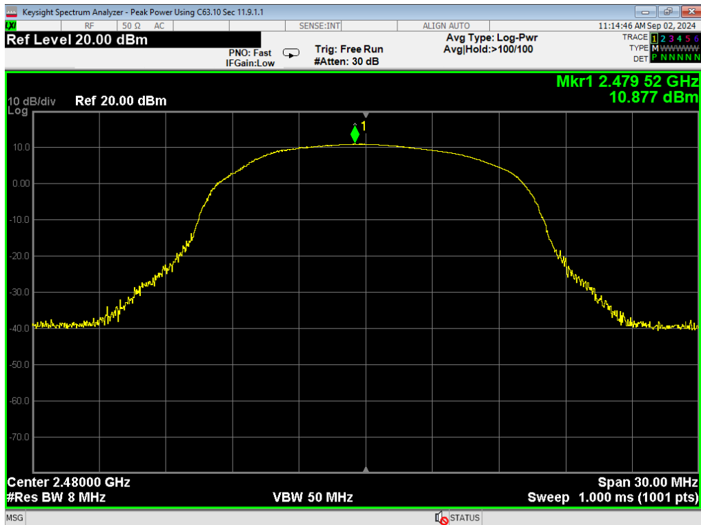
19, Peak Power, 3EDR, High
