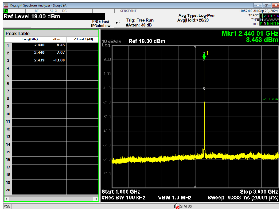
Figure 11 - Radiated Emissions Plot, 3EDR, 1GHz – 3.6GHz, Mid
