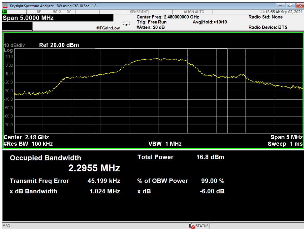
25, 6dB Bandwidth, 3EDR, High
