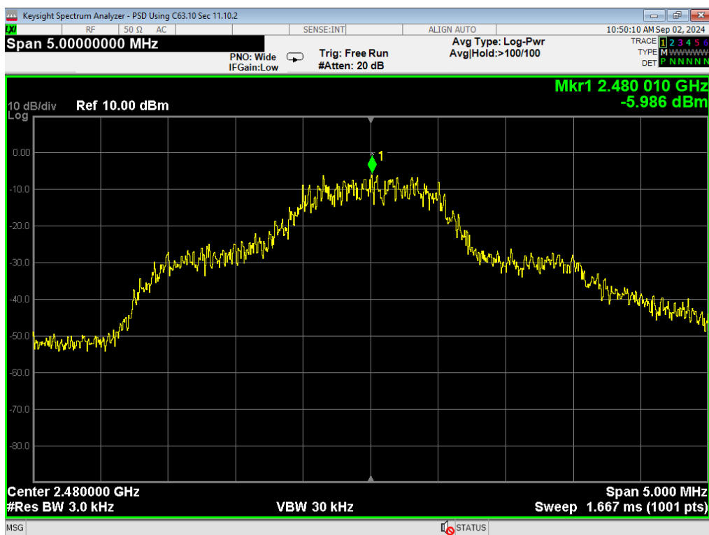
12, PSD, 2EDR, High
