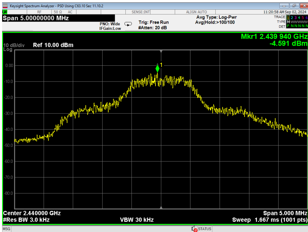
27, PSD, 3EDR, Mid
