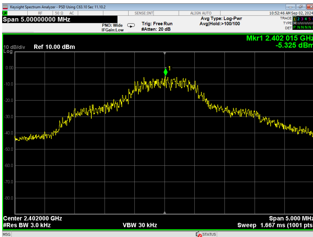
10, PSD, 2EDR, Low
