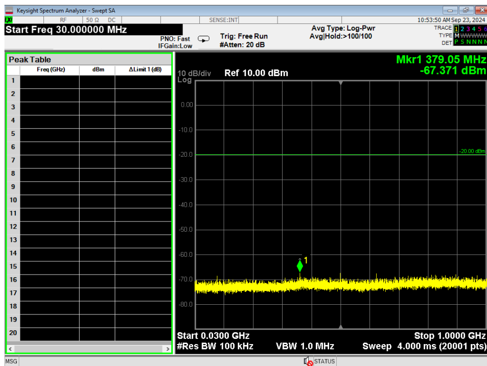
Figure 7 - Radiated Emissions Plot, 2EDR, 30MHz – 1GHz, Mid
