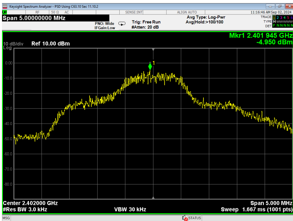
26, PSD, 3EDR, Low
