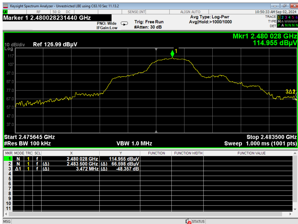
14, HBE Unrestricted, 2EDR
