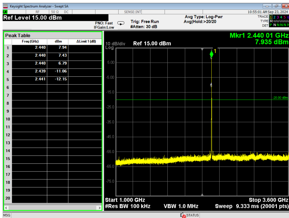
Figure 8 - Radiated Emissions Plot, 2EDR, 1GHz – 3.6GHz, Mid
