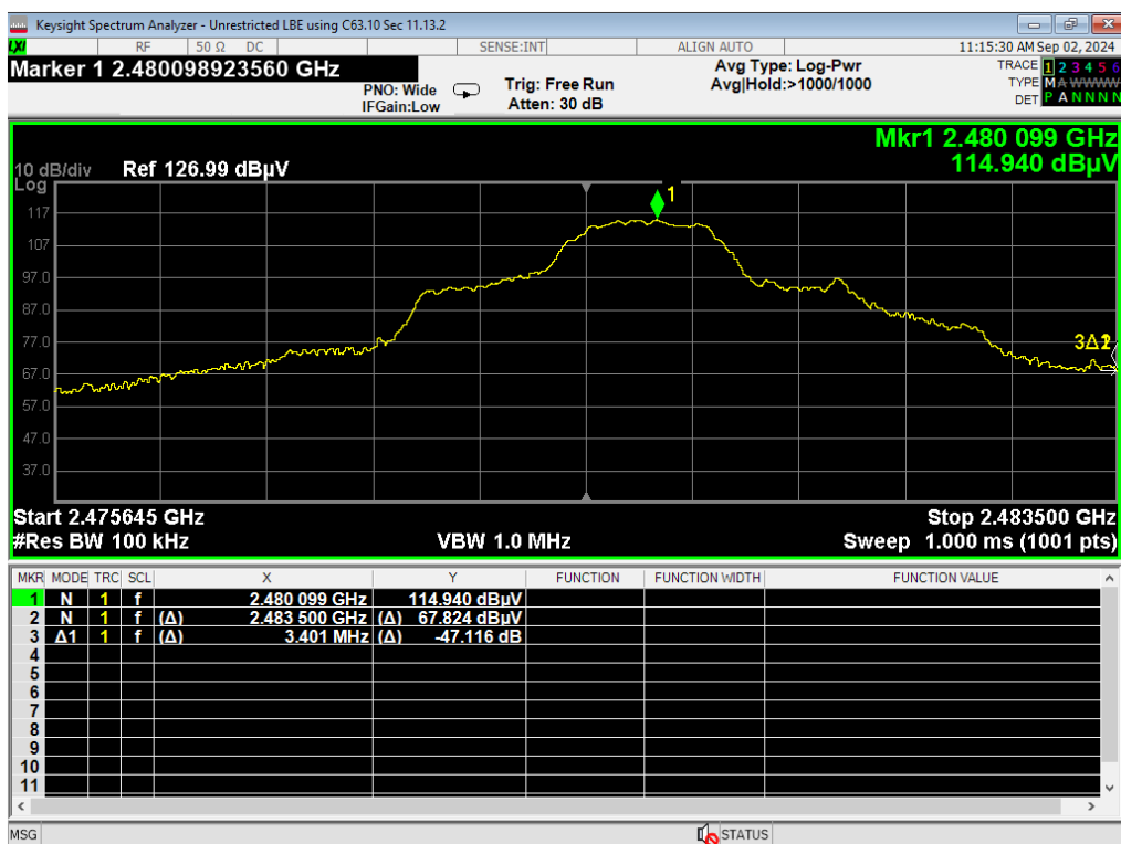
30, HBE Unrestricted, 3EDR
