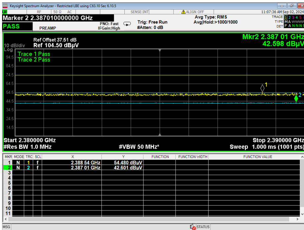
15, LBE Restricted, 2EDR
