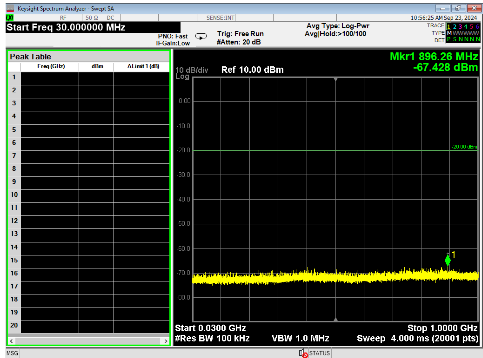
Figure 10 - Radiated Emissions Plot, 3EDR, 30MHz – 1GHz, Mid
