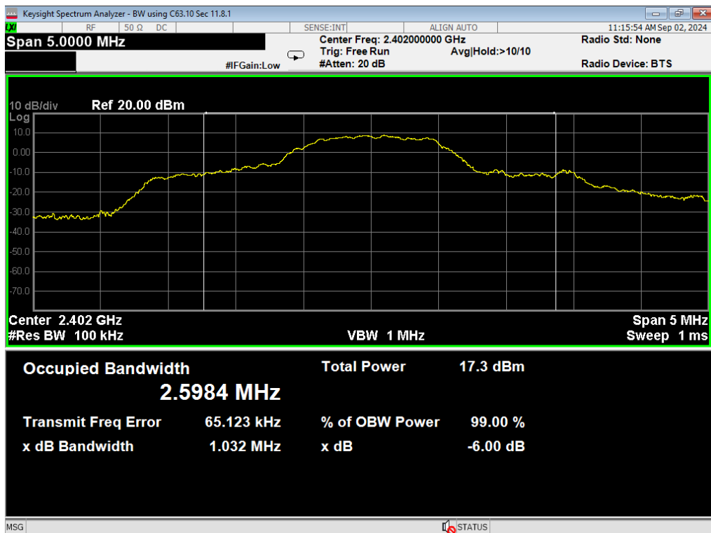
23, 6dB Bandwidth, 3EDR, Low
