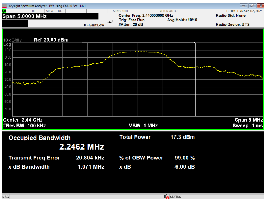
08, 6dB Bandwidth, 2EDR, Mid
