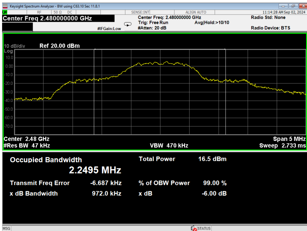
22, Occupied Bandwidth, 3EDR, High
