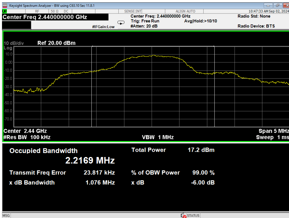
05, Occupied Bandwidth, 2EDR, Mid
