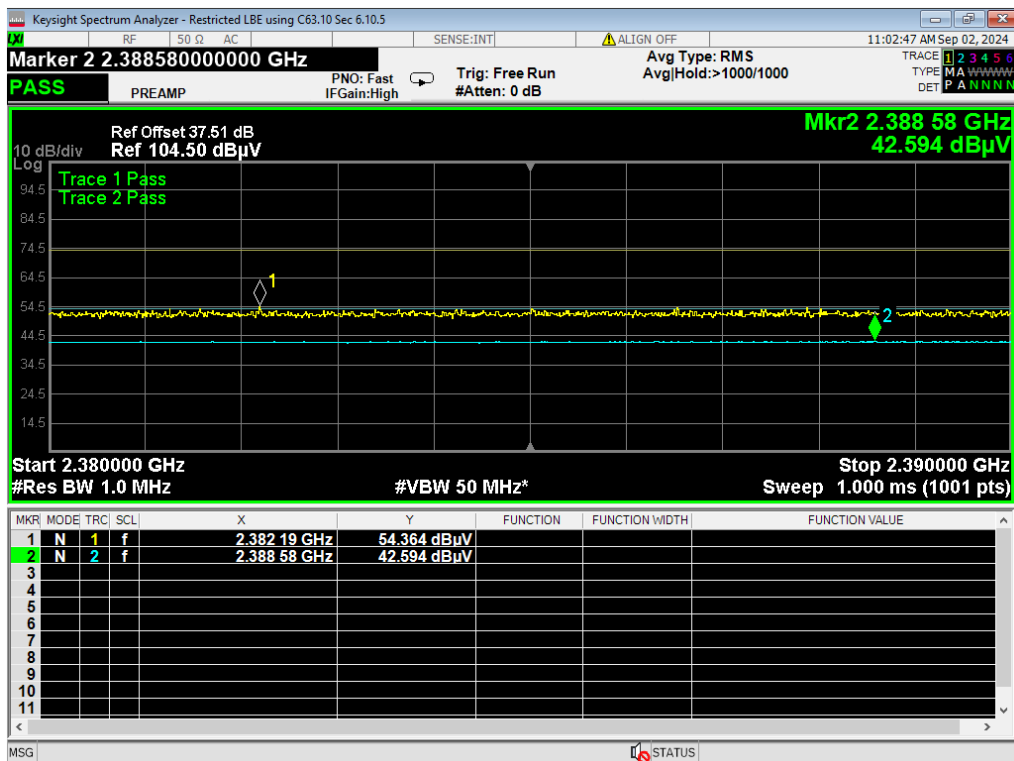
31, LBE Restricted, 3EDR
