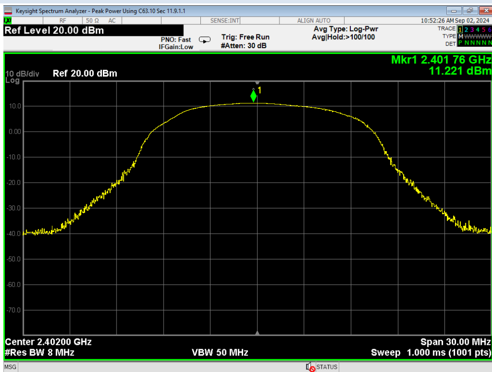
01, Peak Power, 2EDR, Low
