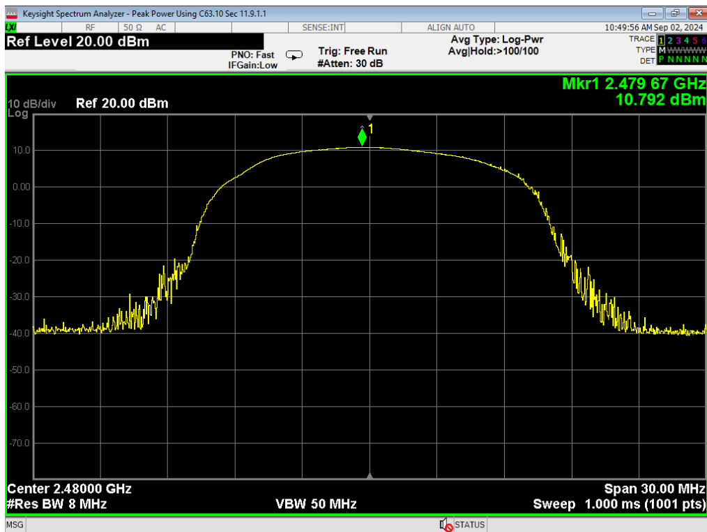
03, Peak Power, 2EDR, High
