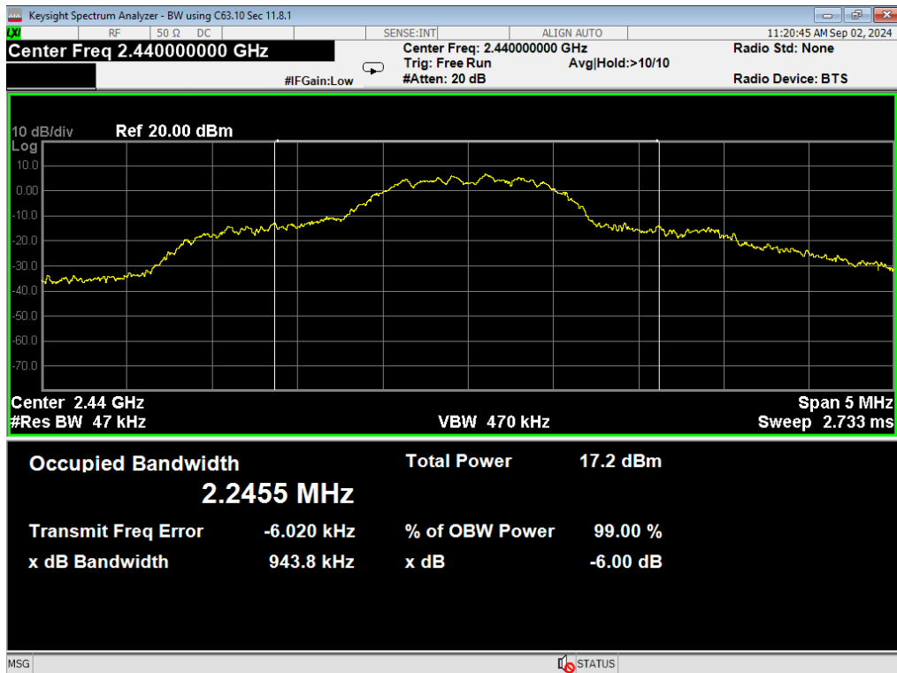
21, Occupied Bandwidth, 3EDR, Mid
