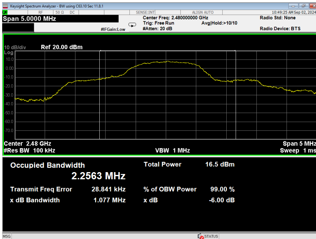
09, 6dB Bandwidth, 2EDR, High
