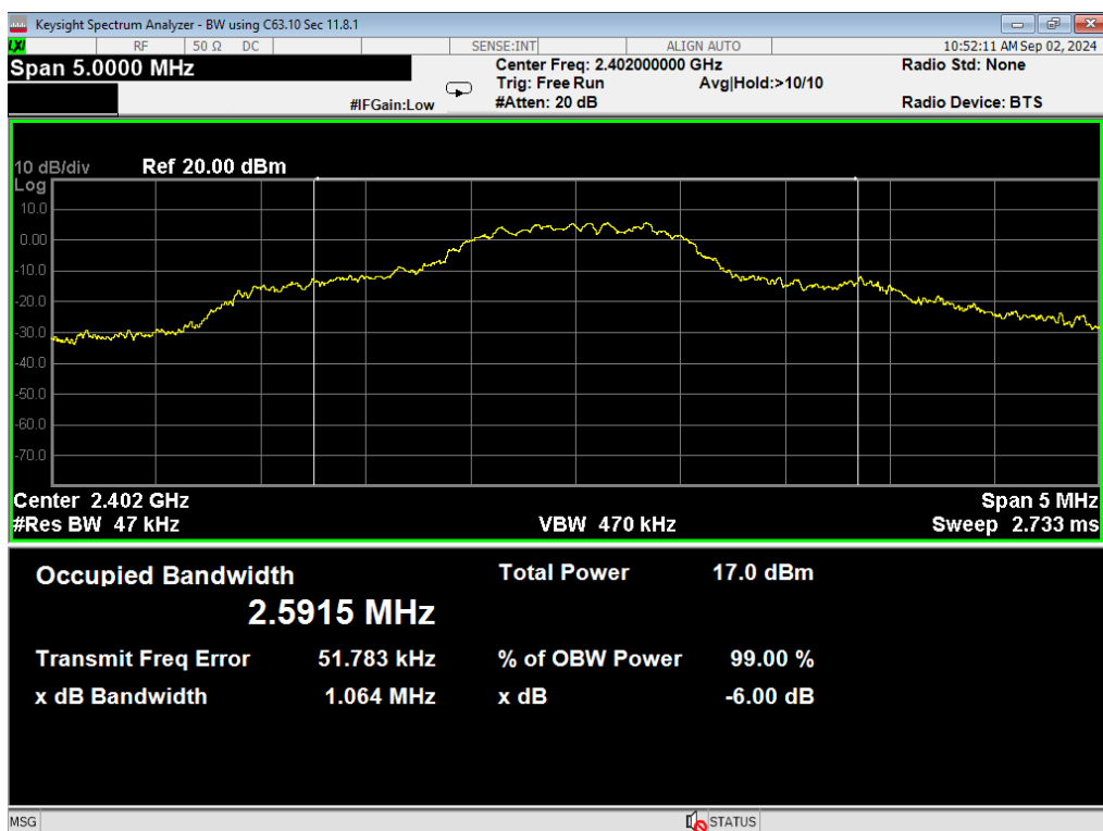
04, Occupied Bandwidth, 2EDR, Low
