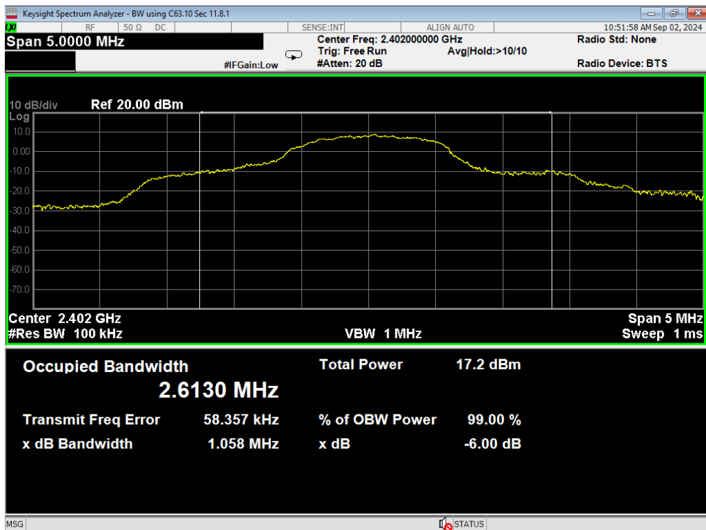
07, 6dB Bandwidth, 2EDR, Low
