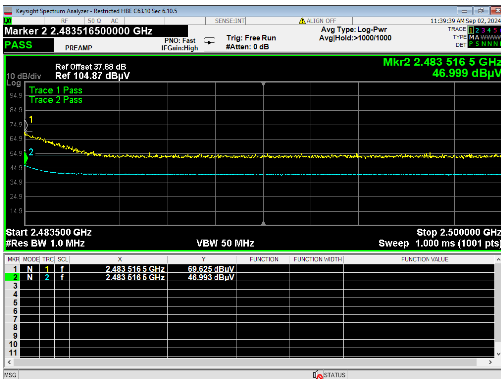
16, HBE Restricted, 2EDR
