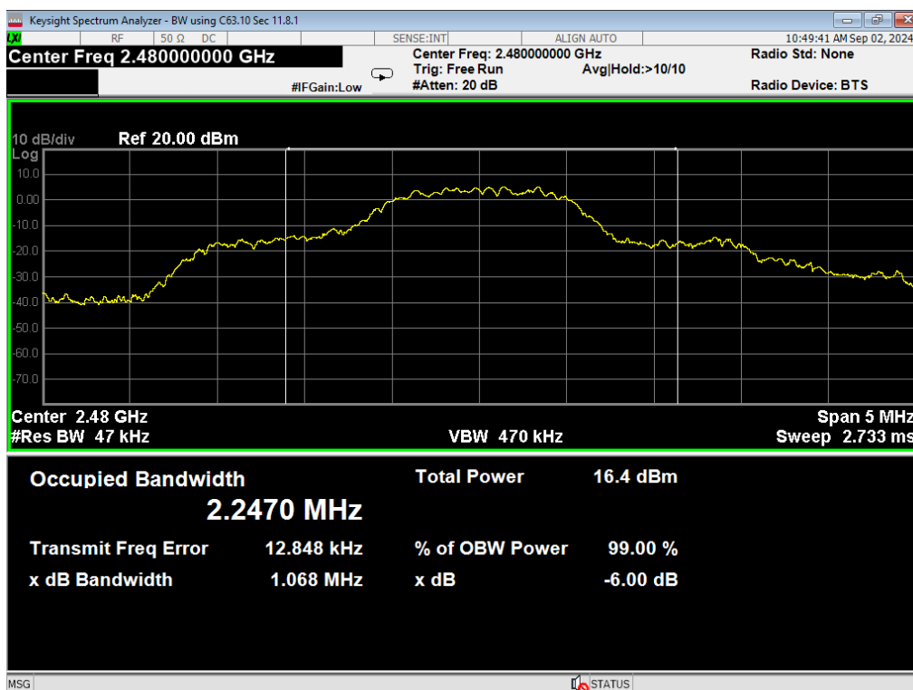
06, Occupied Bandwidth, 2EDR, High
