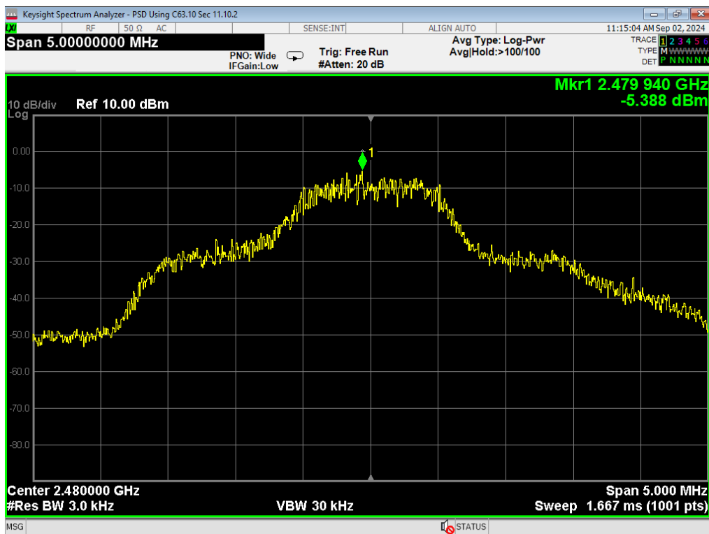
28, PSD, 3EDR, High
