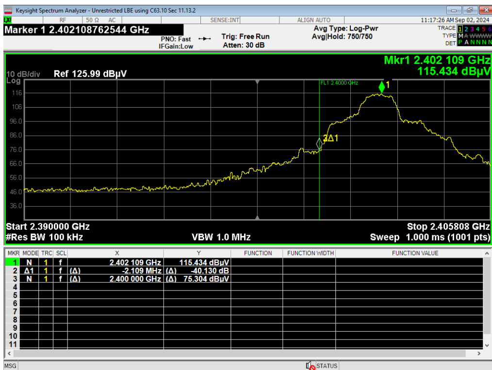
29, LBE Unrestricted, 3EDR
