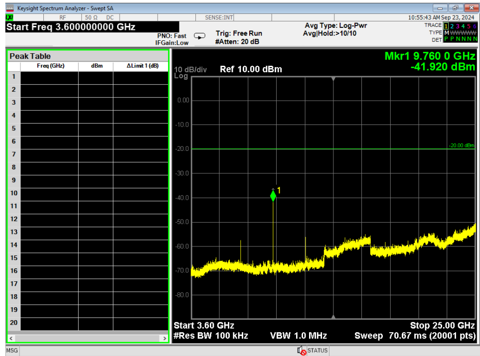
Figure 9 - Radiated Emissions Plot, 2EDR, 3.6GHz – 25GHz, Mid
