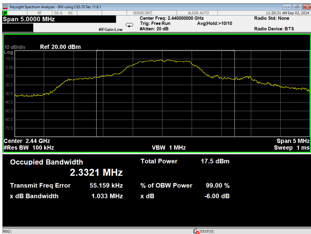
24, 6dB Bandwidth, 3EDR, Mid
