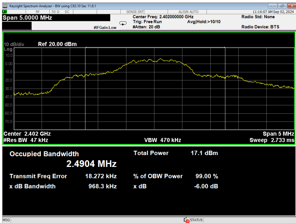
20, Occupied Bandwidth, 3EDR, Low
