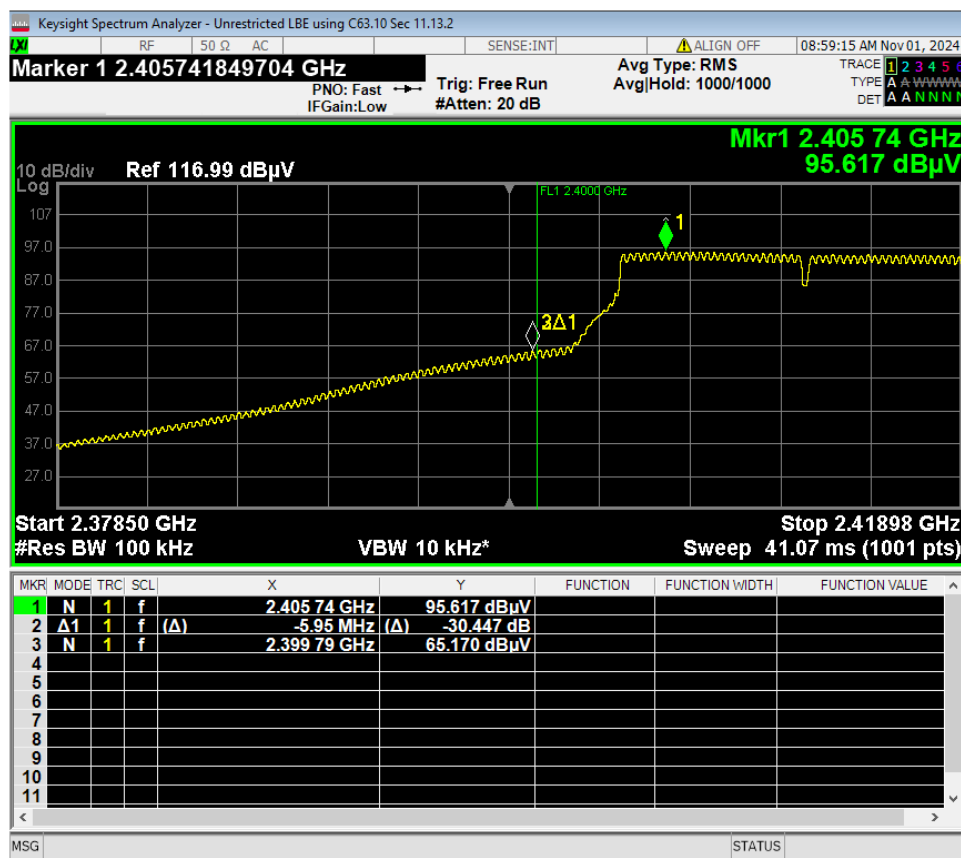
62 Lower Bandedge, Unrestricted, Wifi G, High Data Rate
