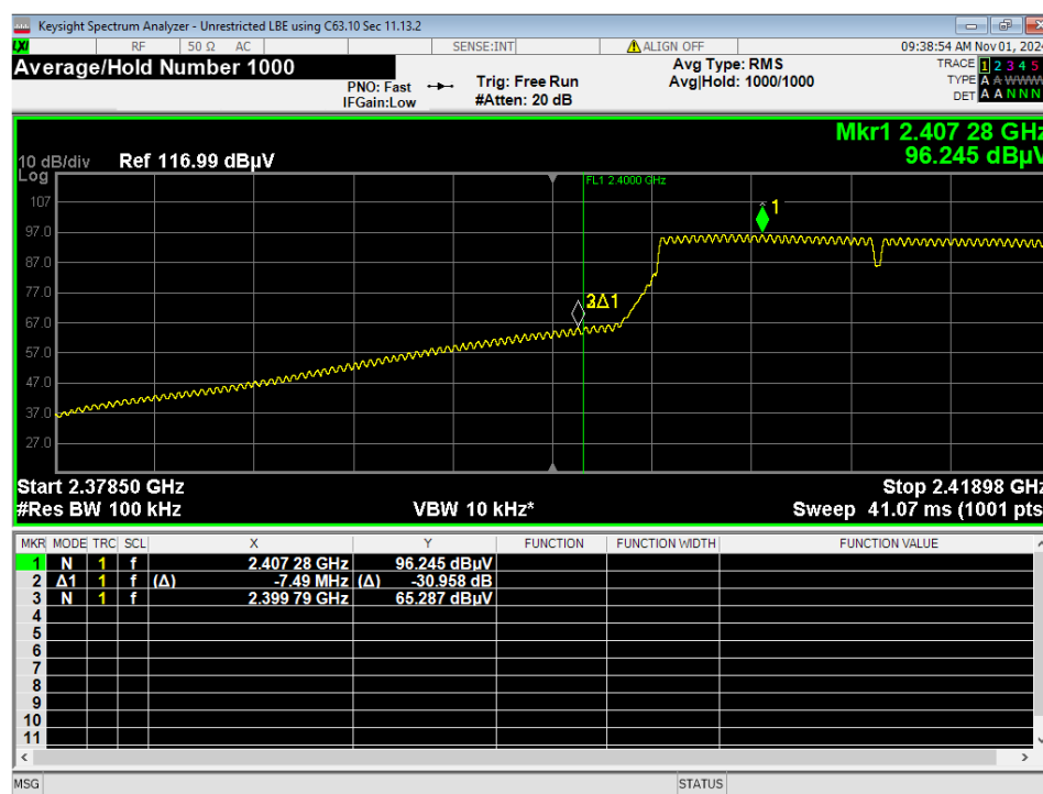
36 Lower Bandedge, Unrestricted, Wifi N, Low Data Rate
