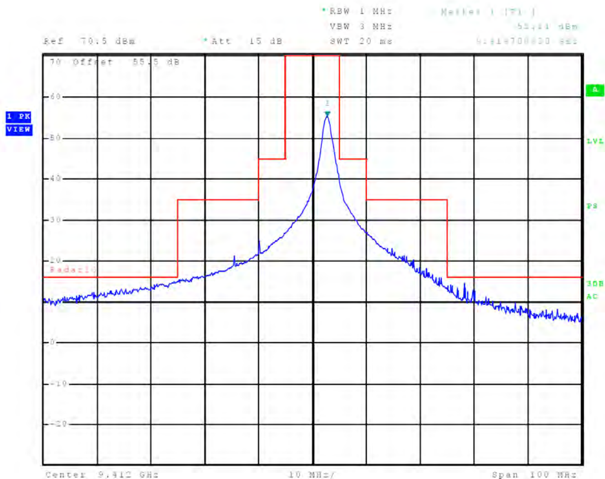
Figure 57 Emissions Mask, 36 nm
