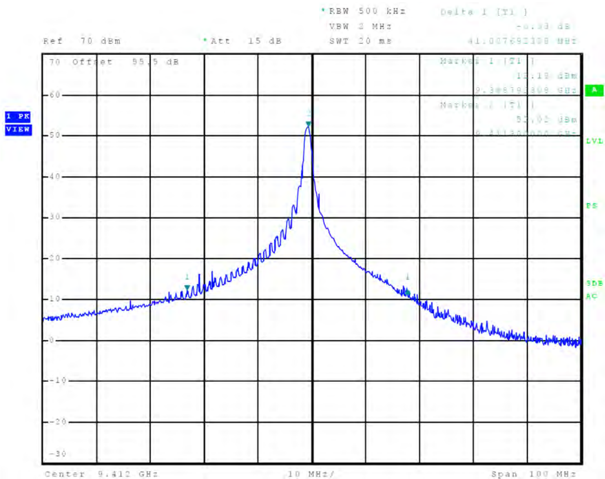
Figure 35 40-dB Occupied Bandwidth Plot, 18 nm
