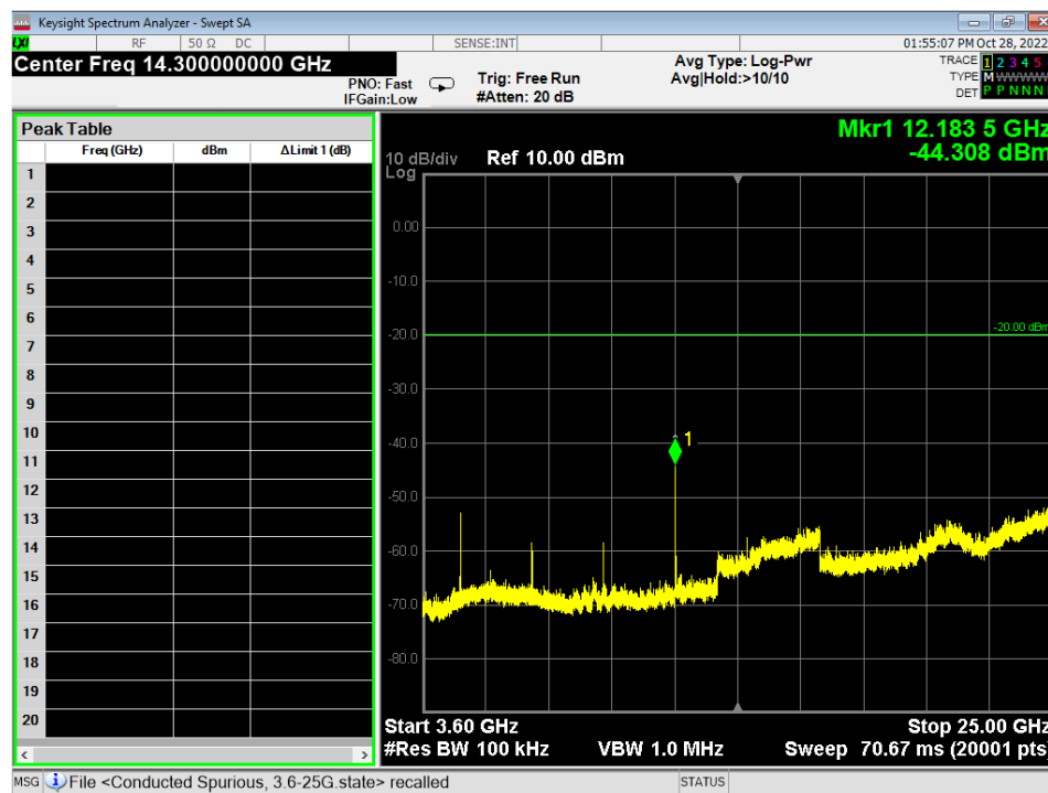
Figure 5 - Conducted Emissions Plot, Wifi B 1MB, 3.6G – 25G
