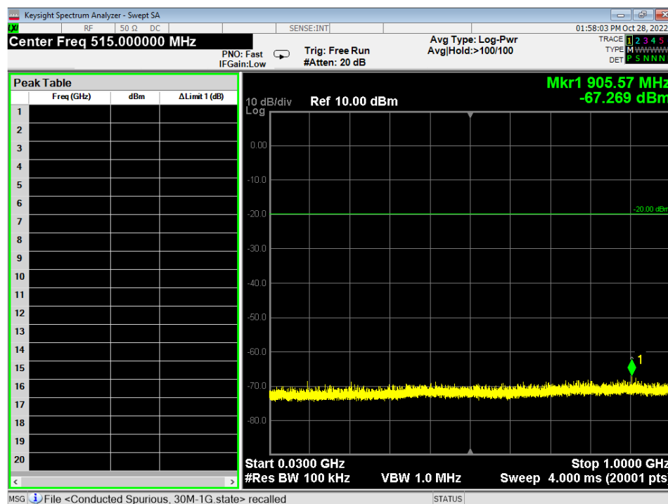
Figure 6 - Conducted Emissions Plot, Wifi G 6MB, 30M – 1G
