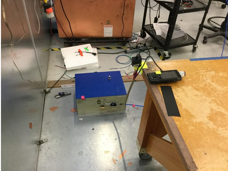
Conducted Emissions, USB-C
