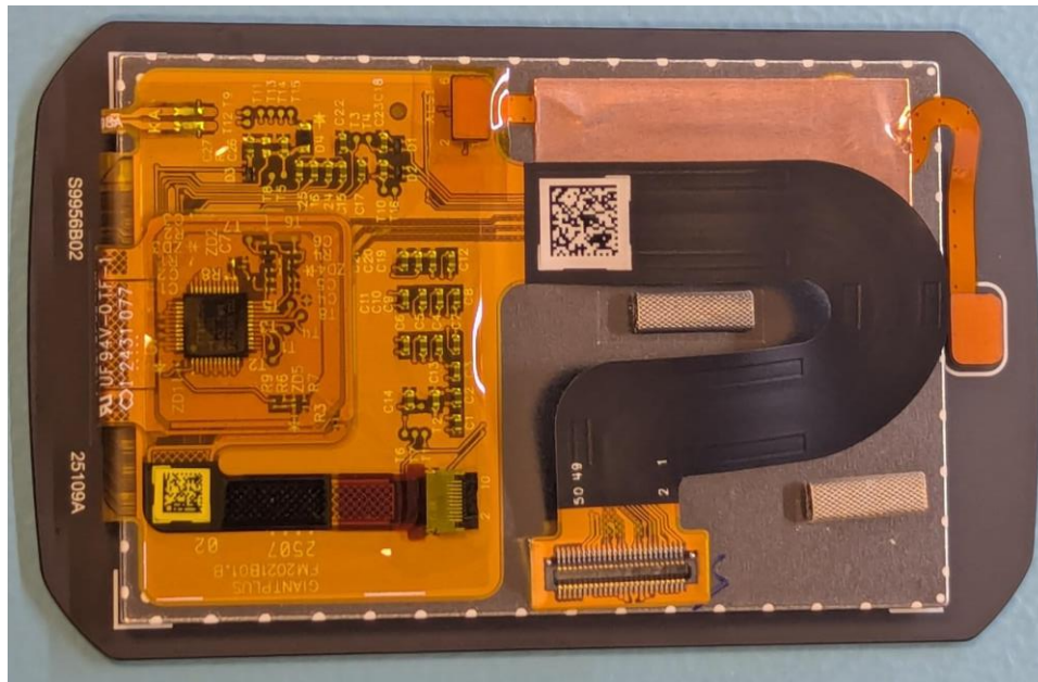
Photograph 07-6: Screen connections
