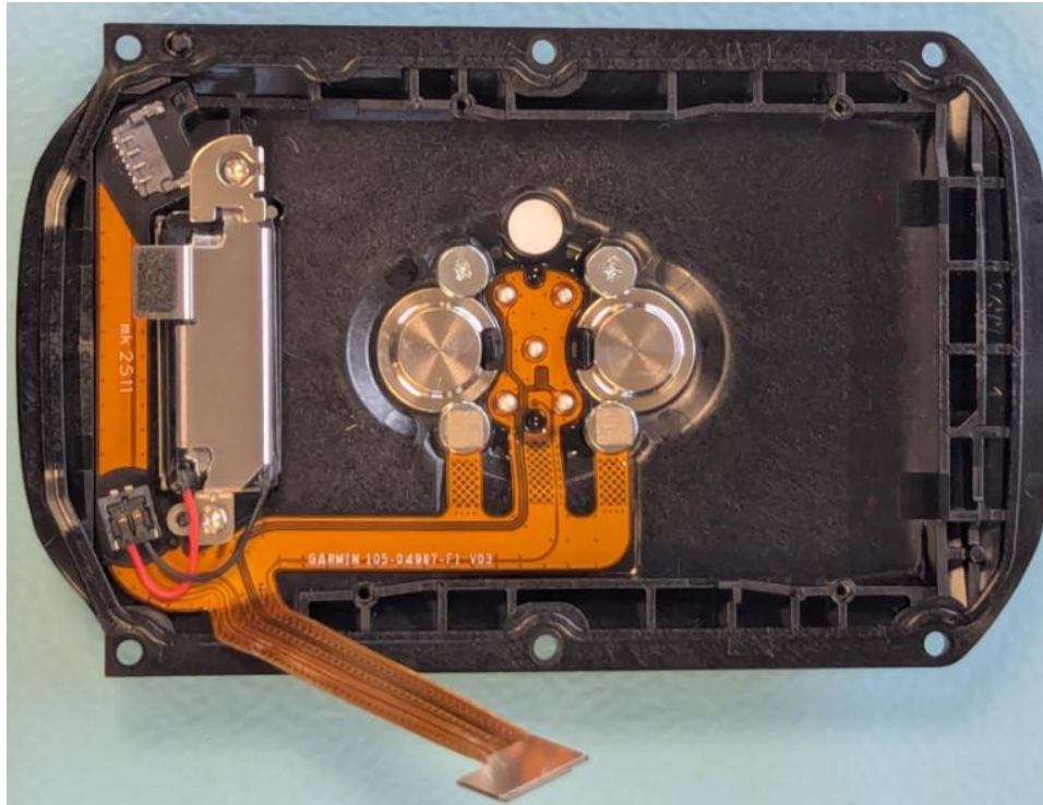
Photograph 07-5: Lower enclosure components – battery removed
