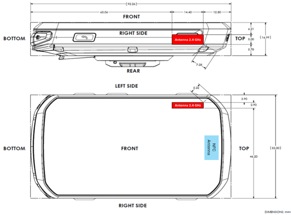
Figure A DUT Antenna Diagram
