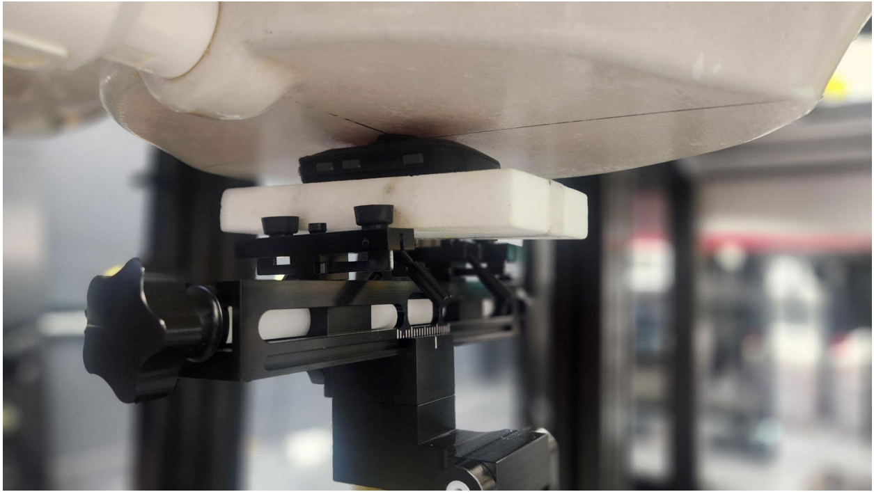
Figure B SAR Test Setup – Body/Extremity – Back 0mm – SAM Phantom
