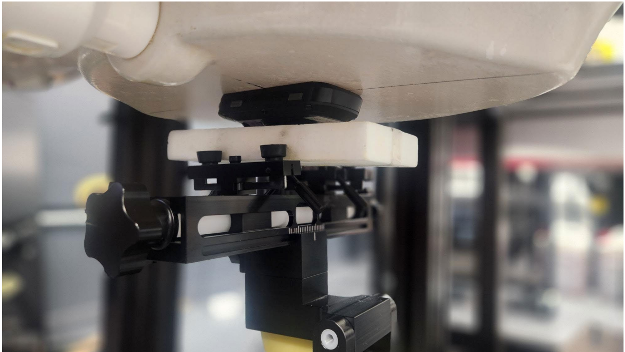
Figure C SAR Test Setup – Body/Extremity – Front 0mm – SAM Phantom
