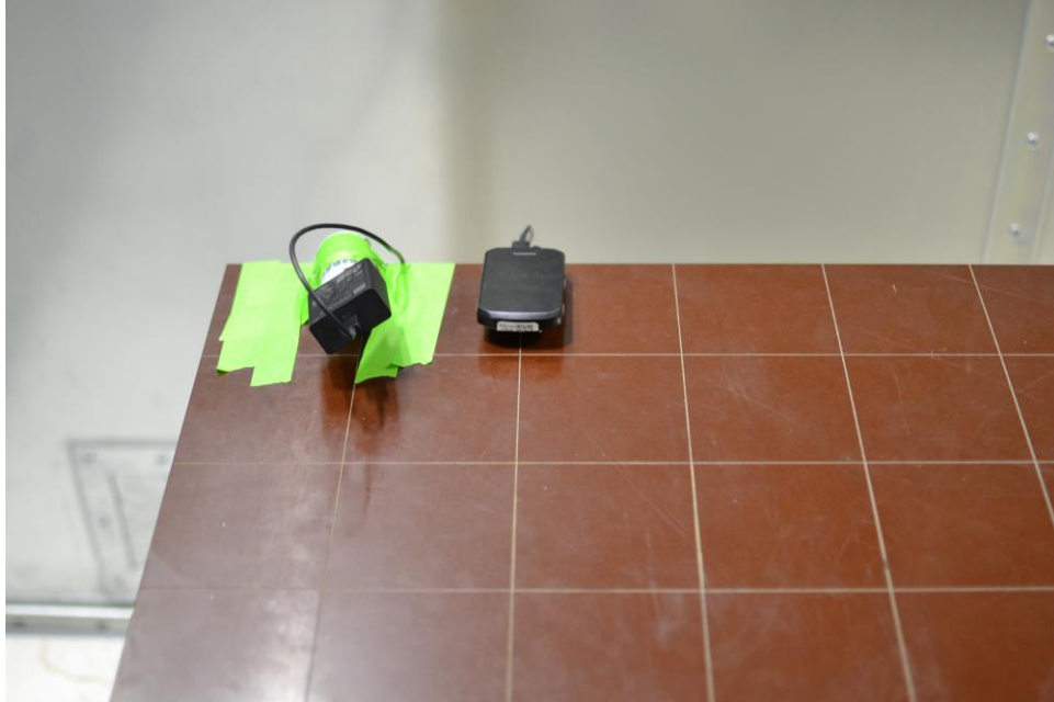
Plot 13. Test Setup – AC Line Conducted - <30MHz
