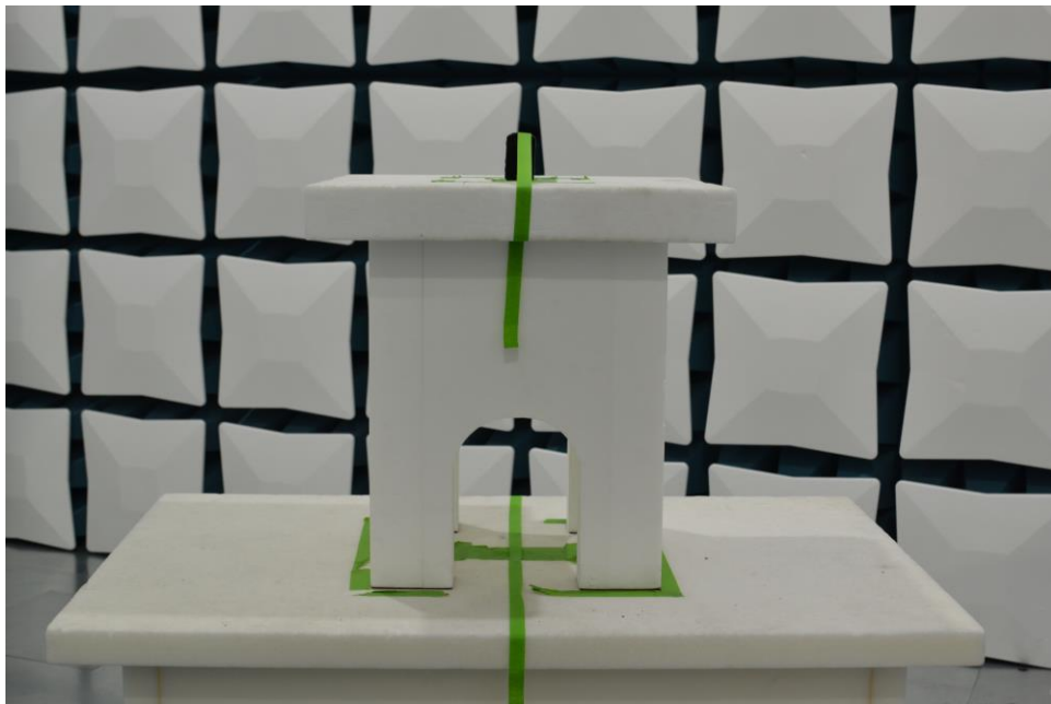
Plot 6. Test Setup – Z Orientation – 1GHz – 26.5GHz - Back
