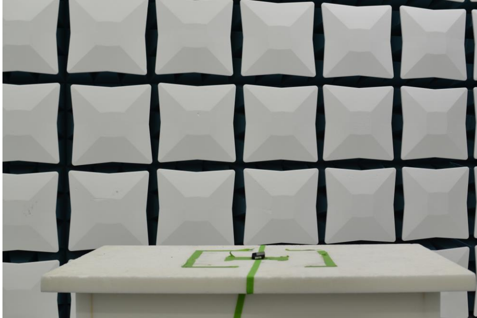
Plot 7. Test Setup – X Orientation – <1GHz - Front
