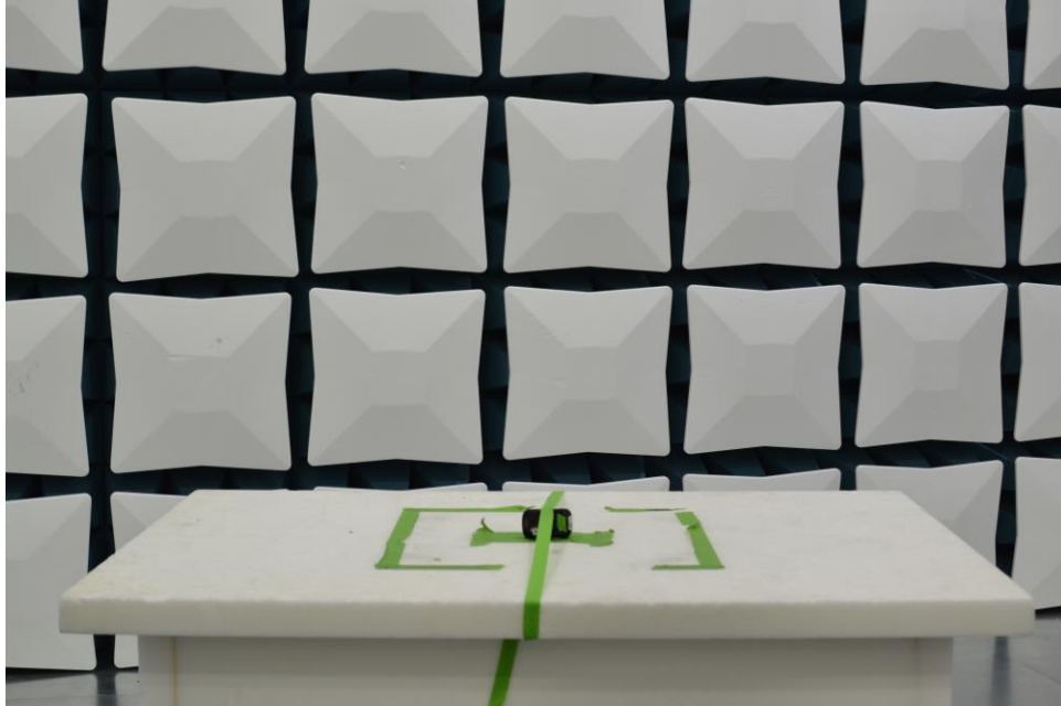
Plot 9. Test Setup – Y Orientation – <1GHz - Front
