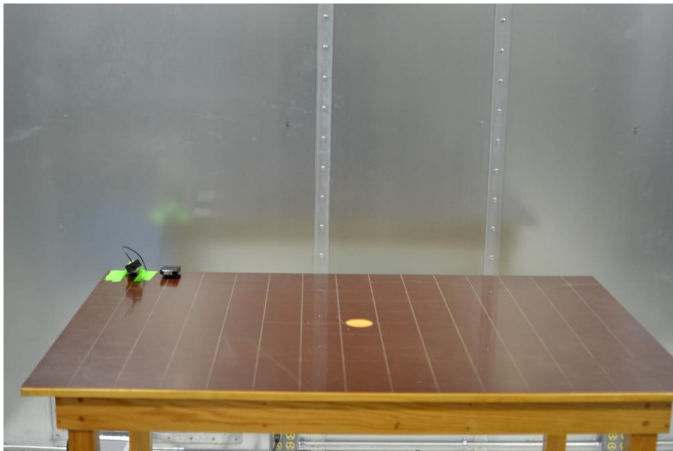
Plot 14. Test Setup – AC Line Conducted - <30MHz
