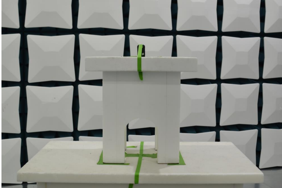
Plot 5. Test Setup – Z Orientation – 1GHz – 26.5GHz - Front
