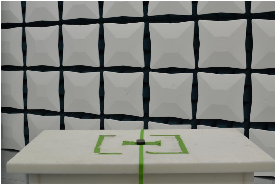
Plot 8. Test Setup – X Orientation – <1GHz - Back
