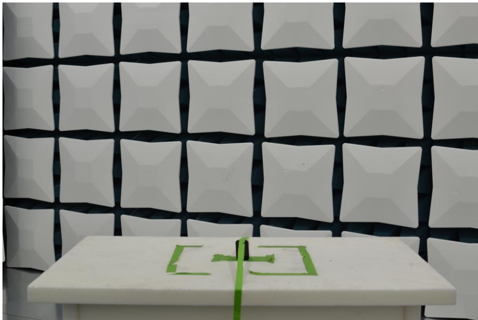
Plot 12. Test Setup – Z Orientation – <1GHz - Back
