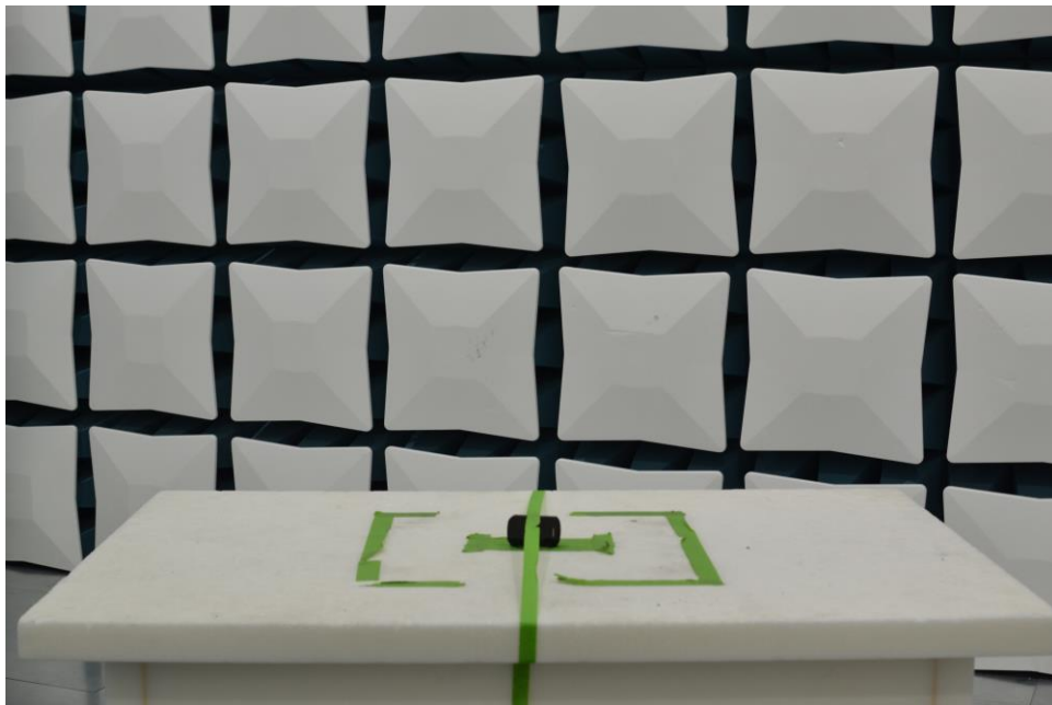
Plot 10. Test Setup – Y Orientation – <1GHz - Back
