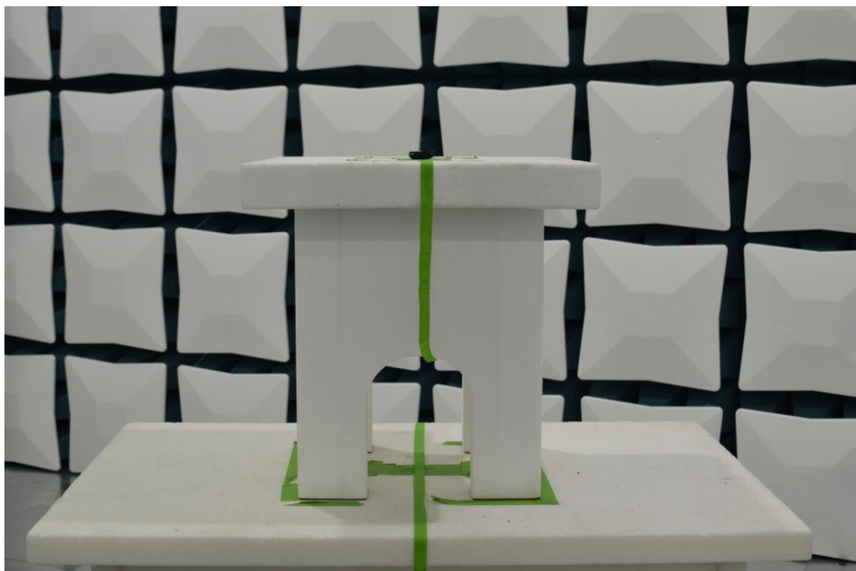
Plot 2. Test Setup – X Orientation – 1GHz – 26.5GHz - Back
