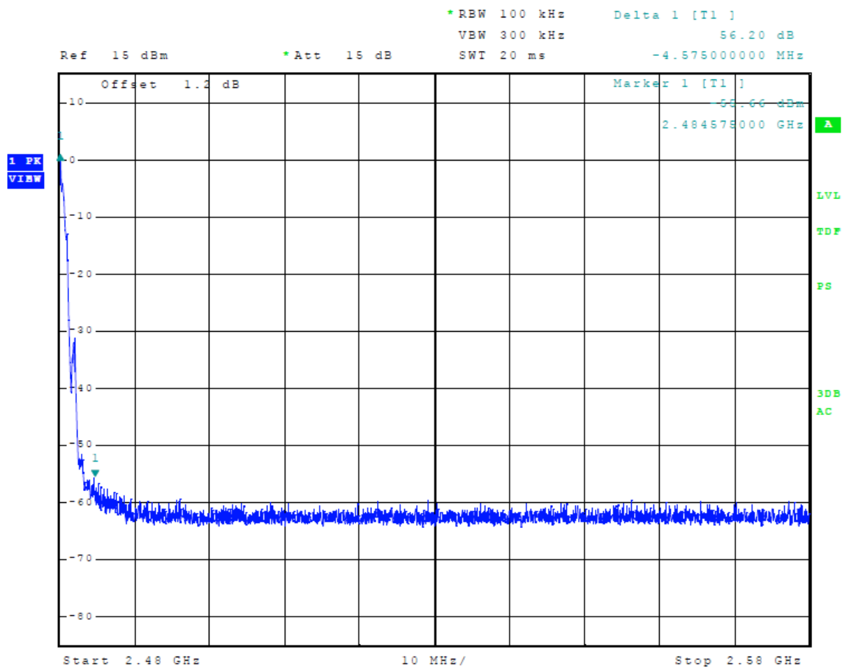
Figure 15 Plot of Transmitter Emissions High Band Edge Mode 3, BT BLE 2M (GMSK)
