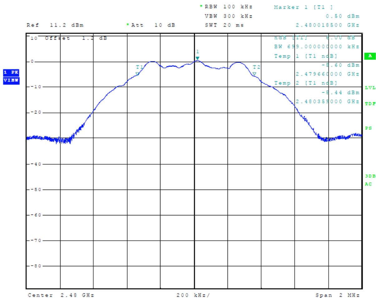
Figure 16 Plot of 6-dB Occupied Bandwidth Mode 2, BT BLE 1M (GMSK)
