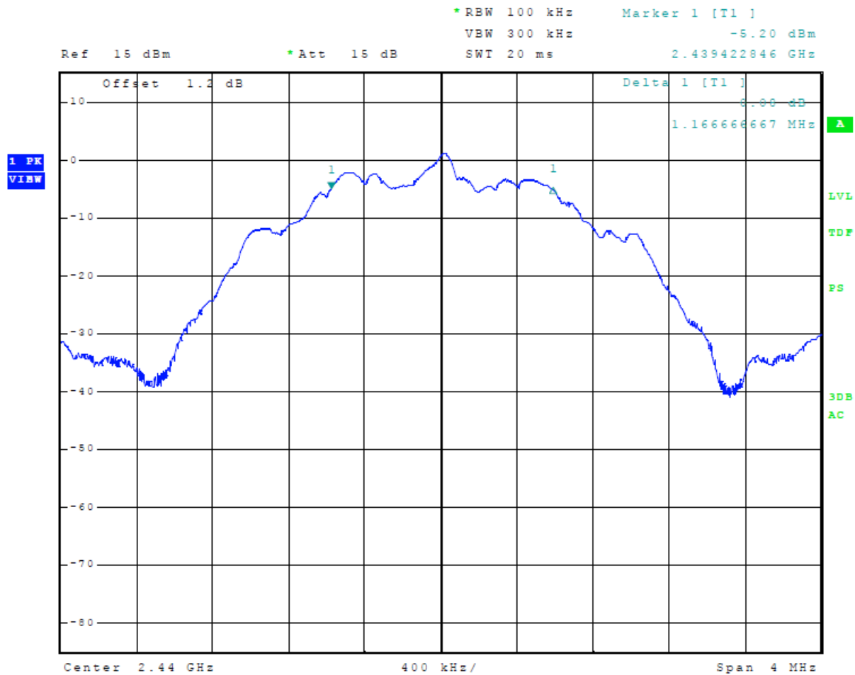
Figure 18 Plot of 6-dB Occupied Bandwidth Mode 3, BT BLE 2M (GMSK)
