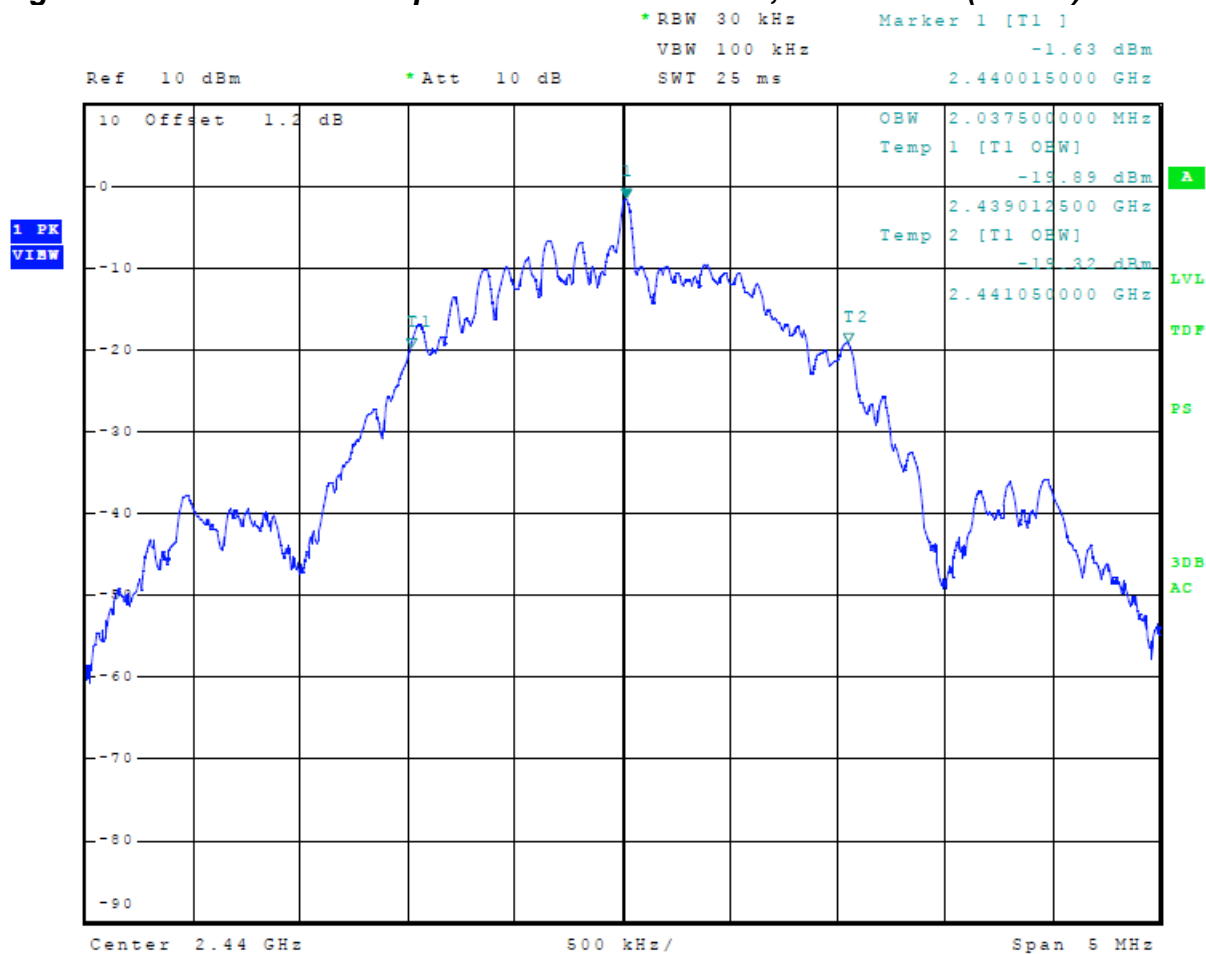
Figure 19 Plot of 99% Occupied Bandwidth Mode 3, BT BLE 2M (GMSK)
