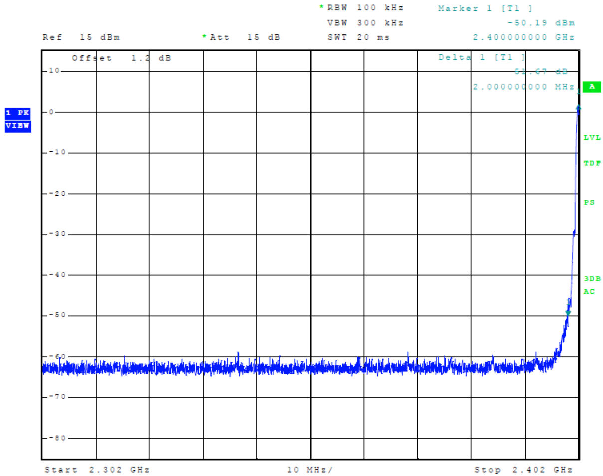
Figure 12 Plot of Emissions Low Band Edge Mode 2, BT BLE 1M (GMSK)
