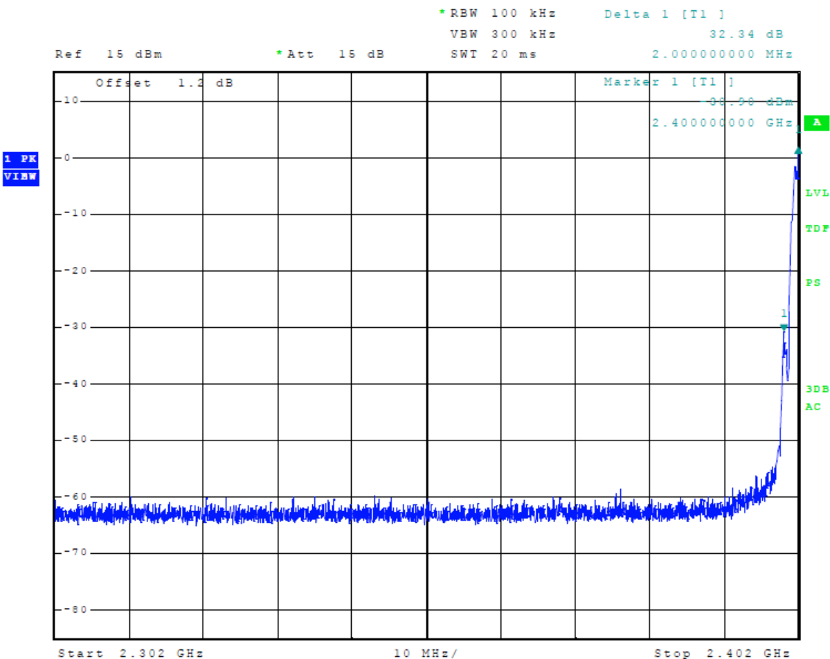
Figure 13 Plot of Emissions Low Band Edge Mode 3, BT BLE 2M (GMSK)
