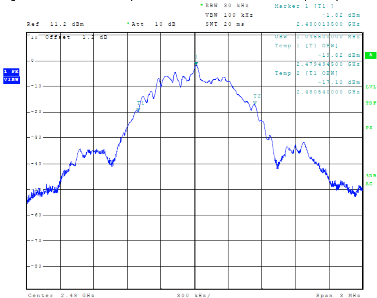
Figure 17 Plot of 99% Occupied Bandwidth Mode 2, BT BLE 1M (GMSK)
