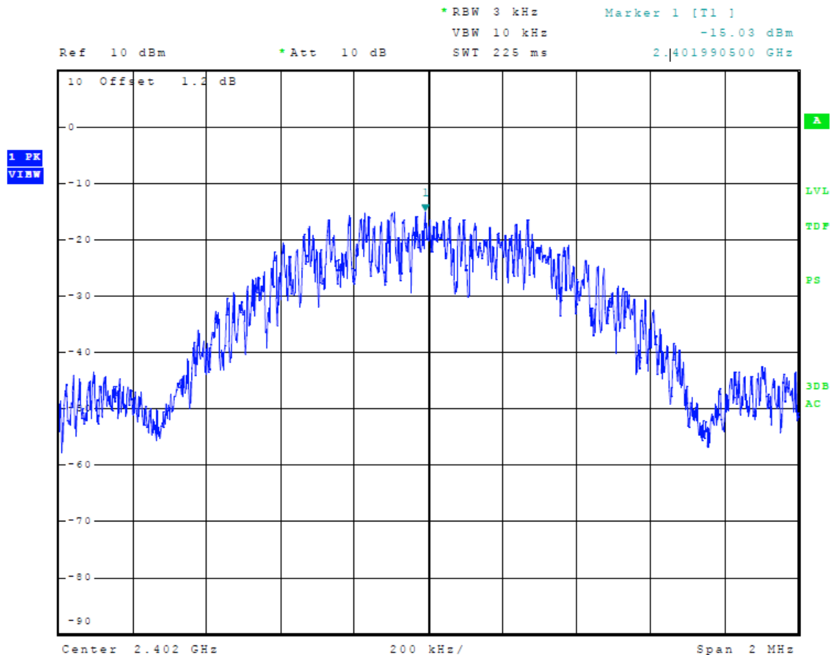
Figure 20 Plot of Transmitter Power Spectral Density Mode 2, BT BLE 1M (GMSK)
