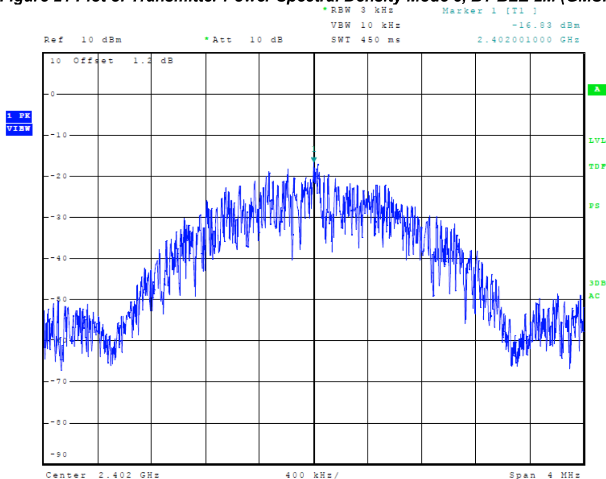
Figure 21 Plot of Transmitter Power Spectral Density Mode 3, BT BLE 2M (GMSK)
