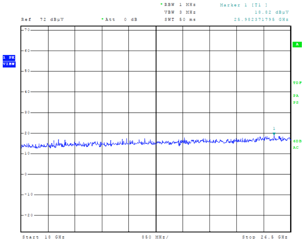
Figure 9 Plot of General Radiated Emissions (18 GHz – 26.5 GHz) All Tx On
