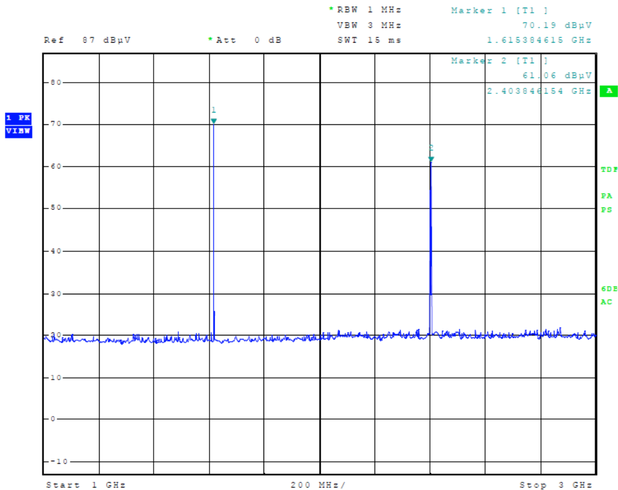
Figure 5 Plot of General Radiated Emissions (1 GHz – 3 GHz) All Tx On
