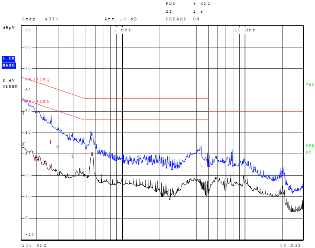
Figure 1 AC Line Conducted Emissions Data L1 (Config. #3, EUT – laptop)
