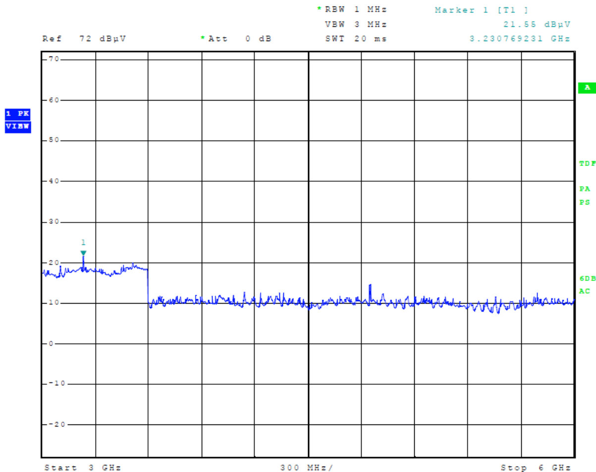
Figure 6 Plot of General Radiated Emissions (3 GHz – 6 GHz) All Tx On
