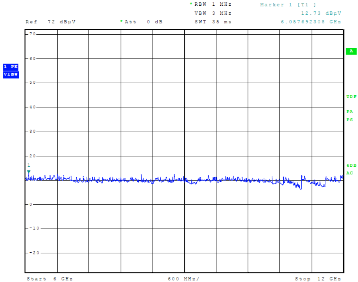
Figure 7 Plot of General Radiated Emissions (6 GHz – 12 GHz) All Tx On
