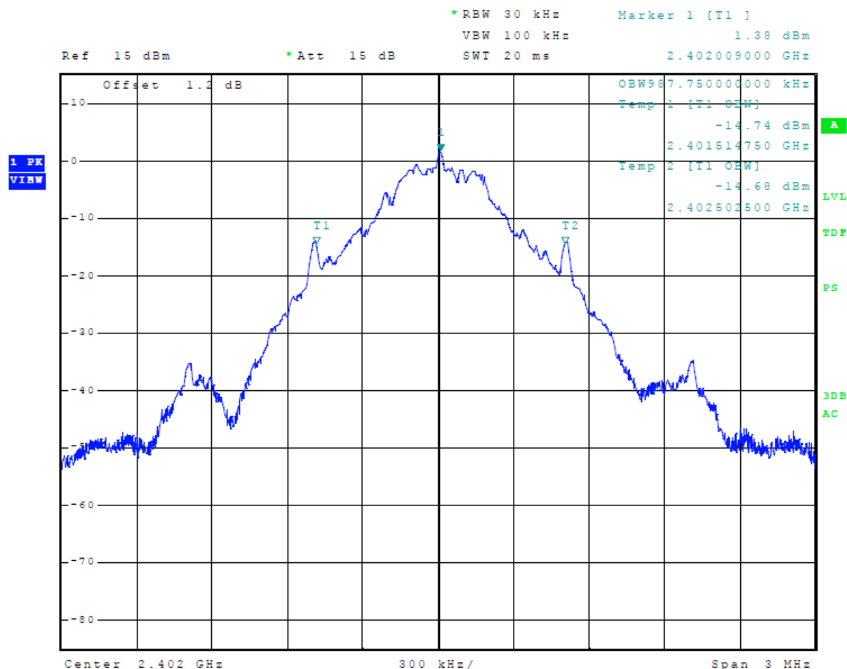
Figure 13 Plot of Transmitter 99% Occupied Bandwidth Mode 1 ANT (GFSK)
