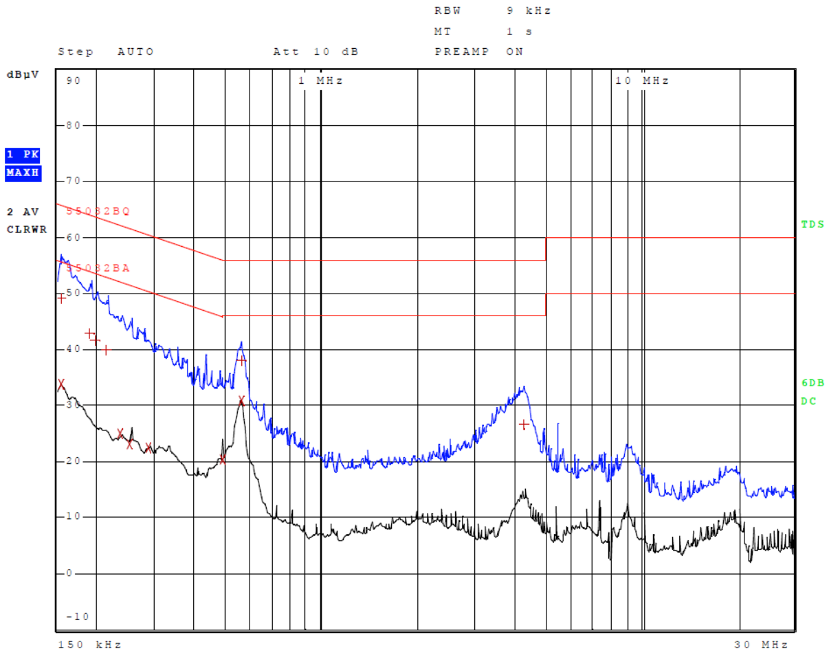
Figure 2 AC Line Conducted Emissions Data L2 (Config. #3, EUT – laptop)
