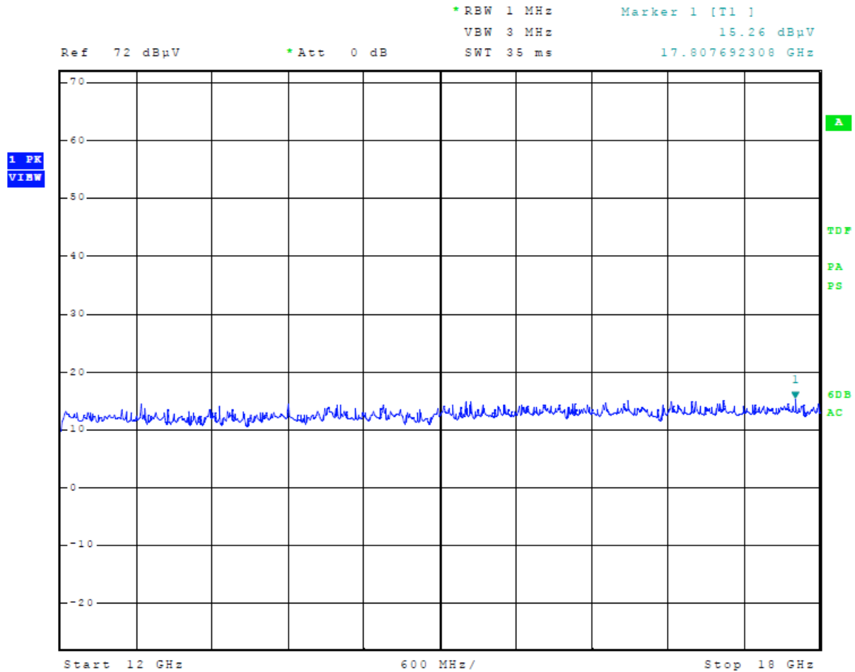
Figure 8 Plot of General Radiated Emissions (12 GHz – 18 GHz) All Tx On
