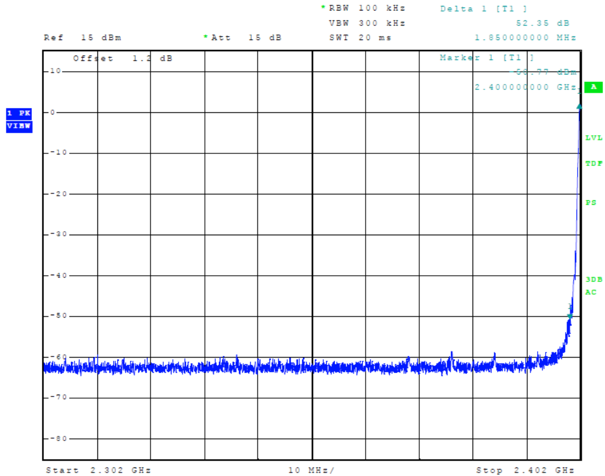
Figure 11 Plot of Transmitter Emissions Low Band Edge Mode 1 ANT (GFSK)
