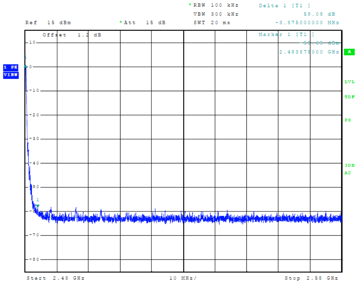
Figure 12 Plot of Transmitter Emissions High Band Edge Mode 1 ANT (GFSK)
