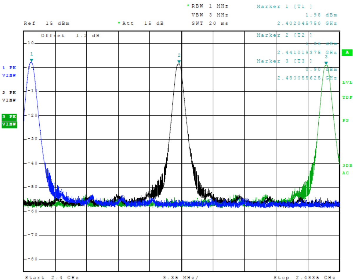
Figure 10 Plot of Transmitter Emissions in 2402-2480 MHz Mode 1 ANT (GFSK)
