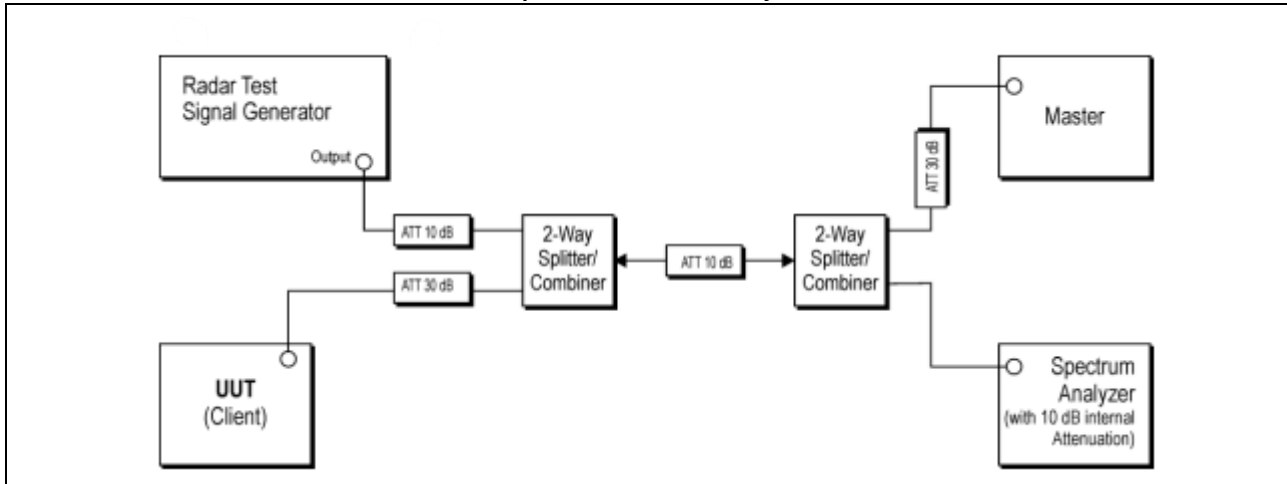
Conducted test setup where Client with injection at the Master
