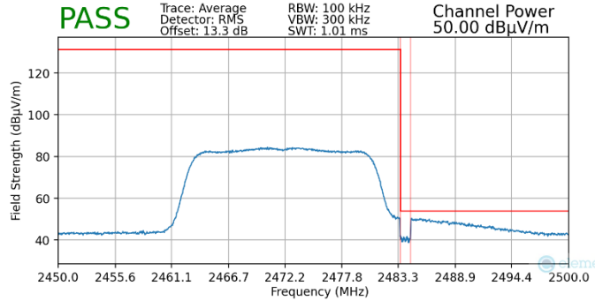
Plot 9-5. Radiated Restricted Upper Band Edge Measurement (Average) – Spot-check
