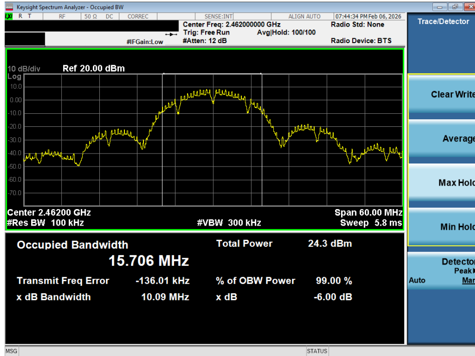
Plot 7-3 6dB BW (20MHz BW 802.11b - Ch.11)
