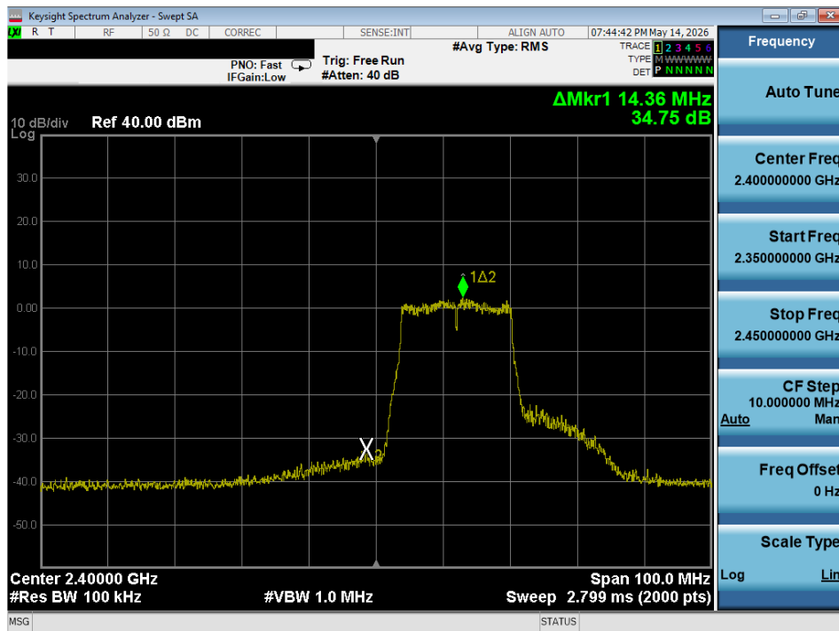
Plot 7-32. Band Edge Plot (802.11g – Ch. 1)
