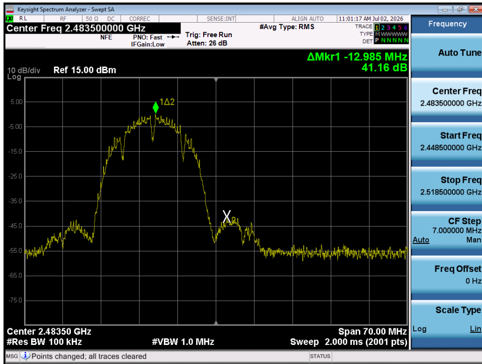
Plot 7-31. Band Edge Plot (802.11b – Ch. 13)
