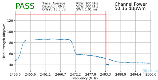
Plot 9-3. Radiated Restricted Upper Band Edge Measurement (Average) – Spot-check
