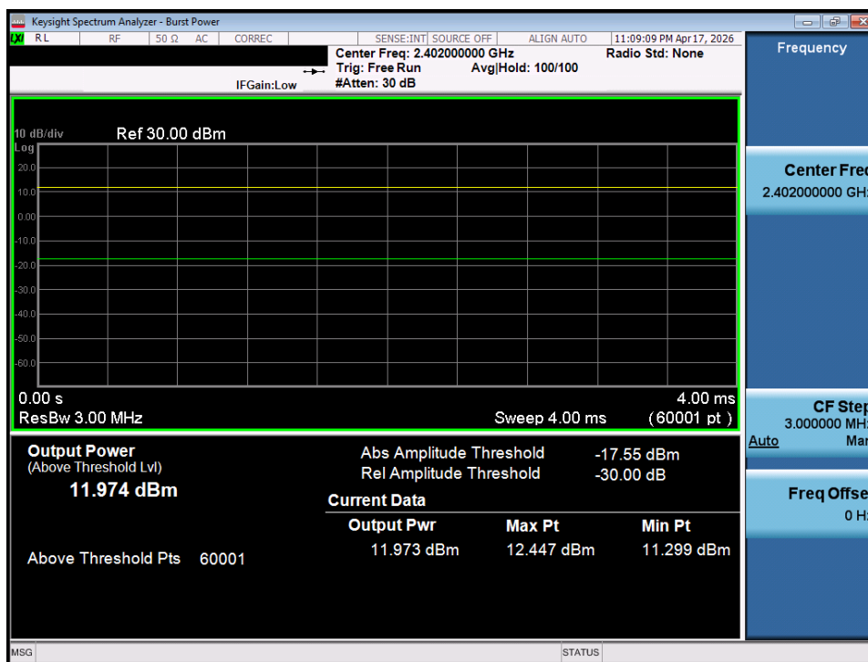
Plot 9-3. Average Conducted Power(Spot-check)
