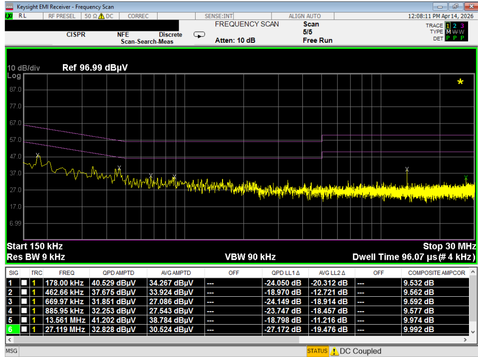
Plot 7-5. Line-Conducted Test Plot (L1)
