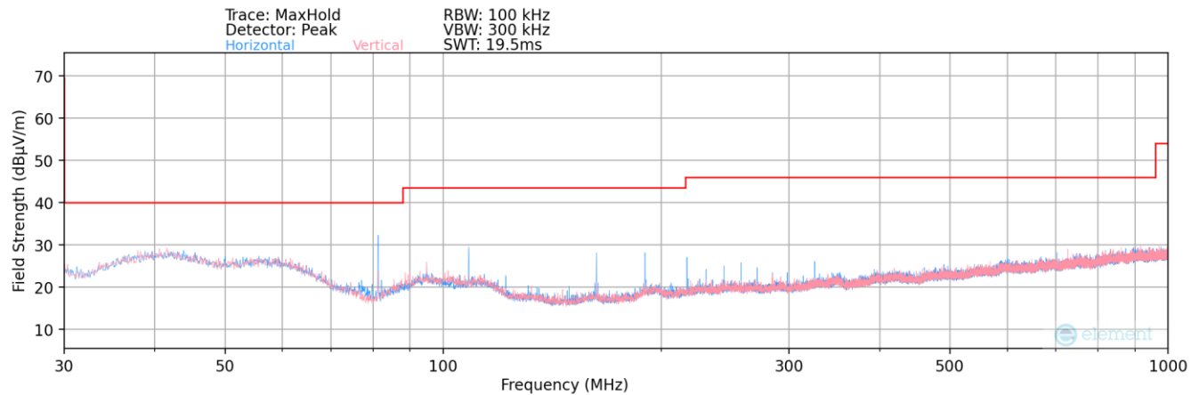
Plot 7-4. Radiated Spurious Plot 30MHz – 1GHz
