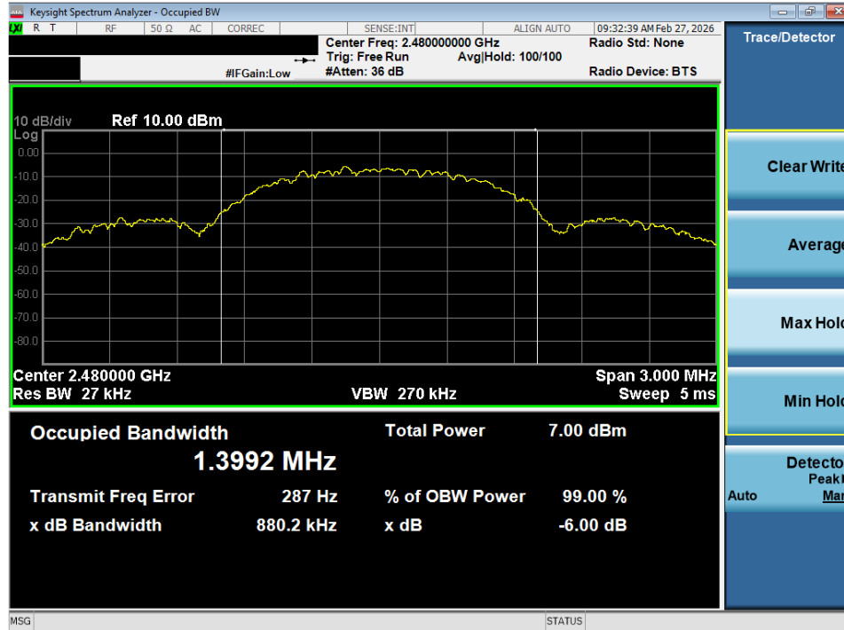
Plot 7-13. OBW Plot (Bluetooth (LE), 1Mbps – Ch. 39)
