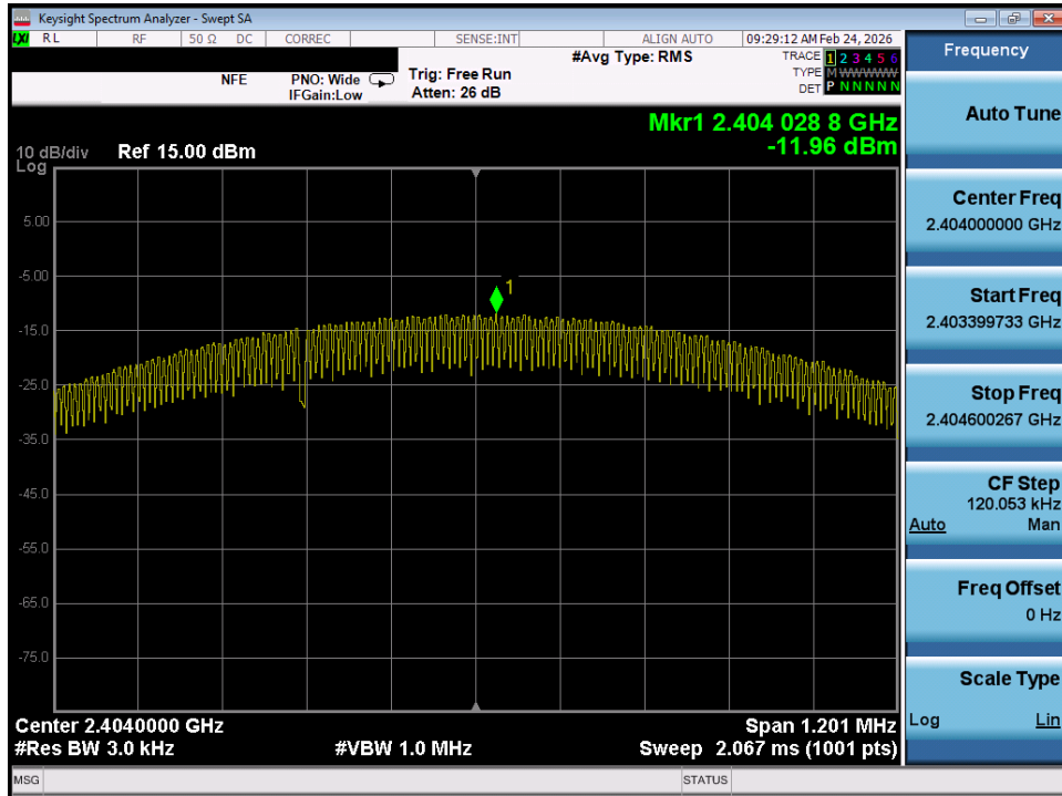
Plot 7-28. Power Spectral Density Plot (Bluetooth (LE), 1Mbps – Ch. 0)
