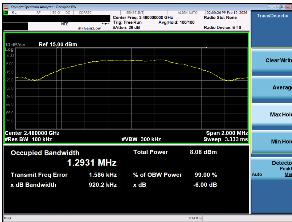
Plot 7-6. 6dB Bandwidth Plot (Bluetooth (LE), 1Mbps – Ch. 39)
