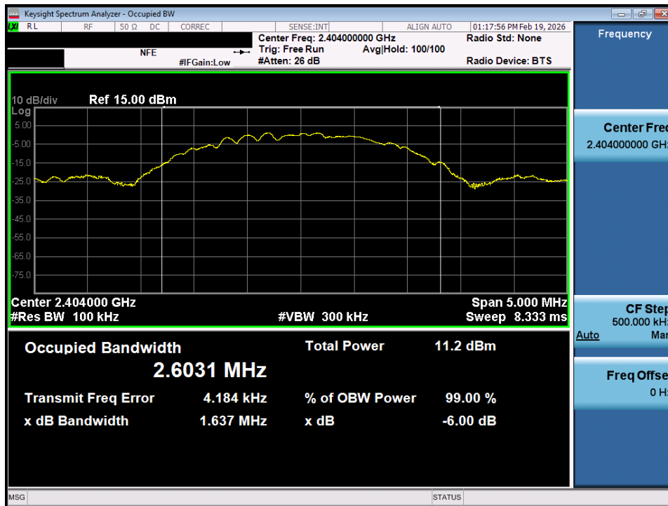
Plot 7-7. 6dB Bandwidth Plot (Bluetooth (LE), 2Mbps – Ch. 0)
