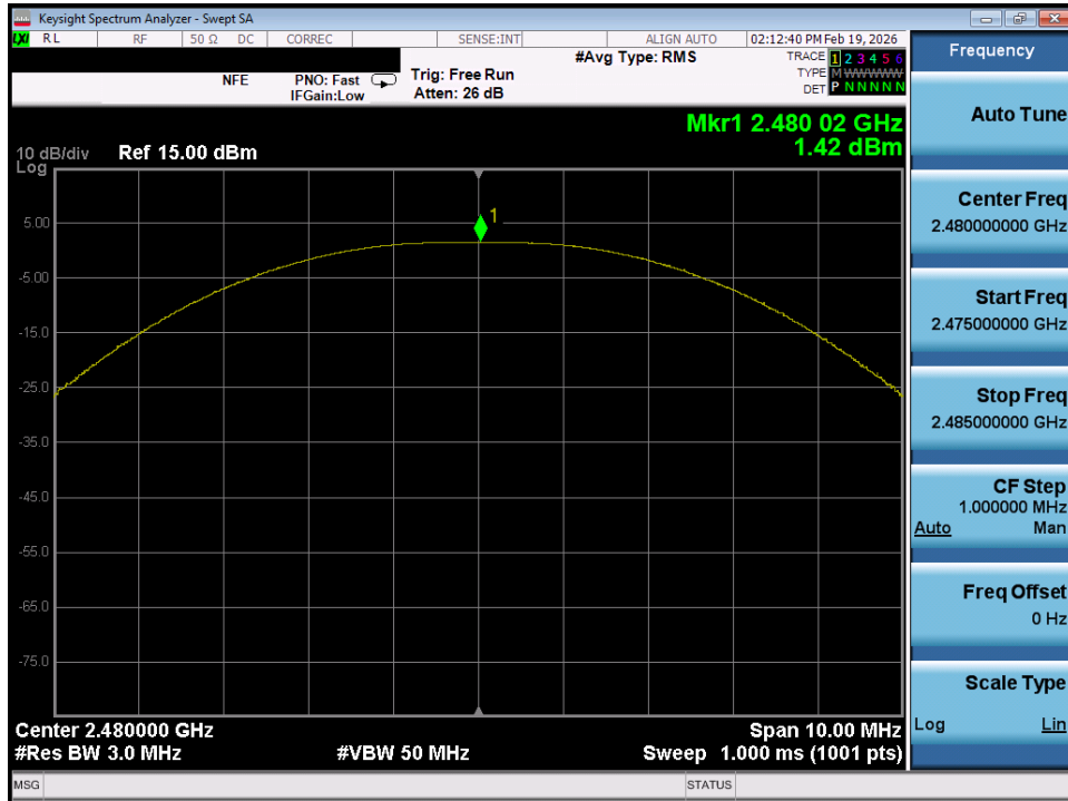
Plot 7-22. Peak Power Plot (Bluetooth (LE), 1Mbps – Ch. 39)
