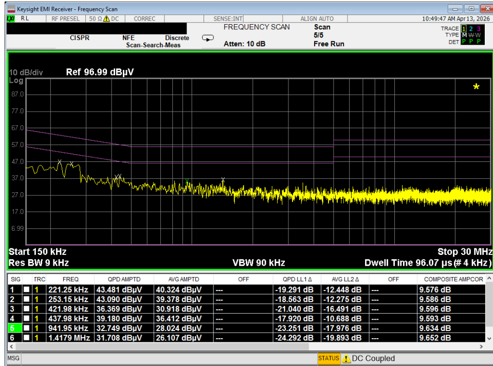
Plot 7-62. Line-Conducted Test Plot (L1)
