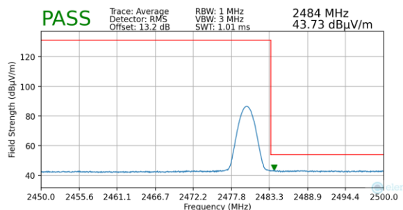
Plot 7-59. Radiated Restricted Upper Band Edge Measurement (Average)
