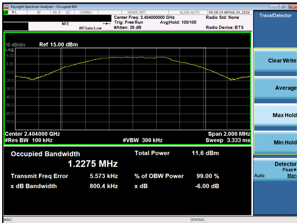
Plot 7-2. 6dB Bandwidth Plot (Bluetooth (LE), 1Mbps – Ch. 0)
