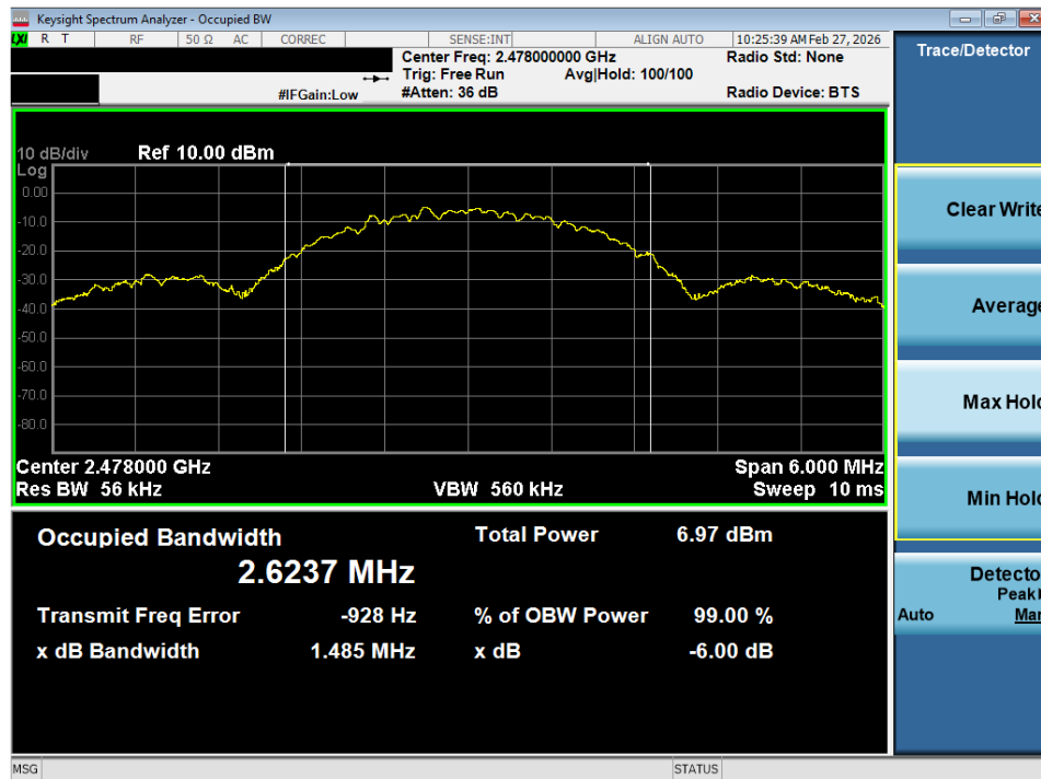
Plot 7-16. OBW Plot (Bluetooth (LE), 2Mbps – Ch. 36)
