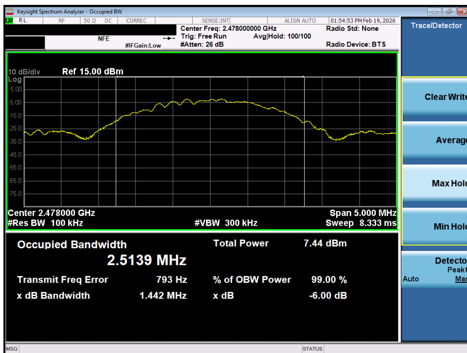
Plot 7-10. 6dB Bandwidth Plot (Bluetooth (LE), 2Mbps – Ch. 36)
