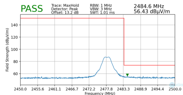
Plot 7-58. Radiated Restricted Upper Band Edge Measurement (Peak)
