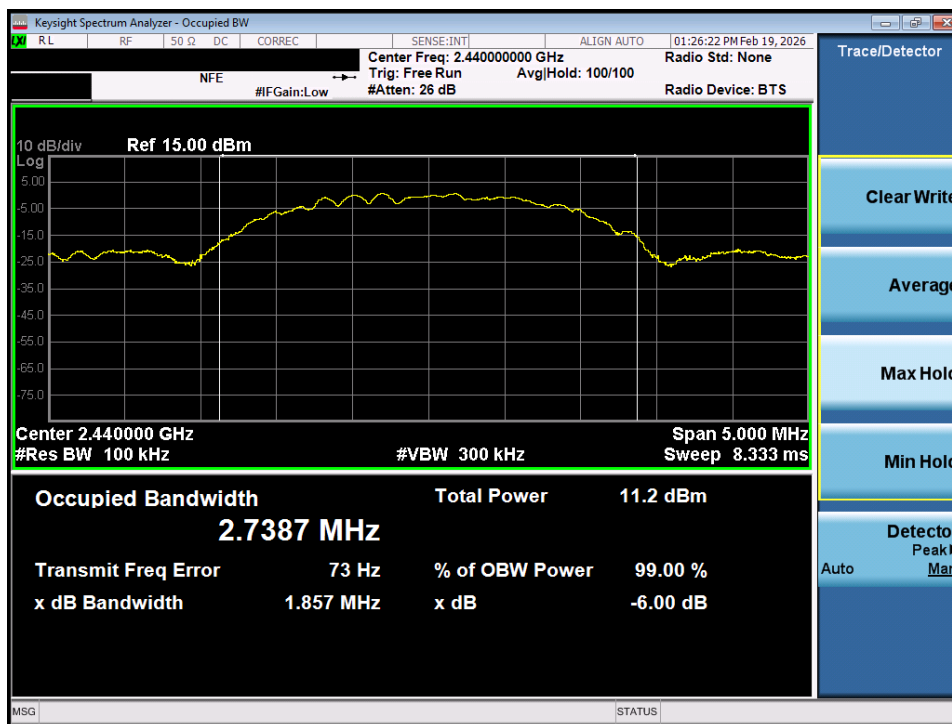
Plot 7-8. 6dB Bandwidth Plot (Bluetooth (LE), 2Mbps – Ch. 17)
