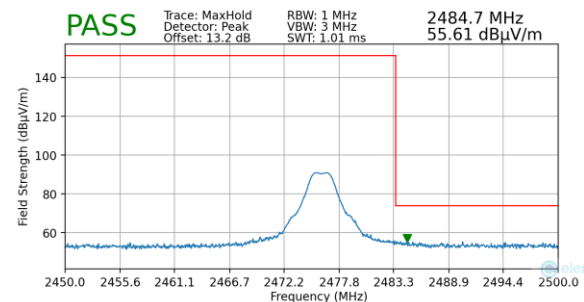
Plot 7-56. Radiated Restricted Upper Band Edge Measurement (Peak)
