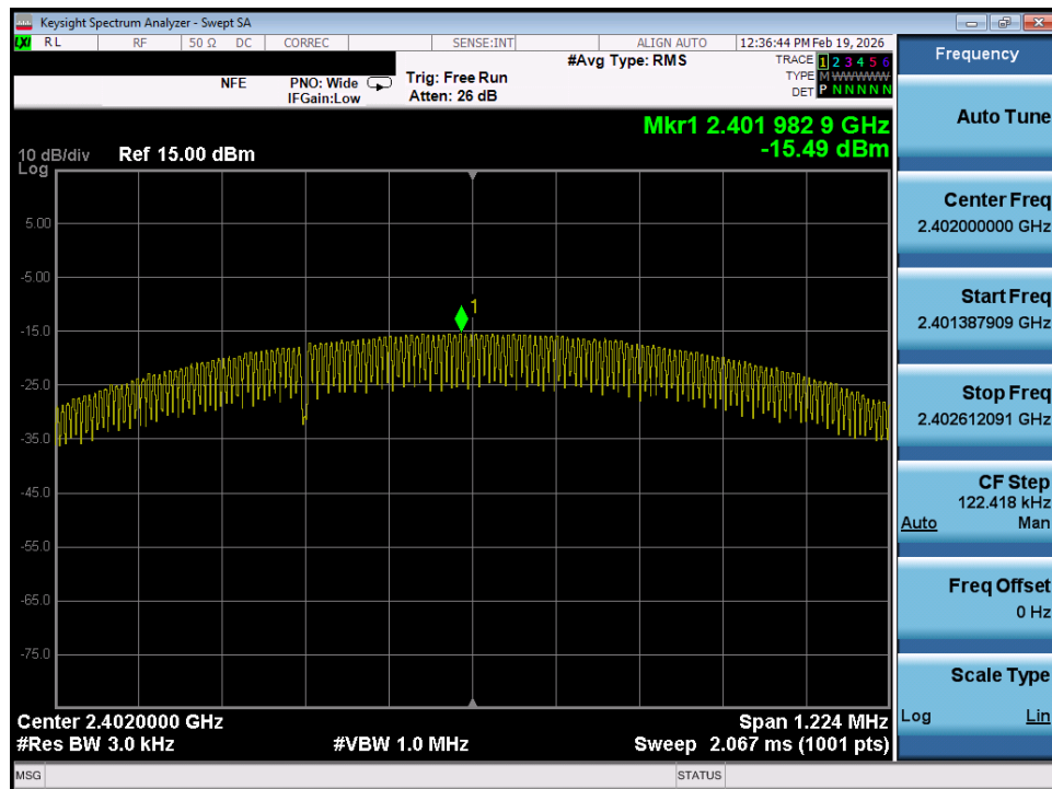
Plot 7-27. Power Spectral Density Plot (Bluetooth (LE), 1Mbps – Ch. 37)
