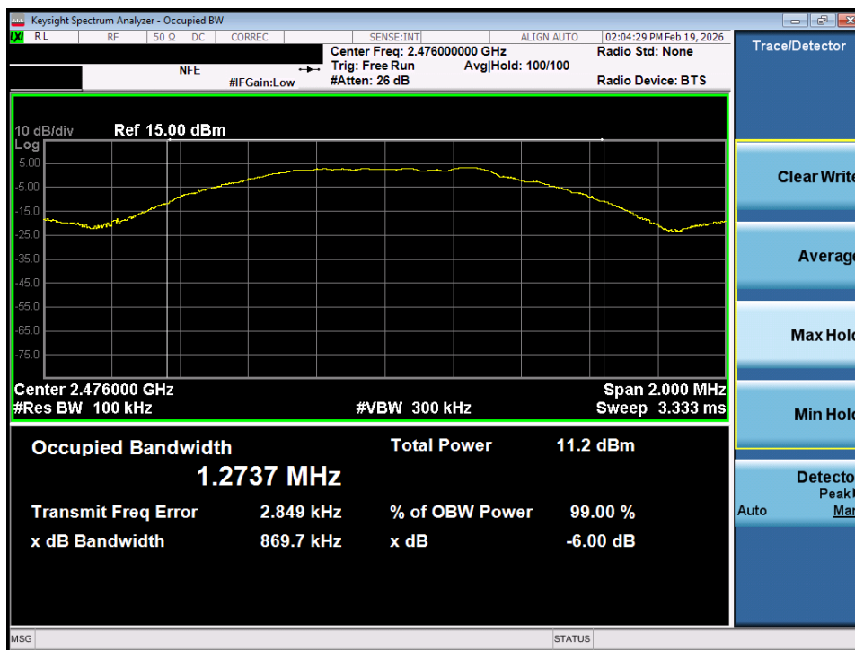
Plot 7-4. 6dB Bandwidth Plot (Bluetooth (LE), 1Mbps – Ch. 35)
