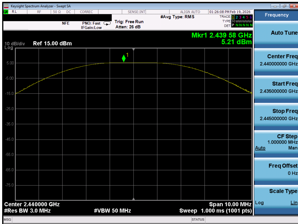
Plot 7-24. Peak Power Plot (Bluetooth (LE), 2Mbps – Ch. 17)
