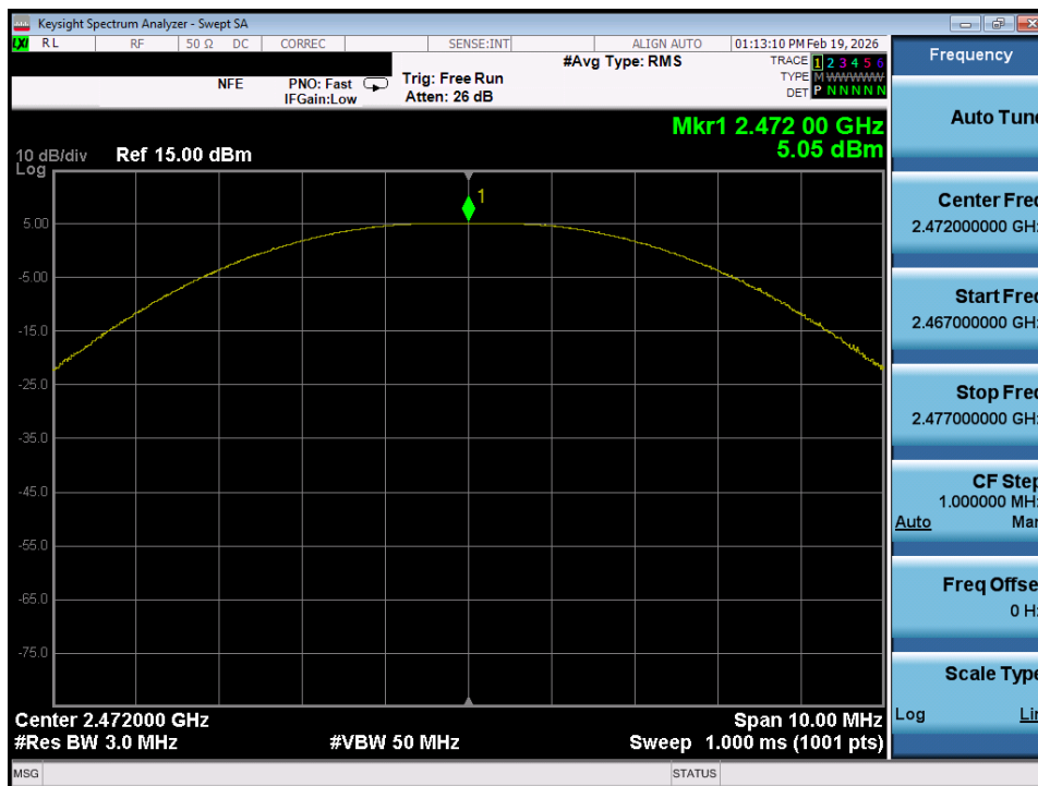
Plot 7-20. Peak Power Plot (Bluetooth (LE), 1Mbps – Ch. 35)
