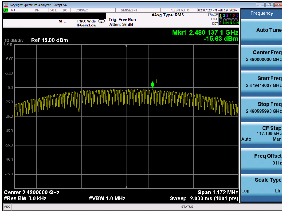
Plot 7-32. Power Spectral Density Plot (Bluetooth (LE), 1Mbps – Ch. 39)
