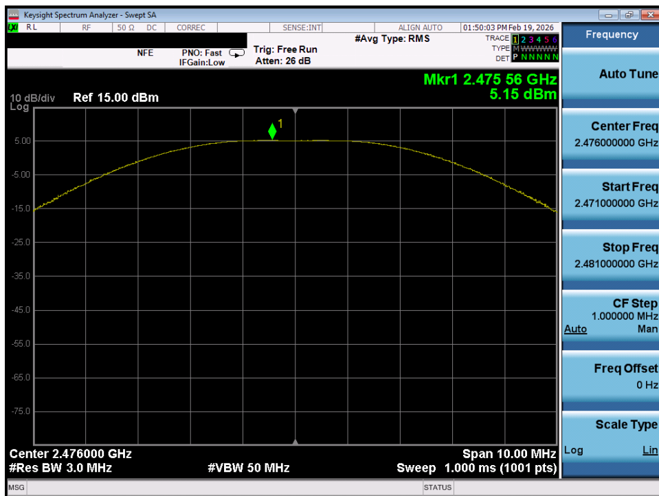
Plot 7-25. Peak Power Plot (Bluetooth (LE), 2Mbps – Ch. 35)
