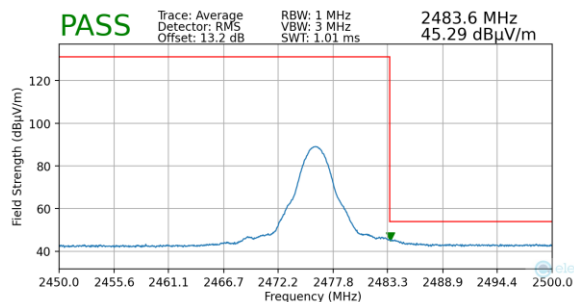
Plot 7-55. Radiated Restricted Upper Band Edge Measurement (Average)
