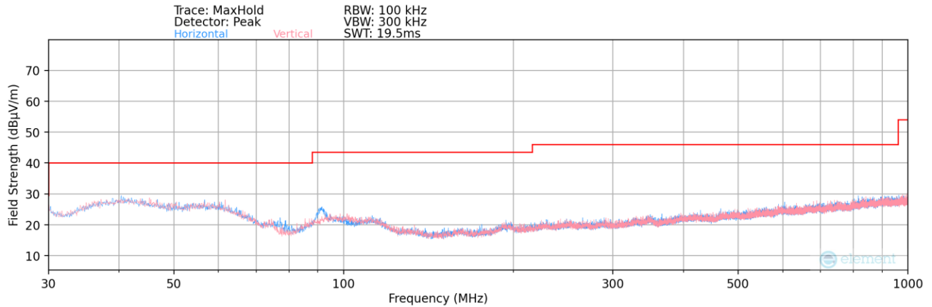
Plot 7-61. Radiated Spurious Plot below 1GHz
