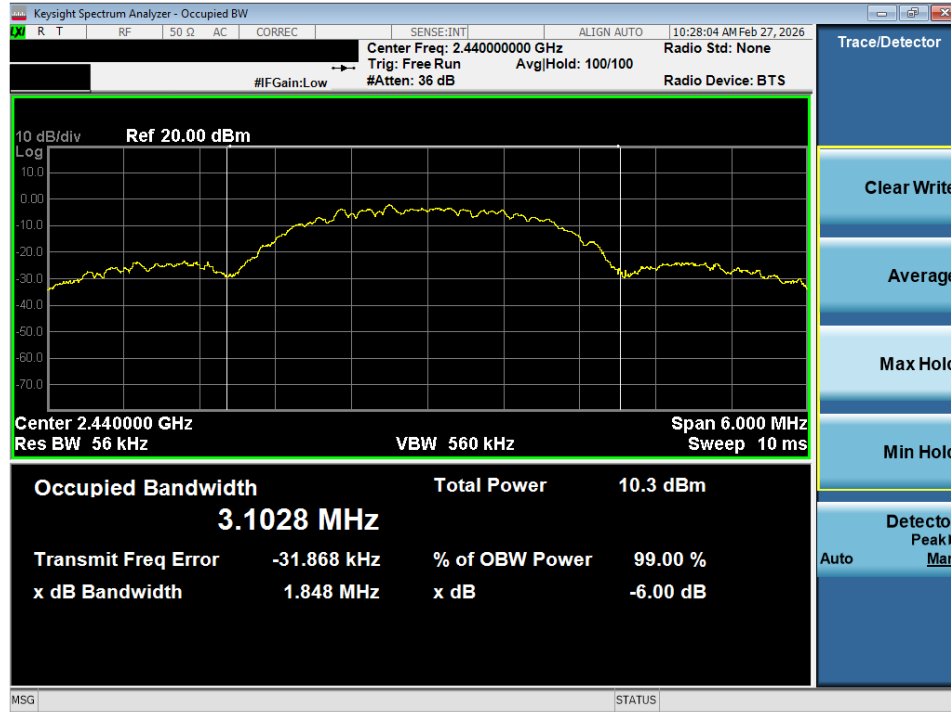
Plot 7-15. OBW Plot (Bluetooth (LE), 2Mbps – Ch. 17)
