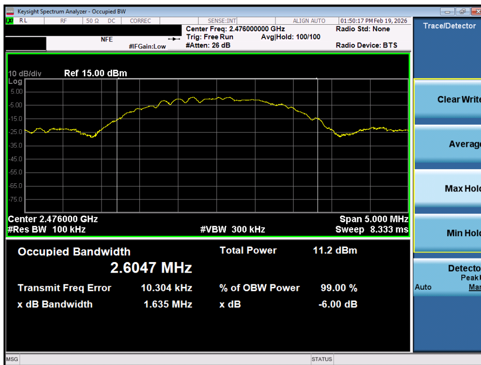
Plot 7-9. 6dB Bandwidth Plot (Bluetooth (LE), 2Mbps – Ch. 35)
