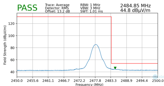
Plot 7-57. Radiated Restricted Upper Band Edge Measurement (Average)
