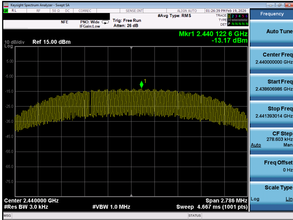
Plot 7-34. Power Spectral Density Plot (Bluetooth (LE), 2Mbps – Ch. 17)
