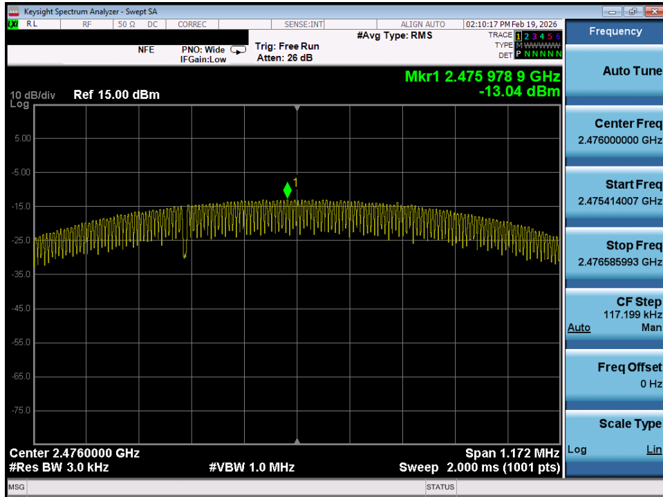
Plot 7-30. Power Spectral Density Plot (Bluetooth (LE), 1Mbps – Ch. 35)
