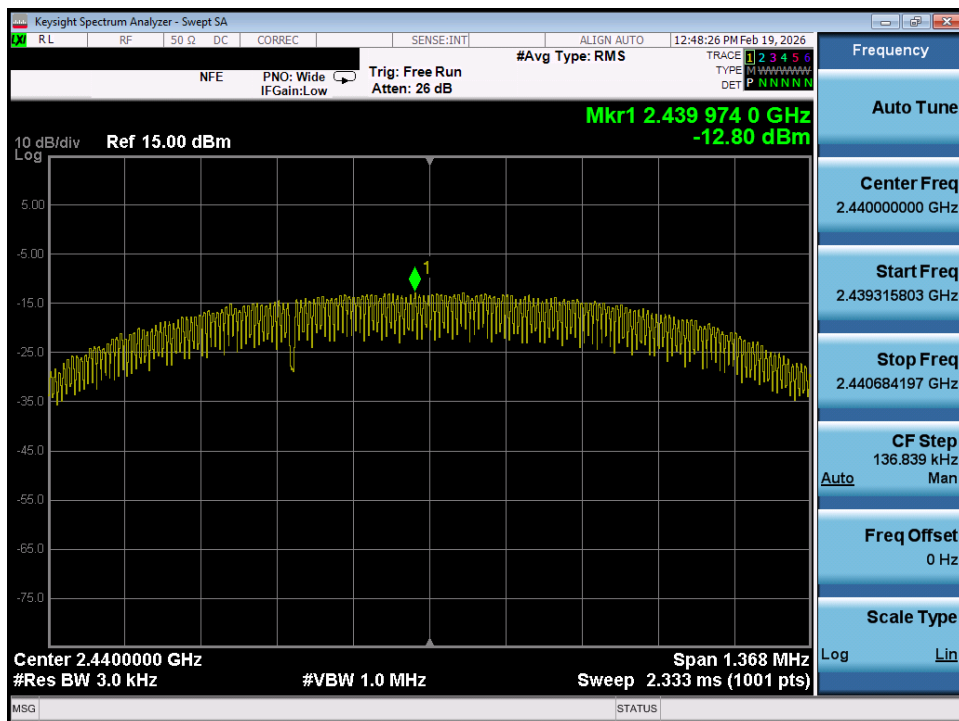
Plot 7-29. Power Spectral Density Plot (Bluetooth (LE), 1Mbps – Ch. 17)
