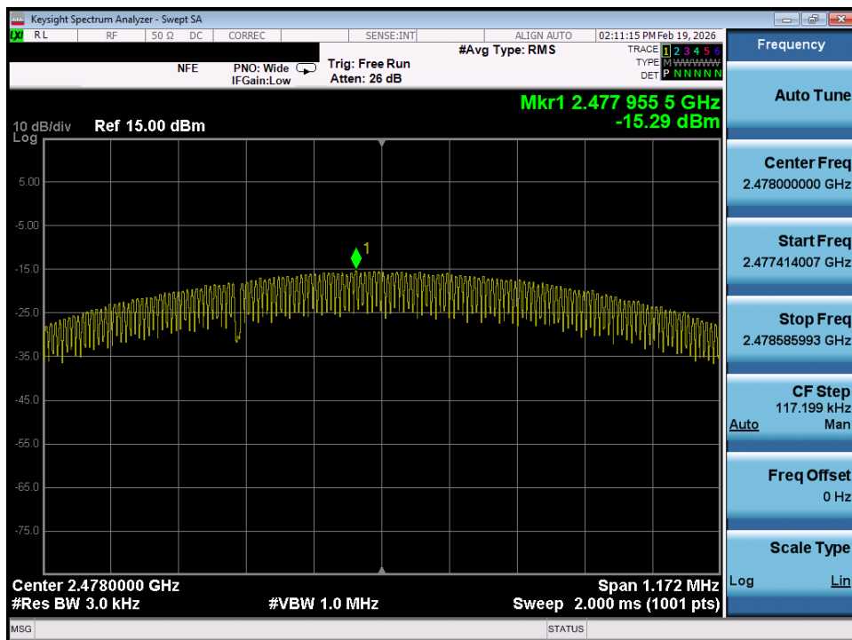
Plot 7-31. Power Spectral Density Plot (Bluetooth (LE), 1Mbps – Ch. 36)
