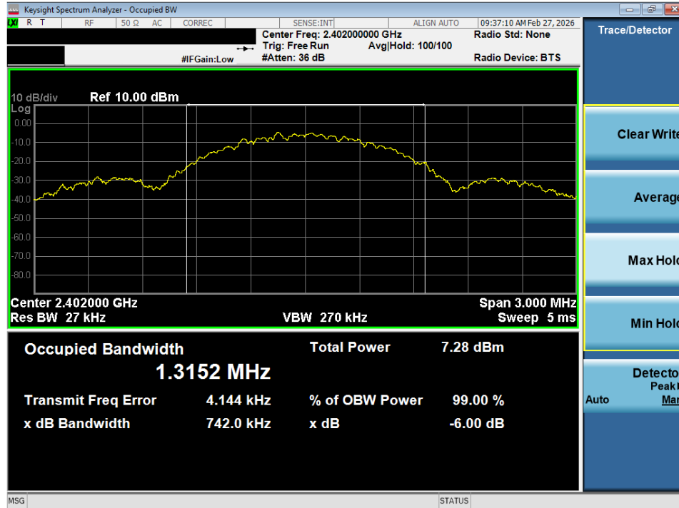
Plot 7-11. OBW Plot (Bluetooth (LE), 1Mbps - Ch. 37)
