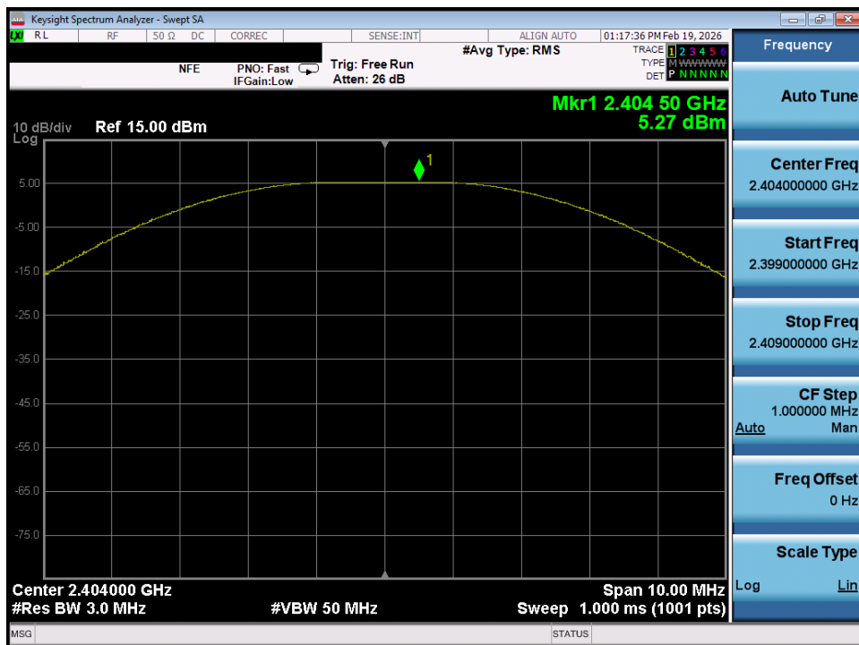
Plot 7-23. Peak Power Plot (Bluetooth (LE), 2Mbps – Ch. 0)
