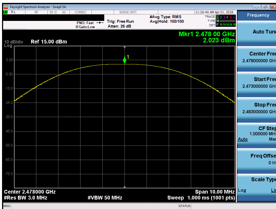
Plot 7-21. Peak Power Plot (Bluetooth (LE), 1Mbps – Ch. 36)
