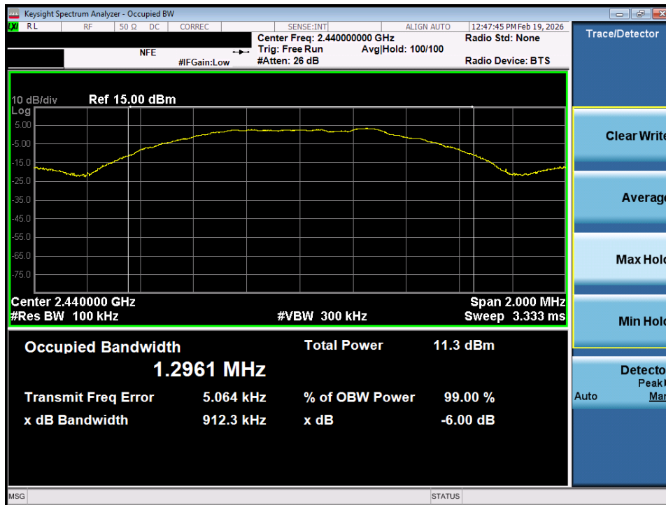
Plot 7-3. 6dB Bandwidth Plot (Bluetooth (LE), 1Mbps – Ch. 17)
