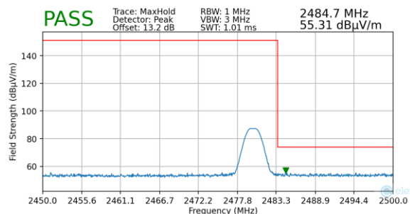
Plot 7-60. Radiated Restricted Upper Band Edge Measurement (Peak)
