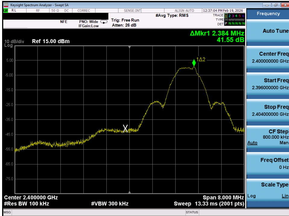
Plot 7-37. Band Edge Plot (Bluetooth (LE), 1Mbps – Ch. 37)
