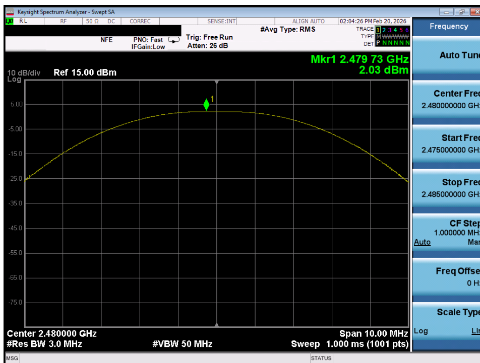
Plot 7-13. Peak Power Plot (ANT+ – Ch. 79)
