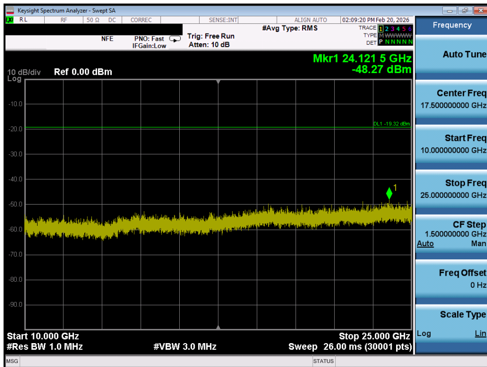
Plot 7-28. Conducted Spurious Plot (ANT+ - Ch. 1)
