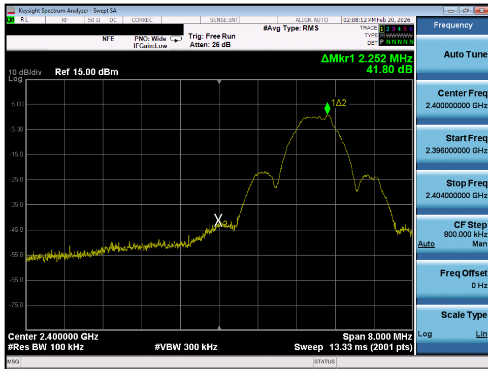
Plot 7-21. Band Edge Plot (ANT+ – Ch. 1)
