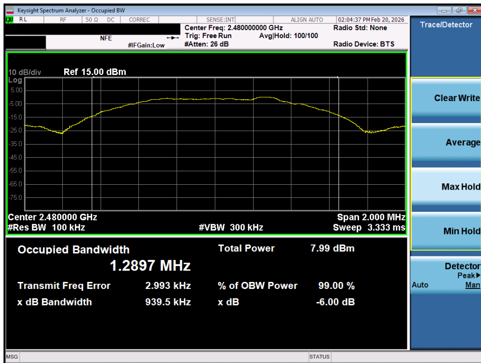
Plot 7-3. 6dB Bandwidth Plot (ANT+ – Ch. 79)
