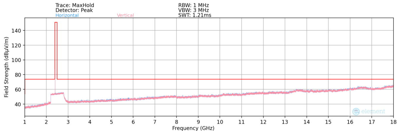
Plot 7-33. Radiated Spurious Plot above 1GHz (ANT+ - Ch. 1)
