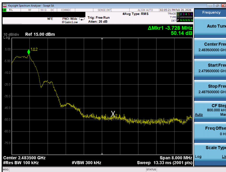
Plot 7-26. Band Edge Plot (ANT+ – Ch. 79)
