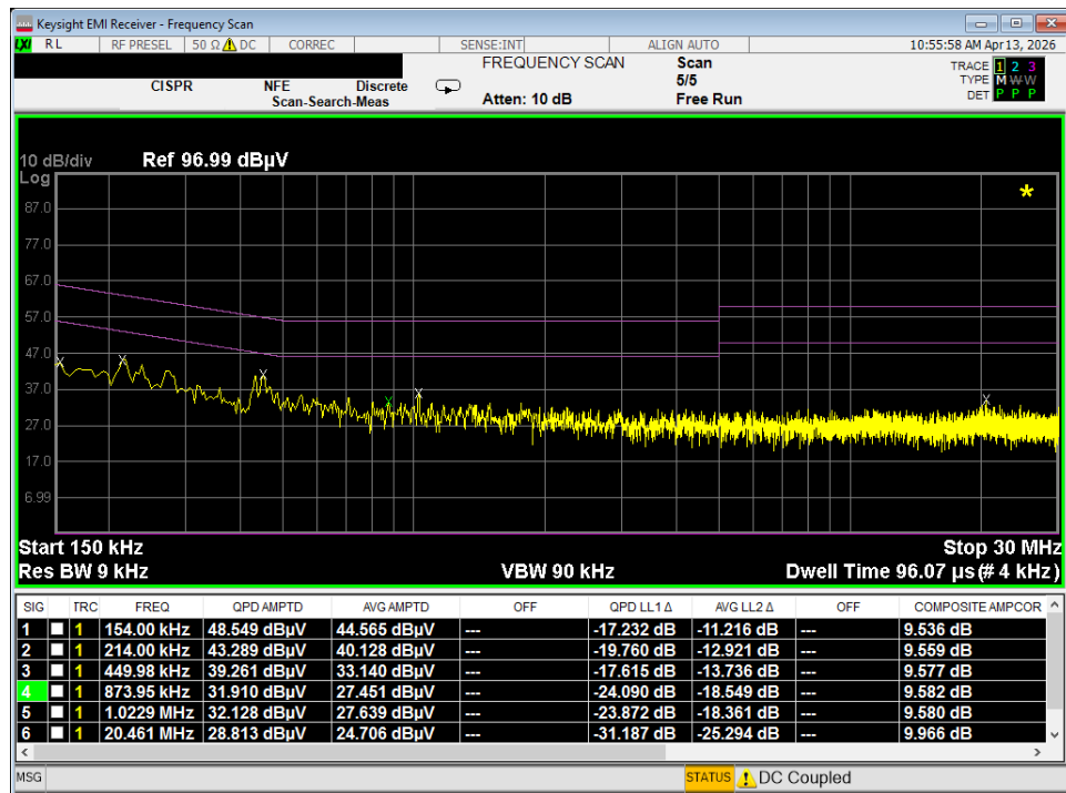
Plot 7-43. Line Conducted Plot with ANT+ (N)
