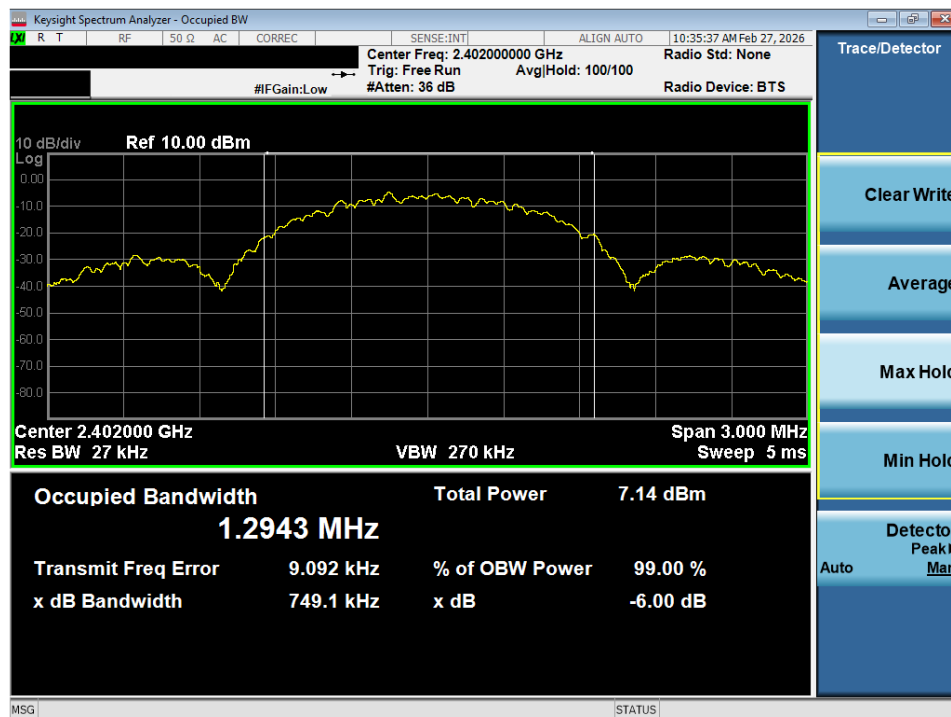
Plot 7-4. Occupied Bandwidth Plot (ANT+ – Ch. 1)
