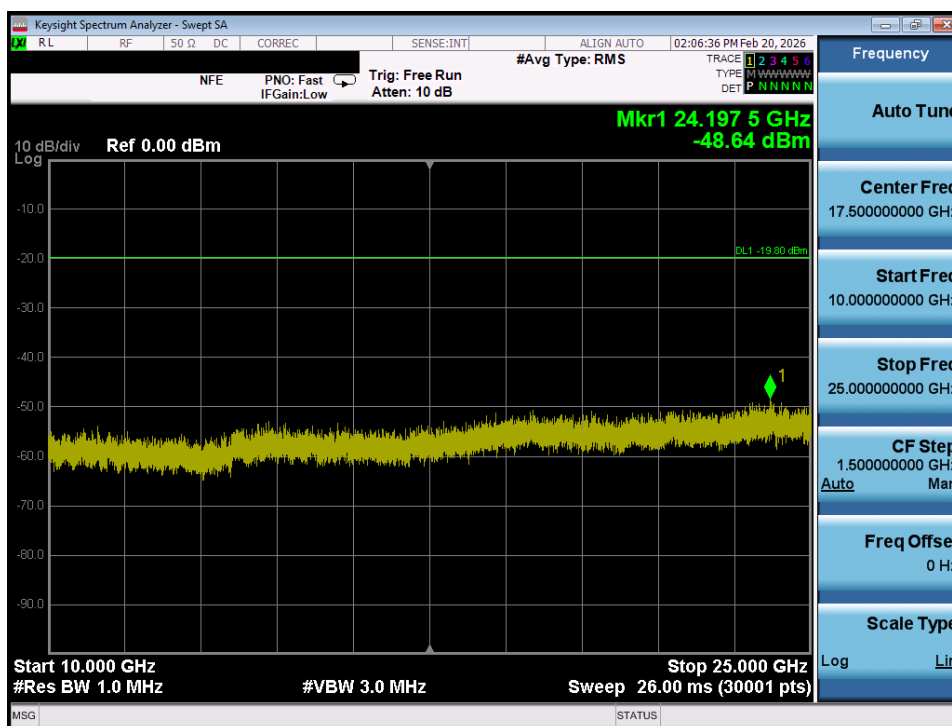
Plot 7-32. Conducted Spurious Plot (ANT+ – Ch. 79)
