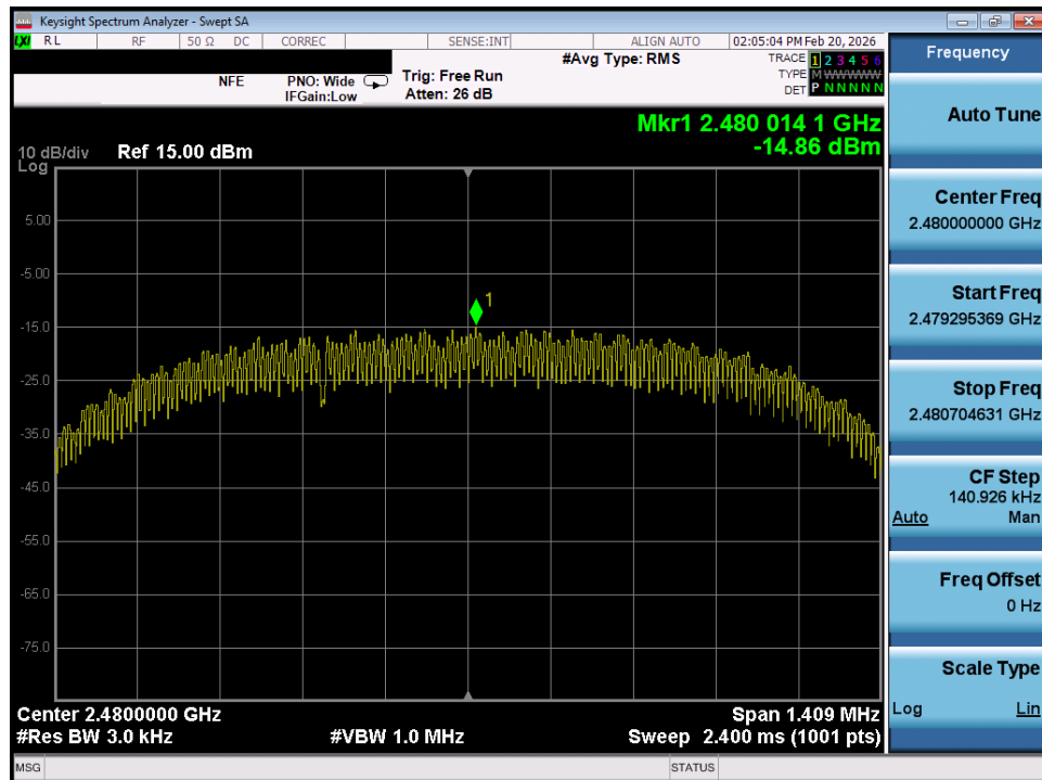
Plot 7-20. Power Spectral Density Plot (ANT+ – Ch. 79)
