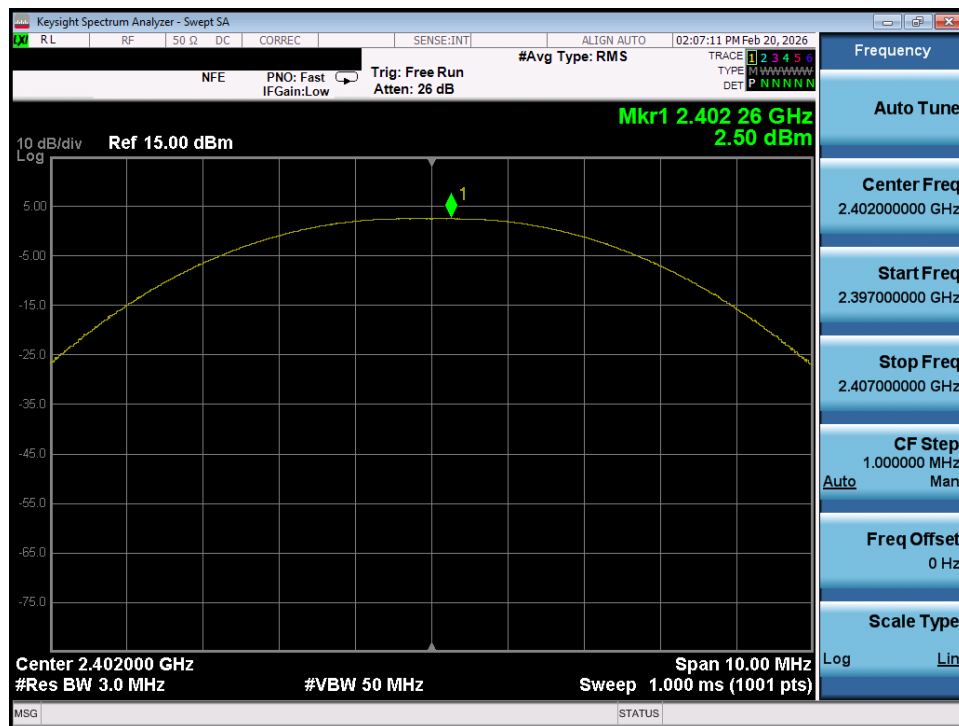
Plot 7-7. Peak Power Plot (ANT+ – Ch. 1)
