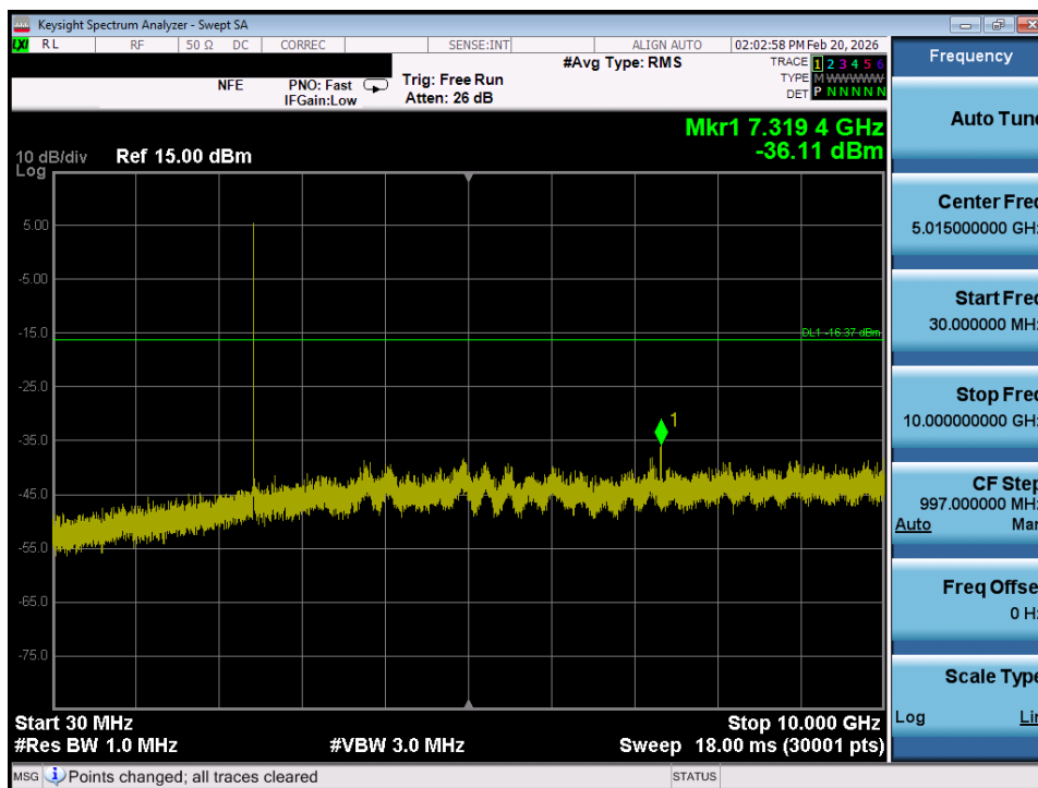
Plot 7-29. Conducted Spurious Plot (ANT+ – Ch. 39)
