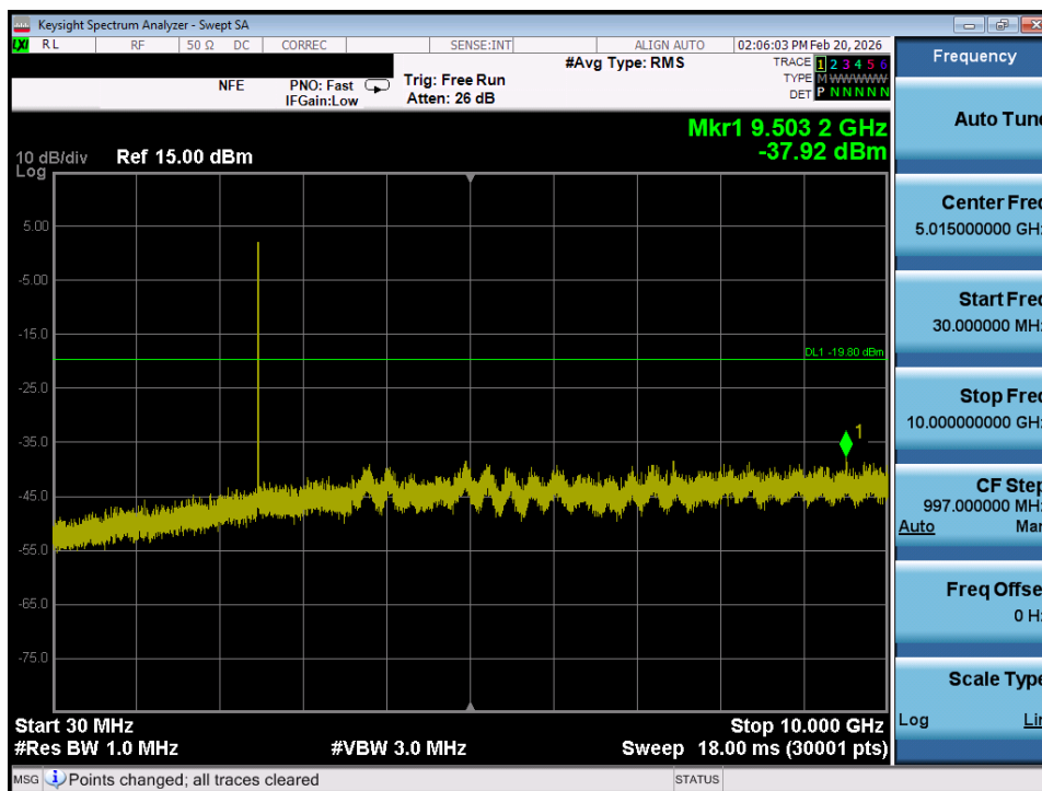
Plot 7-31. Conducted Spurious Plot (ANT+ – Ch. 79)
