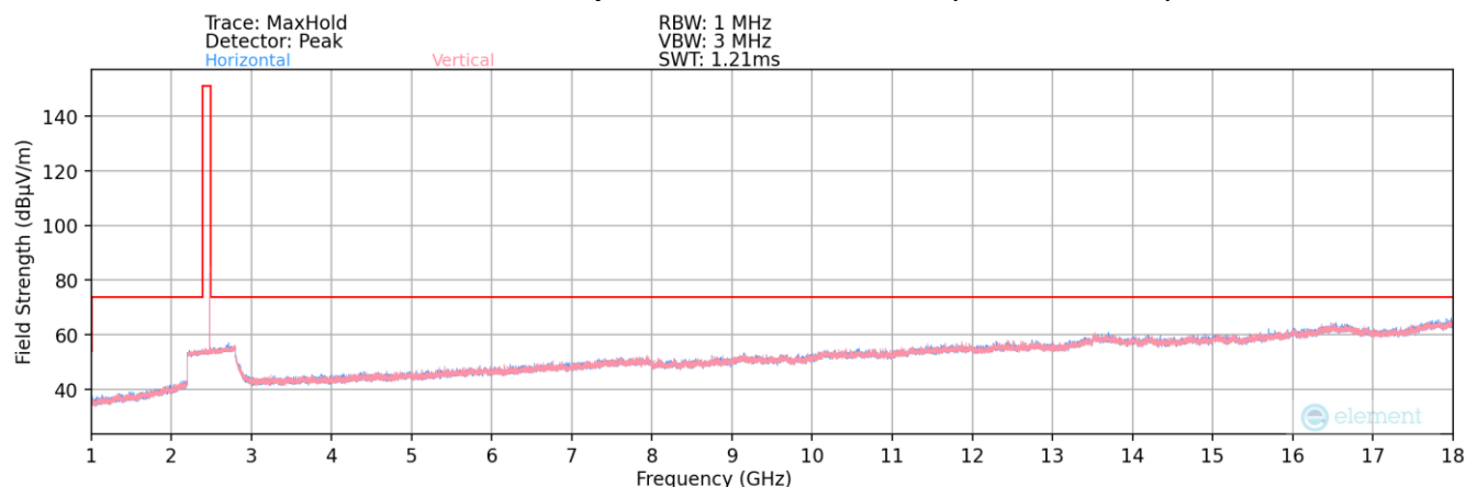
Plot 7-35. Radiated Spurious Plot above 1GHz (ANT+ - Ch. 79)
