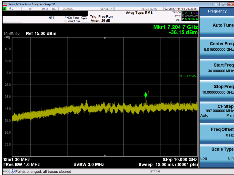
Plot 7-27. Conducted Spurious Plot (ANT+ - Ch. 1)
