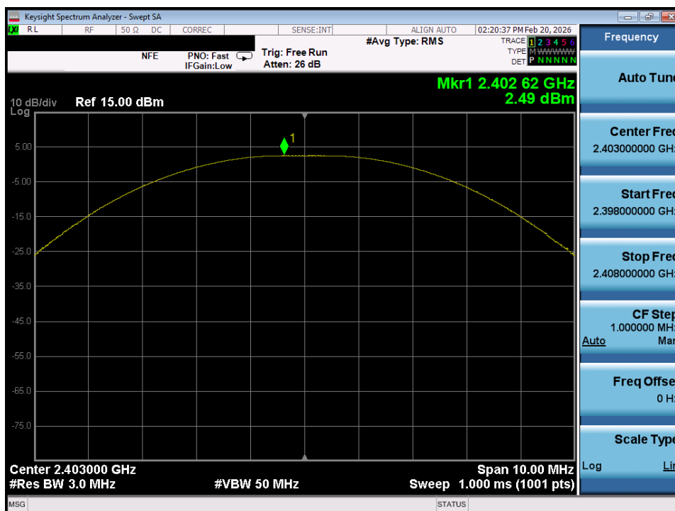
Plot 7-8. Peak Power Plot (ANT+ – Ch. 2)
