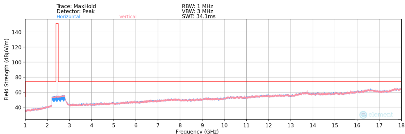
Plot 7-34. Radiated Spurious Plot above 1GHz (ANT+ - Ch. 39)
