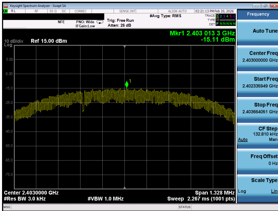
Plot 7-15. Power Spectral Density Plot (ANT+ – Ch. 2)
