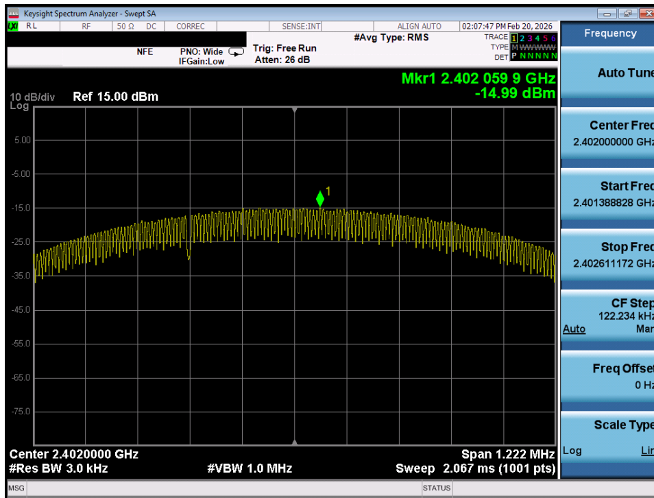
Plot 7-14. Power Spectral Density Plot (ANT+ – Ch. 1)
