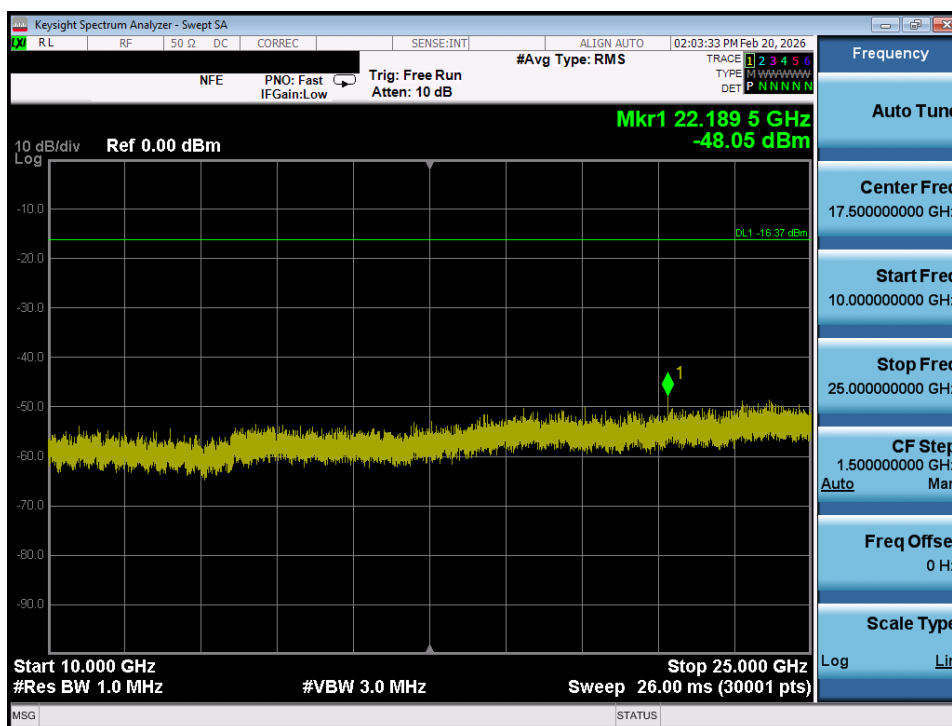
Plot 7-30. Conducted Spurious Plot (ANT+ – Ch. 39)
