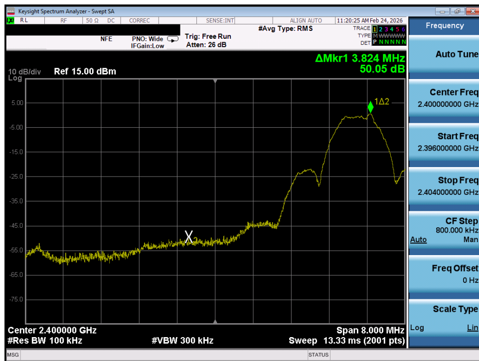
Plot 7-22. Band Edge Plot (ANT+ – Ch. 2)
