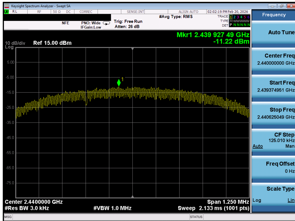
Plot 7-17. Power Spectral Density Plot (ANT+ – Ch. 39)
