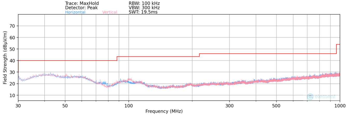
Plot 7-41. Radiated Spurious Plot below 1GHz
