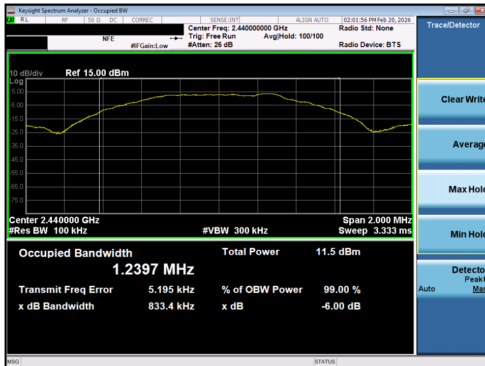
Plot 7-2. 6dB Bandwidth Plot (ANT+ – Ch. 39)
