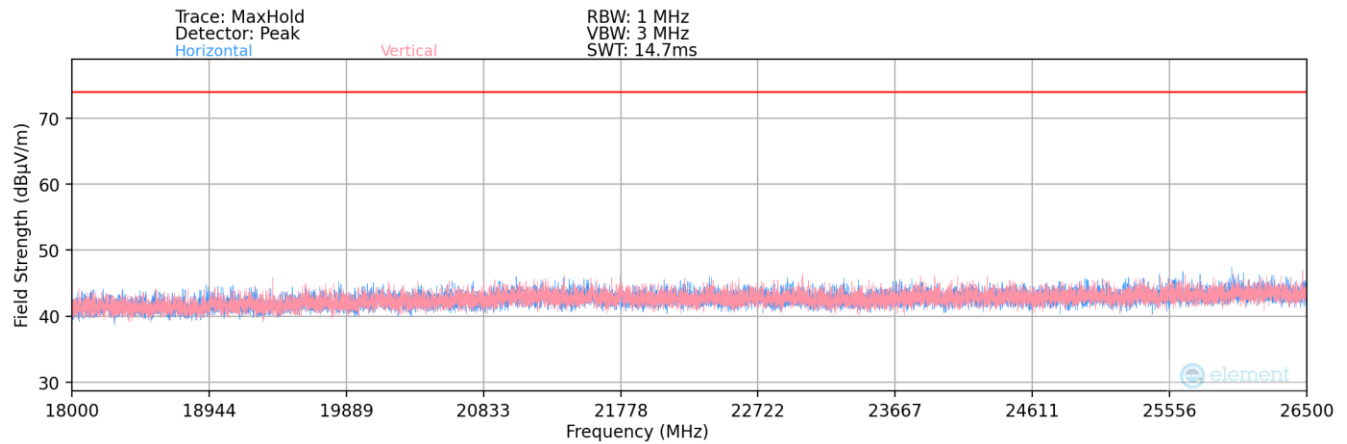
Plot 7-36. Radiated Spurious Plot above 18GHz (ANT+ – Ch. 39)
