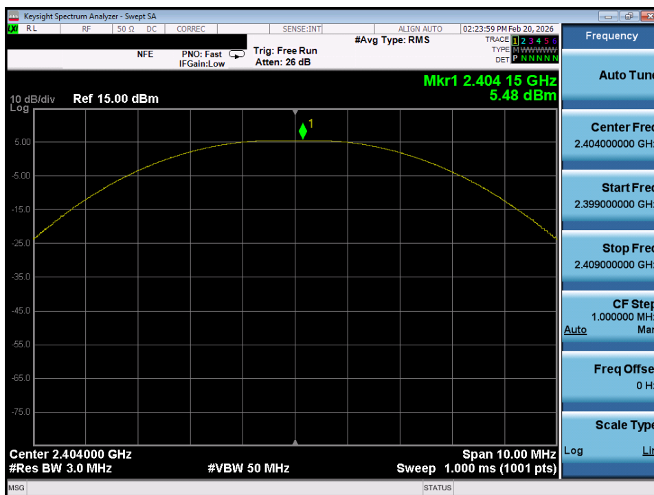
Plot 7-9. Peak Power Plot (ANT+ – Ch. 3)
