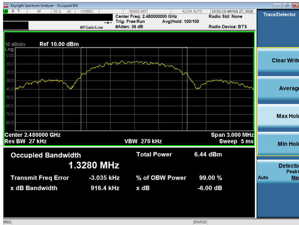
Plot 7-6. Occupied Bandwidth Plot (ANT+ – Ch. 79)
