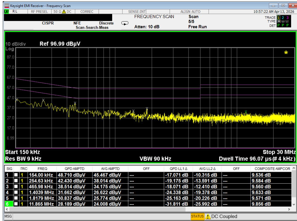
Plot 7-42. Line Conducted Plot with ANT+ (L1)
