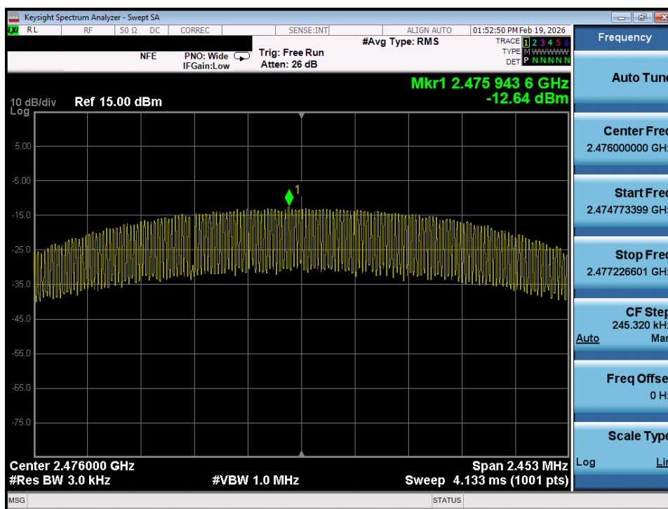
Plot 7-35. Power Spectral Density Plot (Bluetooth (LE), 2Mbps – Ch. 35)
