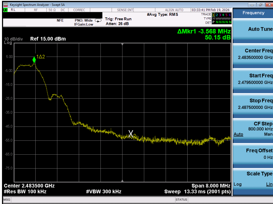
Plot 7-41. Band Edge Plot (Bluetooth (LE), 1Mbps – Ch. 39)
