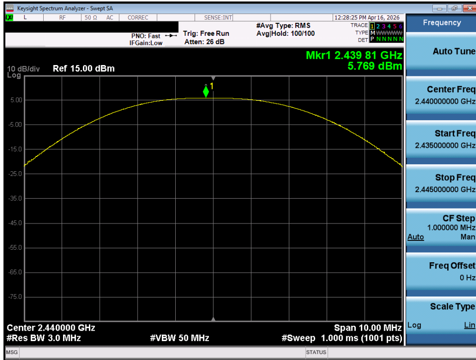
Plot 9-2. Conducted Output Power Measurements (Spot-check)
