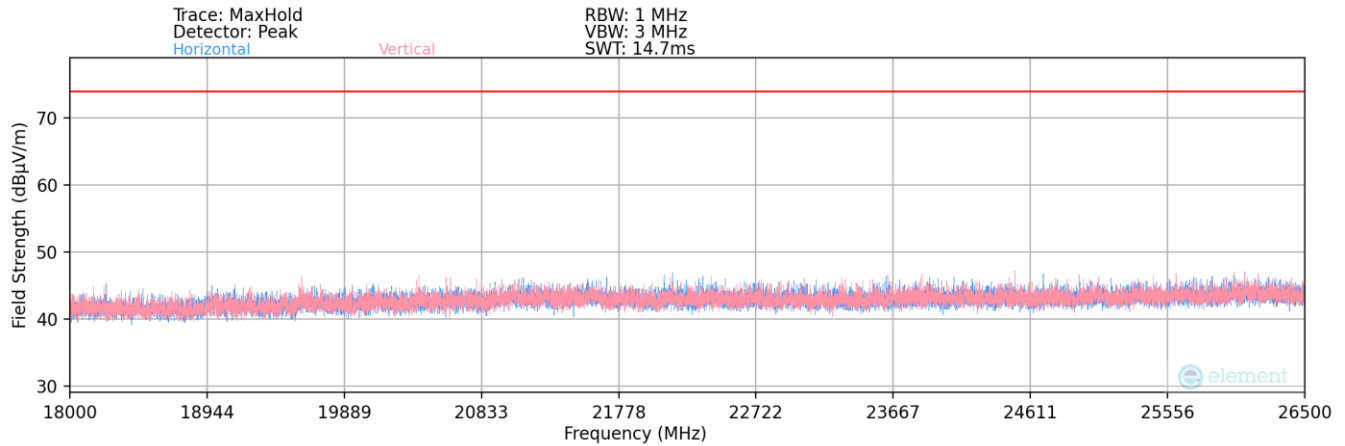
Plot 7-57. Radiated Spurious Plot above 18GHz
