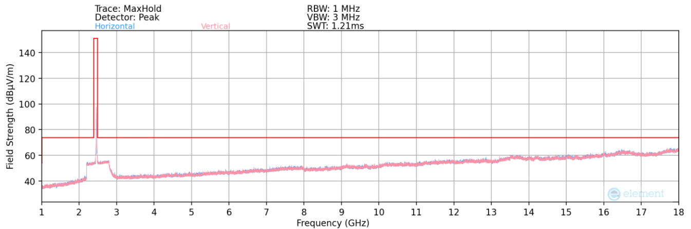
Plot 7-56. Radiated Spurious Plot above 1GHz (802.11b – Ch. OFDM 11)
