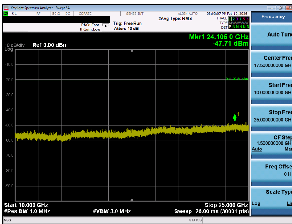
Plot 7-52. Conducted Spurious Plot (802.11b – Ch. 11)
