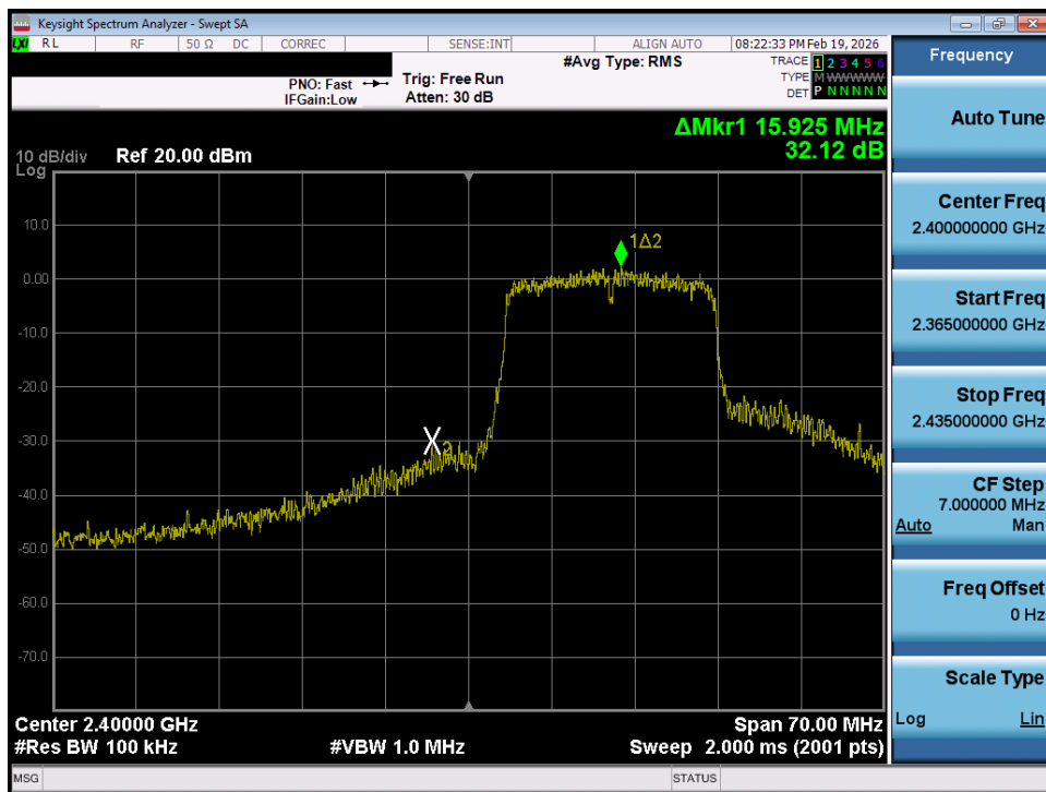
Plot 7-41. Band Edge Plot (802.11n – Ch. 1)
