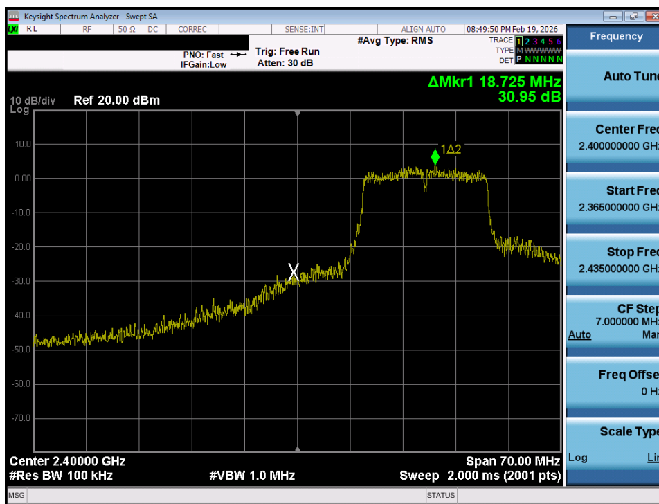
Plot 7-35. Band Edge Plot (802.11g- Ch. 2)
