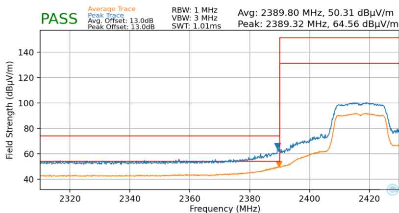
Plot 7-59. Radiated Restricted Lower Band Edge Measurement (Average & Peak)
