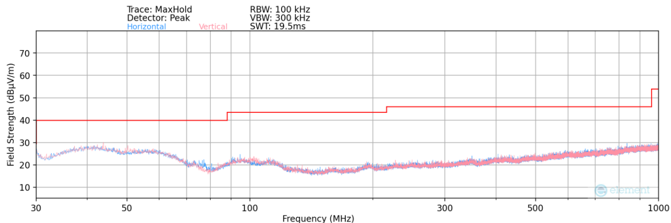
Plot 7-53. Radiated Spurious Plot below 1GHz
