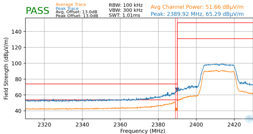
Plot 7-58. Radiated Restricted Lower Band Edge Measurement (Average & Peak)
