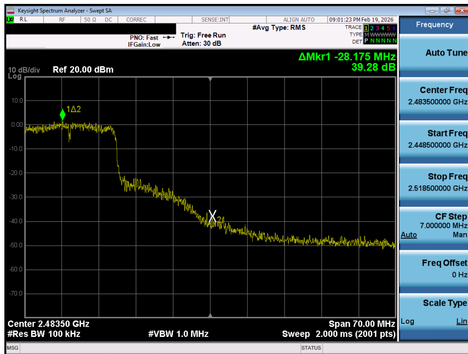
Plot 7-43. Band Edge Plot (802.11n – Ch. 10)
