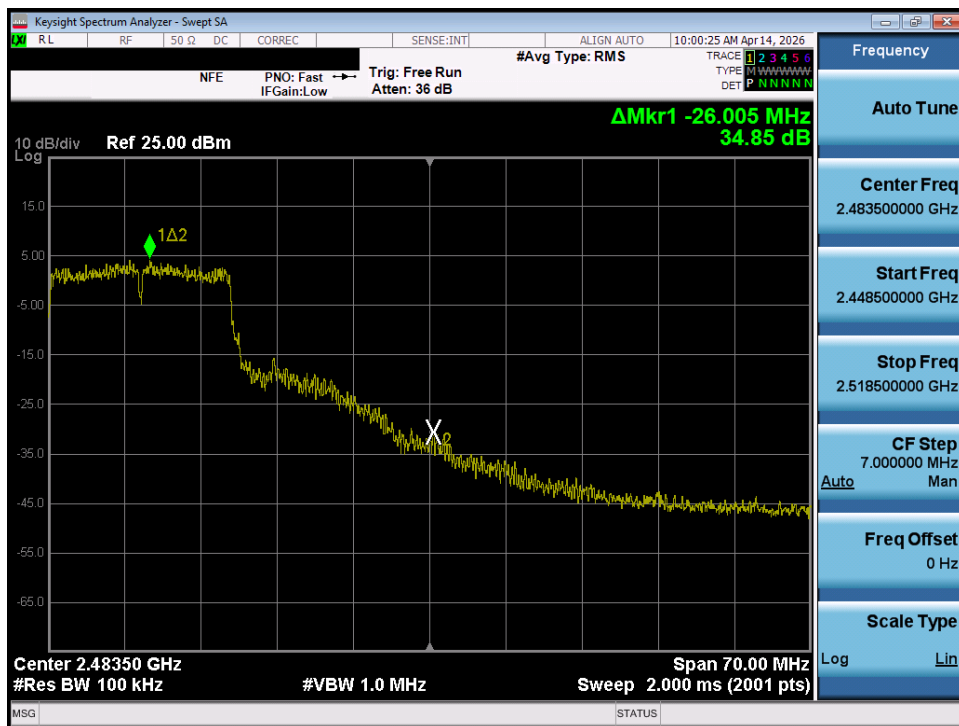
Plot 7-37. Band Edge Plot (802.11g – Ch. 10)
