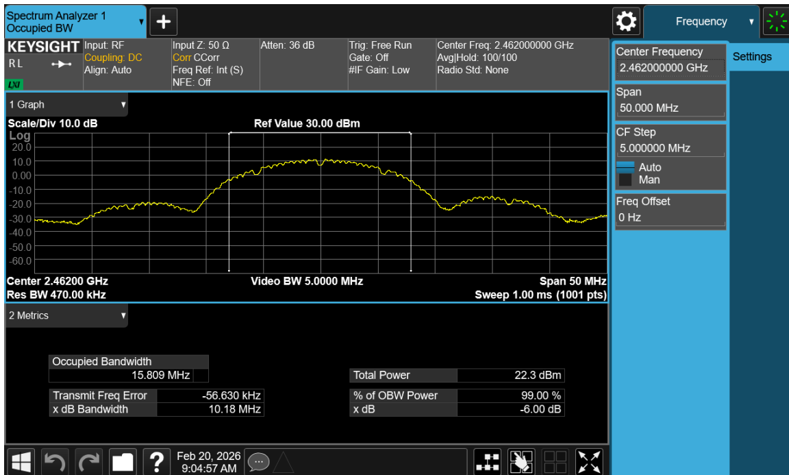
Plot 7-12. OBW Plot SISO ANT1 (802.11b – Ch. 11)
