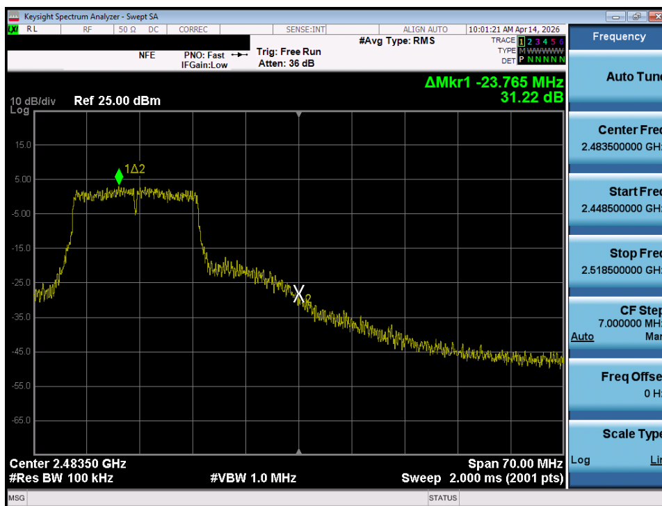
Plot 7-38. Band Edge Plot (802.11g – Ch. 11)
