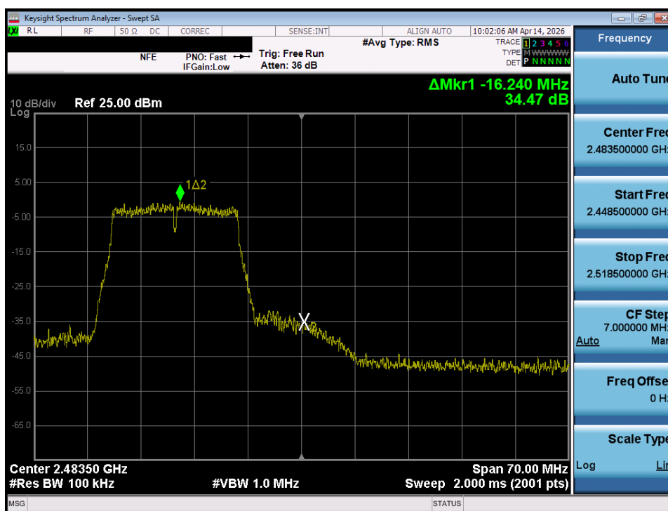
Plot 7-39. Band Edge Plot (802.11g – Ch. 12)
