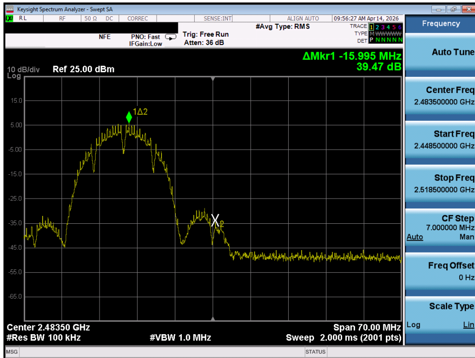
Plot 7-32. Band Edge Plot (802.11b – Ch. 12)
