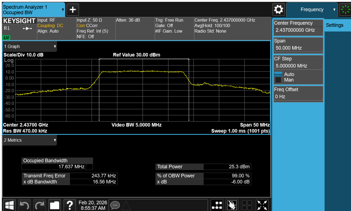
Plot 7-14. OBW Plot SISO ANT1 (802.11g – Ch. 6)
