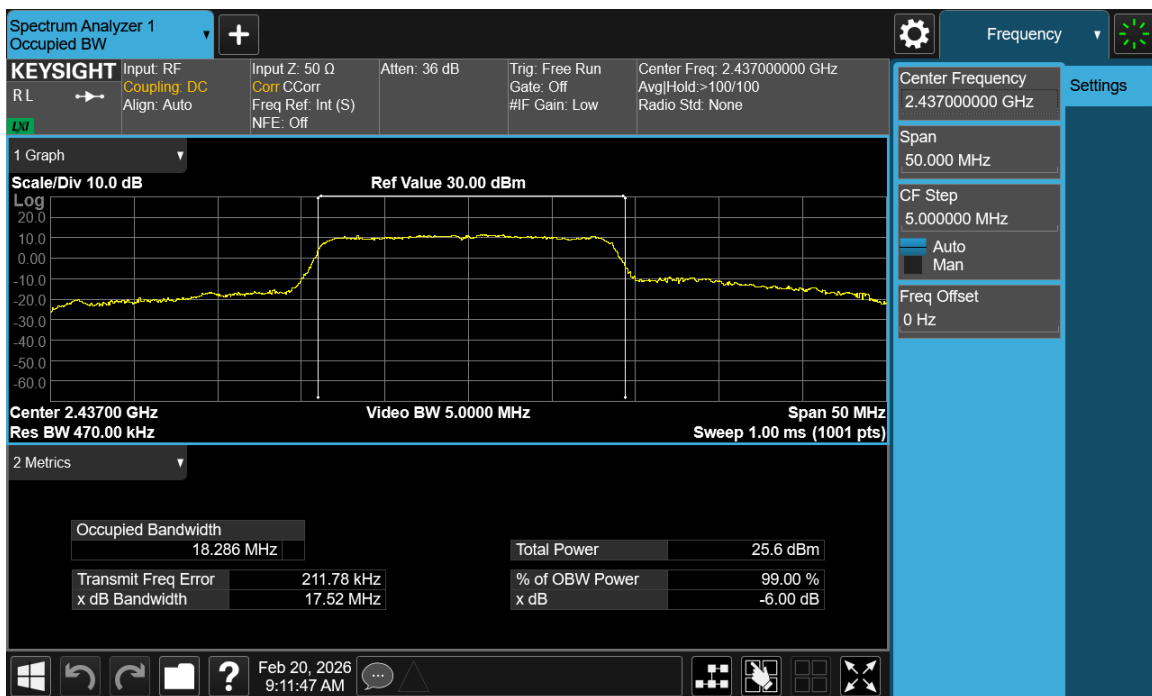
Plot 7-17. OBW Plot SISO ANT1 (802.11n- Ch. 6)
