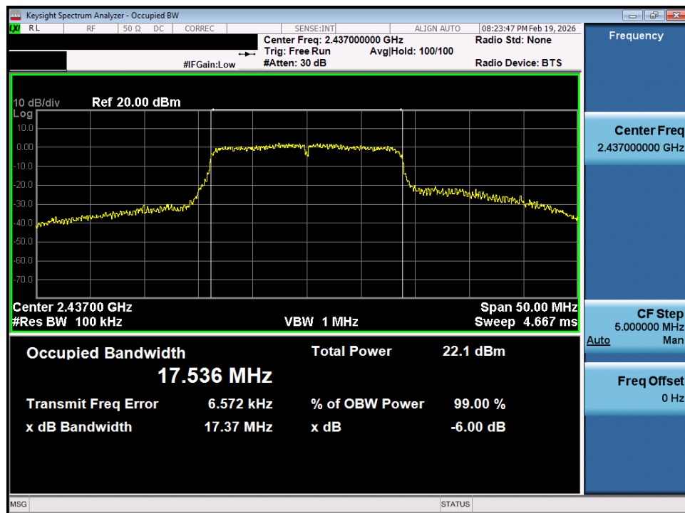
Plot 7-8. 6dB Bandwidth Plot (802.11n – Ch. 6)
