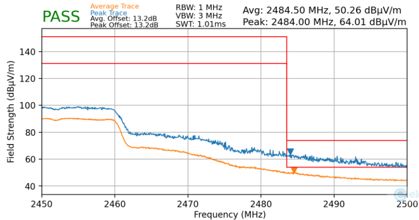
Plot 7-60. Radiated Restricted Upper Band Edge Measurement (Average & Peak)
