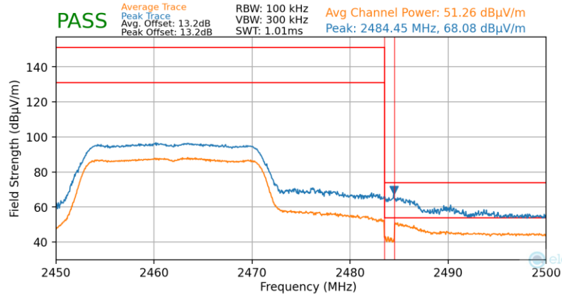
Plot 7-62. Radiated Restricted Upper Band Edge Measurement (Average & Peak)
