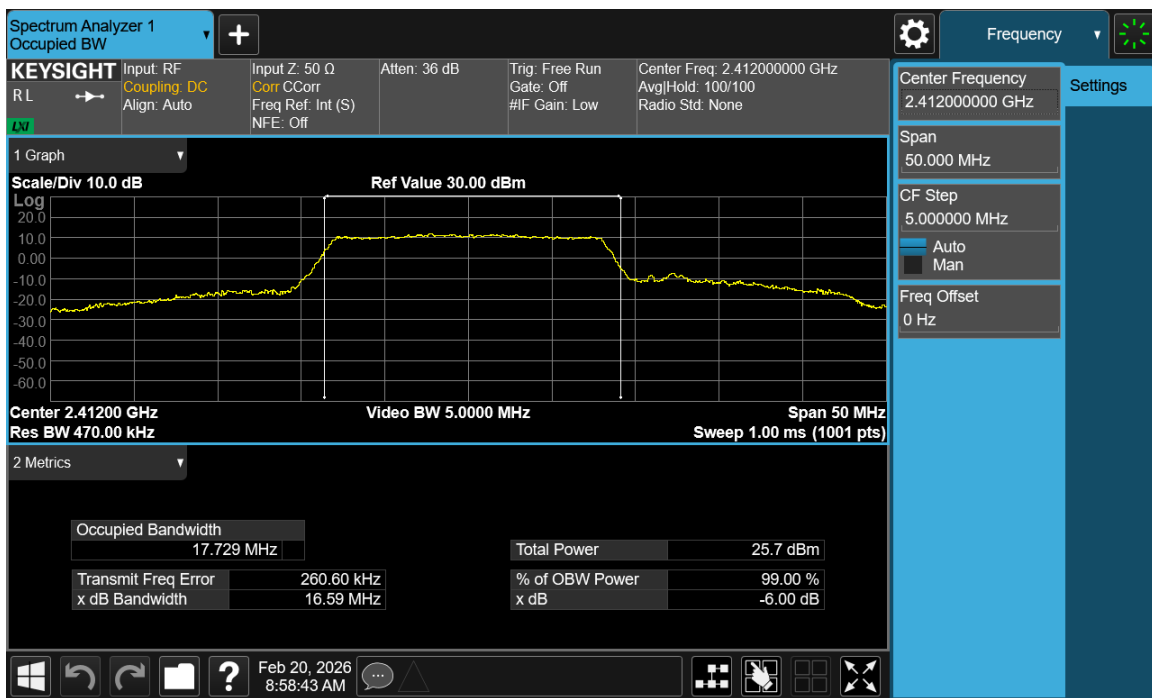
Plot 7-13. OBW Plot SISO ANT1 (802.11g – Ch. 1)
