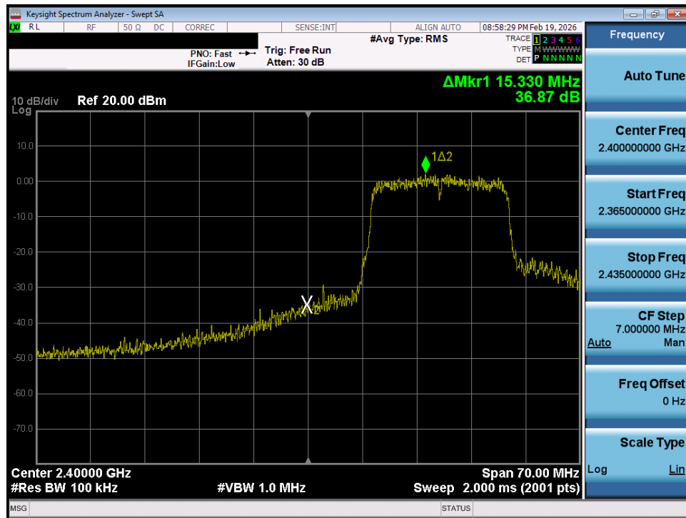
Plot 7-42. Band Edge Plot (802.11n – Ch. 2)
