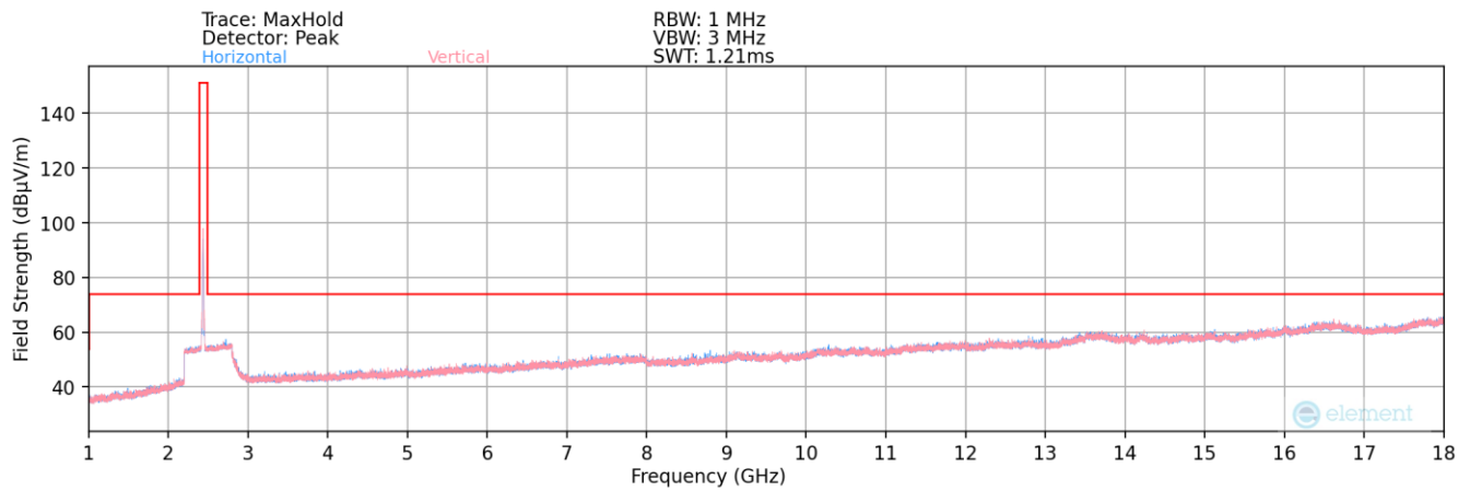
Plot 7-55. Radiated Spurious Plot above 1GHz (802.11b – Ch. OFDM 6)
