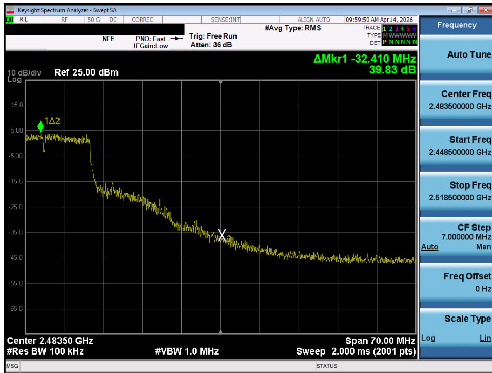
Plot 7-36. Band Edge Plot (802.11g – Ch. 9)
