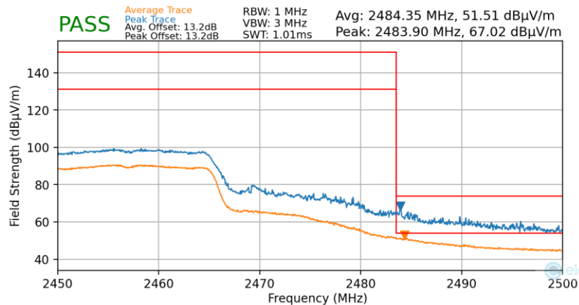
Plot 7-61. Radiated Restricted Upper Band Edge Measurement (Average & Peak)
