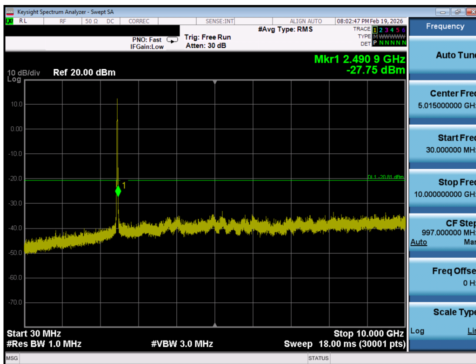
Plot 7-51. Conducted Spurious Plot (802.11b – Ch. 11)
