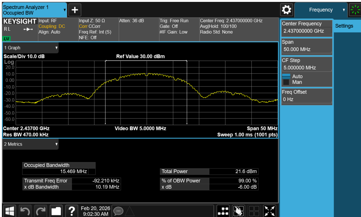
Plot 7-11. OBW Plot SISO ANT1 (802.11b – Ch. 6)
