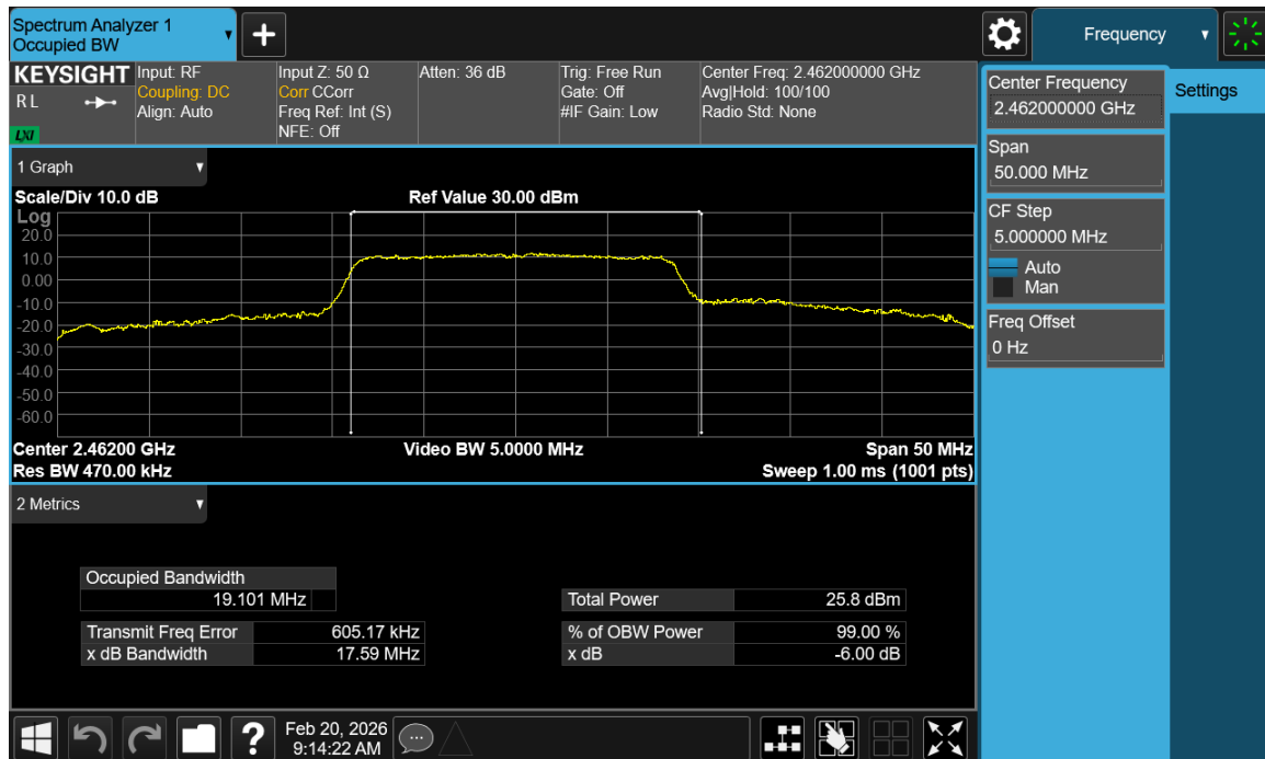
Plot 7-18. OBW Plot SISO ANT1 (802.11n – Ch. 11)
