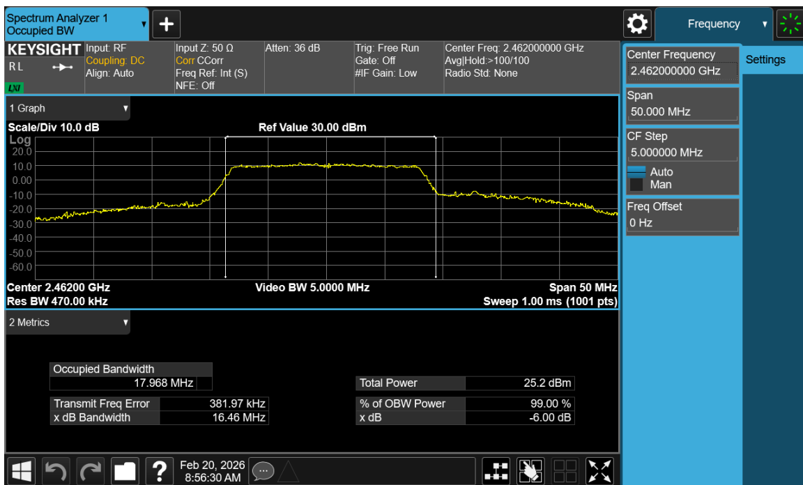
Plot 7-15. OBW Plot SISO ANT1 (802.11g – Ch. 11)
