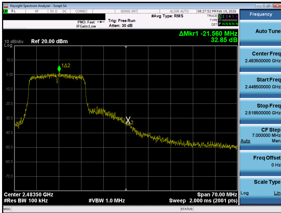
Plot 7-44. Band Edge Plot (802.11n – Ch. 11)
