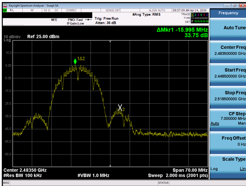
Plot 7-33. Band Edge Plot (802.11b – Ch. 13)
