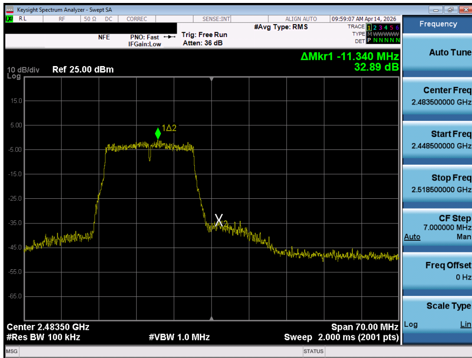
Plot 7-40. Band Edge Plot (802.11g – Ch. 13)
