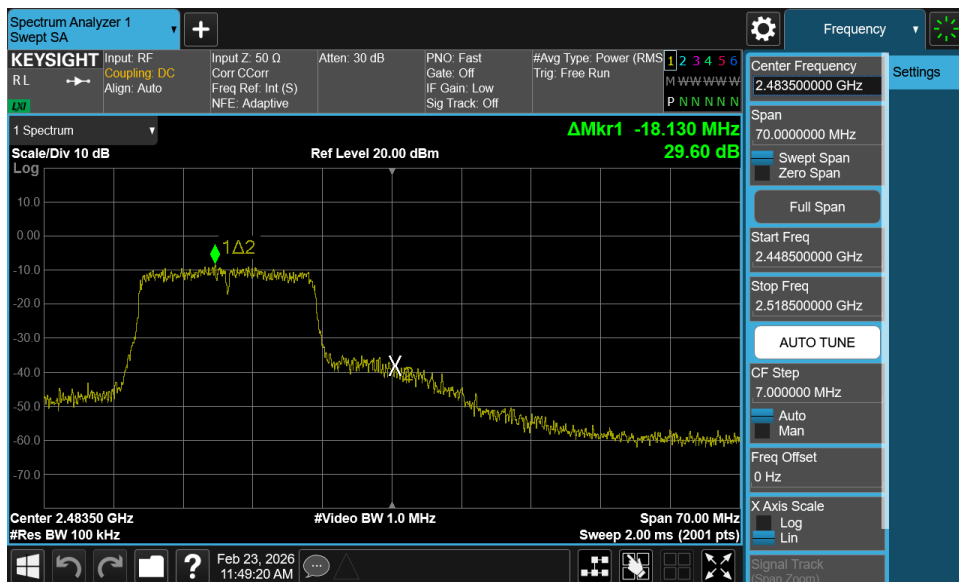
Plot 7-45. Band Edge Plot (802.11n – Ch. 12)
