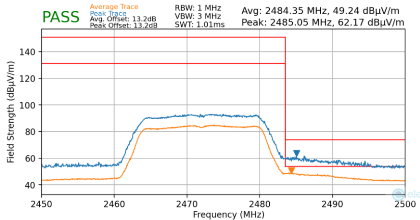
Plot 7-64. Radiated Restricted Upper Band Edge Measurement (Average & Peak)
