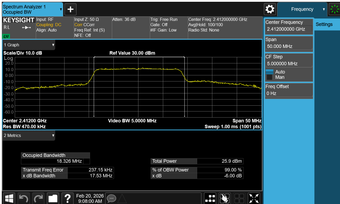
Plot 7-16. OBW Plot SISO ANT1 (802.11n- Ch. 1)
