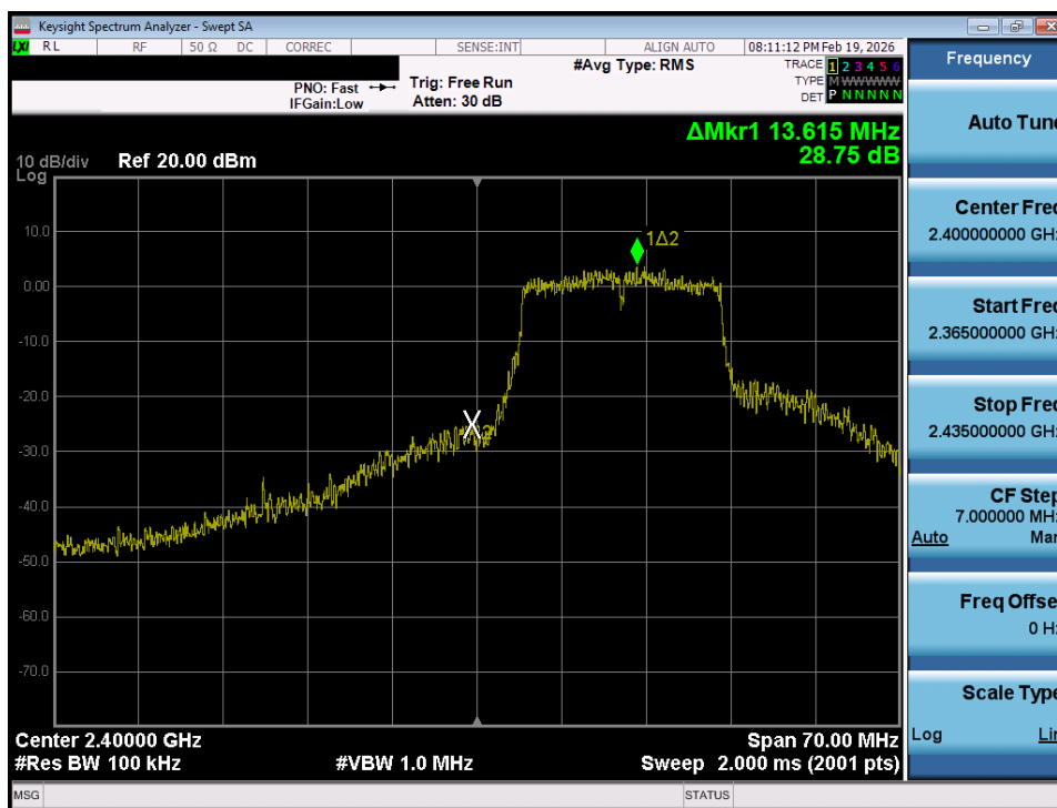
Plot 7-34. Band Edge Plot (802.11g- Ch. 1)
