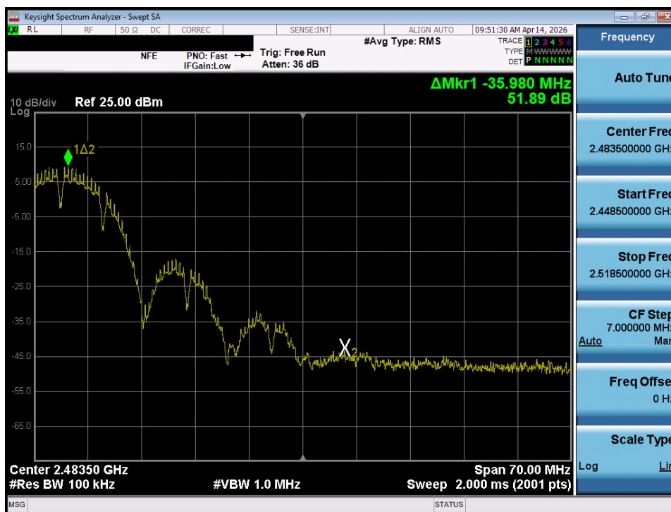
Plot 7-29. Band Edge Plot (802.11b – Ch. 9)
