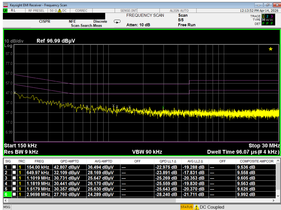
Plot 7-66. Line Conducted Plot with 802.11b (N)
