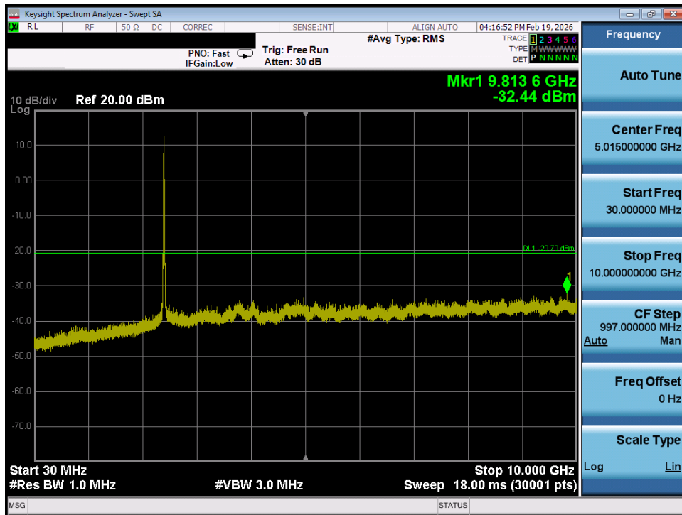
Plot 7-47. Conducted Spurious Plot (802.11b – Ch. 1)
