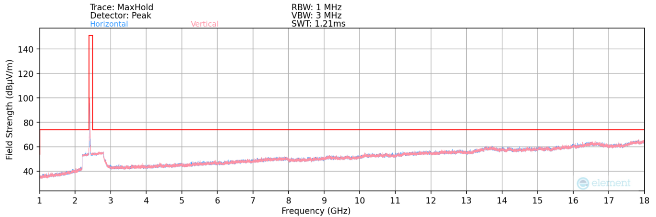
Plot 7-54. Radiated Spurious Plot above 1GHz (802.11b – Ch. OFDM 1)
