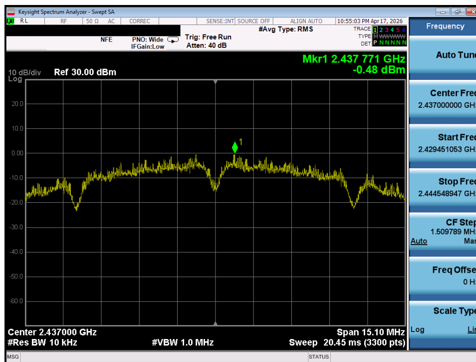
Plot 9-3. Power Spectral Density Plot (Spot-check)
