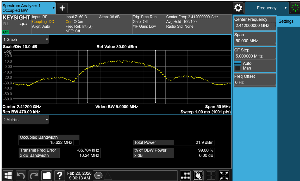
Plot 7-10. OBW Plot SISO ANT1 (802.11b – Ch. 1)
