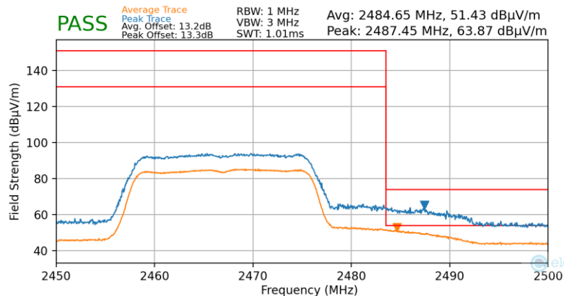
Plot 7-63. Radiated Restricted Upper Band Edge Measurement (Average & Peak)
