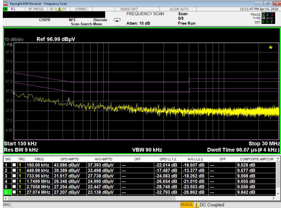
Plot 7-65. Line Conducted Plot with 802.11b (L1)
